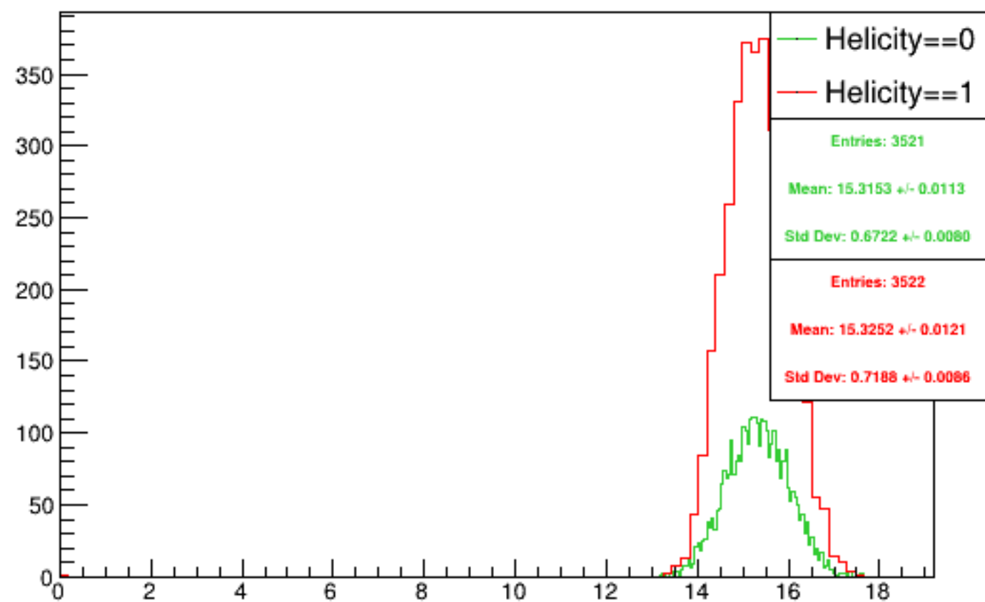
Run 5972 mpwise, acc0: Beam ON, Laser ON
