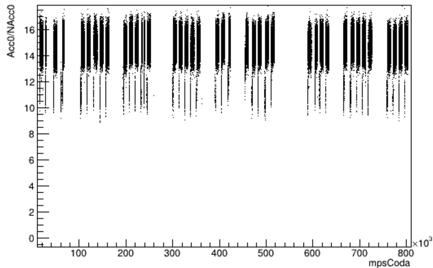
Run 5979 mpwise, Acc0 vs Time: Beam ON, Laser ON
