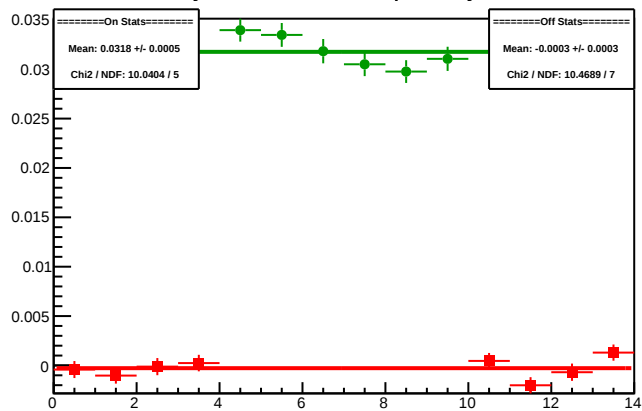
Cycle 5979.11: Multiplet Asyms
