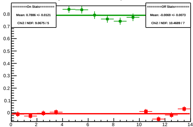
Cycle 5979.11: Multiplet Diffs
