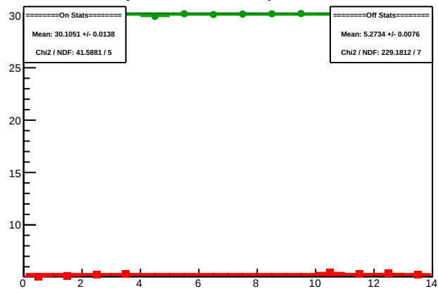
Cycle 5979.11: Multiplet Sums
