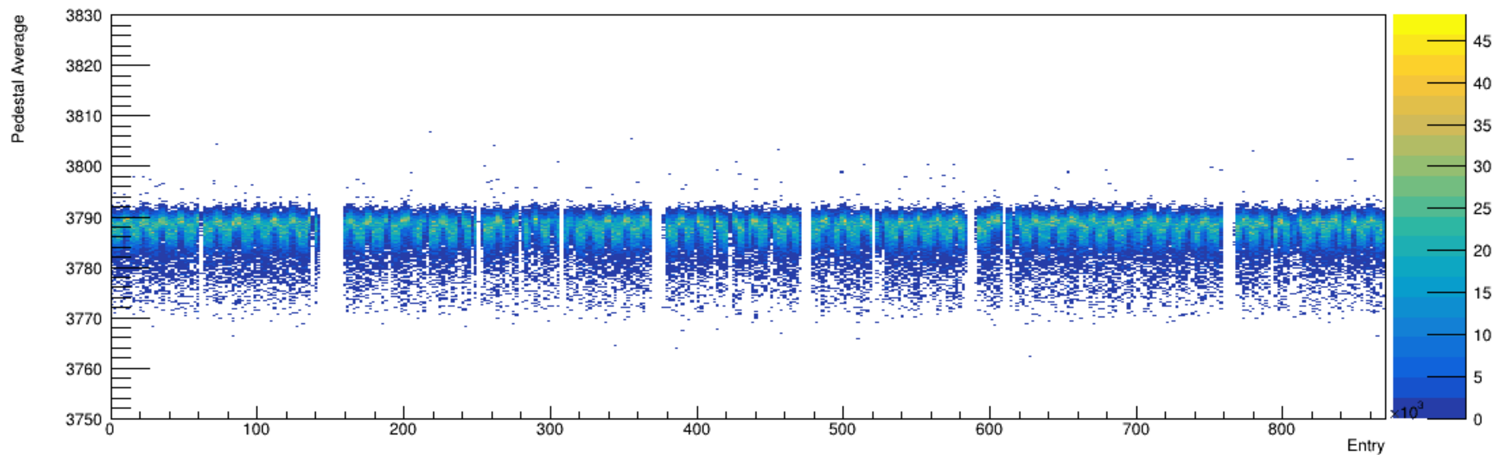
Run 5986, snapshots: Pedestal vs. Time
