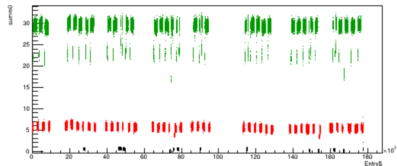
Run 5987 quartetwise, summ0 vs time
