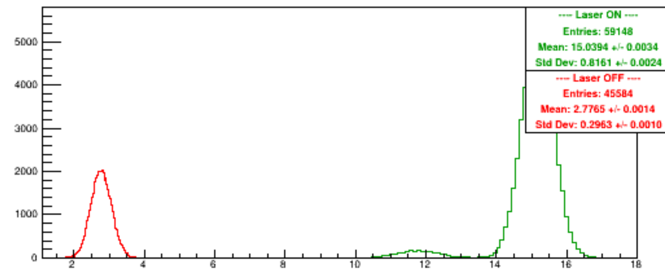
Run 5987 quartetwise, NegHelAcc0/NSamples0
