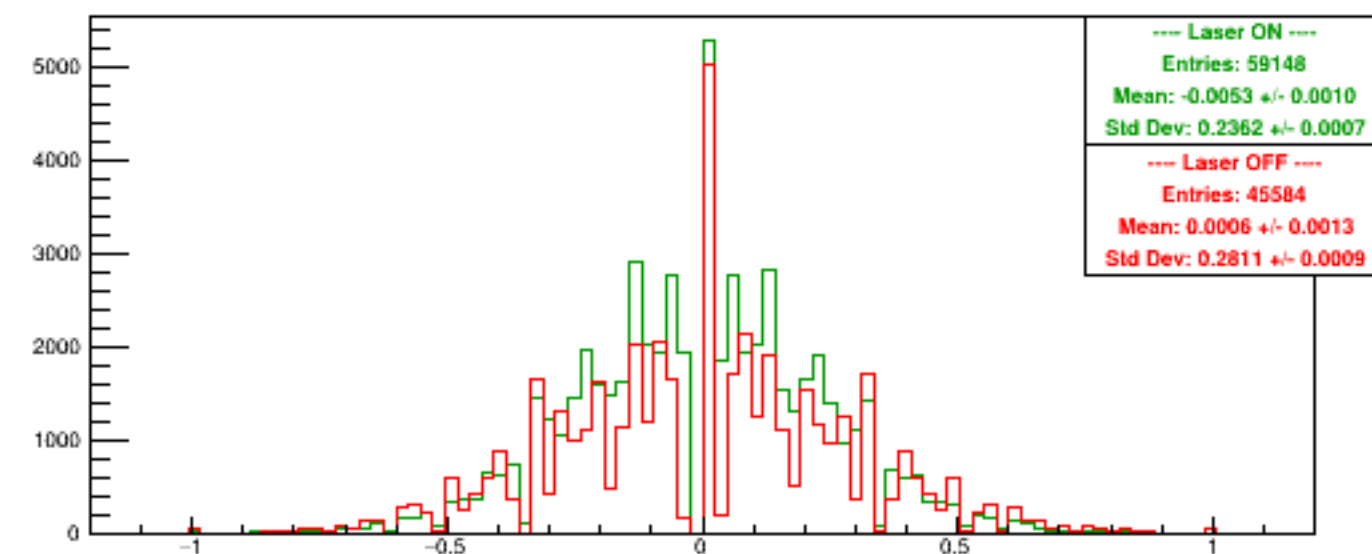
Run 5987 quartetwise, Asyms Vert Finger
