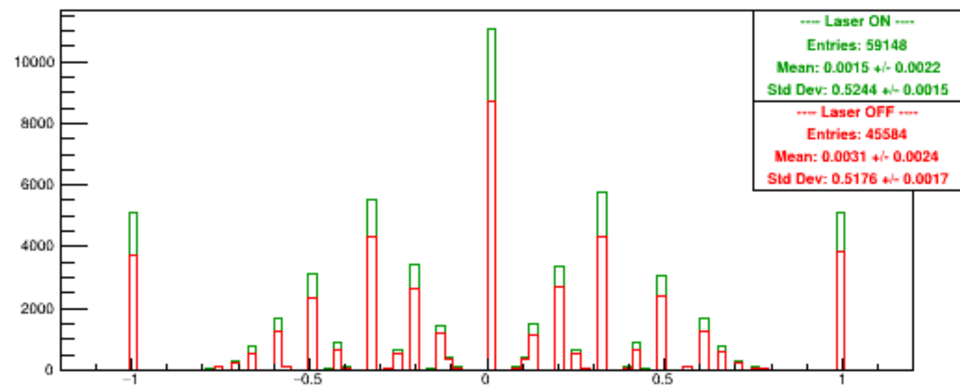
Run 5987 quartetwise, Asyms USbg1
