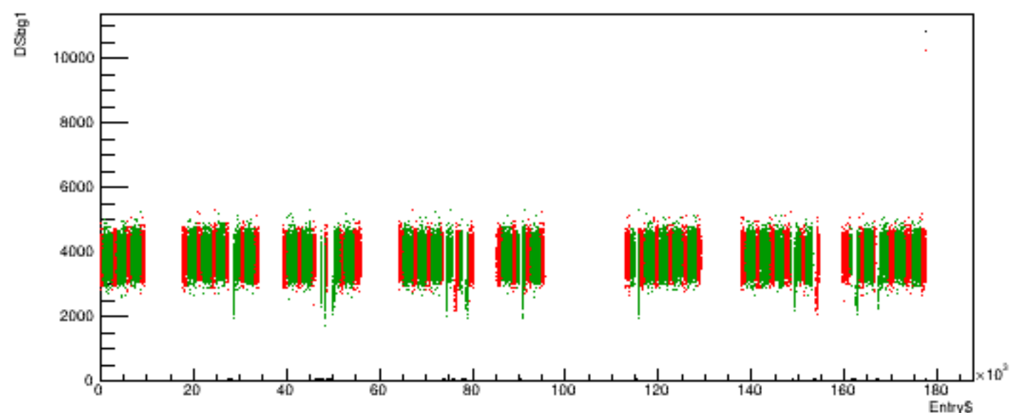
Run 5987 quartetwise, DSbg1 vs time
