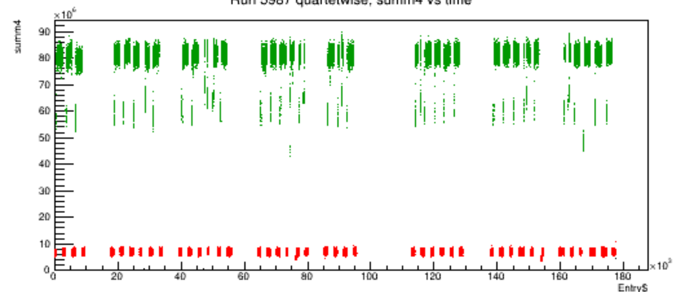
Run 5987 quartetwise, summ4 vs time
