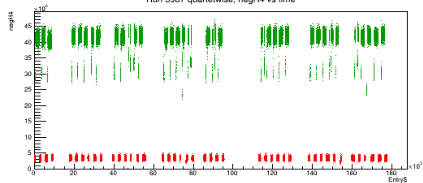
Run 5987 quartetwise, negH4 vs time
