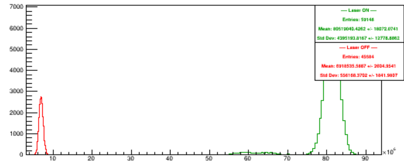
Run 5987 quartetwise, Sums4
