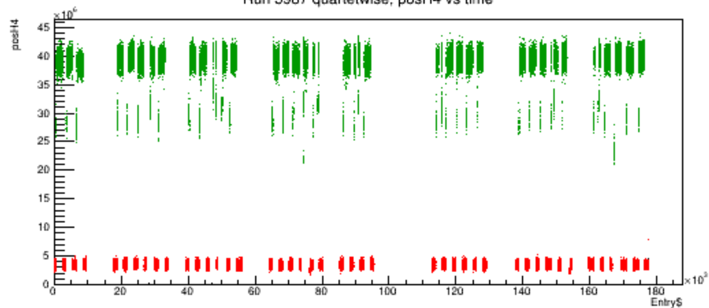
Run 5987 quartetwise, posH4 vs time
