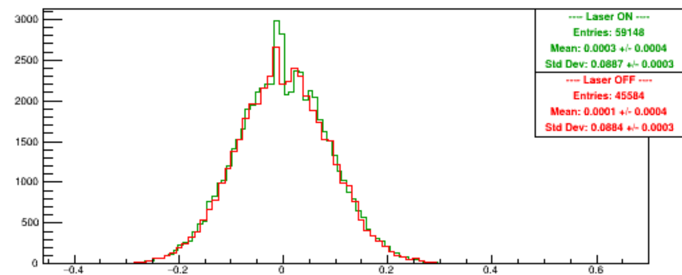
Run 5987 quartetwise, Asyms DSbg1
