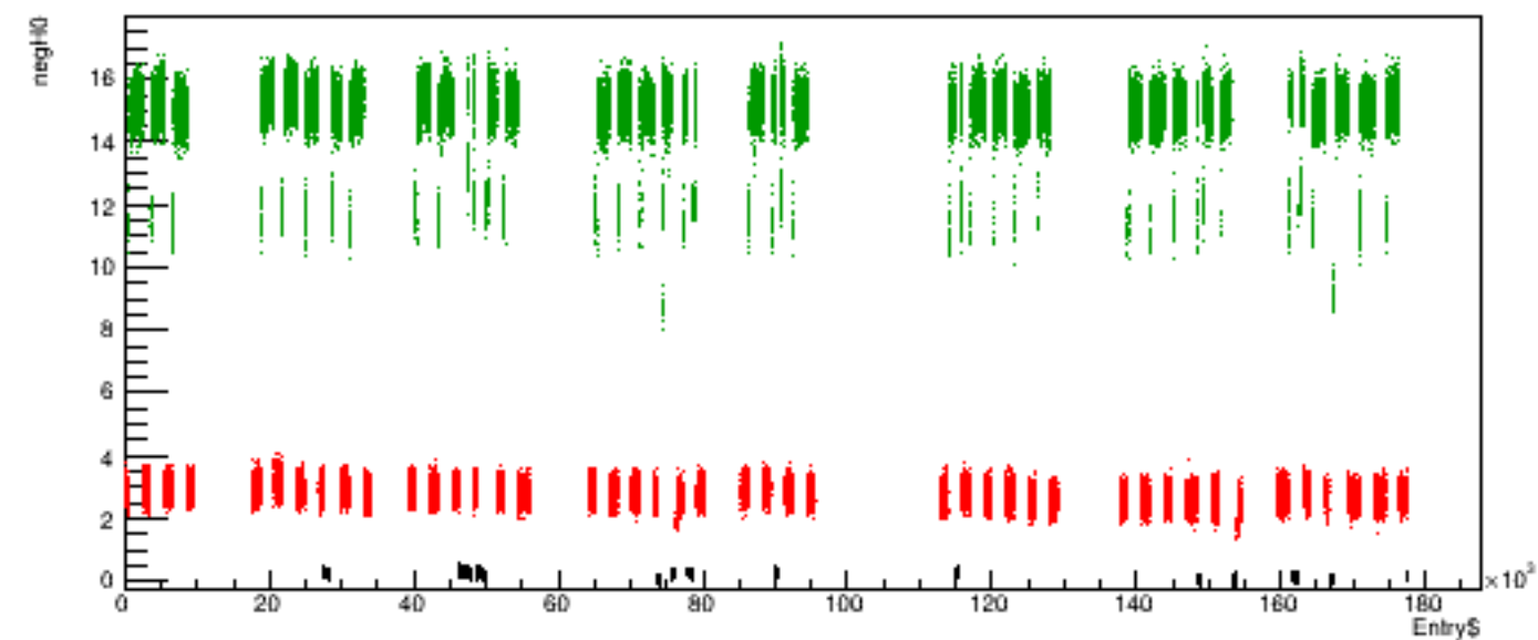
Run 5987 quartetwise, negH0 vs time
