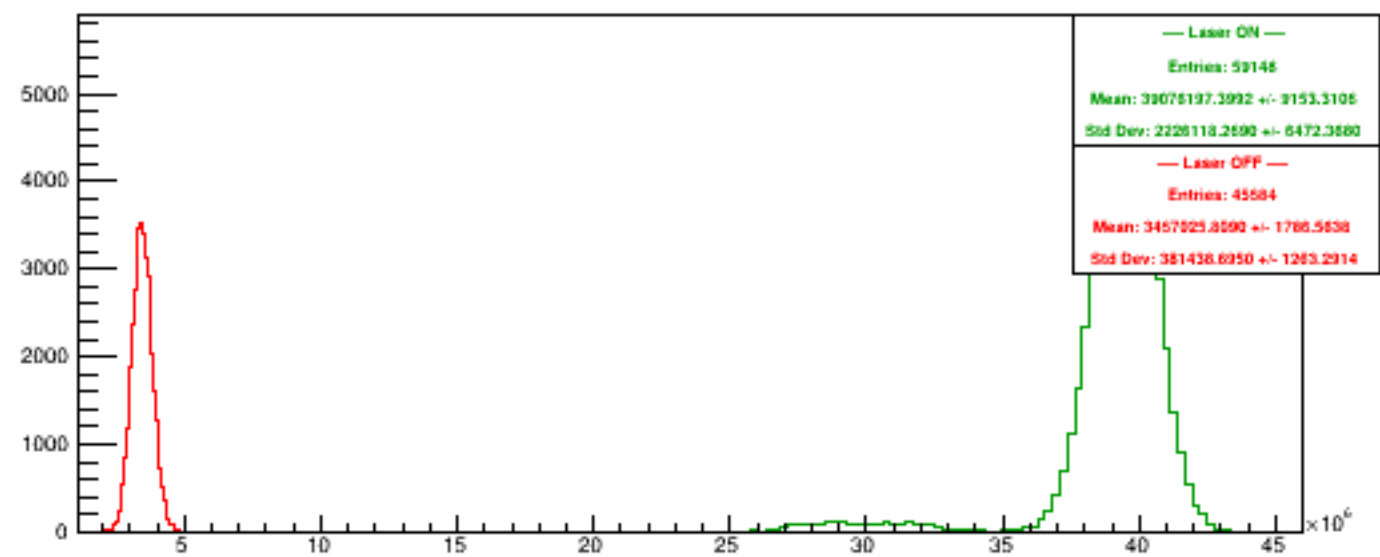
Run 5987 quartetwise, PosHelAcc4
