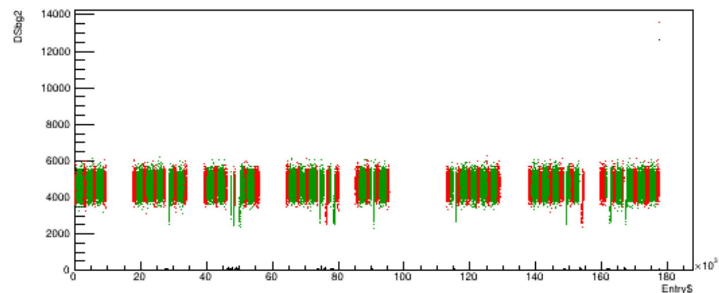
Run 5987 quartetwise, DSbg2 vs time
