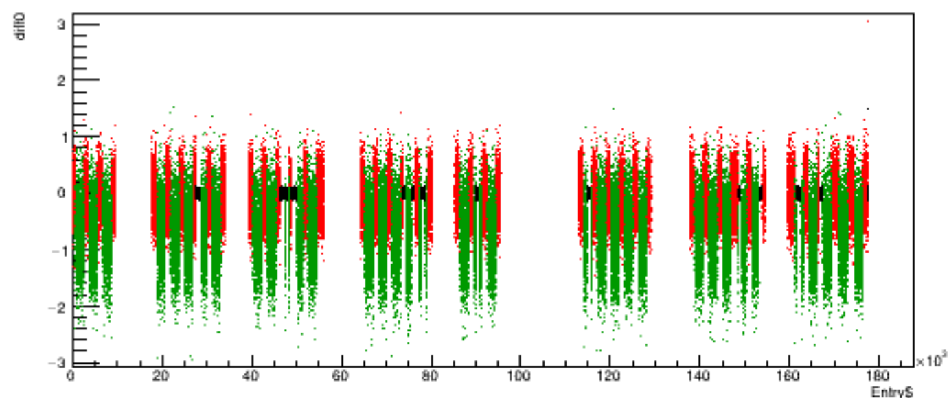
Run 5987 quartetwise, diff0 vs time
