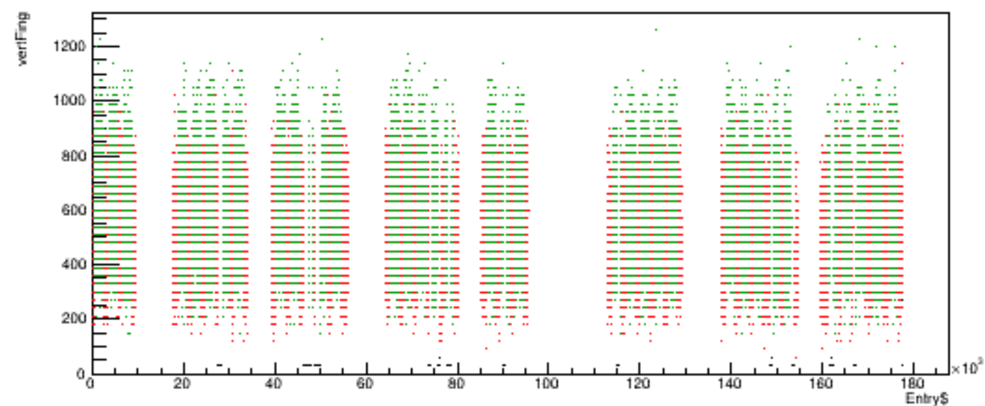
Run 5987 quartetwise, vertFing vs time
