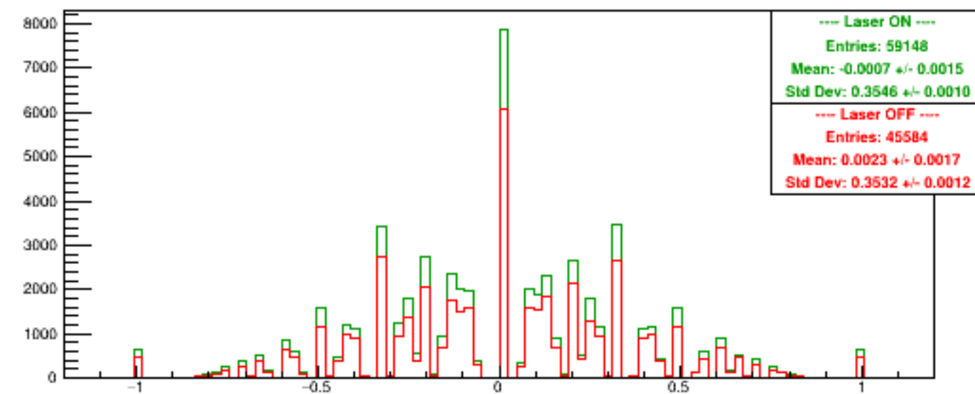
Run 5987 quartetwise, Asyms USbg2
