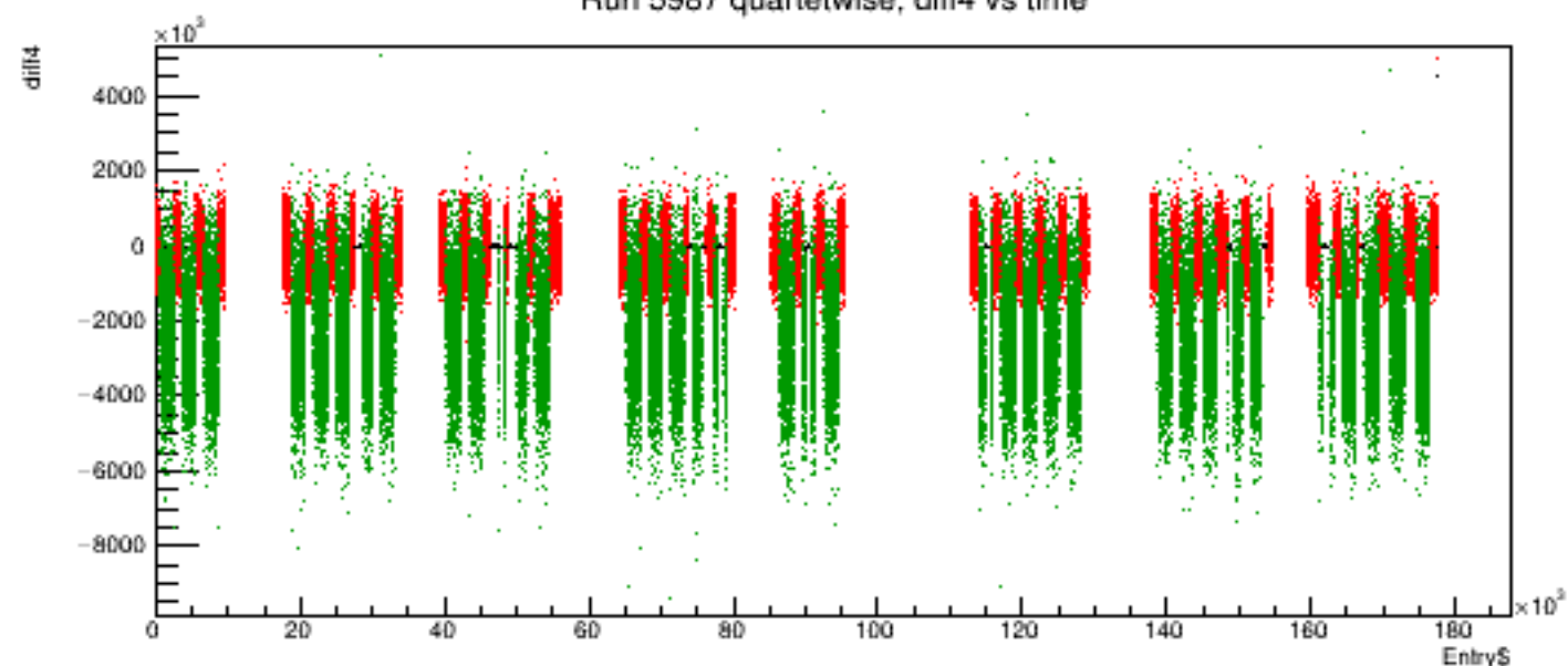
Run 5987 quartetwise, diff4 vs time
