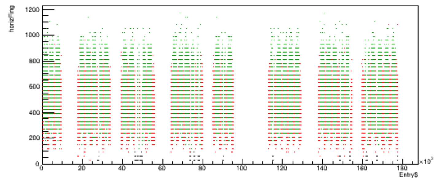
Run 5987 quartetwise, horizFing vs time
