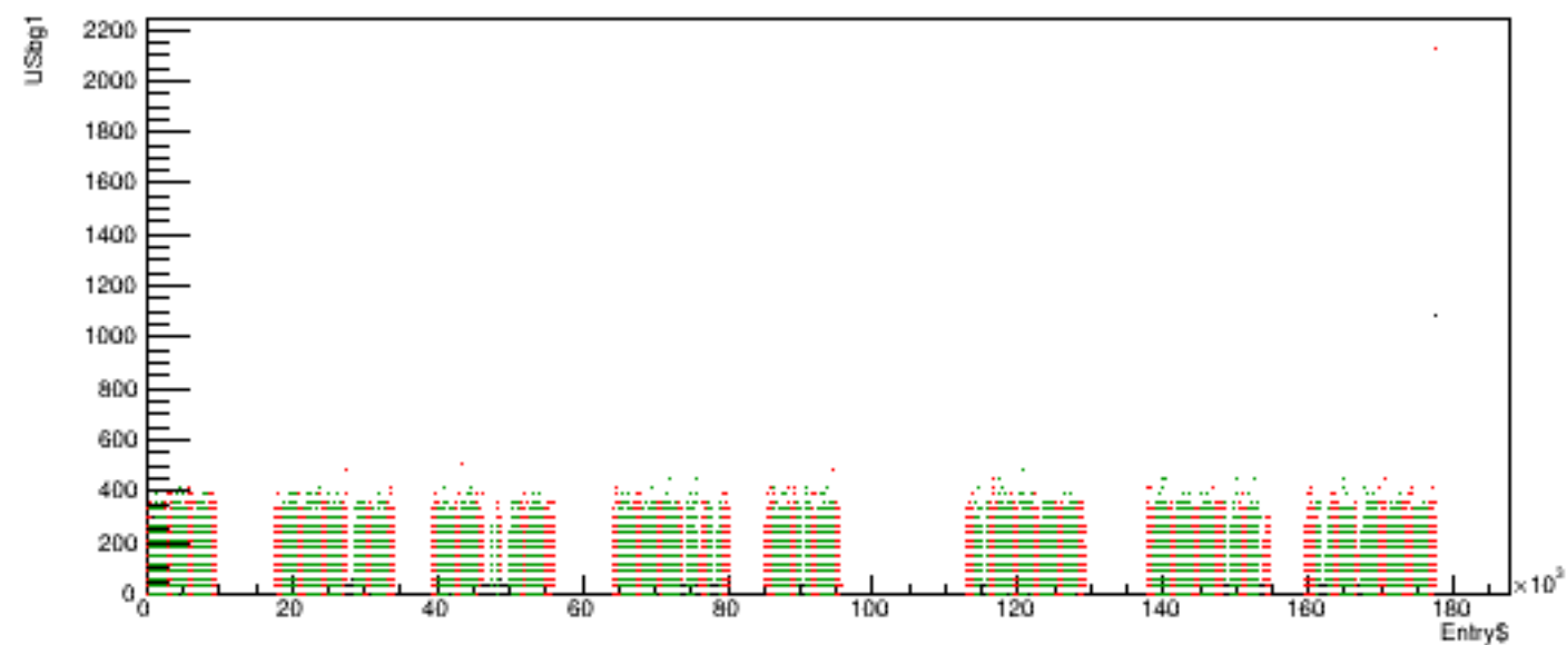
Run 5987 quartetwise, USbg1 vs time
