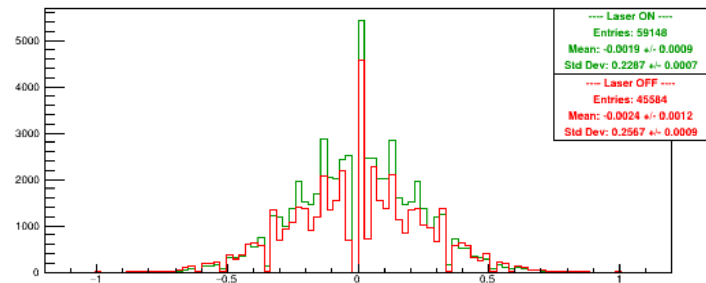
Run 5987 quartetwise, Asyms Horiz Finger
