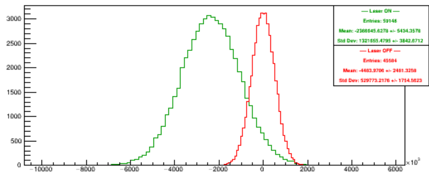
Run 5987 quartetwise, Diffs4
