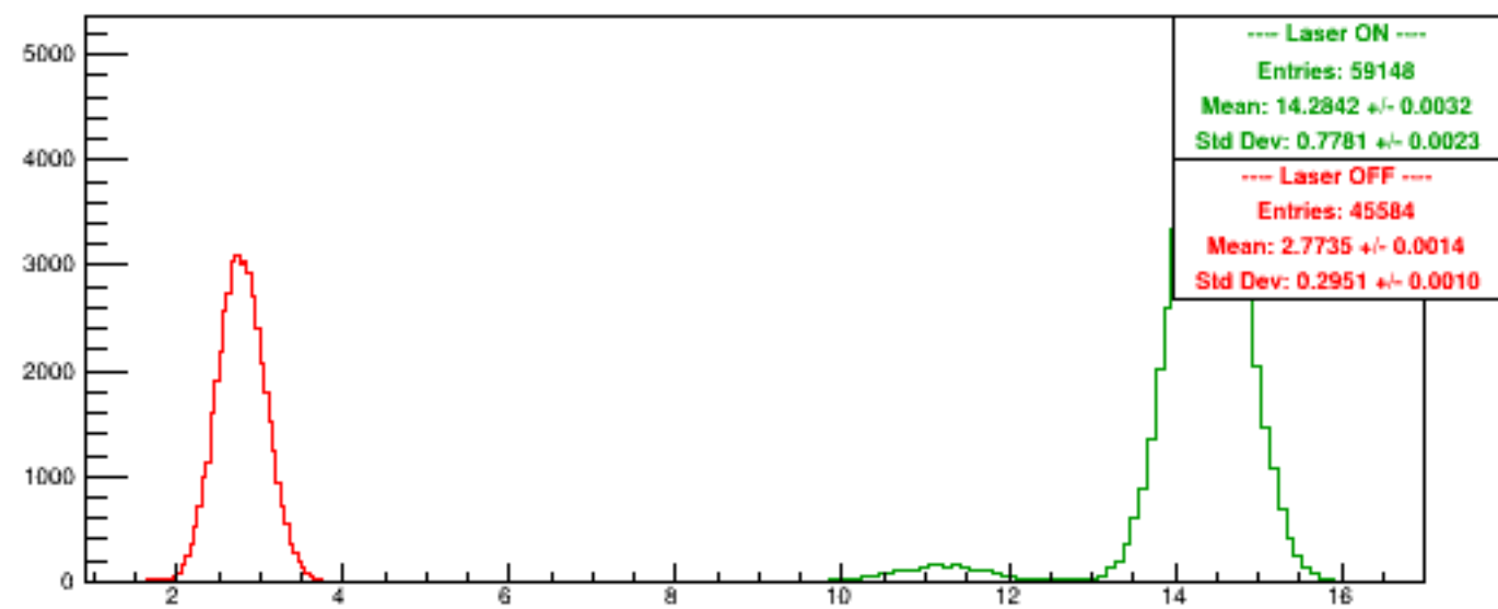
Run 5987 quartetwise, PosHelAcc0/NSamples0
