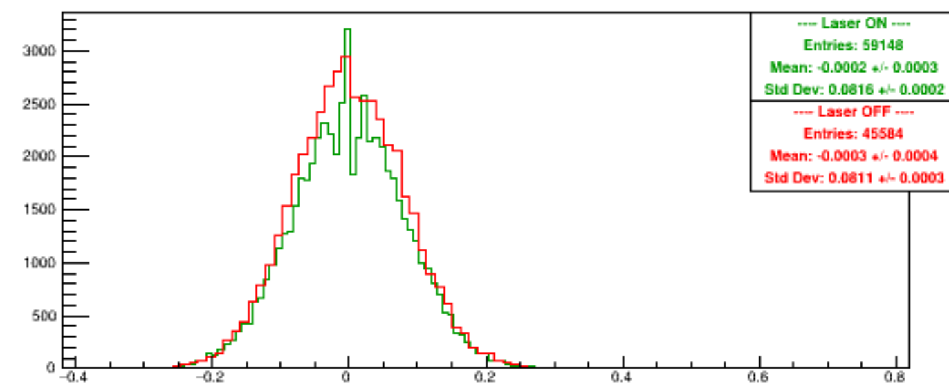
Run 5987 quartetwise, Asyms DSbg2
