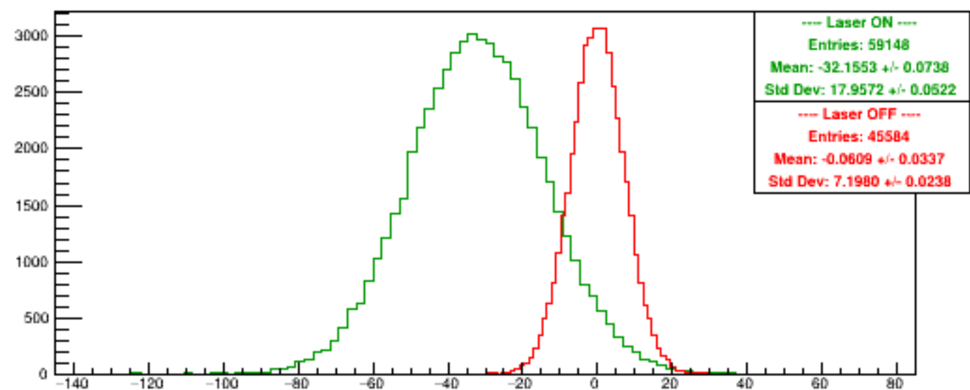
Run 5987 quartetwise, Asyms4
