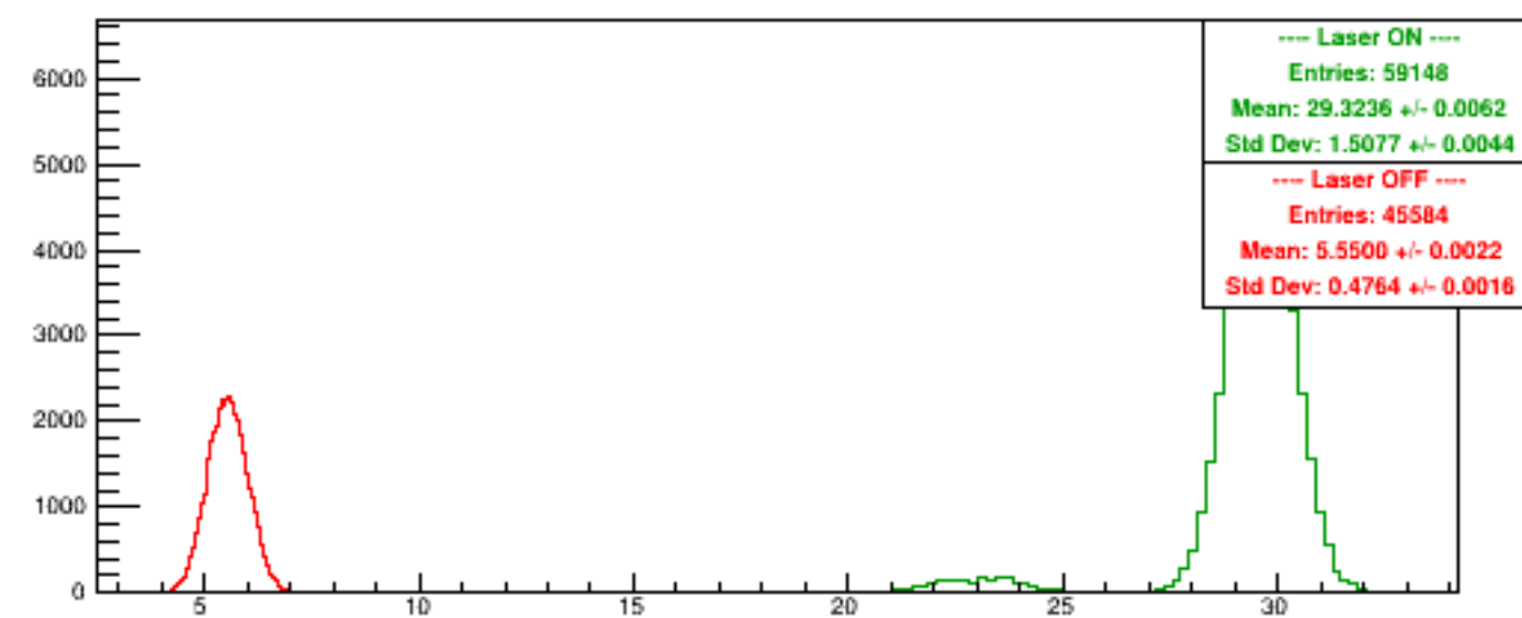
Run 5987 quartetwise, Sums0
