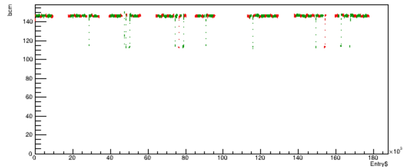
Run 5987 quartetwise, posH4 vs time
