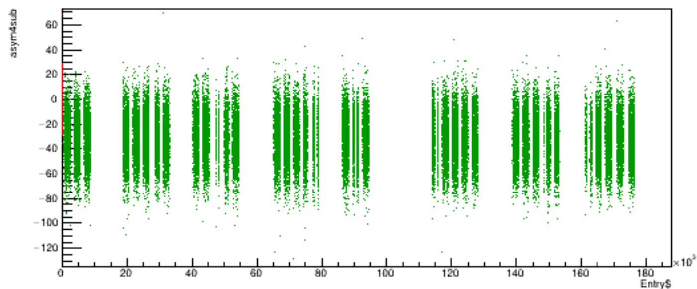
Run 5987 quartetwise, asym4sub vs time
