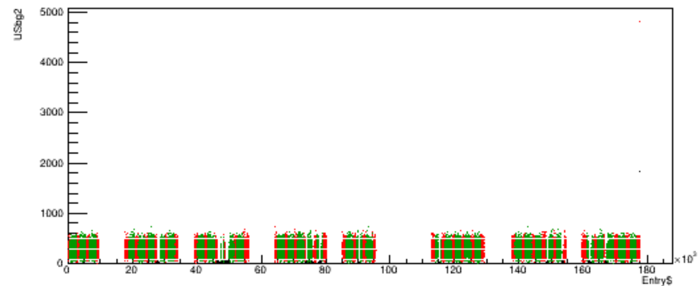
Run 5987 quartetwise, USbg2 vs time
