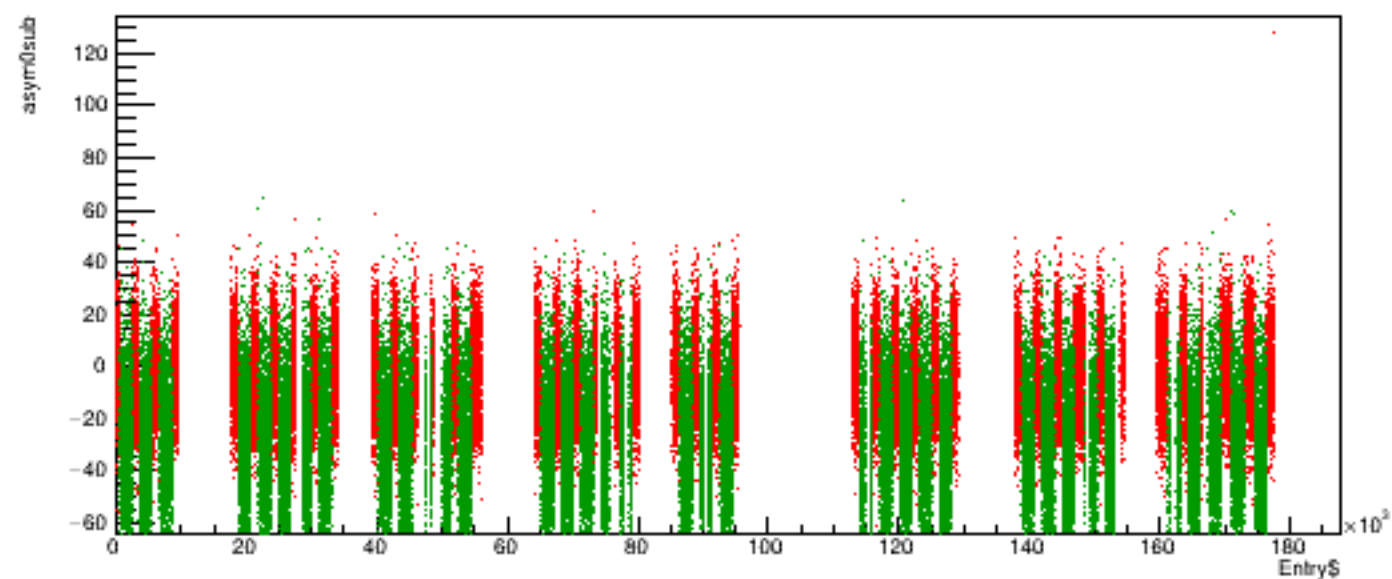
Run 5987 quartetwise, asym0sub vs time
