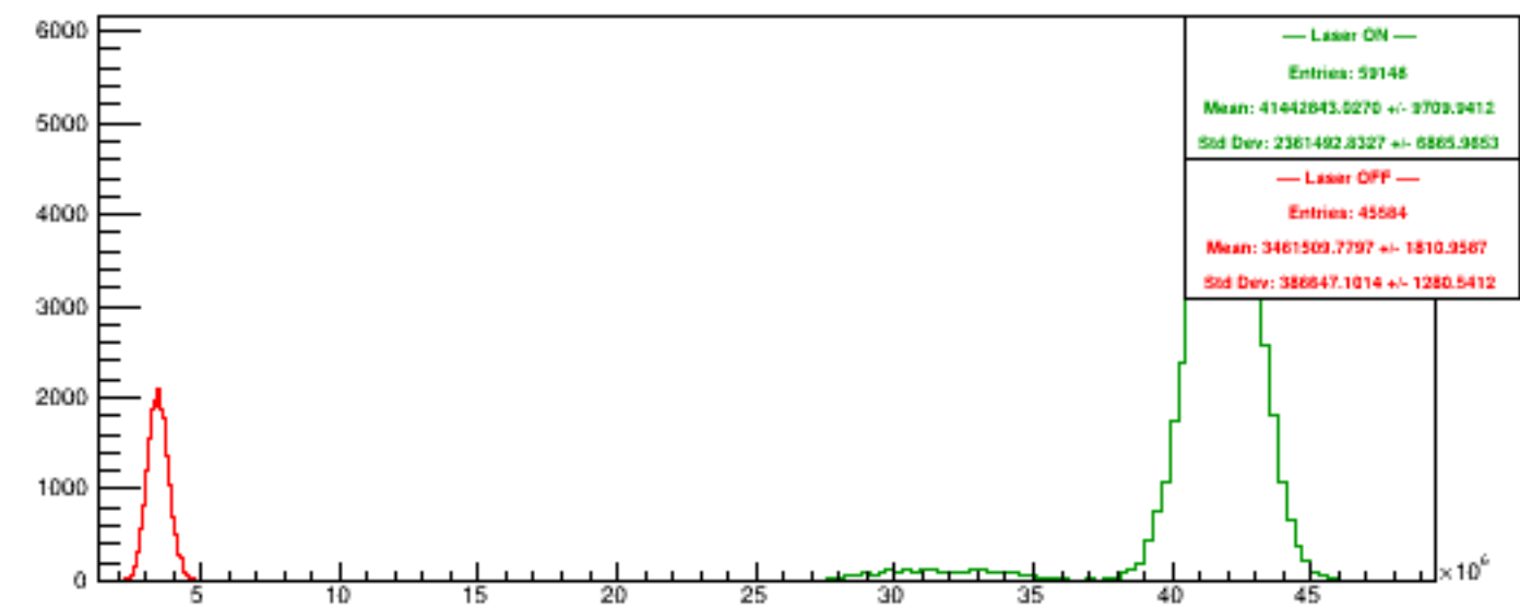
Run 5987 quartetwise, NegHelAcc4
