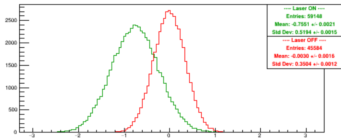
Run 5987 quartetwise, Diffs0
