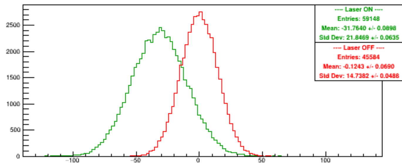
Run 5987 quartetwise, Asyms0
