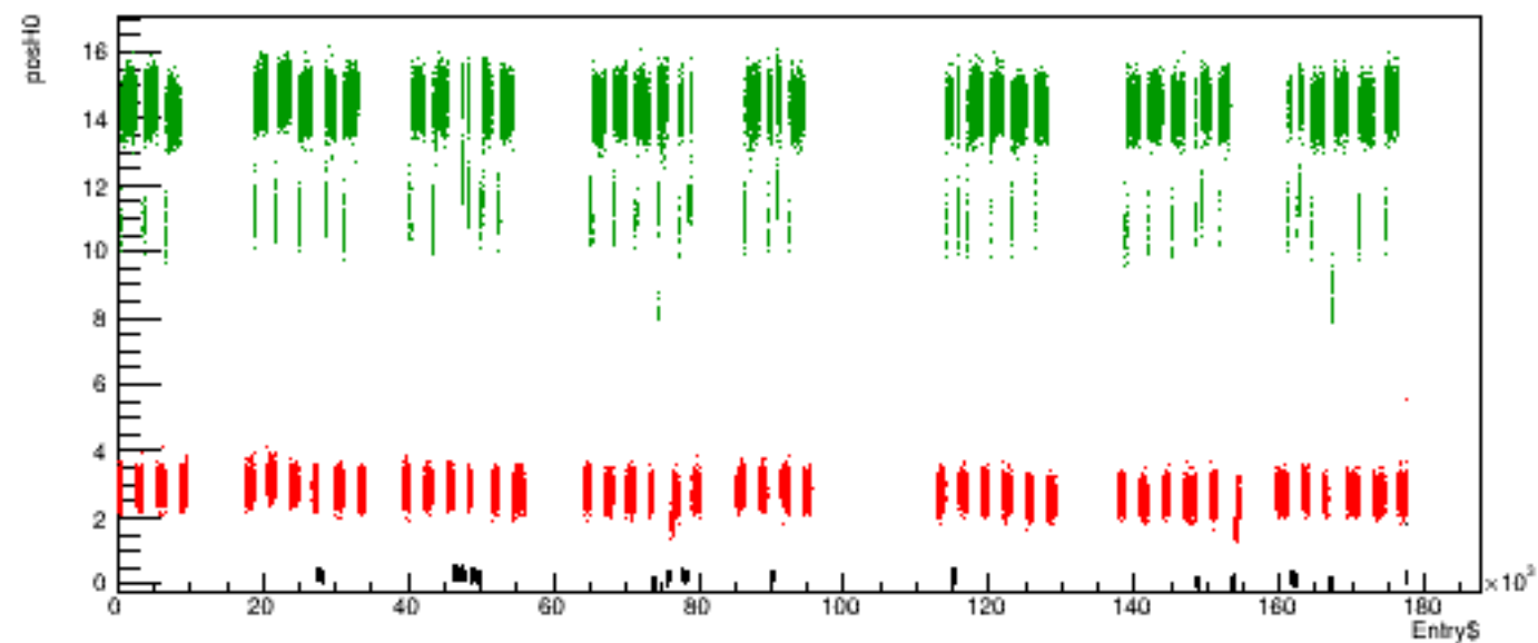
Run 5987 quartetwise, posH0 vs time
