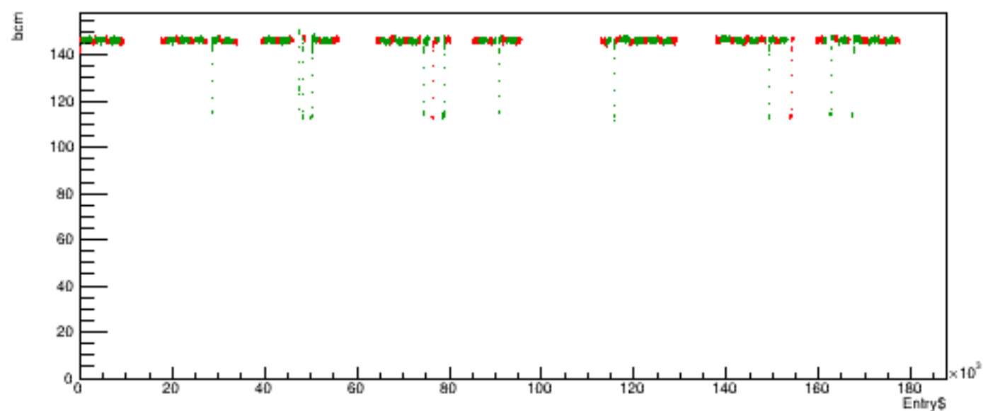
Run 5987 quartetwise, posH4 vs time
