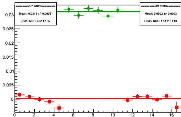
Cycle 5988.1: Multiplet Asyms
