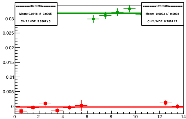
Cycle 5988.37: Multiplet Asyms
