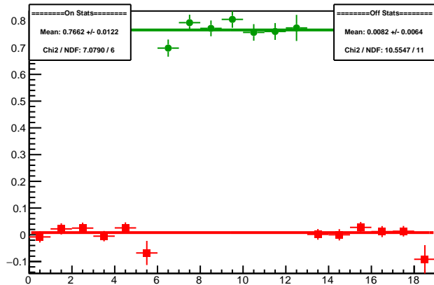
Cycle 5988.2: Multiplet Diffs
