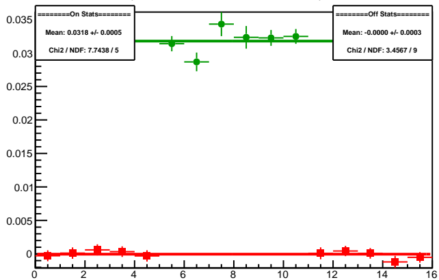
Cycle 5988.14: Multiplet Asyms
