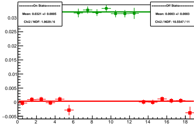
Cycle 5988.2: Multiplet Asyms
