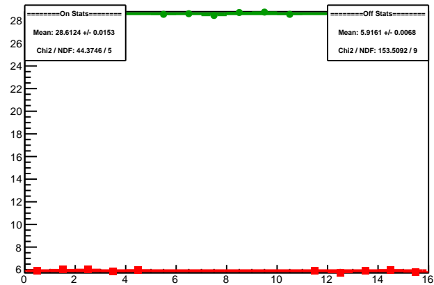
Cycle 5988.29: Multiplet Sums
