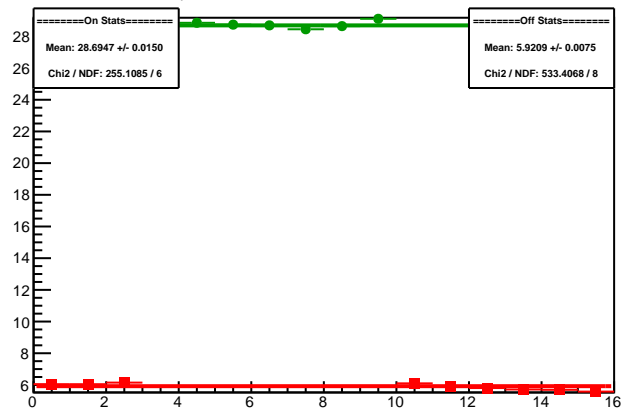
Cycle 5988.35: Multiplet Sums
