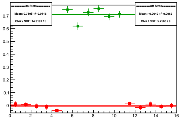
Cycle 5988.19: Multiplet Diffs
