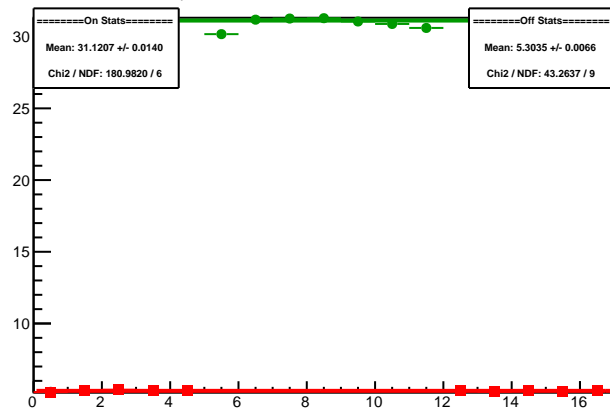
Cycle 5988.16: Multiplet Sums
