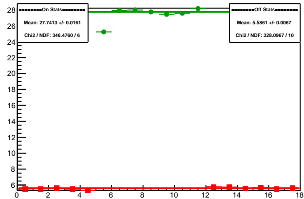
Cycle 5988.23: Multiplet Sums
