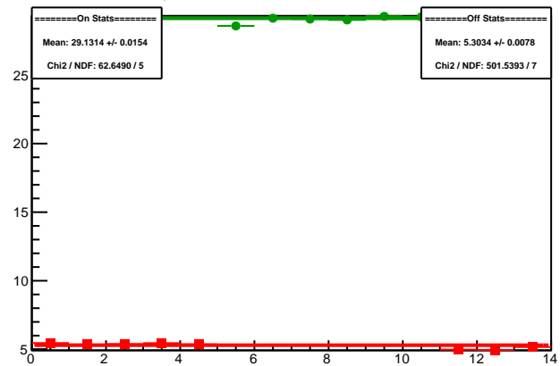
Cycle 5988.13: Multiplet Sums
