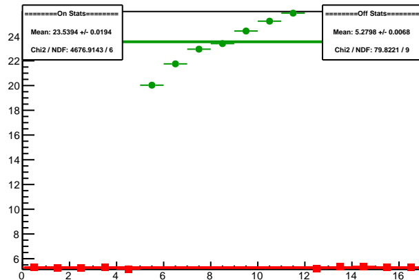
Cycle 5988.15: Multiplet Sums
