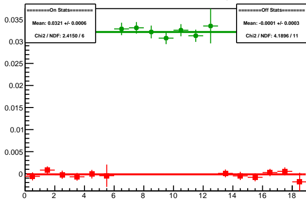
Cycle 5988.34: Multiplet Asyms
