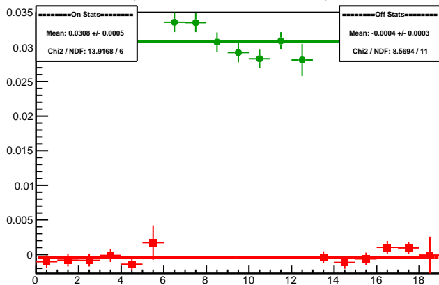
Cycle 5988.32: Multiplet Asyms
