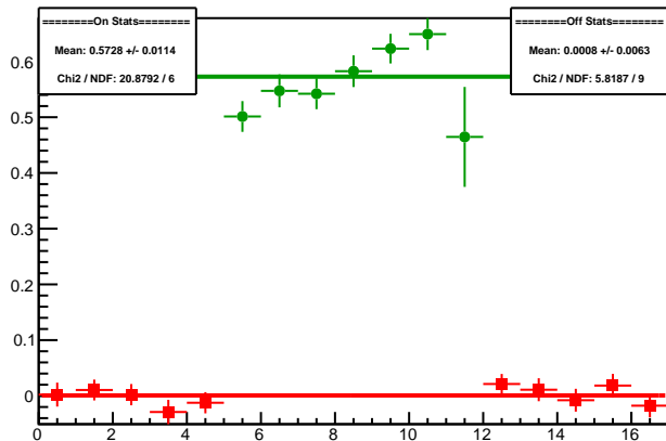
Cycle 5988.15: Multiplet Diffs
