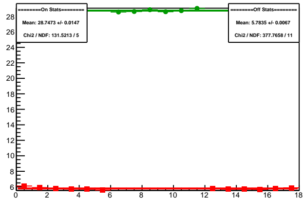
Cycle 5988.36: Multiplet Sums
