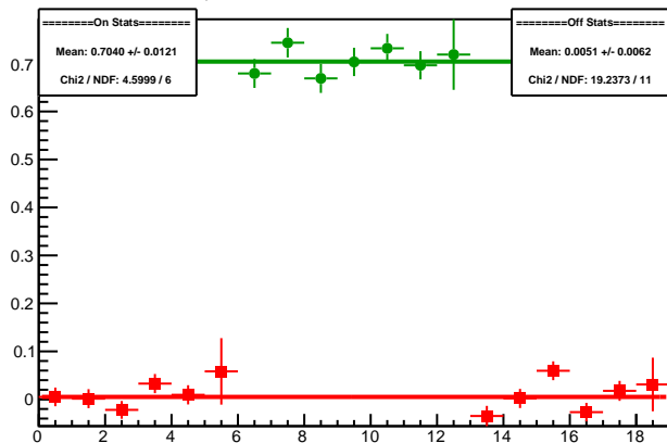
Cycle 5988.24: Multiplet Diffs
