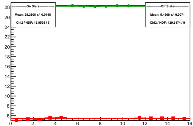
Cycle 5988.18: Multiplet Sums
