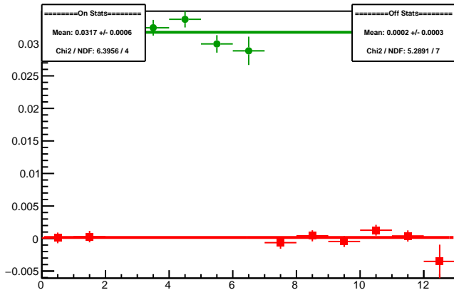
Cycle 5988.8: Multiplet Asyms
