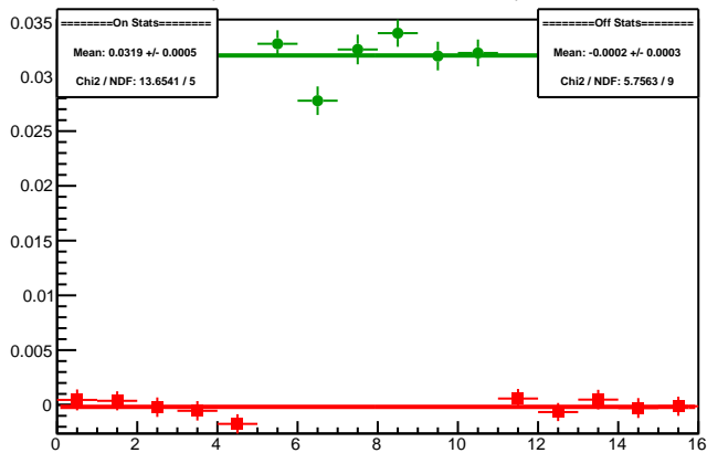
Cycle 5988.19: Multiplet Asyms
