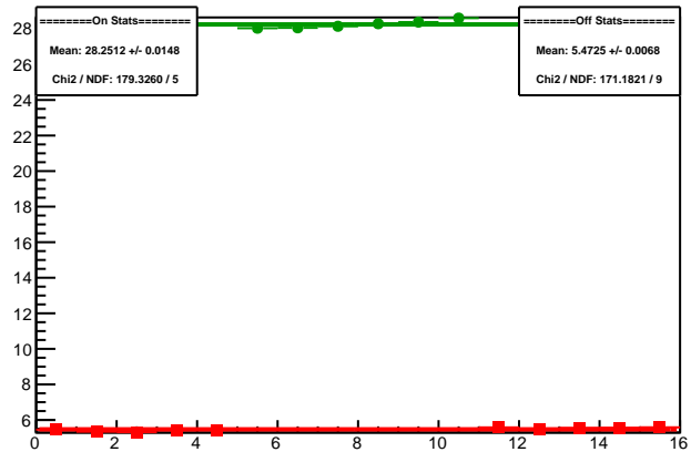
Cycle 5988.20: Multiplet Sums
