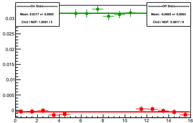
Cycle 5988.18: Multiplet Asyms
