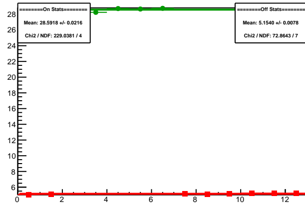
Cycle 5988.8: Multiplet Sums
