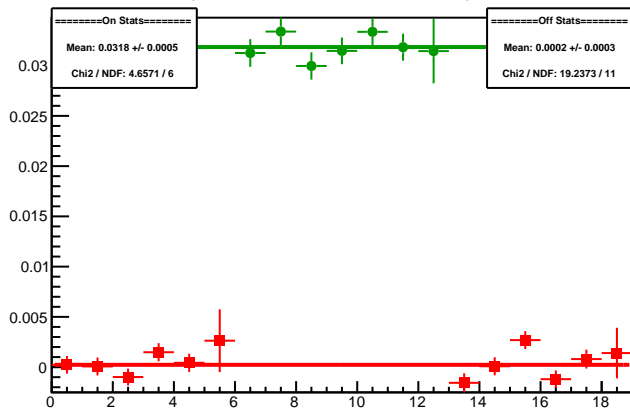
Cycle 5988.24: Multiplet Asyms
