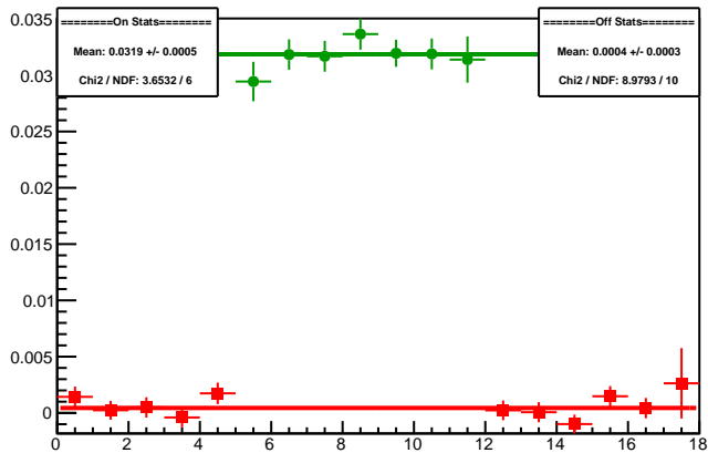
Cycle 5988.23: Multiplet Asyms
