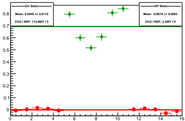
Cycle 5988.14: Multiplet Diffs
