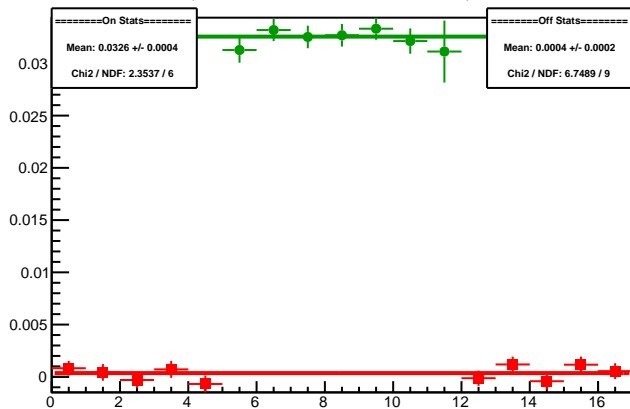
Cycle 5988.16: Multiplet Asyms
