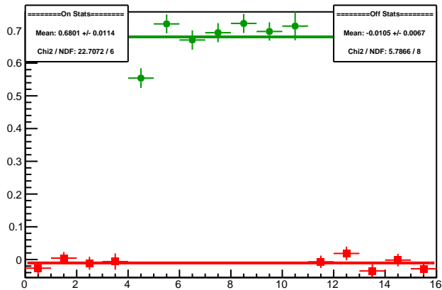
Cycle 5988.27: Multiplet Diffs
