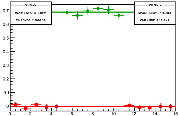
Cycle 5988.20: Multiplet Diffs
