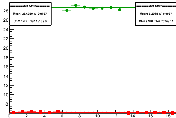
Cycle 5988.31: Multiplet Sums
