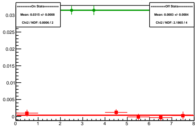
Cycle 5988.6: Multiplet Asyms
