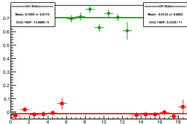
Cycle 5988.31: Multiplet Diffs
