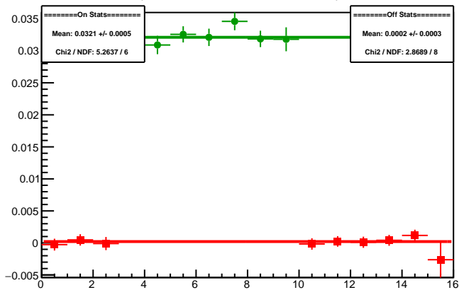
Cycle 5988.35: Multiplet Asyms
