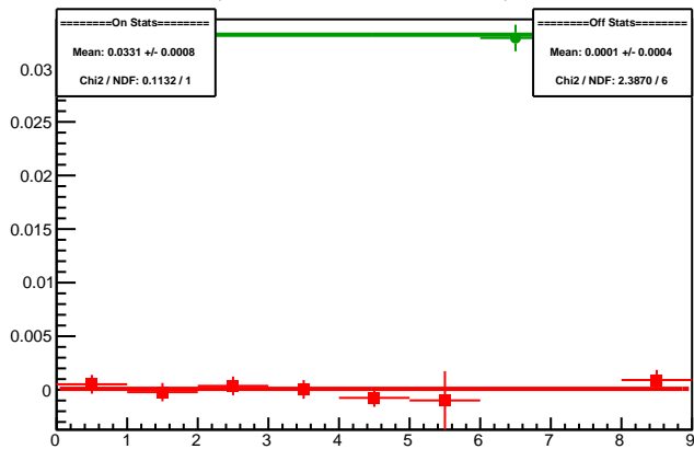
Cycle 5988.5: Multiplet Asyms
