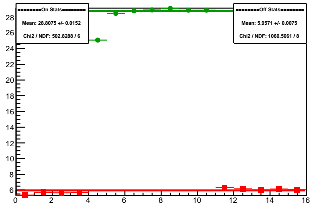
Cycle 5988.27: Multiplet Sums
