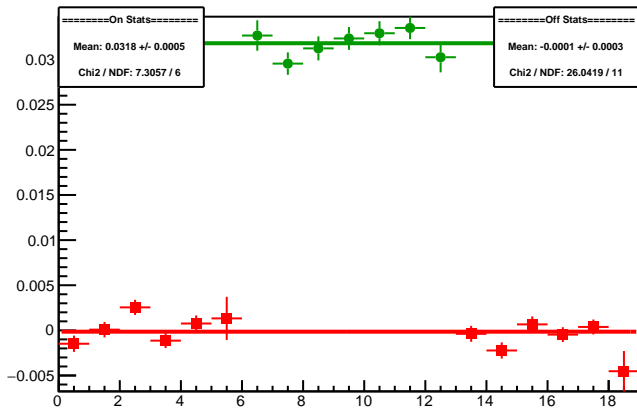
Cycle 5988.25: Multiplet Asyms
