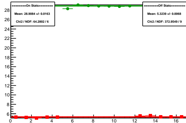
Cycle 5988.12: Multiplet Sums
