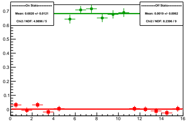
Cycle 5988.30: Multiplet Diffs
