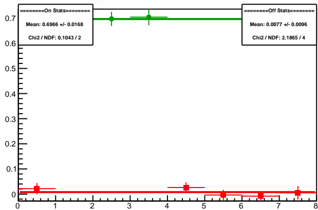
Cycle 5988.6: Multiplet Diffs
