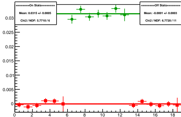
Cycle 5988.33: Multiplet Asyms
