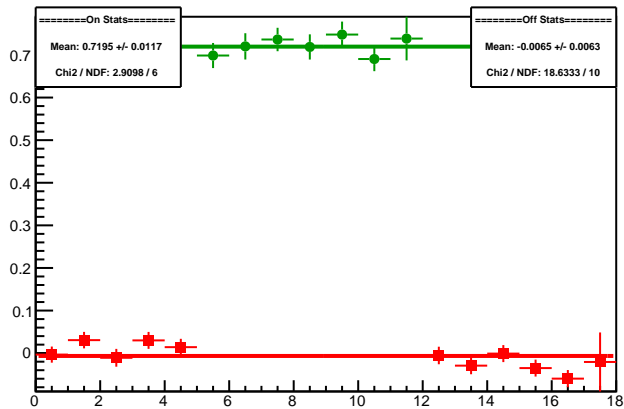
Cycle 5988.17: Multiplet Diffs
