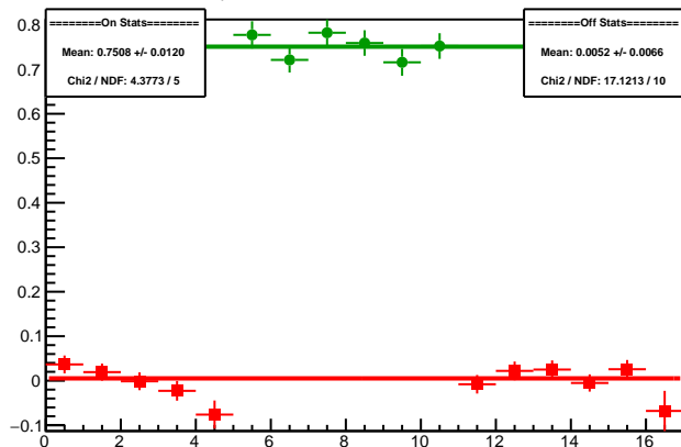
Cycle 5988.1: Multiplet Diffs
