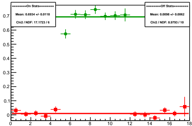
Cycle 5988.23: Multiplet Diffs
