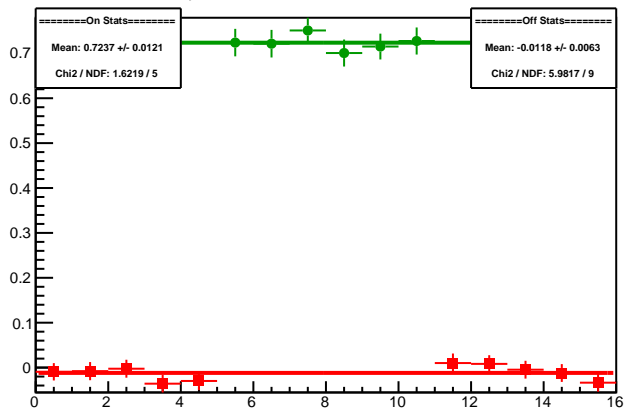
Cycle 5988.18: Multiplet Diffs
