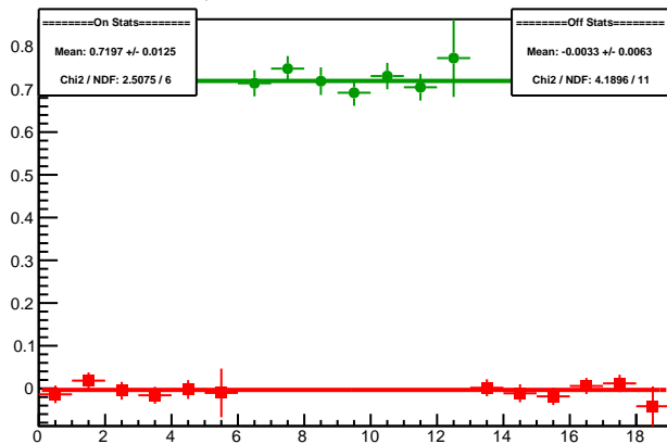
Cycle 5988.34: Multiplet Diffs
