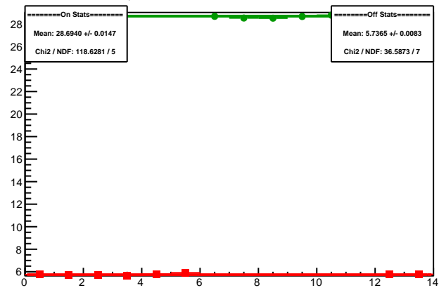
Cycle 5988.37: Multiplet Sums
