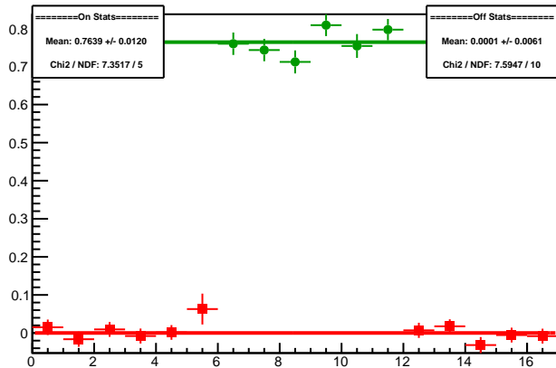
Cycle 5988.10: Multiplet Diffs
