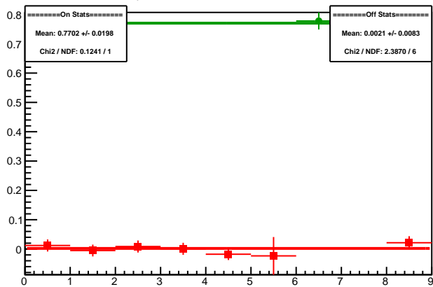
Cycle 5988.5: Multiplet Diffs
