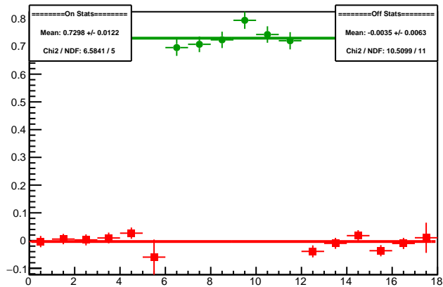
Cycle 5988.36: Multiplet Diffs
