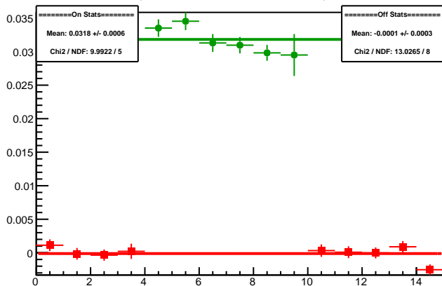
Cycle 5988.7: Multiplet Asyms
