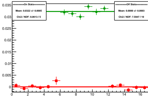
Cycle 5988.10: Multiplet Asyms
