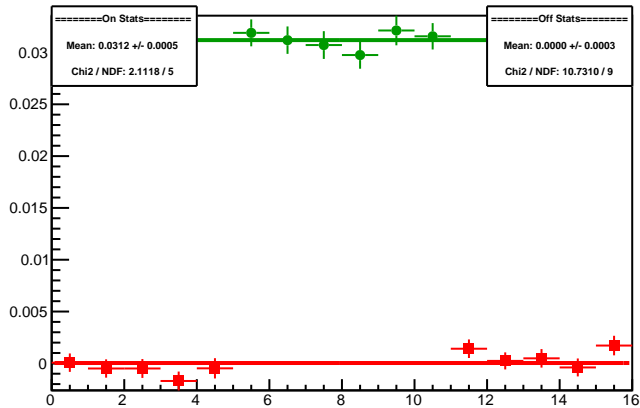
Cycle 5988.22: Multiplet Asyms
