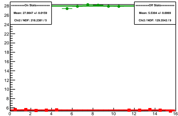
Cycle 5988.22: Multiplet Sums
