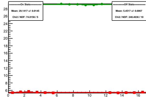
Cycle 5988.10: Multiplet Sums
