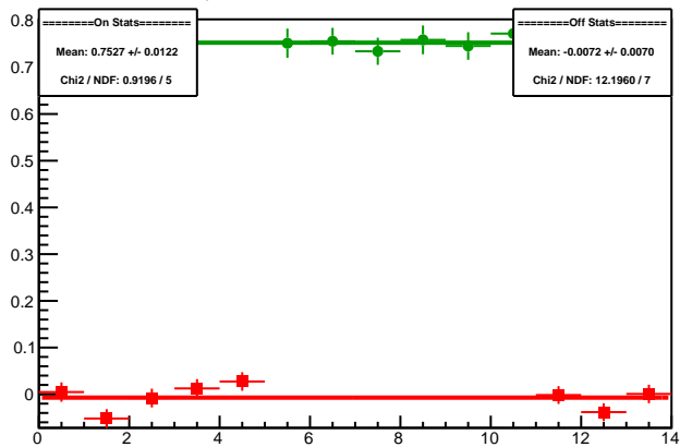
Cycle 5988.13: Multiplet Diffs
