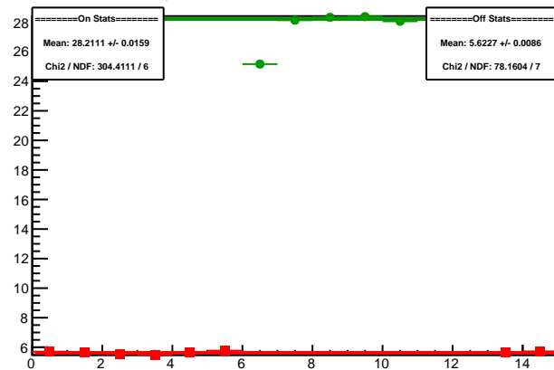
Cycle 5988.26: Multiplet Sums
