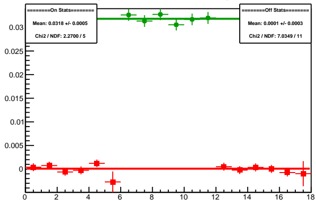
Cycle 5988.4: Multiplet Asyms
