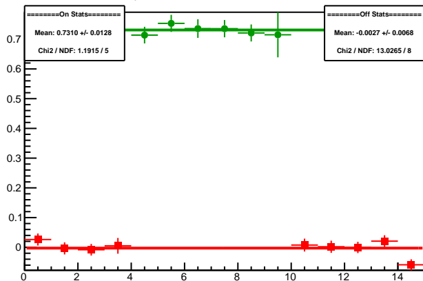
Cycle 5988.7: Multiplet Diffs
