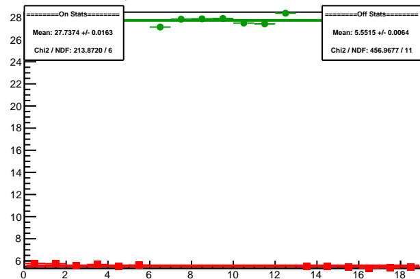
Cycle 5988.24: Multiplet Sums
