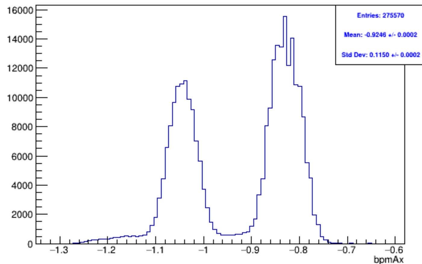
Run 5988, mpwise, bpmAx: Beam ON, Laser OFF
