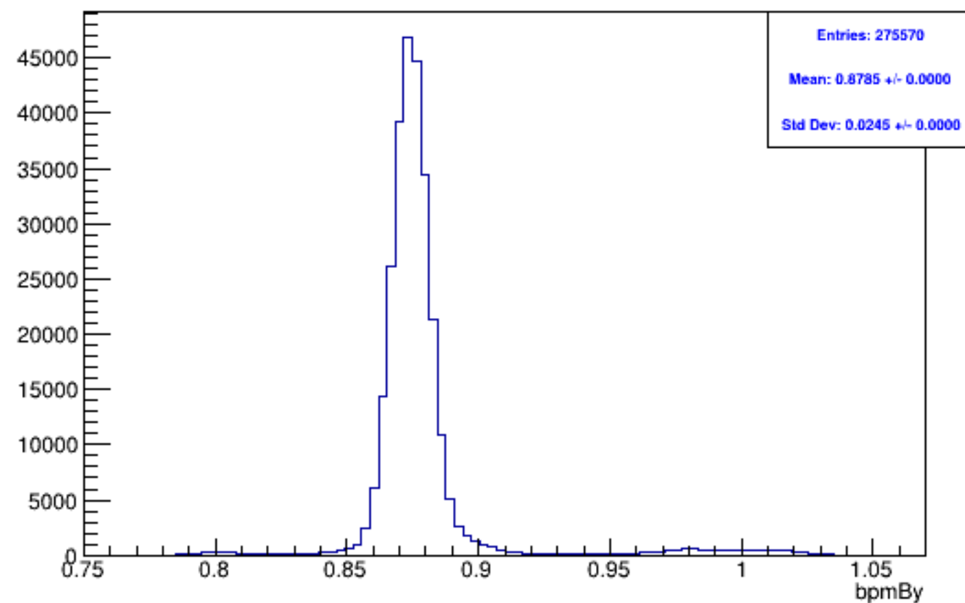
Run 5988, mpswise, bpmBy: Beam ON, Laser OFF
