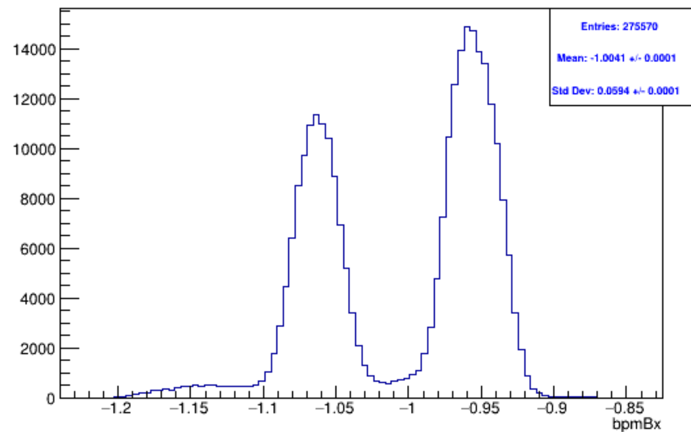
Run 5988, mpswise, bpmBx: Beam ON, Laser OFF
