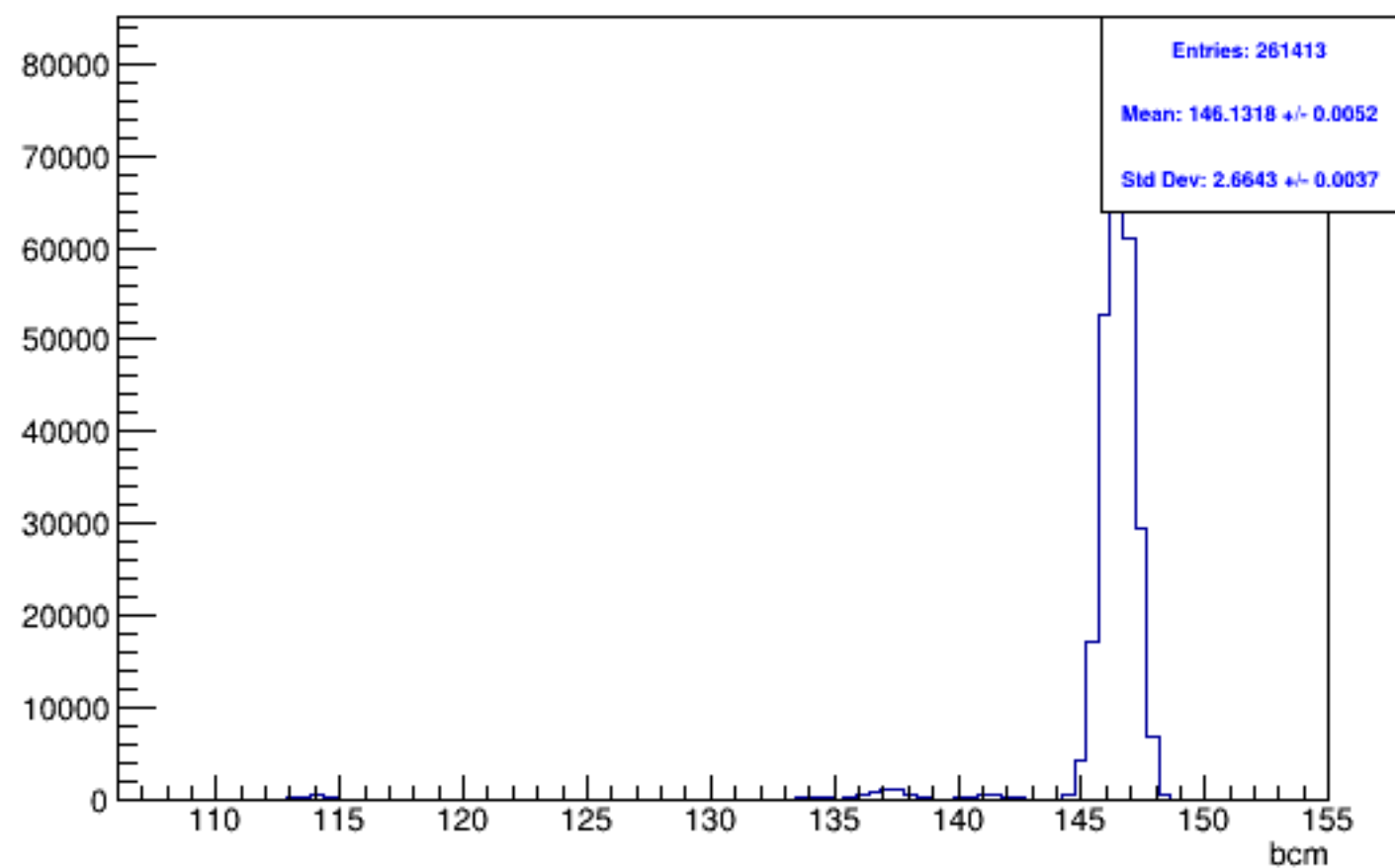
Run 5988, mpwise, BCM: Beam ON, Laser ON
