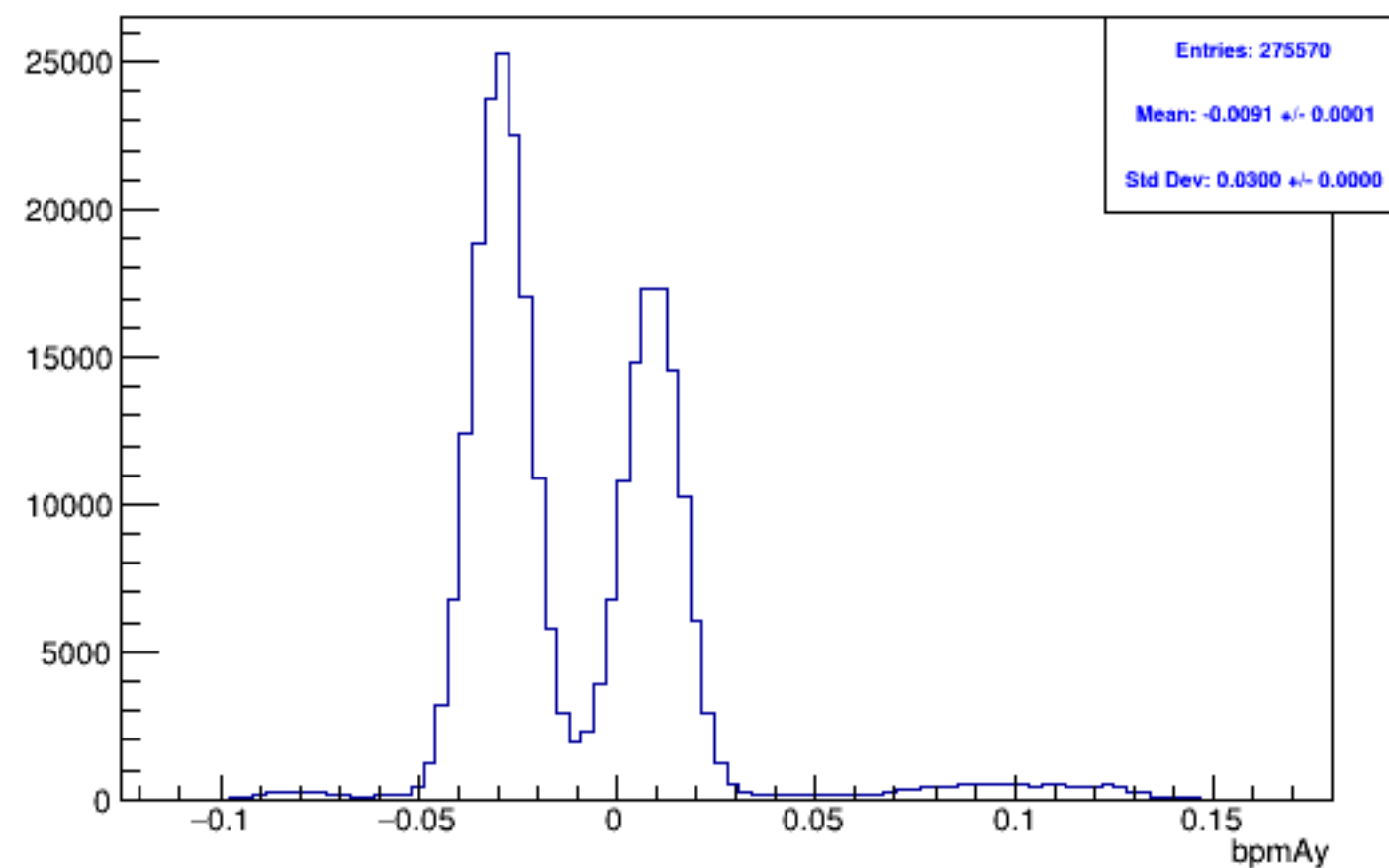
Run 5988, mpwise, bpmAy: Beam ON, Laser OFF
