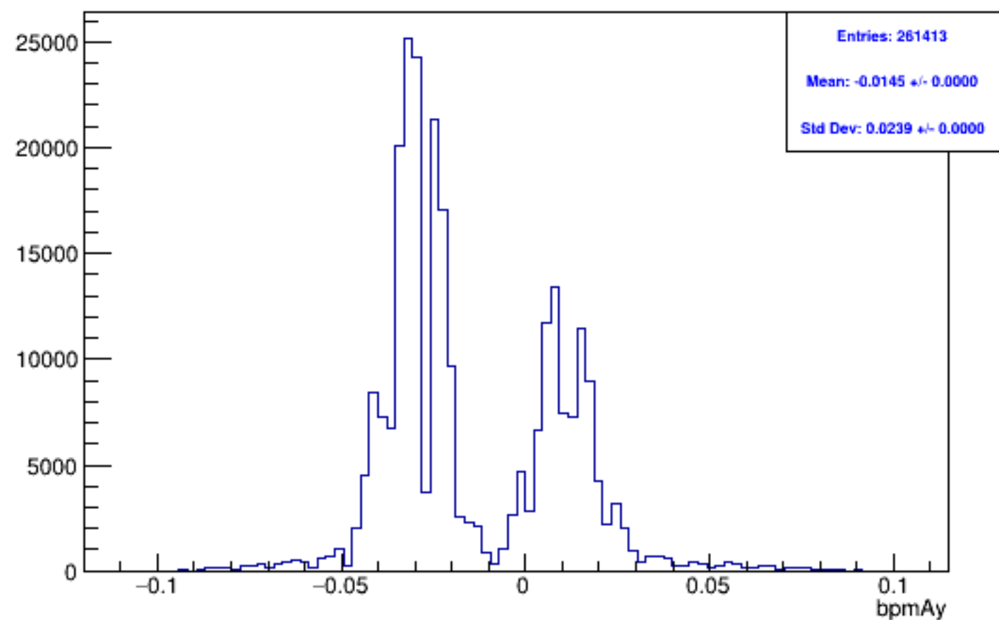
Run 5988, mpwise, bpmAy: Beam ON, Laser ON
