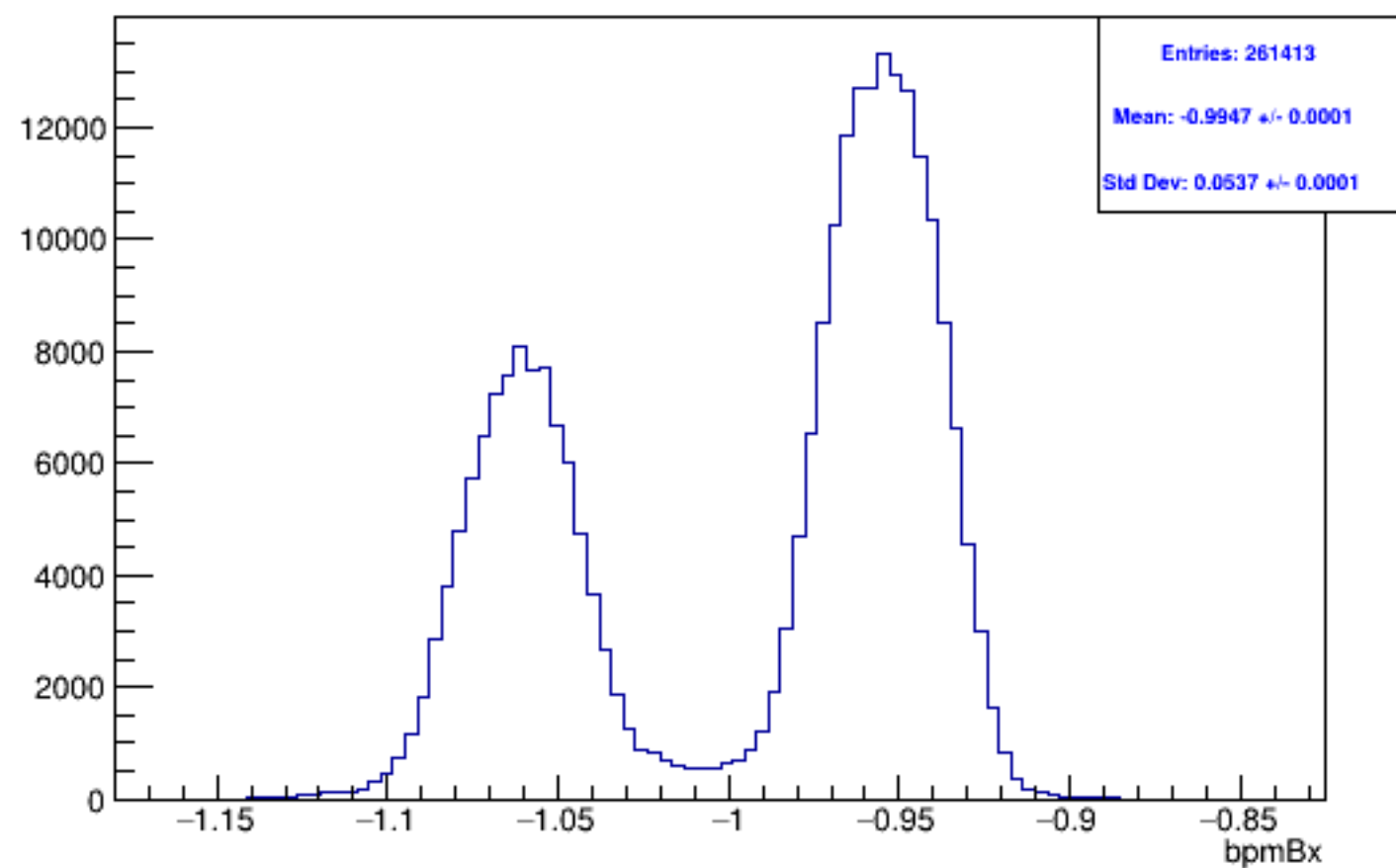
Run 5988, mpswise, bpmBx: Beam ON, Laser ON
