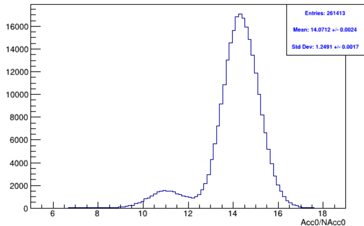
Run 5988, mpwise, acc0: Beam ON, Laser ON
