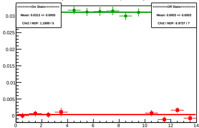
Cycle 5989.9: Multiplet Asyms
