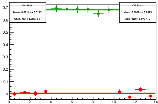
Cycle 5989.9: Multiplet Diffs
