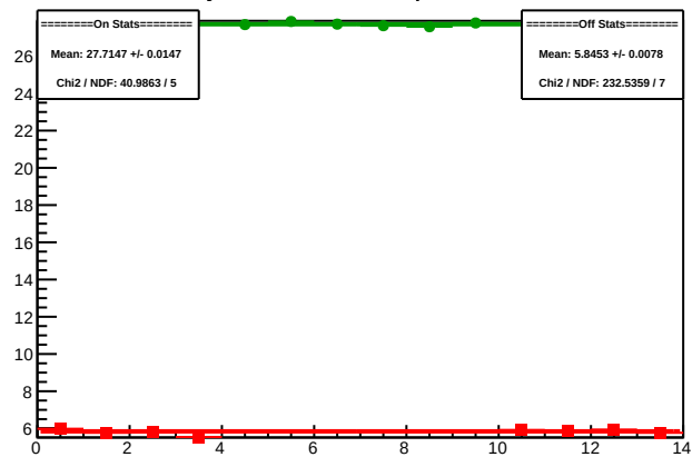
Cycle 5989.9: Multiplet Sums
