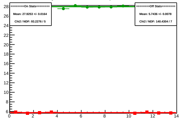
Cycle 5989.11: Multiplet Sums
