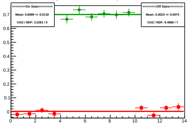
Cycle 5989.11: Multiplet Diffs
