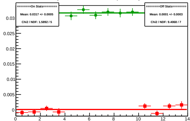
Cycle 5989.11: Multiplet Asyms
