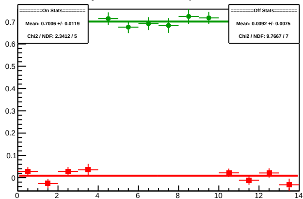
Cycle 5989.12: Multiplet Diffs
