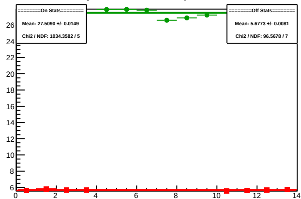
Cycle 5989.12: Multiplet Sums
