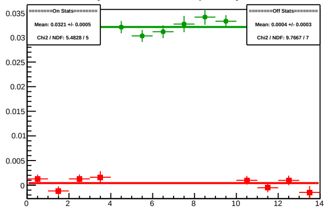
Cycle 5989.12: Multiplet Asyms
