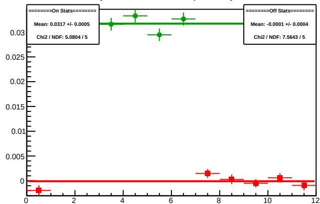
Cycle 5992.2: Multiplet Asyms
