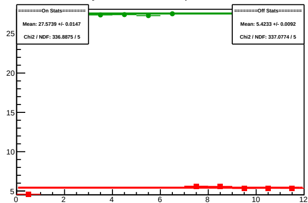
Cycle 5992.2: Multiplet Sums
