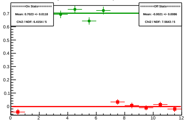
Cycle 5992.2: Multiplet Diffs
