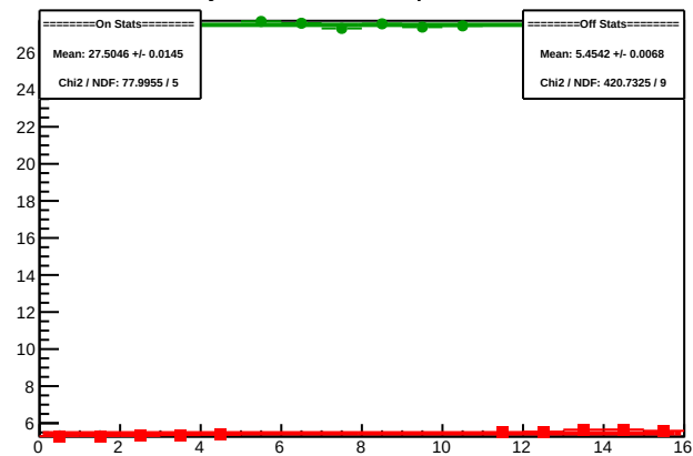
Cycle 5992.4: Multiplet Sums
