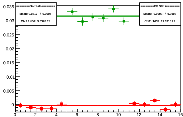
Cycle 5992.4: Multiplet Asyms
