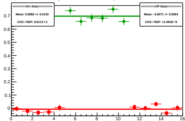
Cycle 5992.4: Multiplet Diffs
