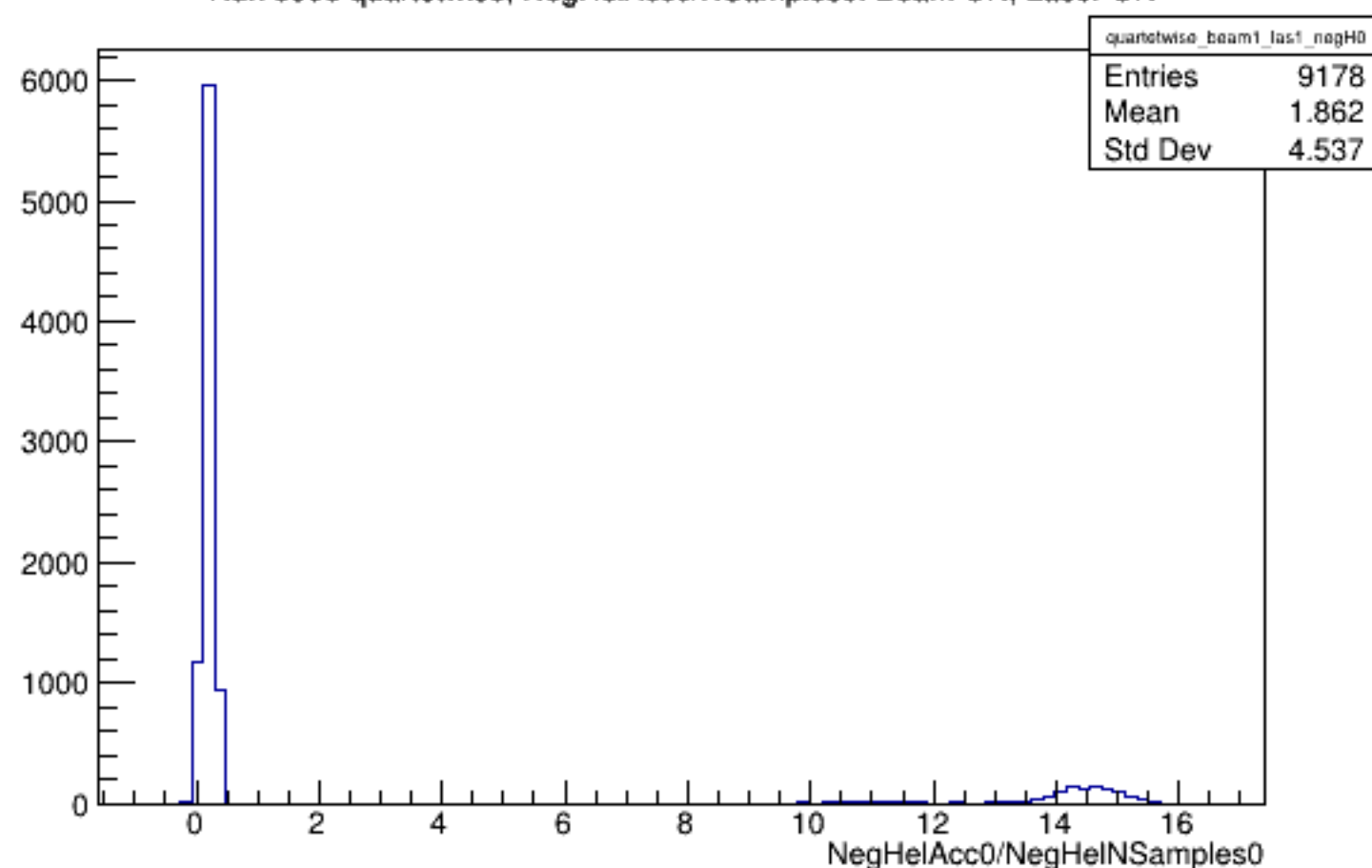
Run 5996 quartetwise, NegHelAcc0/NSamples0: Beam ON, Laser ON
