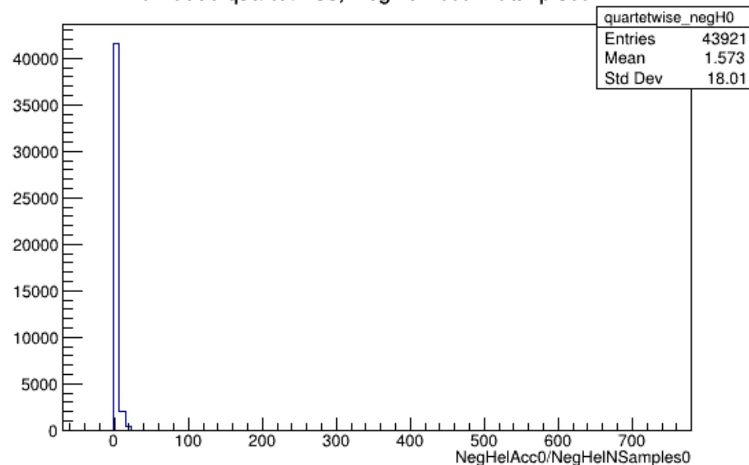
Run 5996 quartetwise, NegHelAcc0/NSamples0: All
