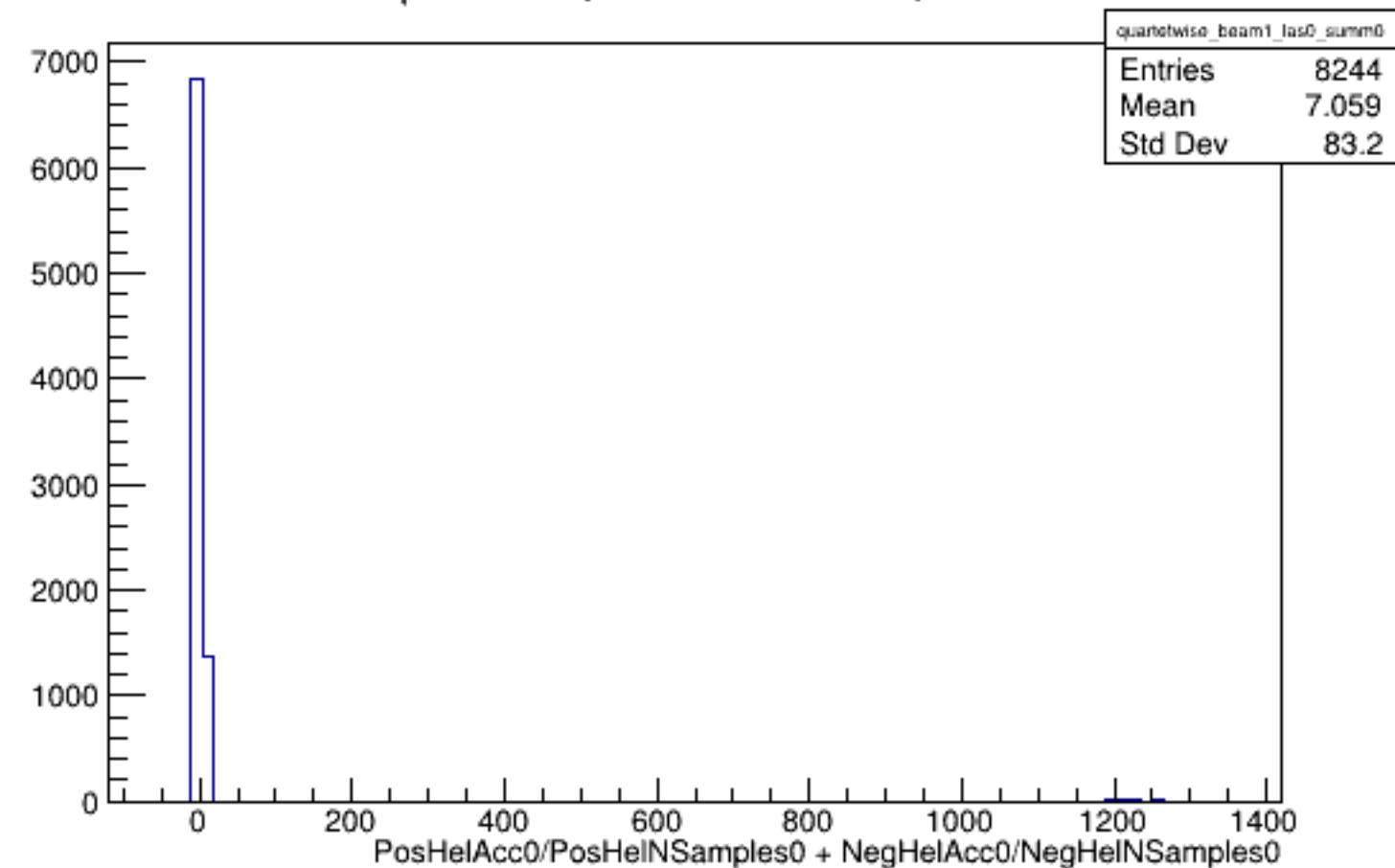
Run 5996 quartetwise, Sums0: Beam ON, Laser OFF
