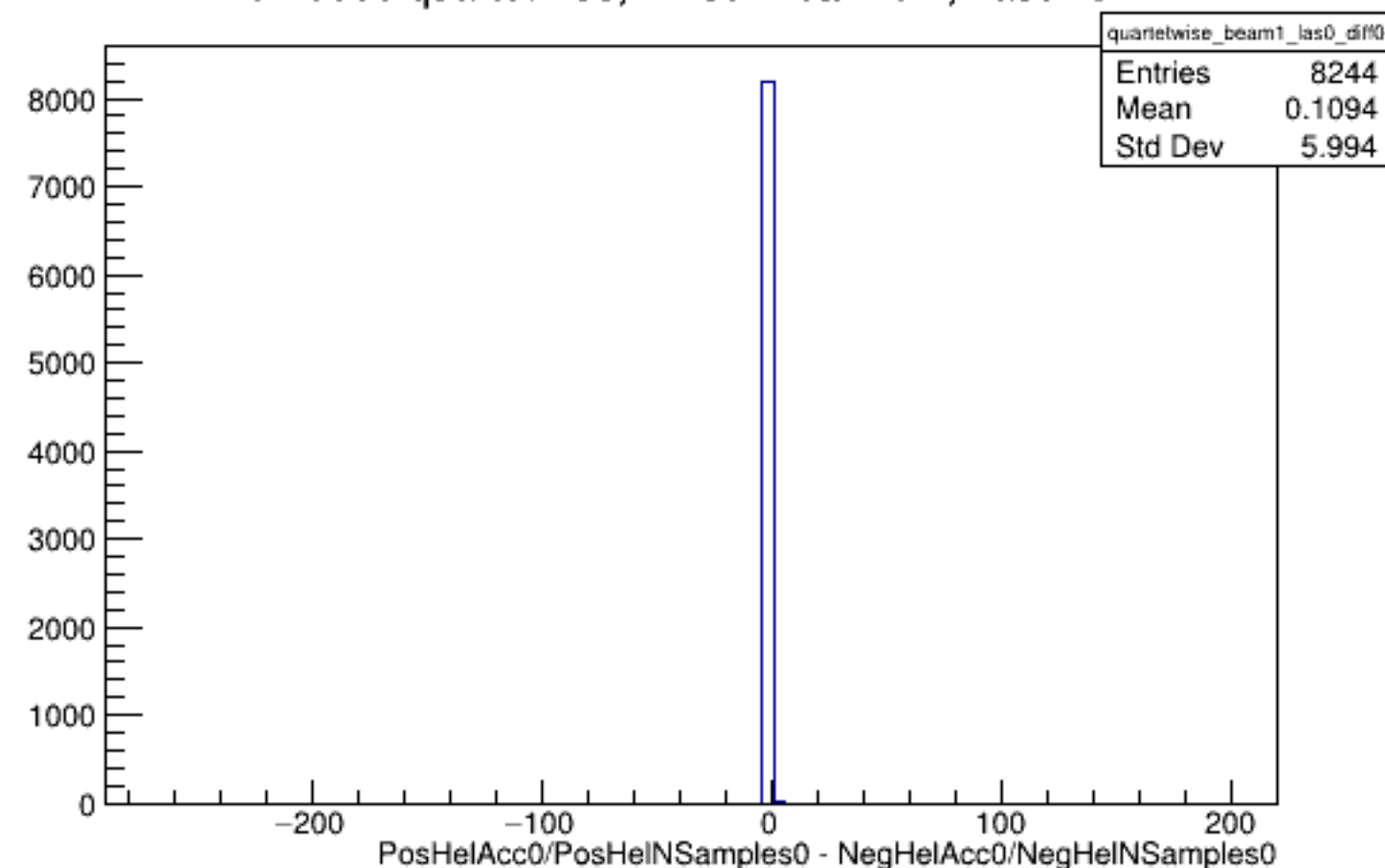
Run 5996 quartetwise, Diffs0: Beam ON, Laser OFF
