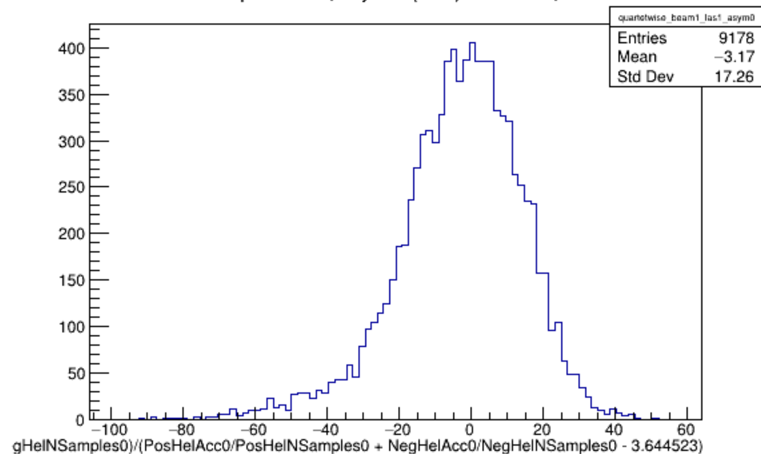
Run 5996 quartetwise, Asyms0 (Raw): Beam ON, Laser ON
