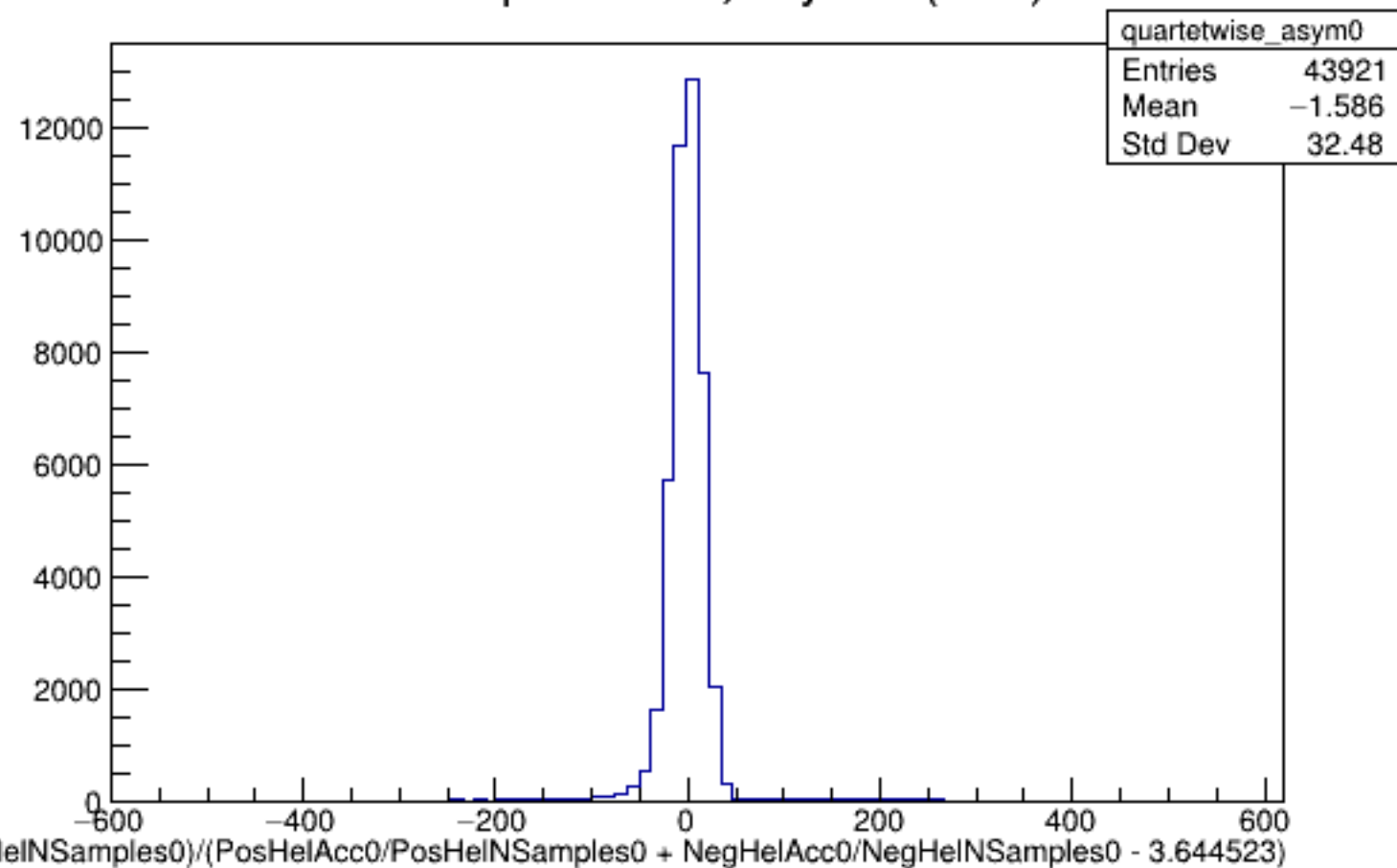
Run 5996 quartetwise, Asyms0 (Raw): All
