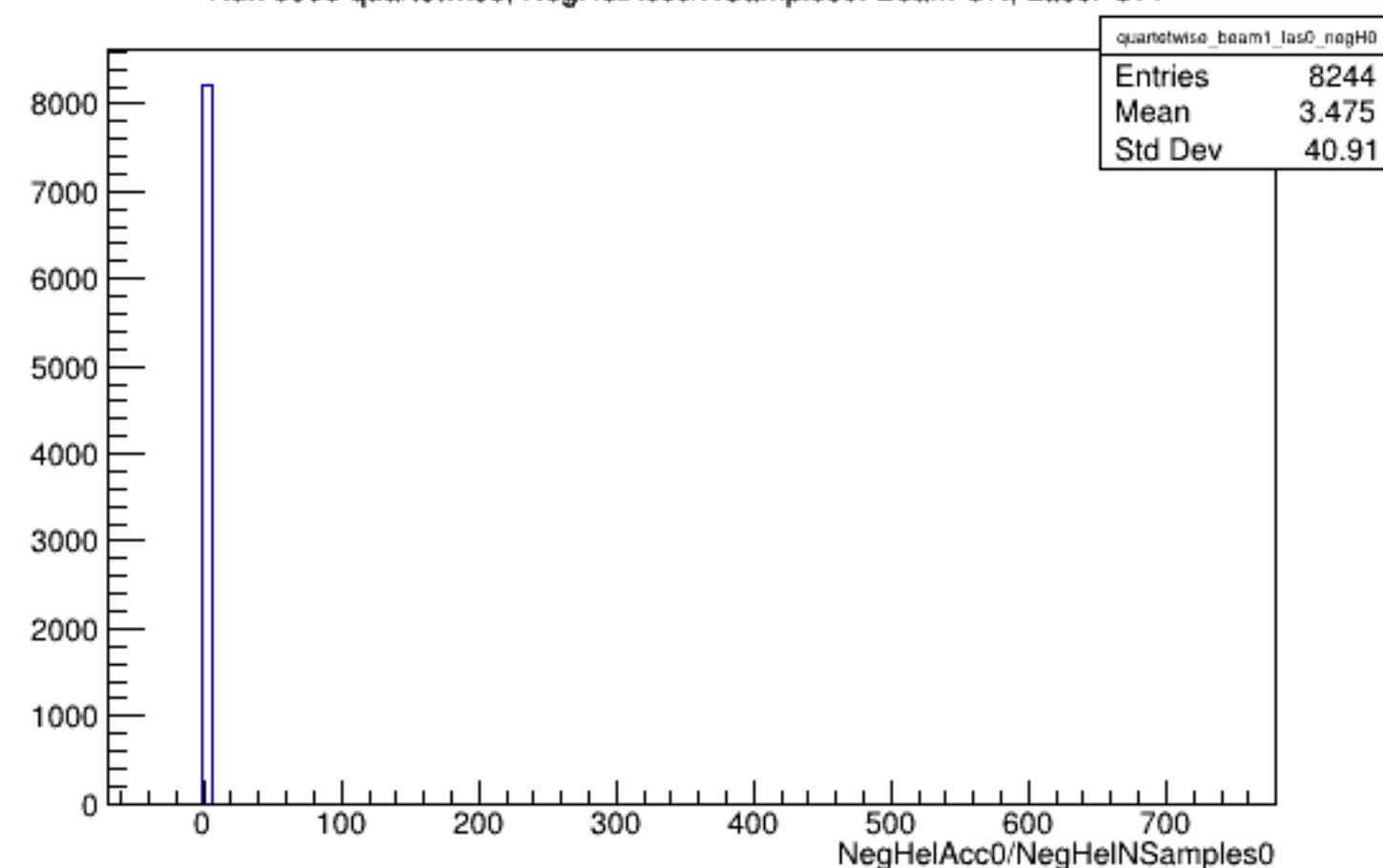
Run 5996 quartetwise, NegHelAcc0/NSamples0: Beam ON, Laser OFF
