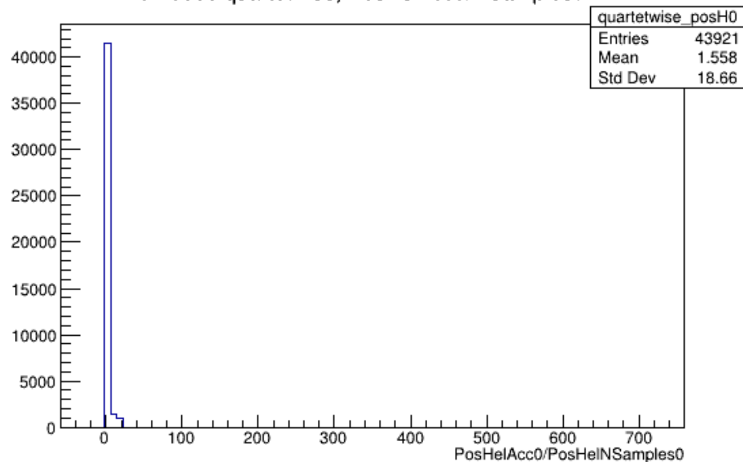
Run 5996 quartetwise, PosHelAcc0/NSamples0: All
