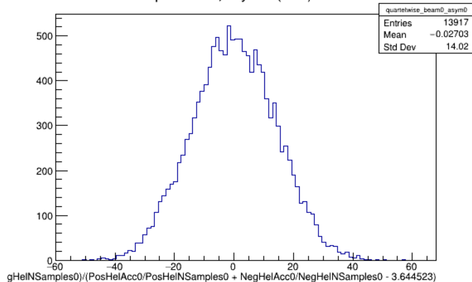
Run 5996 quartetwise, Asyms0 (Raw): Beam OFF
