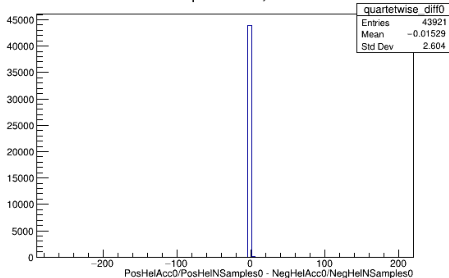
Run 5996 quartetwise, Diffs0: All
