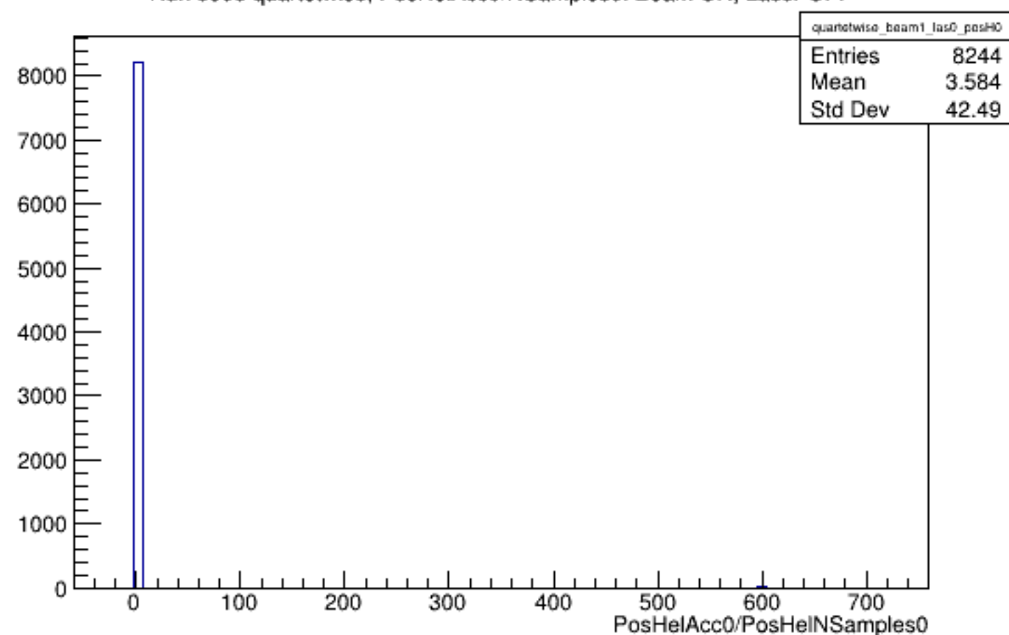
Run 5996 quartetwise, PosHelAcc0/NSamples0: Beam ON, Laser OFF
