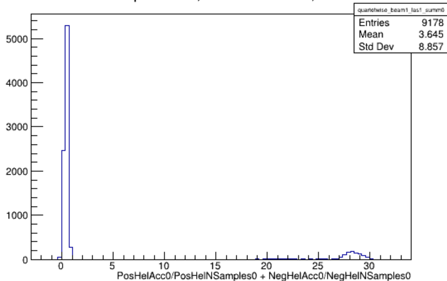
Run 5996 quartetwise, Sums0: Beam ON, Laser ON
