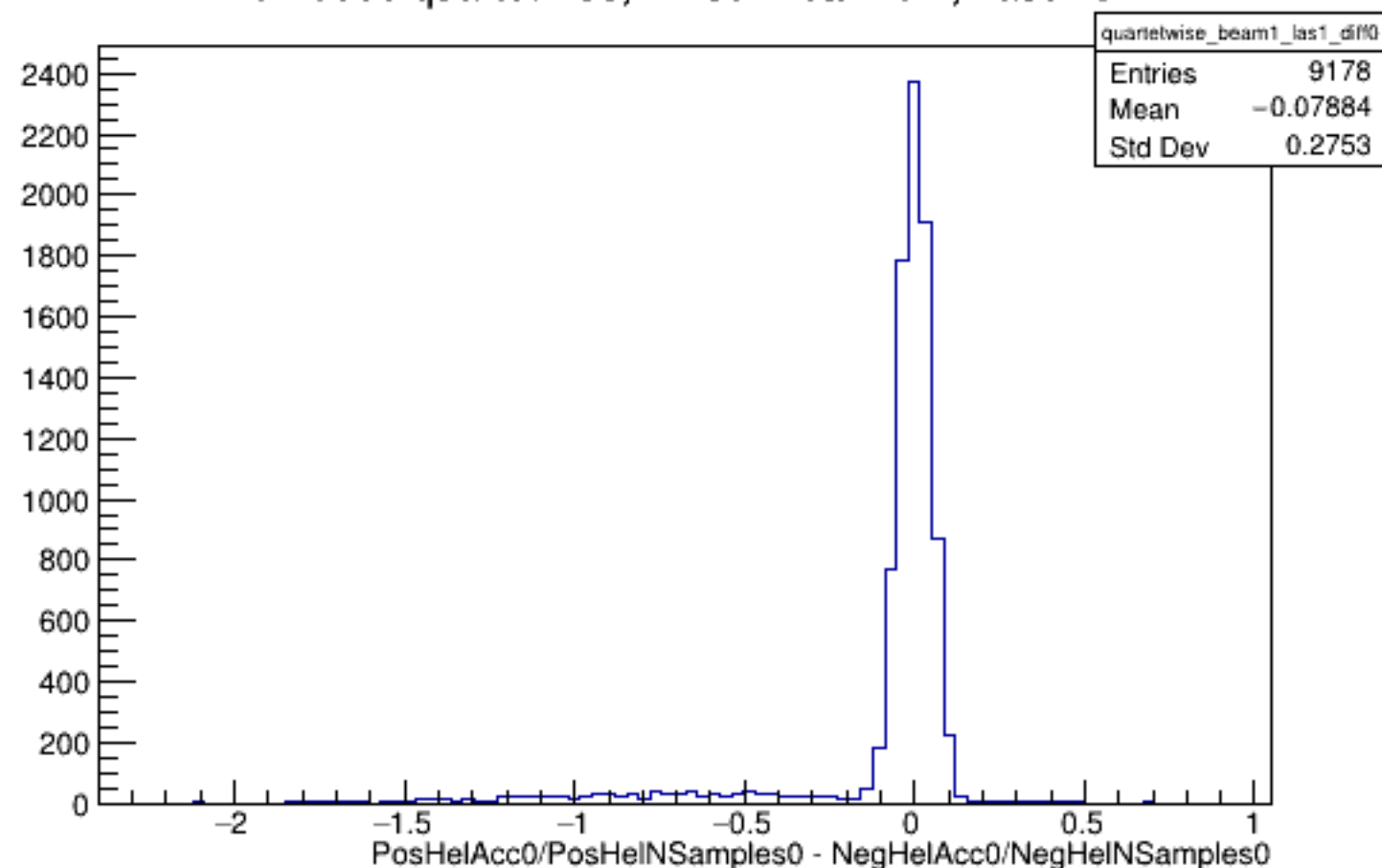
Run 5996 quartetwise, Diffs0: Beam ON, Laser ON
