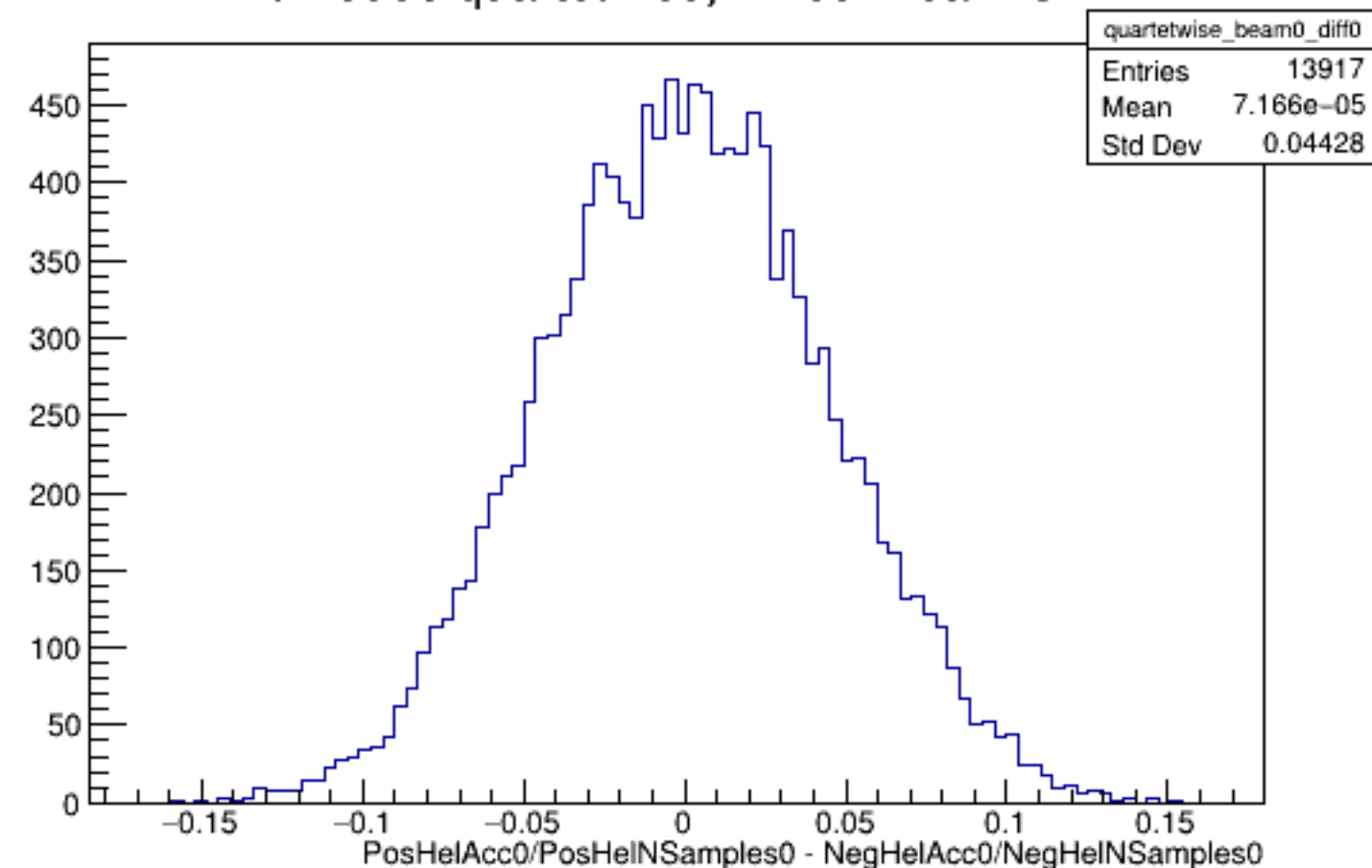
Run 5996 quartetwise, Diffs0: Beam OFF
