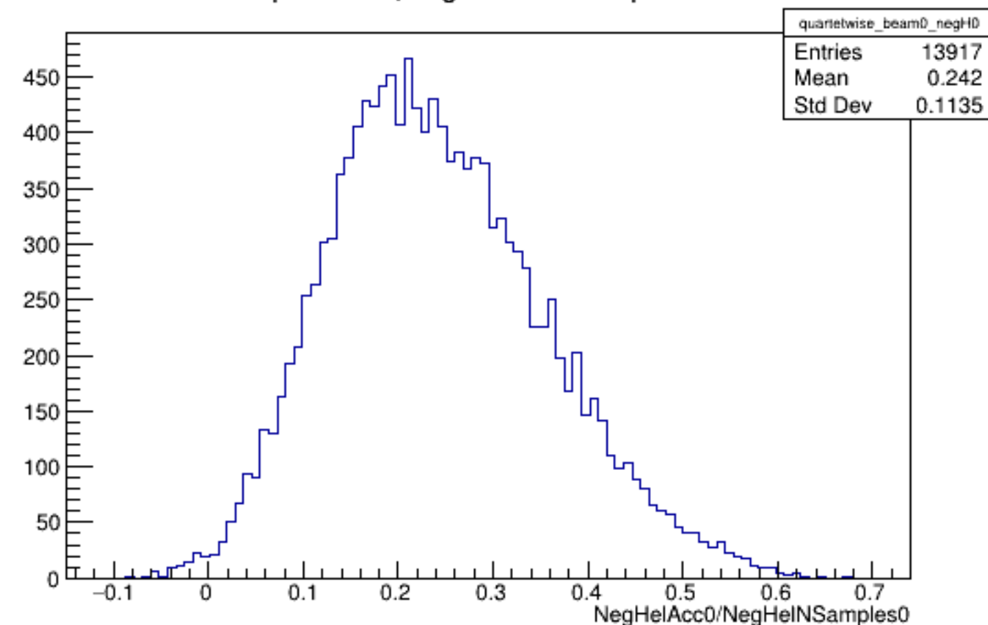
Run 5996 quartetwise, NegHelAcc0/NSamples0: Beam OFF
