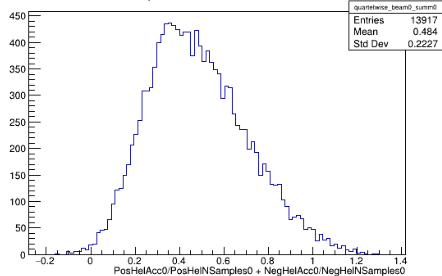
Run 5996 quartetwise, Sums0: Beam OFF
