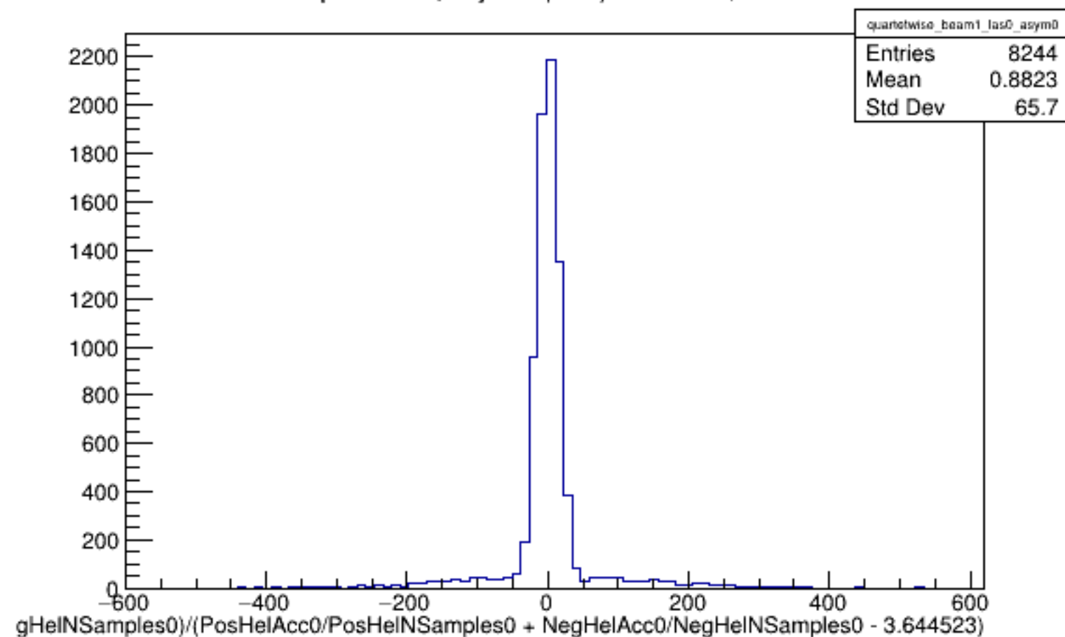
Run 5996 quartetwise, Asyms0 (Raw): Beam ON, Laser OFF
