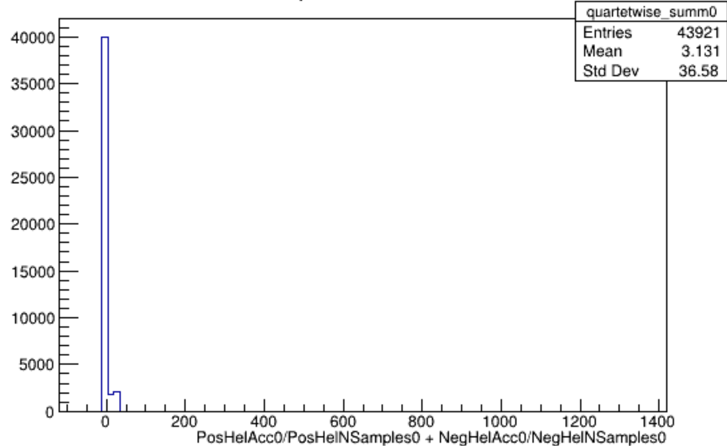
Run 5996 quartetwise, Sums0: All
