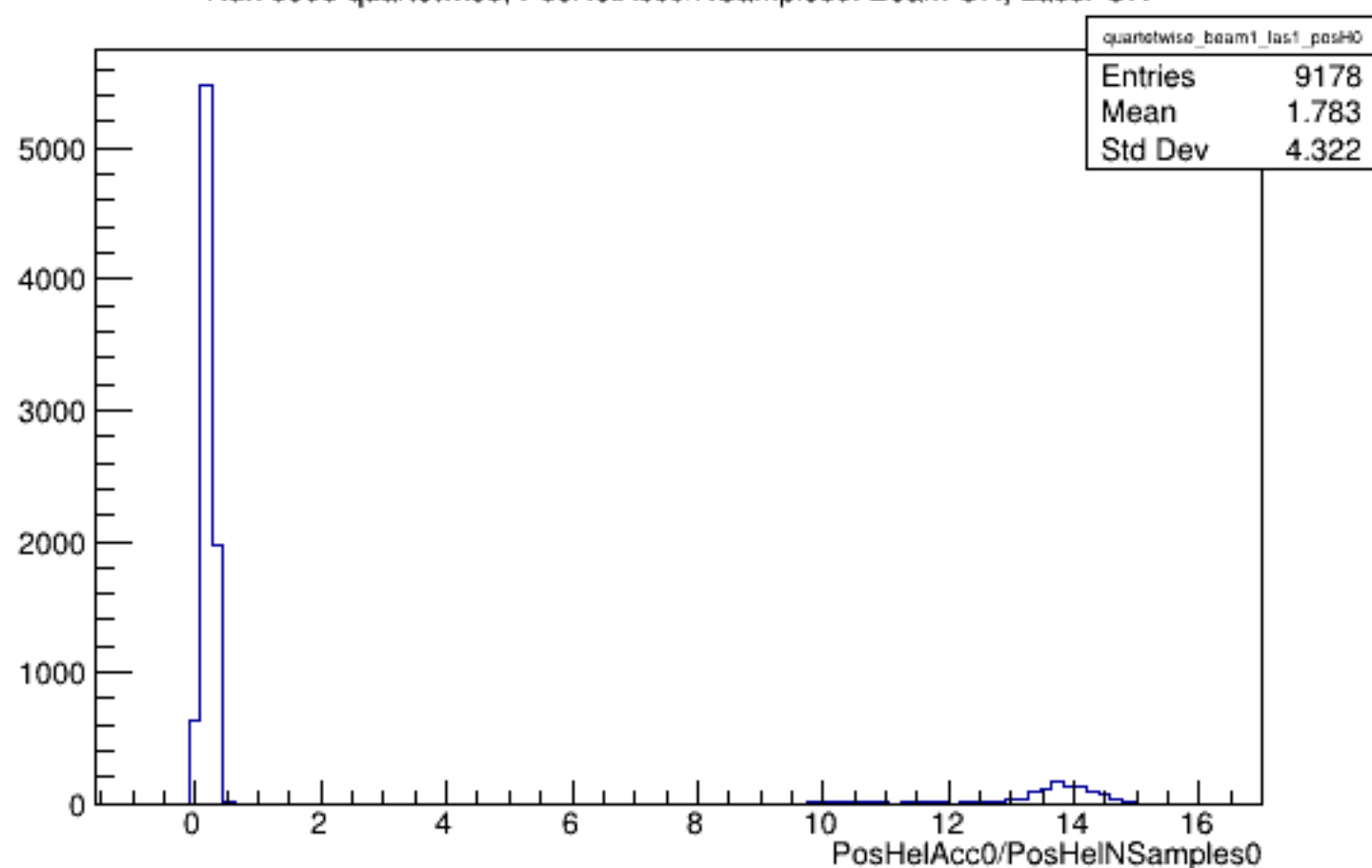
Run 5996 quartetwise, PosHelAcc0/NSamples0: Beam ON, Laser ON
