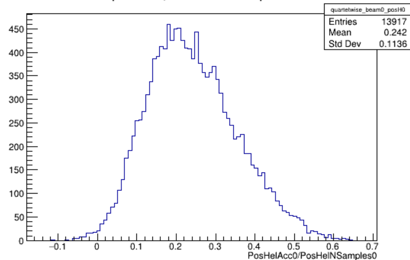
Run 5996 quartetwise, PosHelAcc0/NSamples0: Beam OFF
