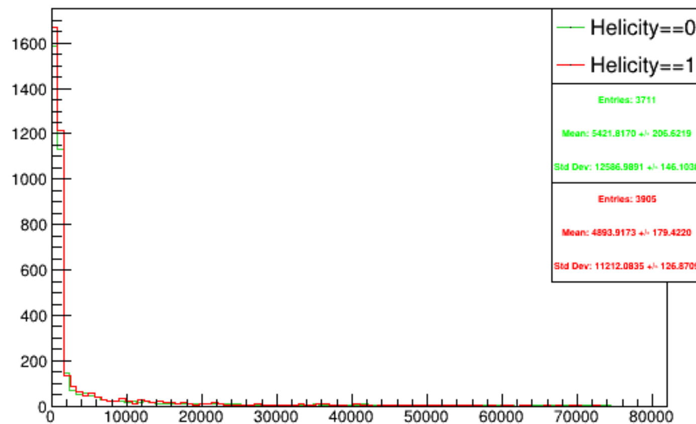
Run 5996 triggerwise, sums: Beam ON, Laser OFF
