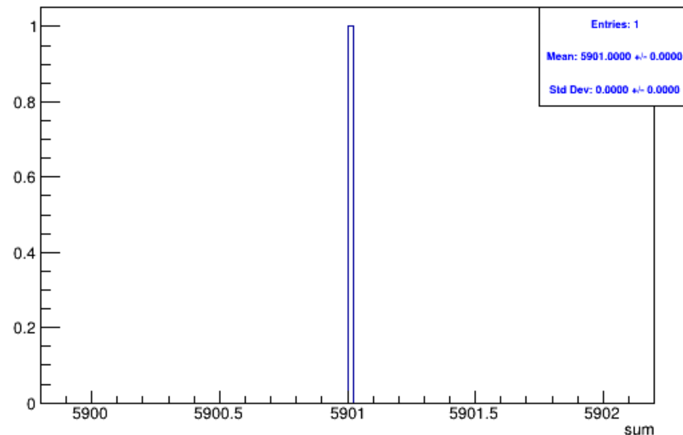
Run 5996 triggerwise, sums: Beam OFF
