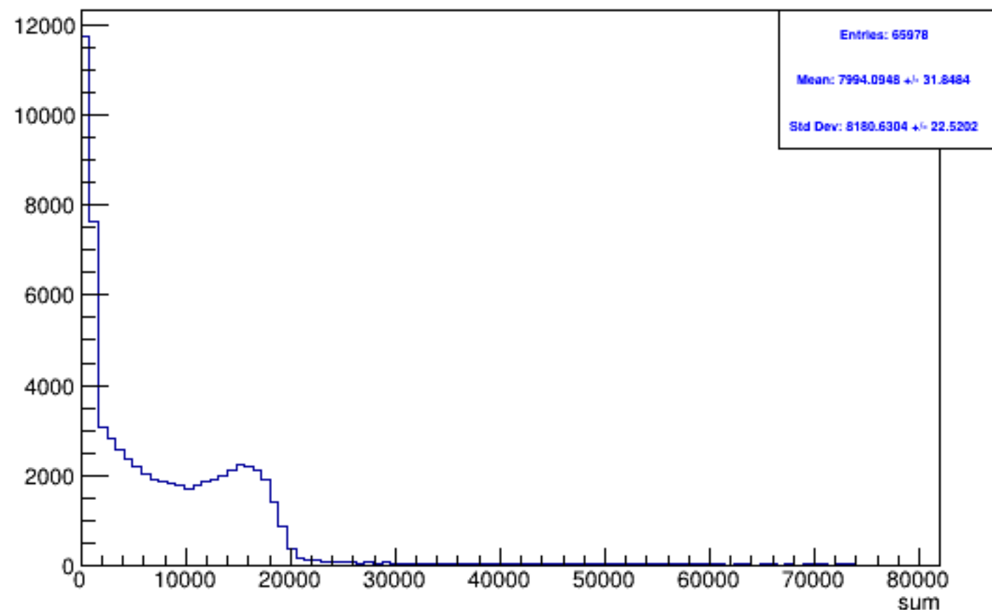
Run 5996 triggerwise, sums: All
