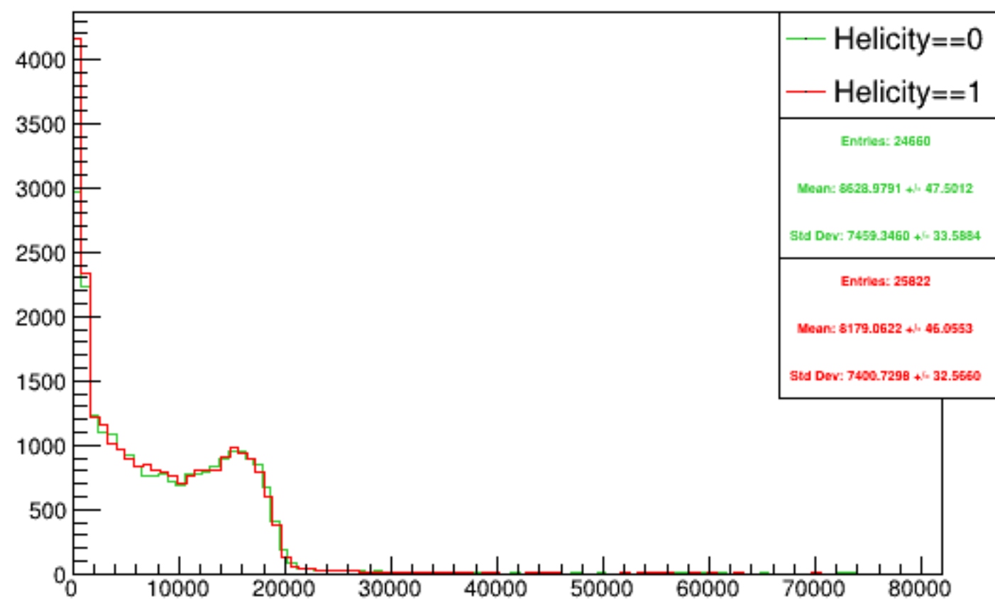
Run 5996 triggerwise, sums: Beam ON, Laser ON
