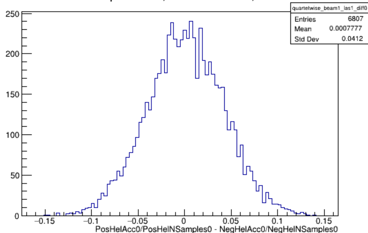
Run 5997 quartetwise, Diffs0: Beam ON, Laser ON
