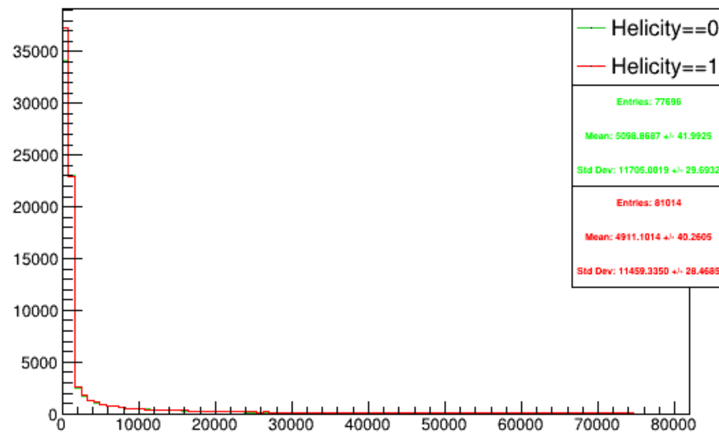
Run 5998 triggerwise, sums: Beam ON, Laser OFF
