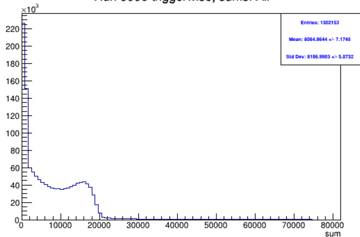
Run 5998 triggerwise, sums: All
