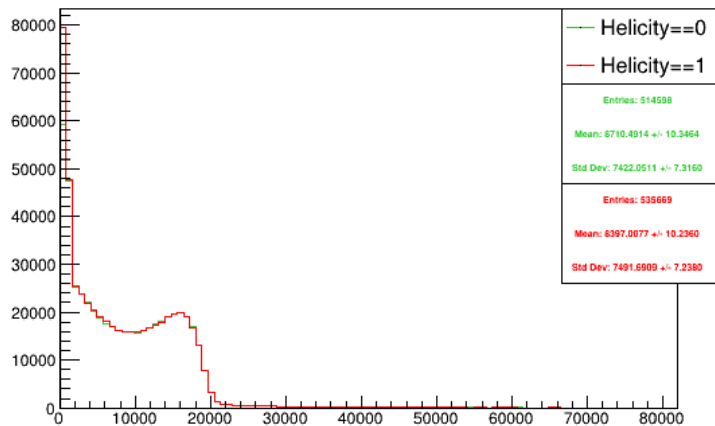
Run 5998 triggerwise, sums: Beam ON, Laser ON
