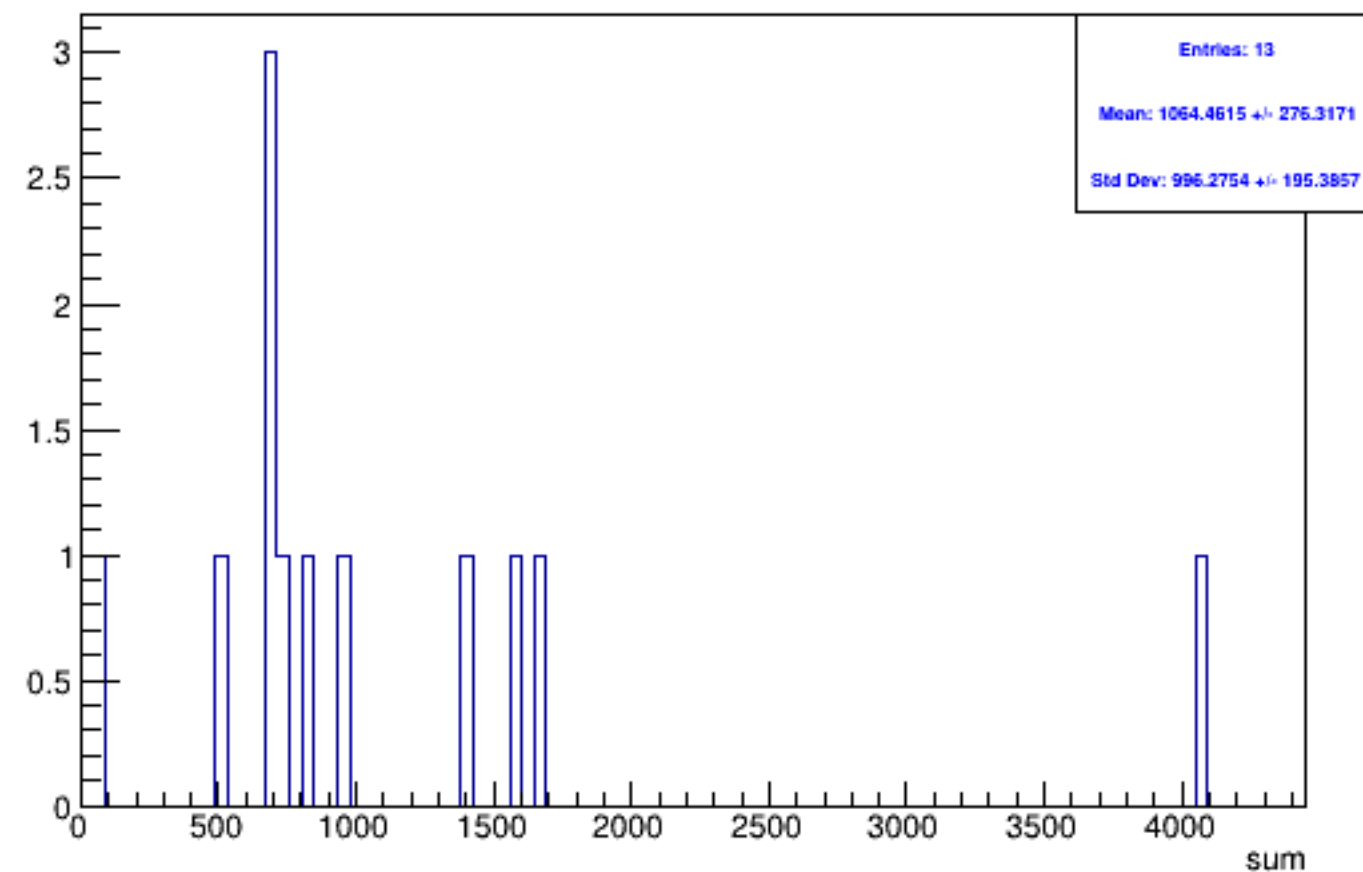
Run 5998 triggerwise, sums: Beam OFF
