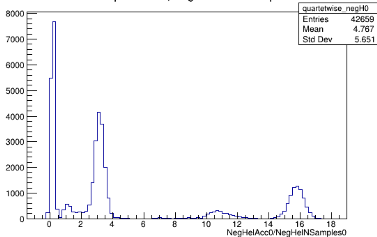
Run 6004 quartetwise, NegHelAcc0/NSamples0: All
