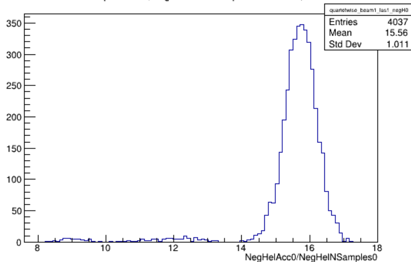
Run 6004 quartetwise, NegHelAcc0/NSamples0: Beam ON, Laser ON
