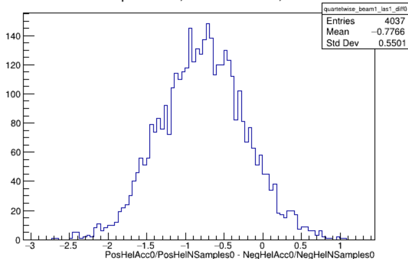
Run 6004 quartetwise, Diffs0: Beam ON, Laser ON
