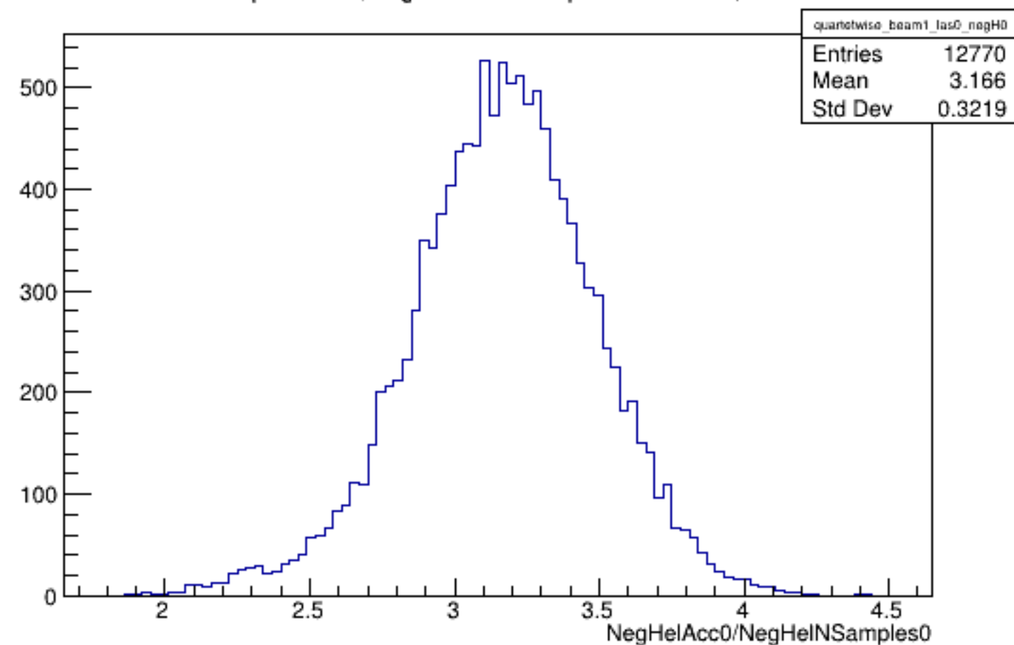
Run 6004 quartetwise, NegHelAcc0/NSamples0: Beam ON, Laser OFF
