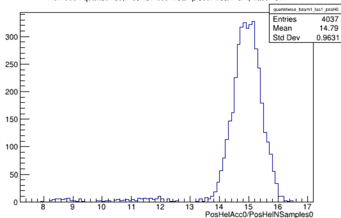
Run 6004 quartetwise, PosHelAcc0/NSamples0: Beam ON, Laser ON
