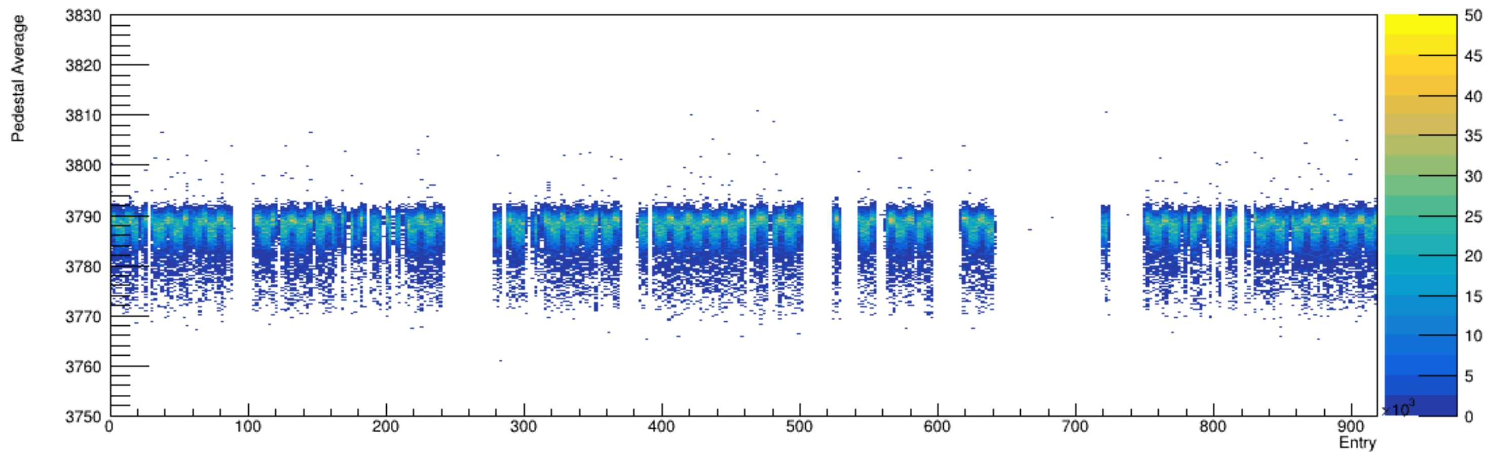
Run 6005, snapshots: Pedestal vs. Time
