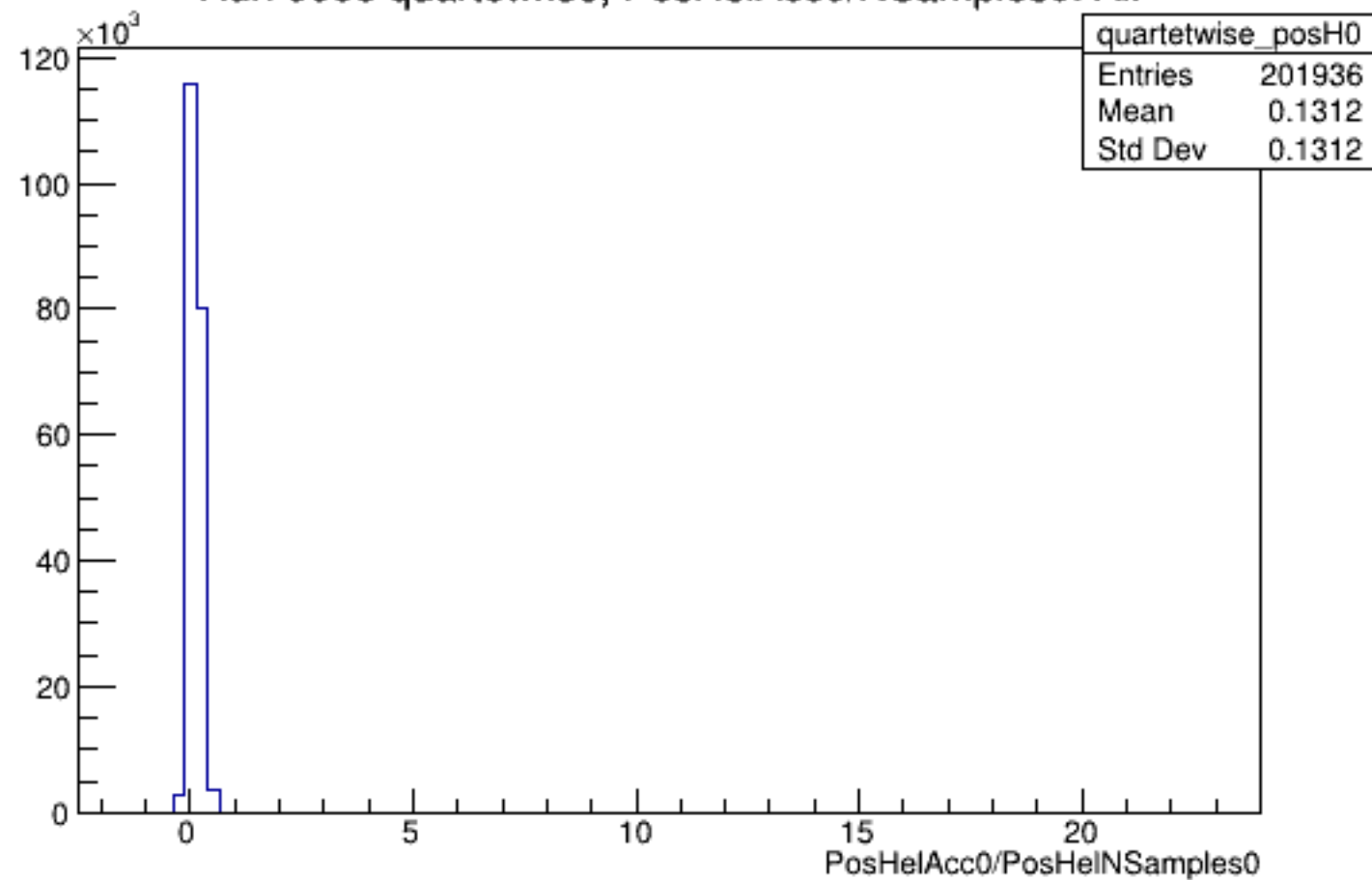
Run 6008 quartetwise, PosHelAcc0/NSamples0: All
