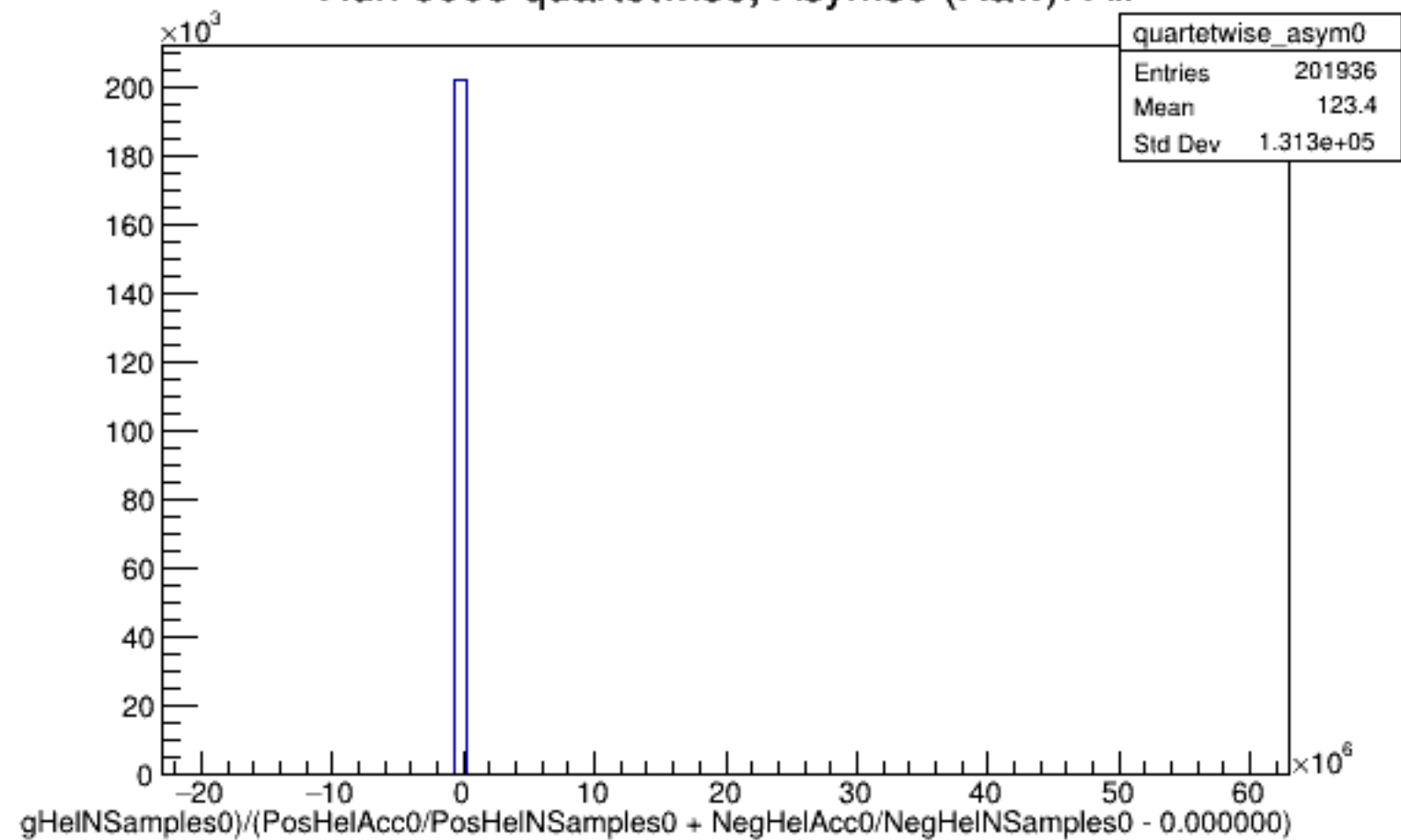
Run 6008 quartetwise, Asyms0 (Raw): All
