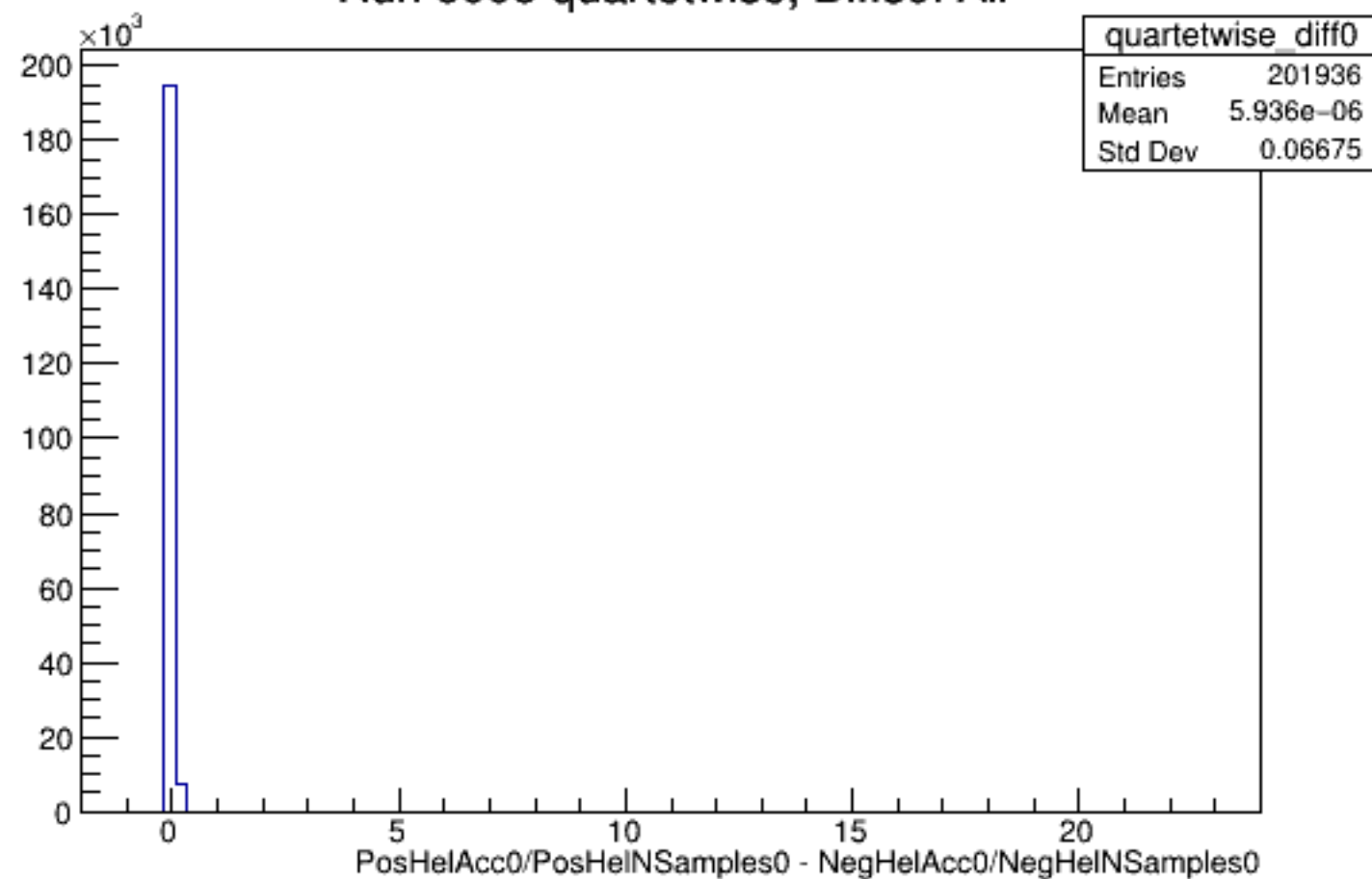
Run 6008 quartetwise, Diffs0: All
