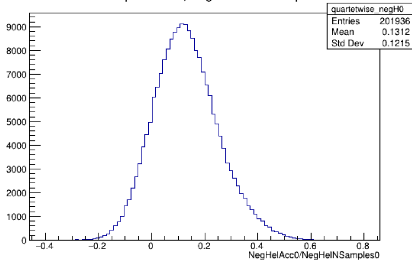
Run 6008 quartetwise, NegHelAcc0/NSamples0: All
