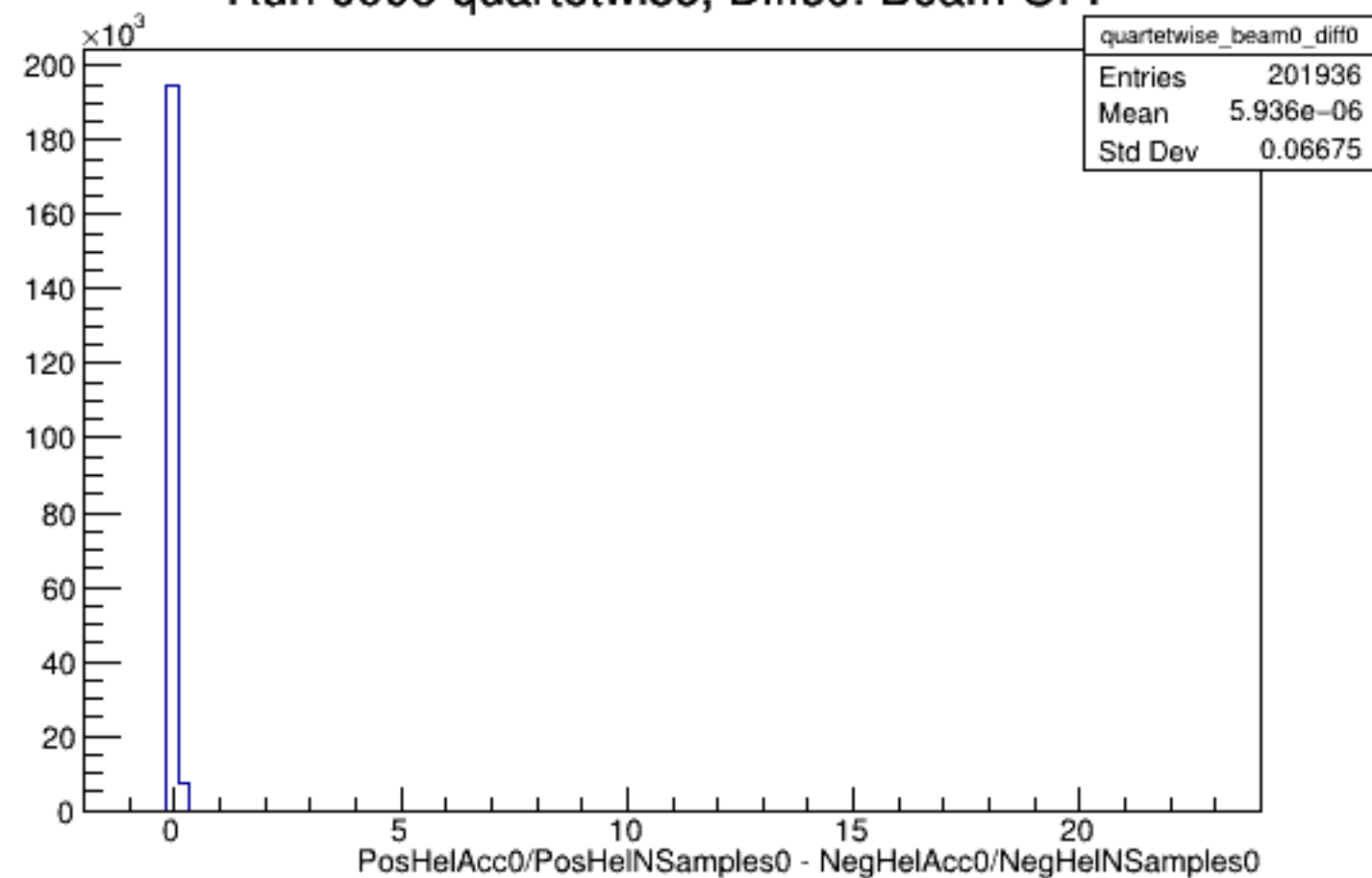
Run 6008 quartetwise, Diffs0: Beam OFF
