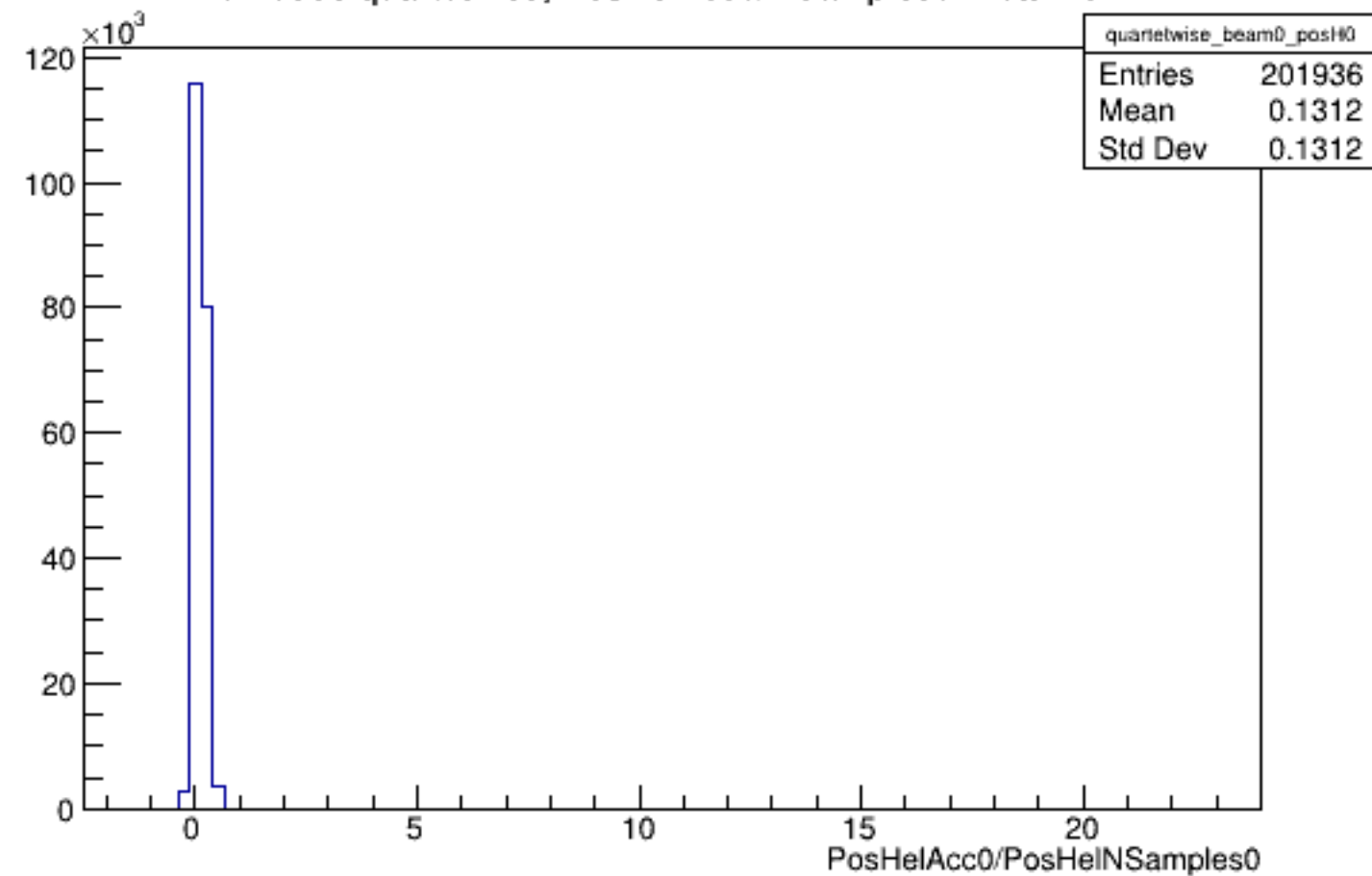
Run 6008 quartetwise, PosHelAcc0/NSamples0: Beam OFF
