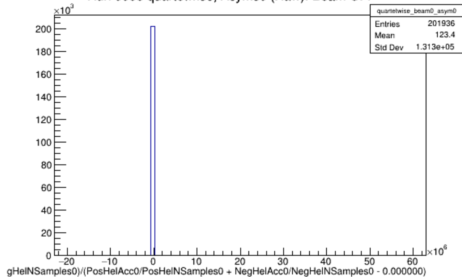
Run 6008 quartetwise, Asyms0 (Raw): Beam OFF
