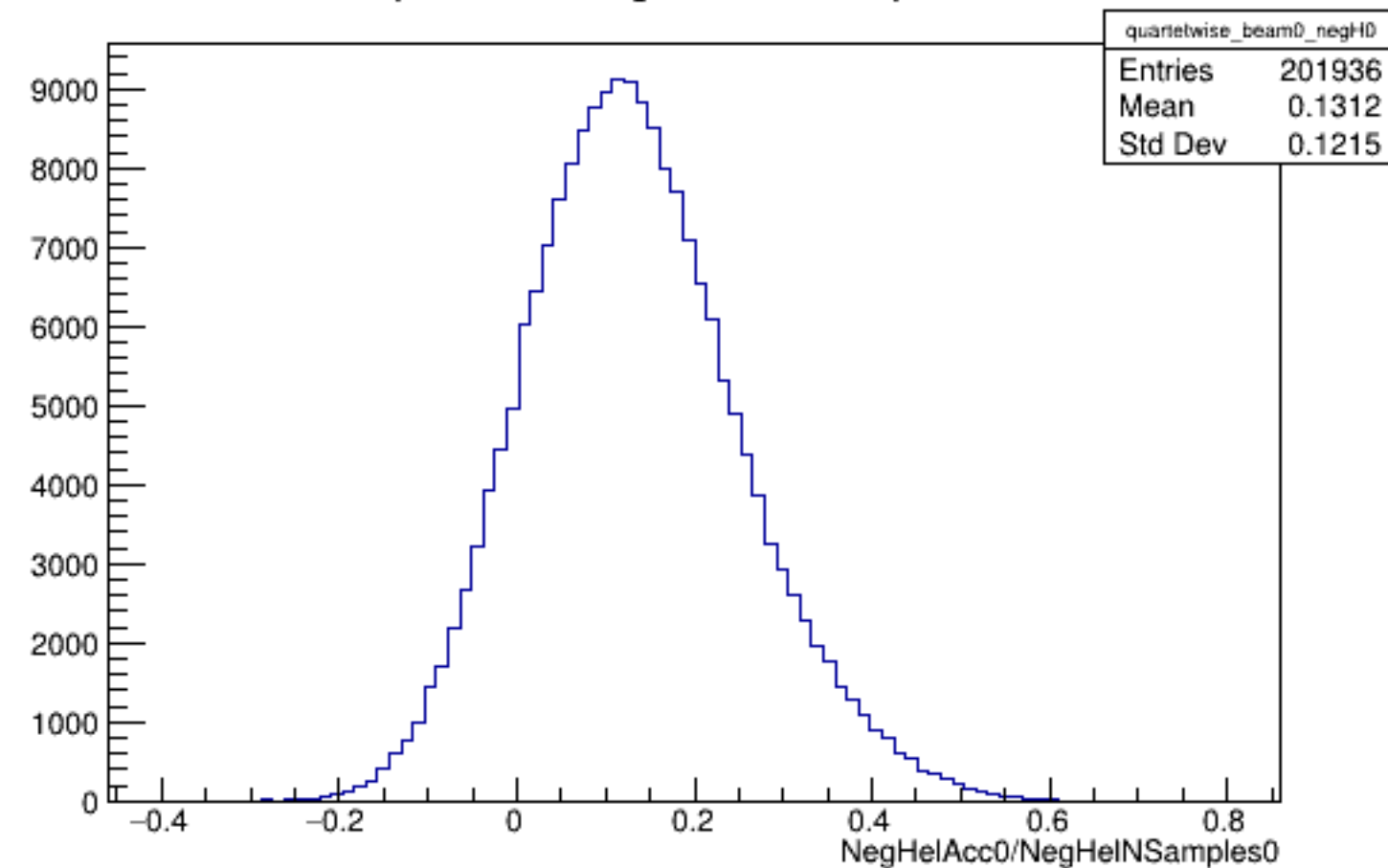
Run 6008 quartetwise, NegHelAcc0/NSamples0: Beam OFF
