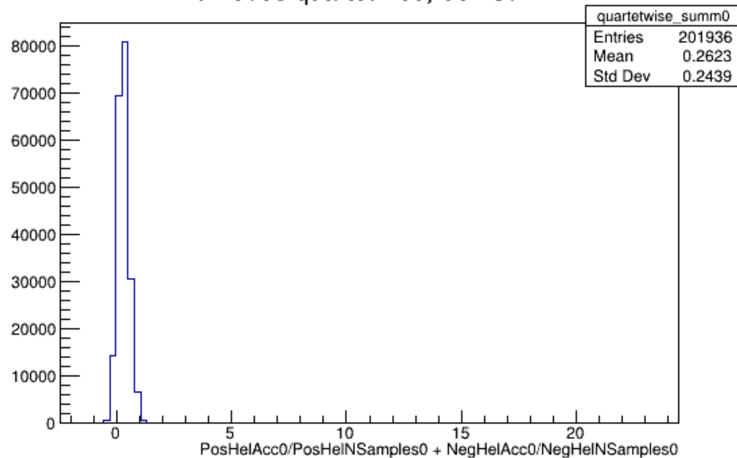
Run 6008 quartetwise, Sums0: All
