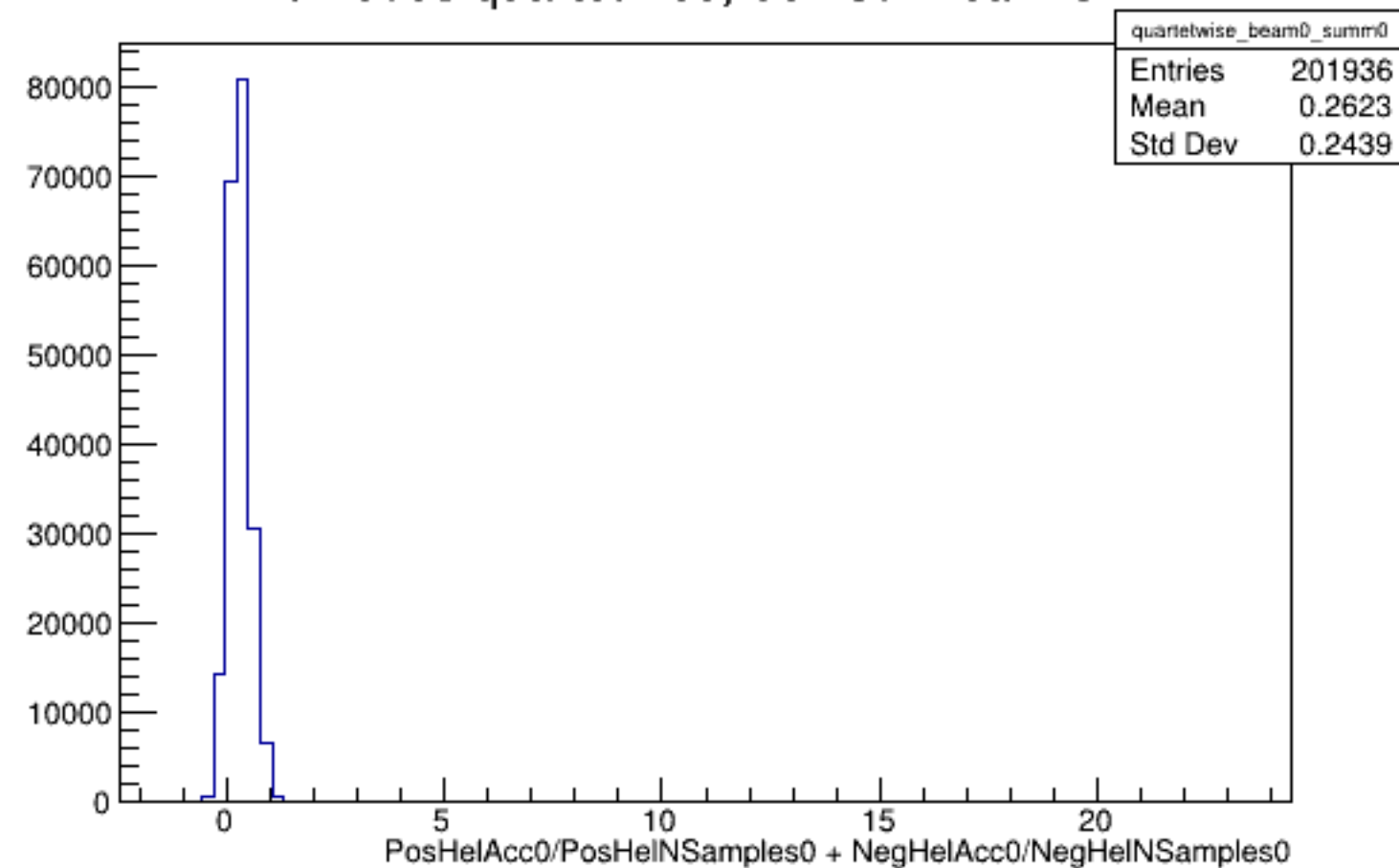
Run 6008 quartetwise, Sums0: Beam OFF
