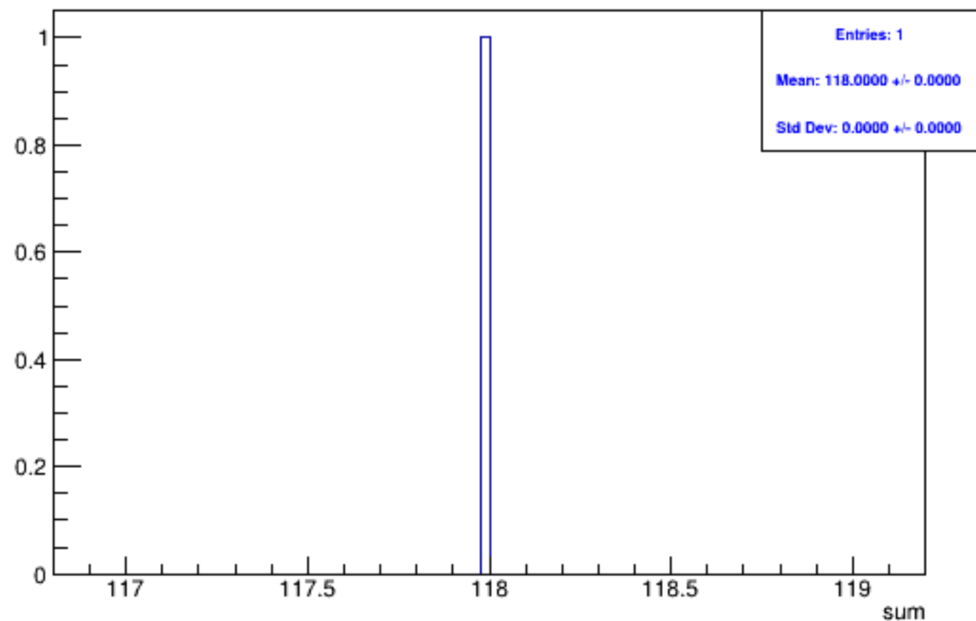
Run 6011 triggerwise, sums: All
