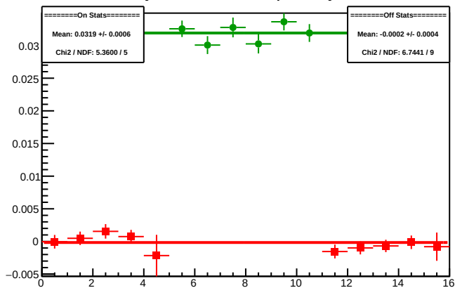
Cycle 6016.3: Multiplet Asyms
