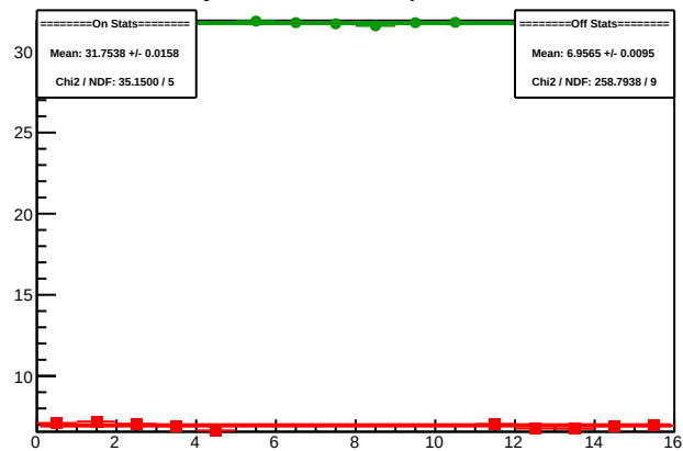
Cycle 6016.3: Multiplet Sums
