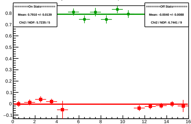
Cycle 6016.3: Multiplet Diffs
