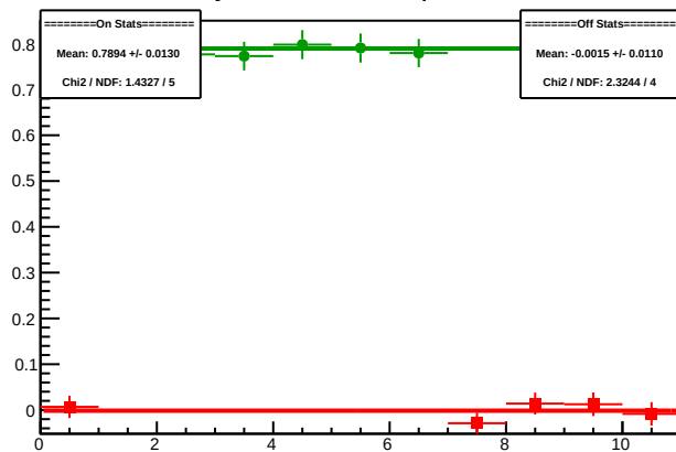
Cycle 6016.4: Multiplet Diffs
