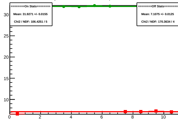
Cycle 6016.4: Multiplet Sums
