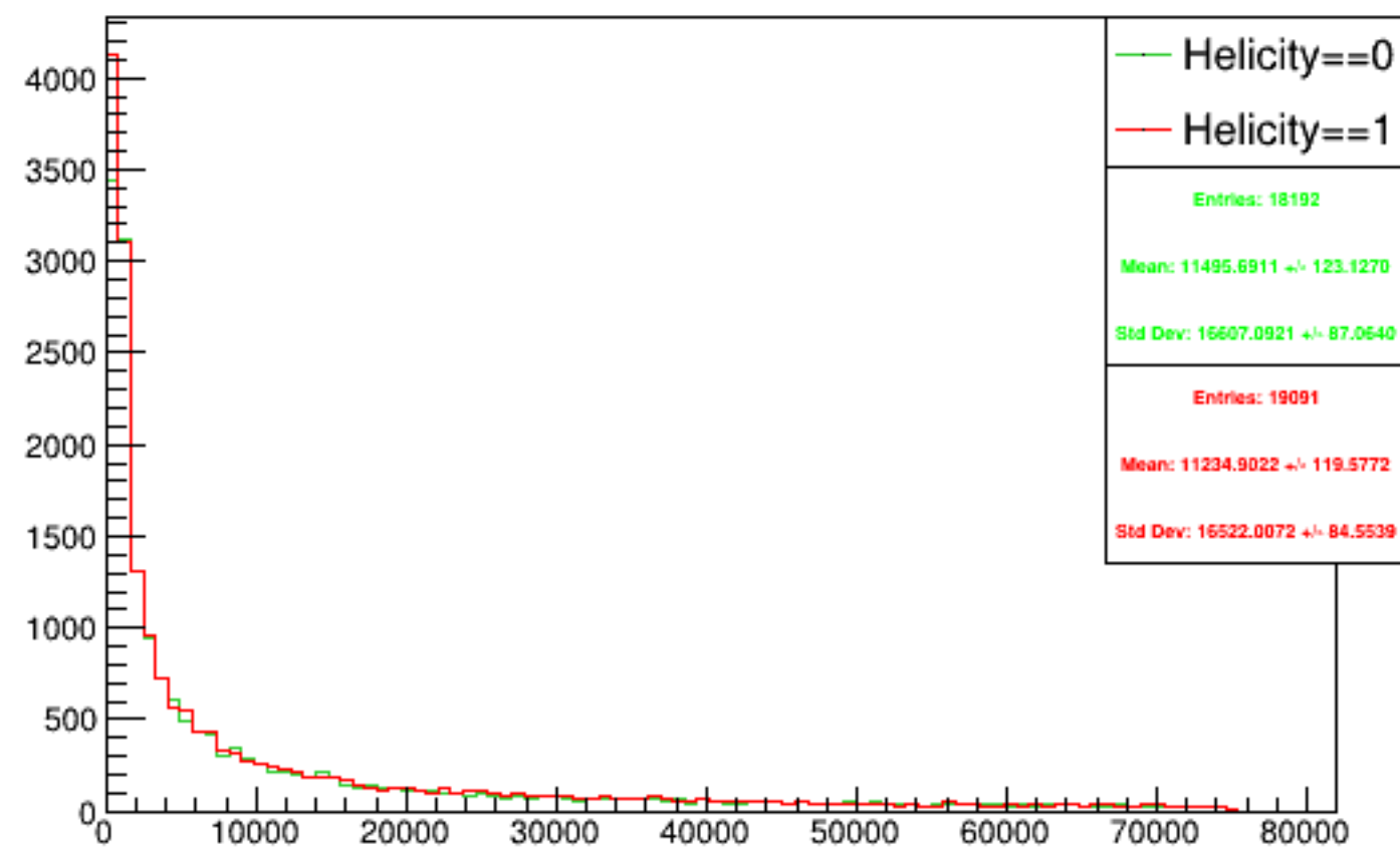
Run 6021 triggerwise, sums: Beam ON, Laser OFF
