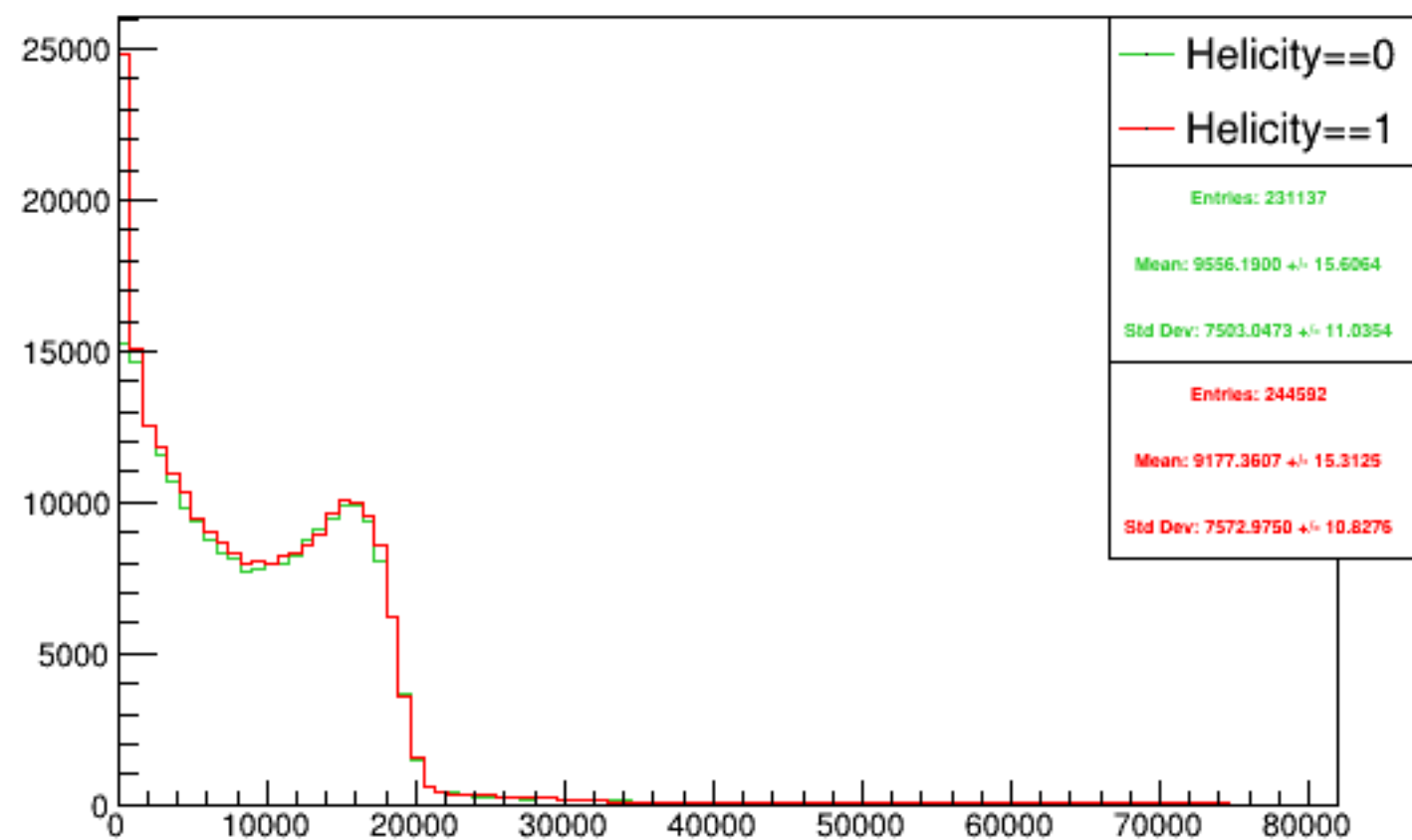
Run 6021 triggerwise, sums: Beam ON, Laser ON
