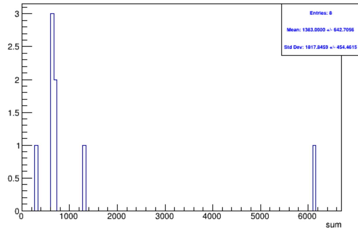
Run 6021 triggerwise, sums: Beam OFF
