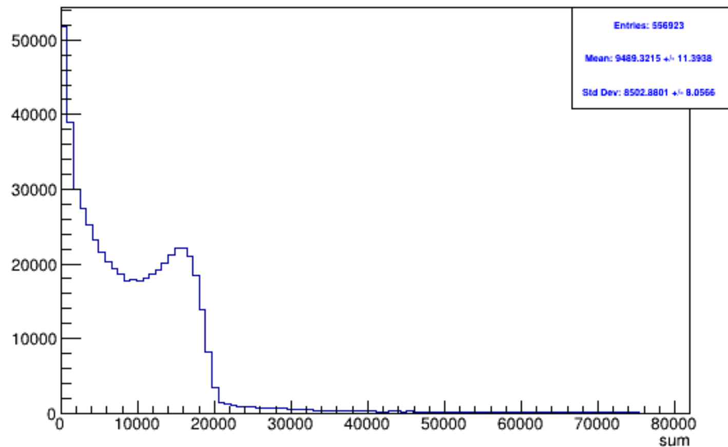
Run 6021 triggerwise, sums: All
