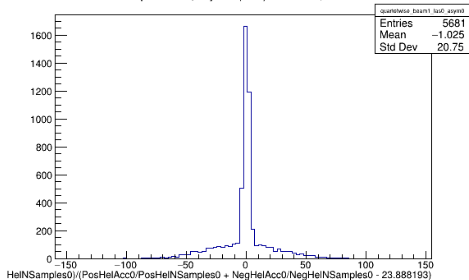
Run 6024 quartetwise, Asyms0 (Raw): Beam ON, Laser OFF
