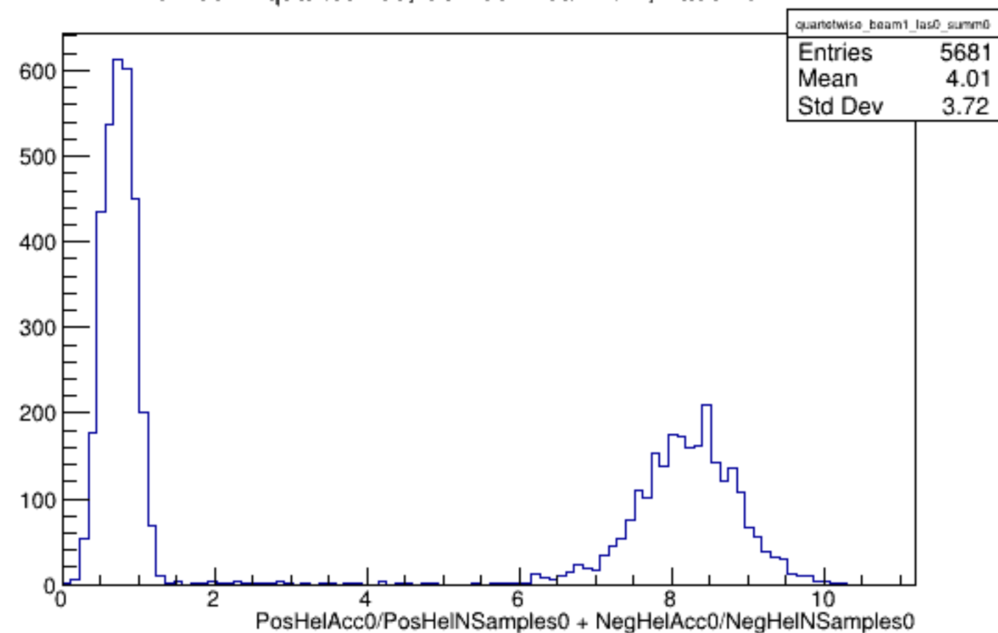
Run 6024 quartetwise, Sums0: Beam ON, Laser OFF
