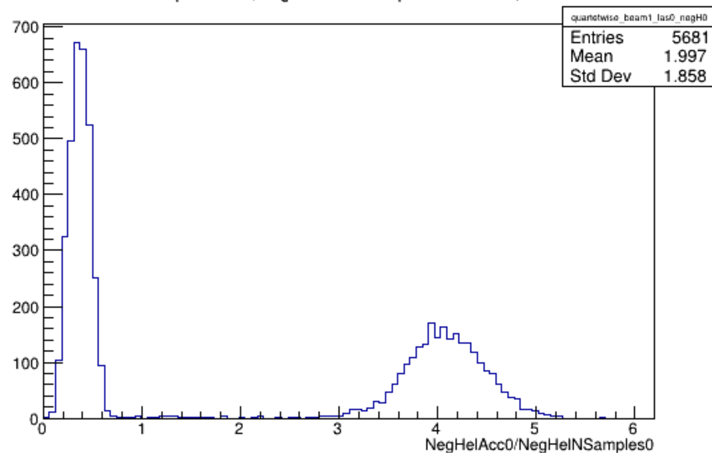
Run 6024 quartetwise, NegHelAcc0/NSamples0: Beam ON, Laser OFF
