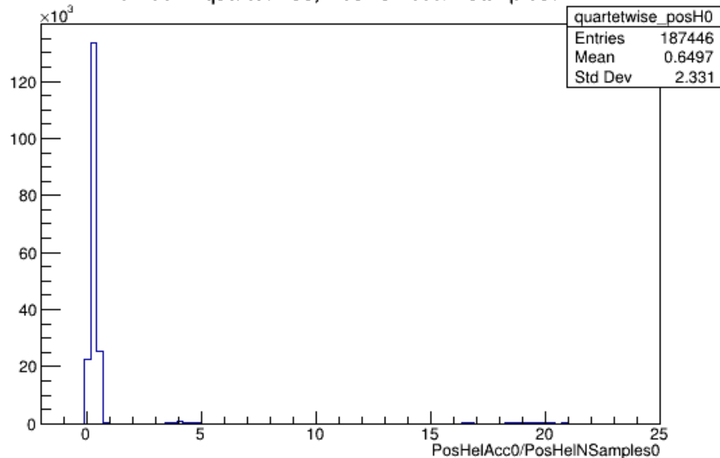
Run 6024 quartetwise, PosHelAcc0/NSamples0: All
