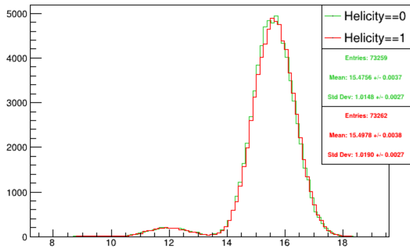
Run 6026 mpwise, acc0: Beam ON, Laser ON
