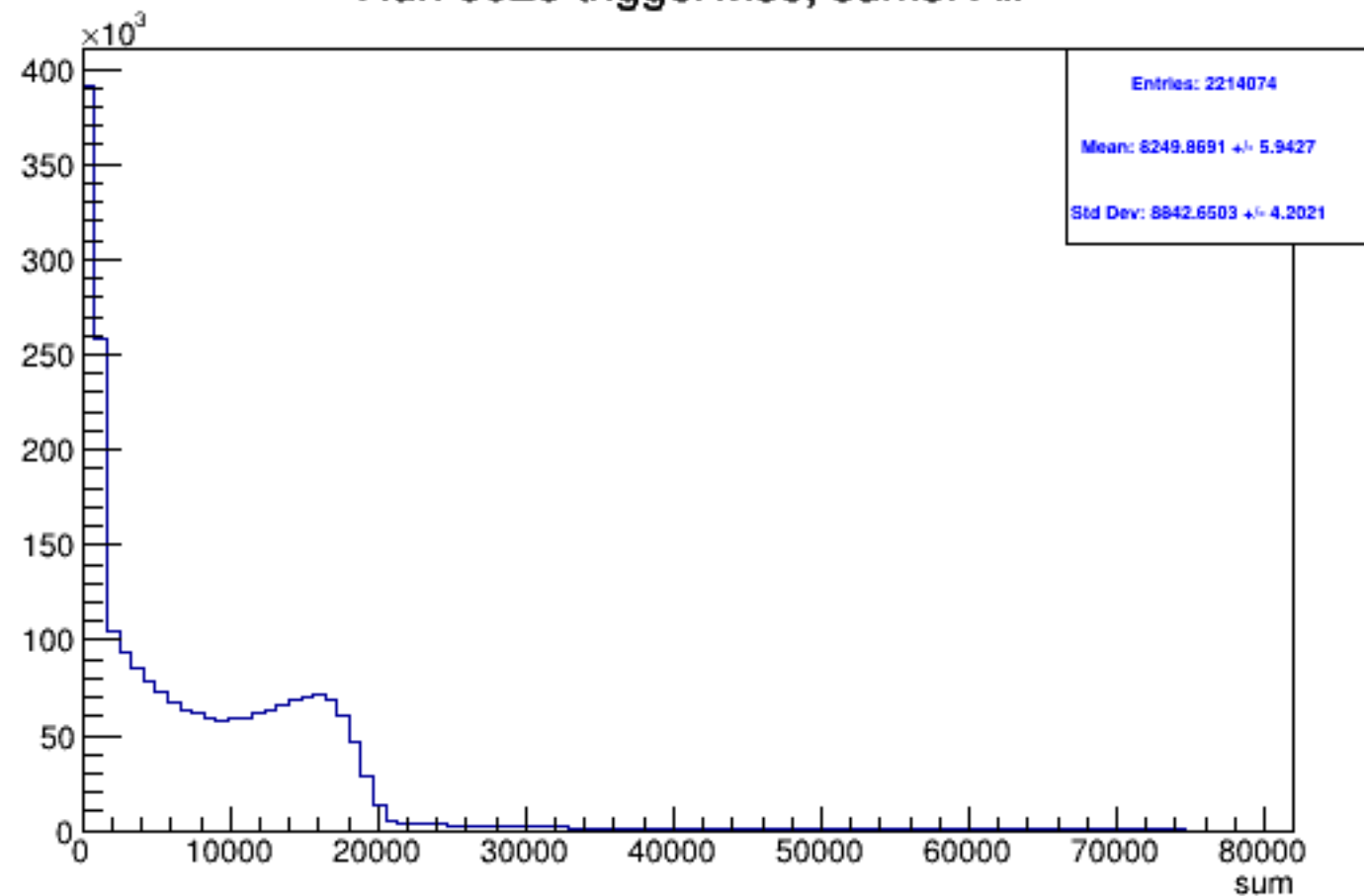
Run 6026 triggerwise, sums: All
