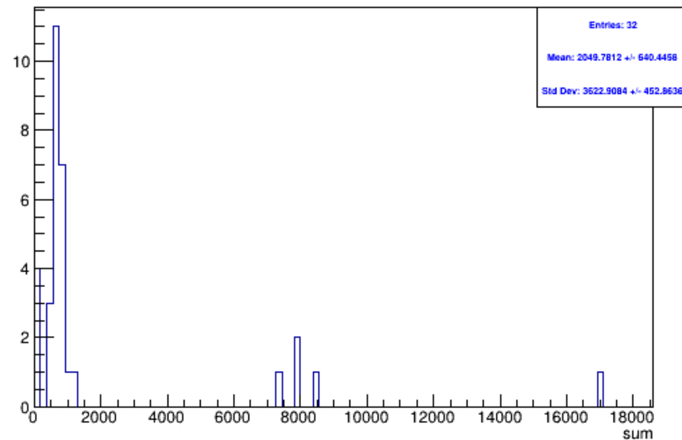
Run 6026 triggerwise, sums: Beam OFF
