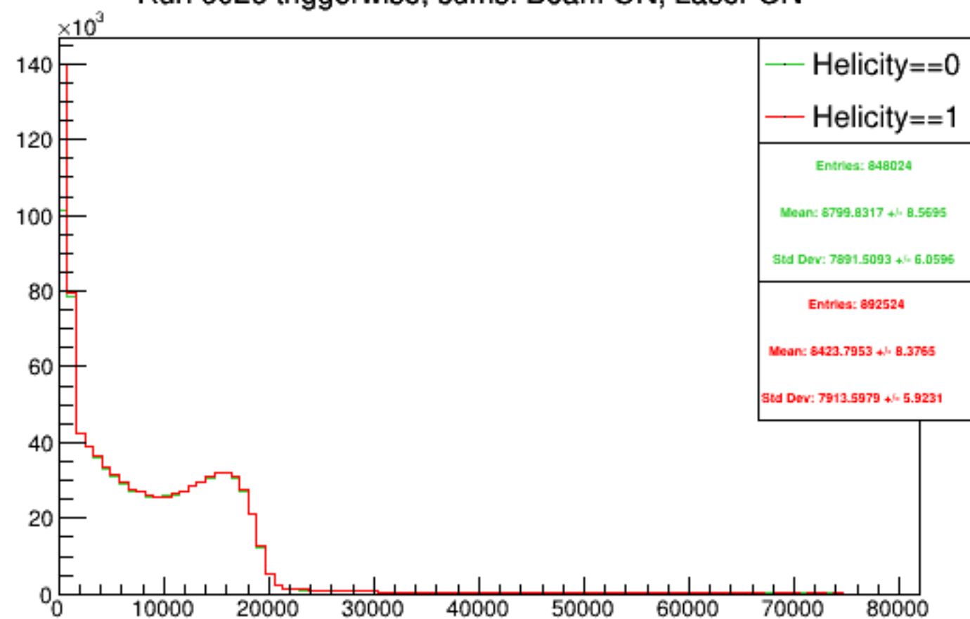
Run 6026 triggerwise, sums: Beam ON, Laser ON
