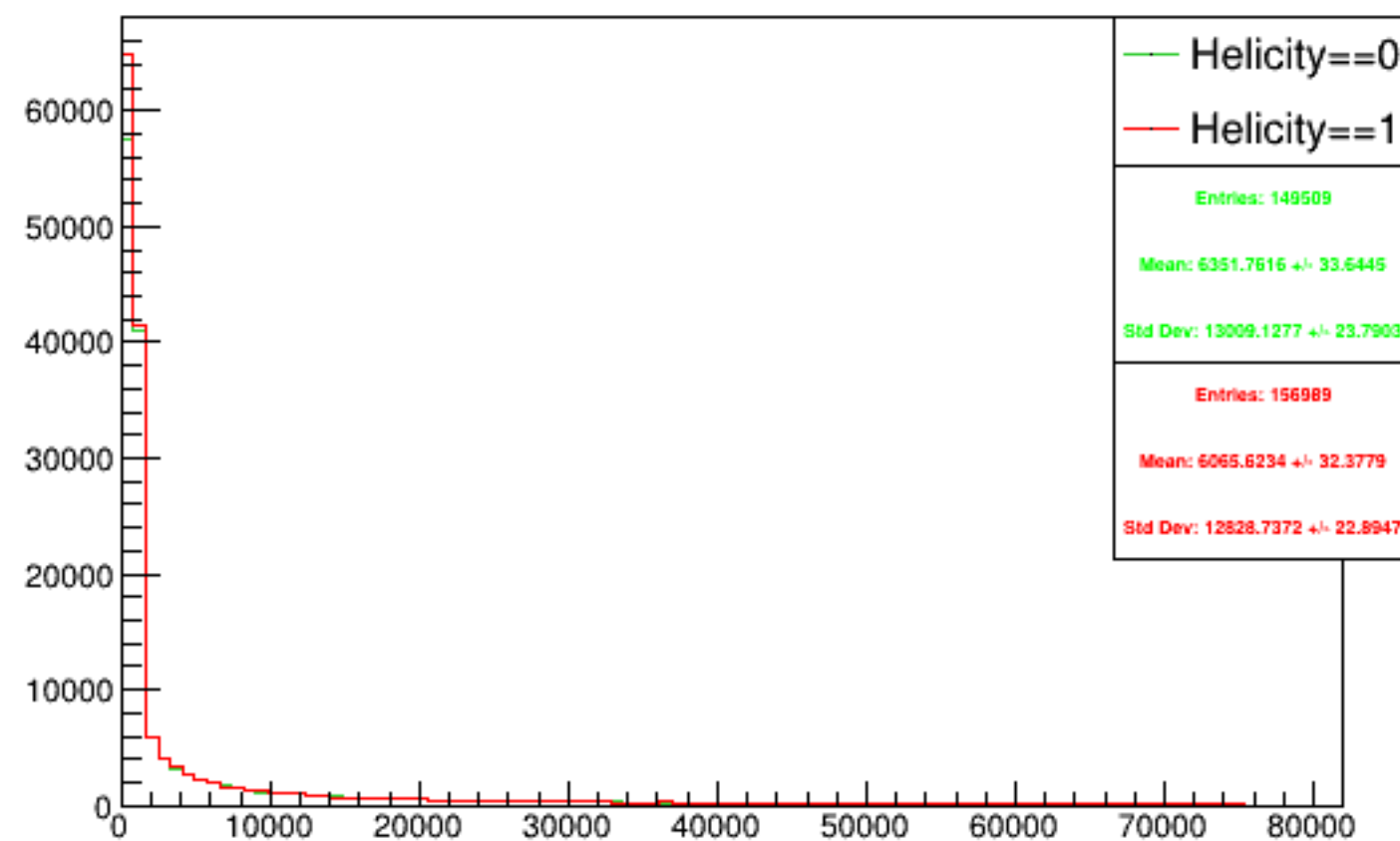
Run 6026 triggerwise, sums: Beam ON, Laser OFF
