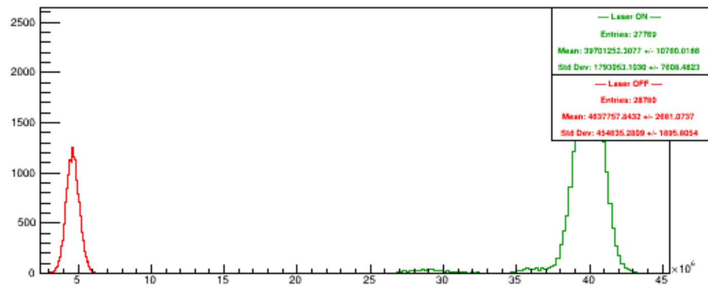
Run 6030 quartetwise, PosHelAcc4
