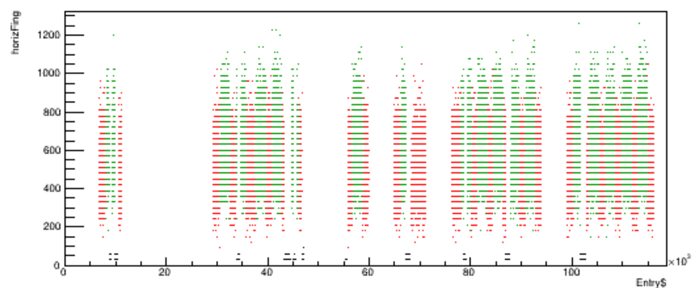
Run 6030 quartetwise, horizFing vs time
