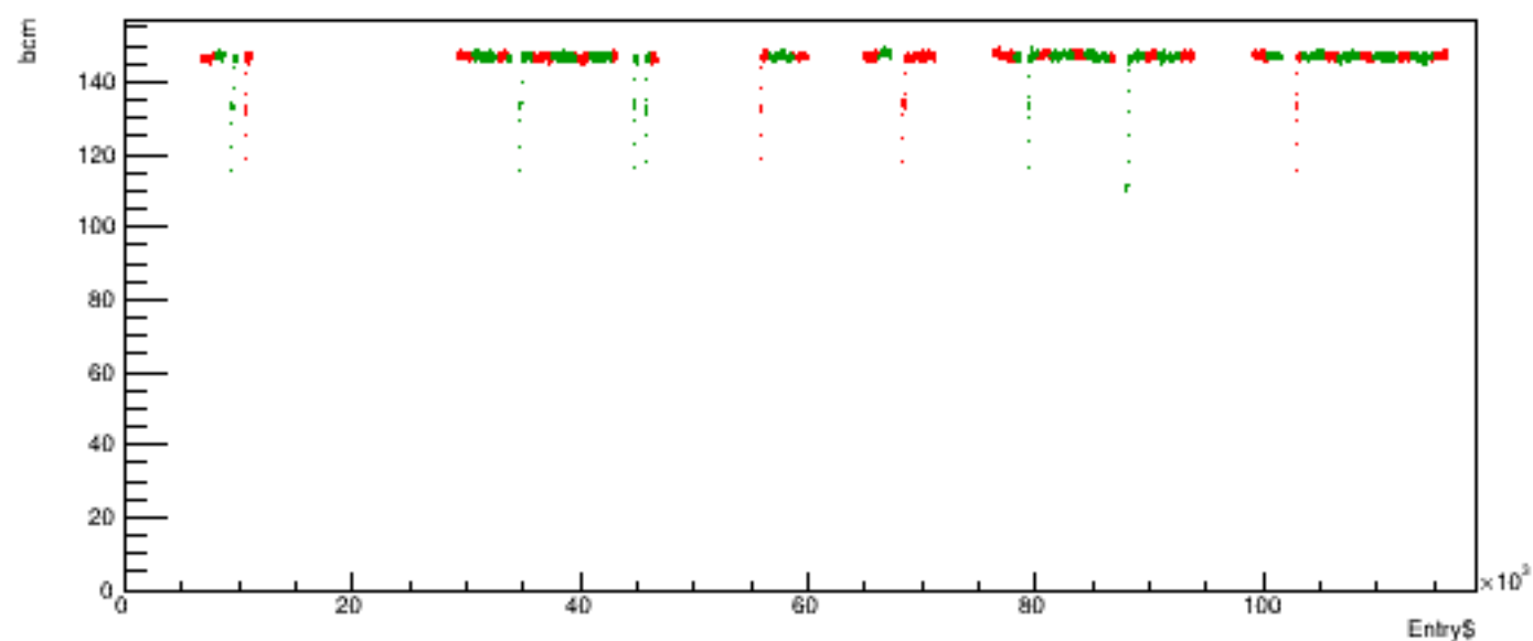
Run 6030 quartetwise, posH4 vs time
