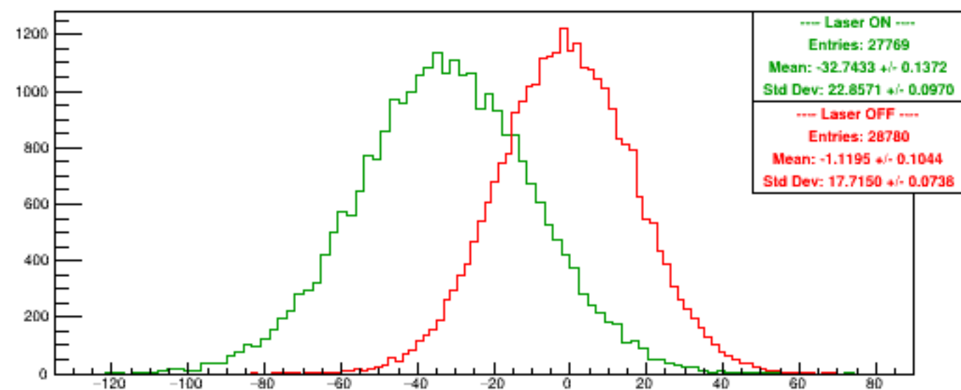
Run 6030 quartetwise, Asyms0
