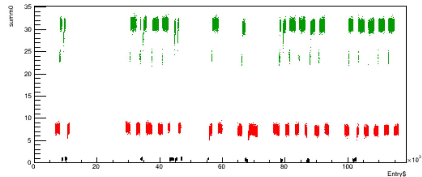
Run 6030 quartetwise, summ0 vs time
