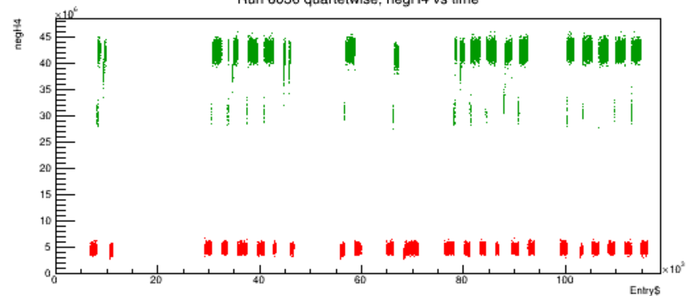
Run 6030 quartetwise, negH4 vs time
