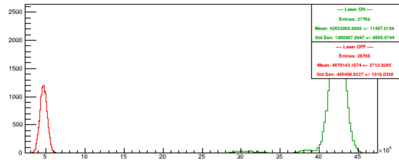
Run 6030 quartetwise, NegHelAcc4
