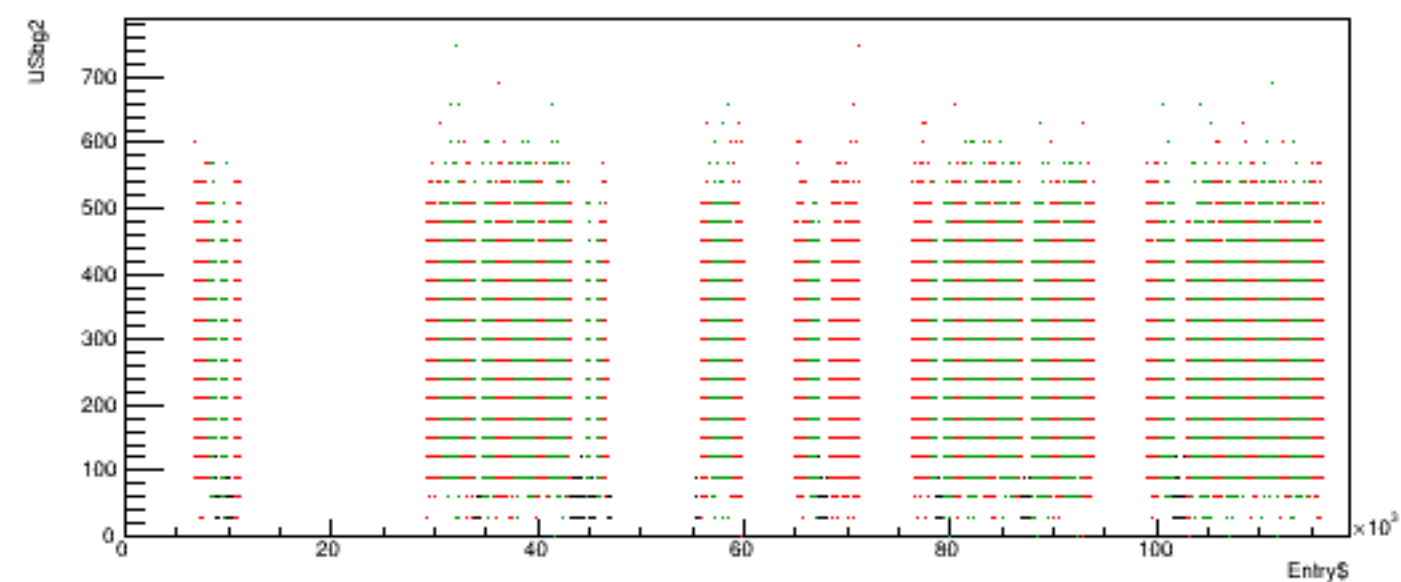
Run 6030 quartetwise, USbg2 vs time
