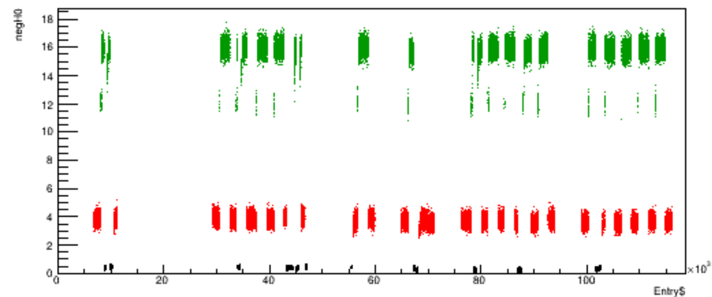
Run 6030 quartetwise, negH0 vs time
