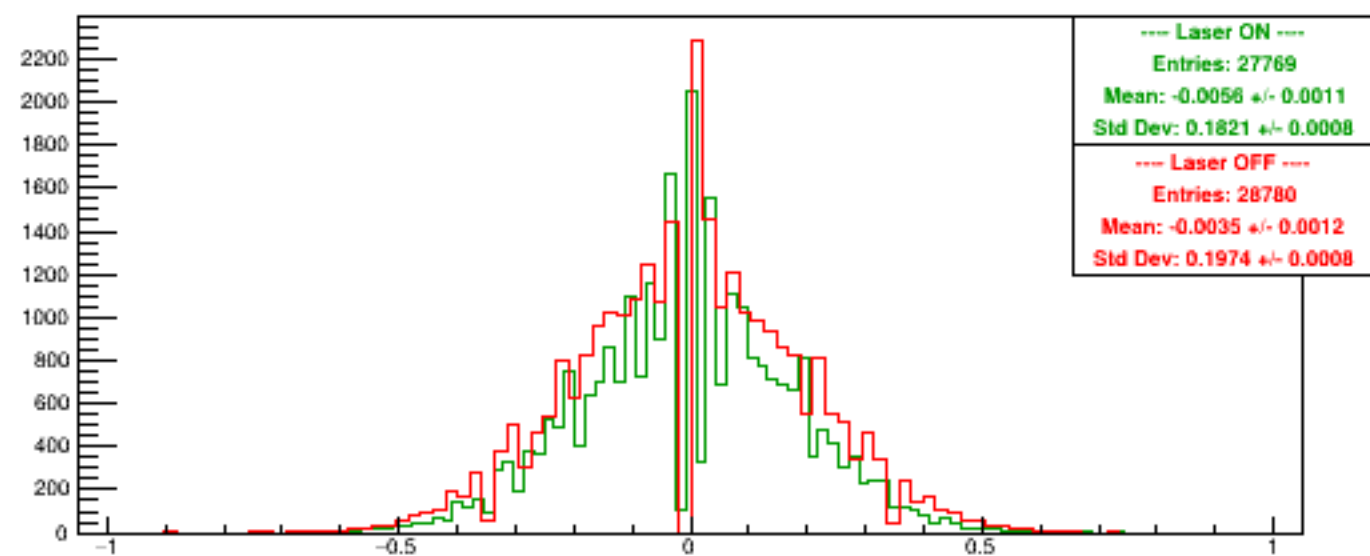
Run 6030 quartetwise, Asyms Horiz Finger
