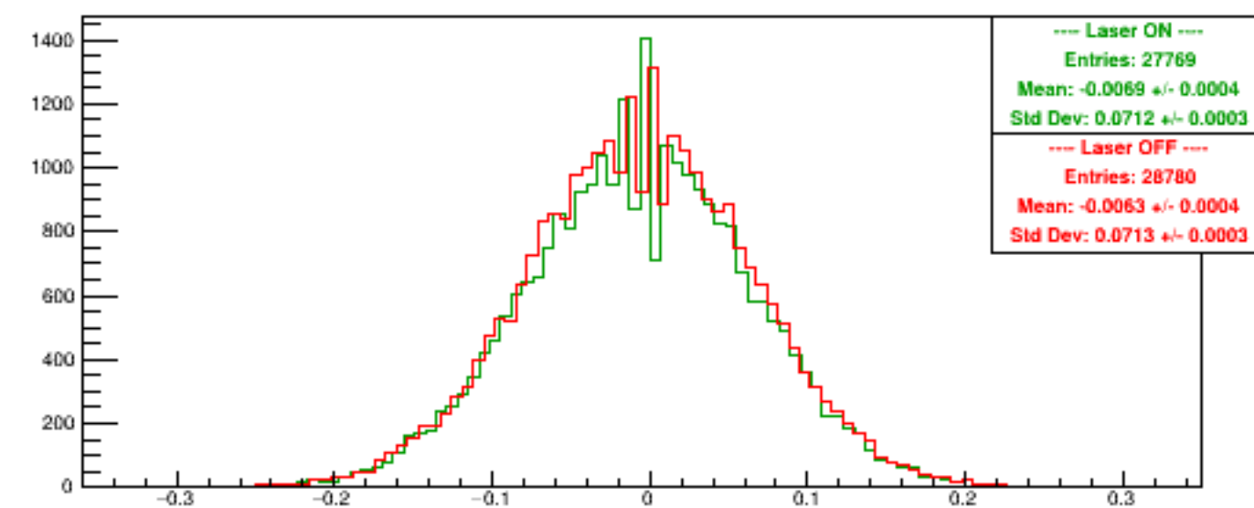
Run 6030 quartetwise, Asyms DSbg2
