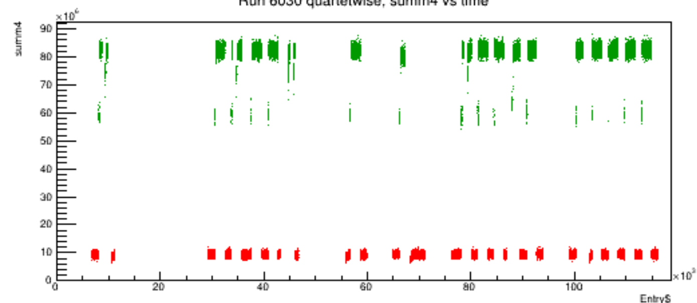
Run 6030 quartetwise, summ4 vs time
