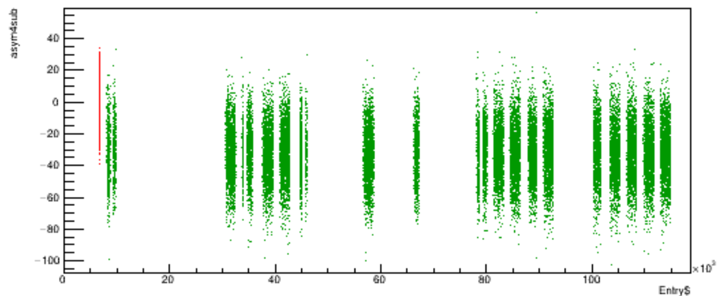
Run 6030 quartetwise, asym4sub vs time
