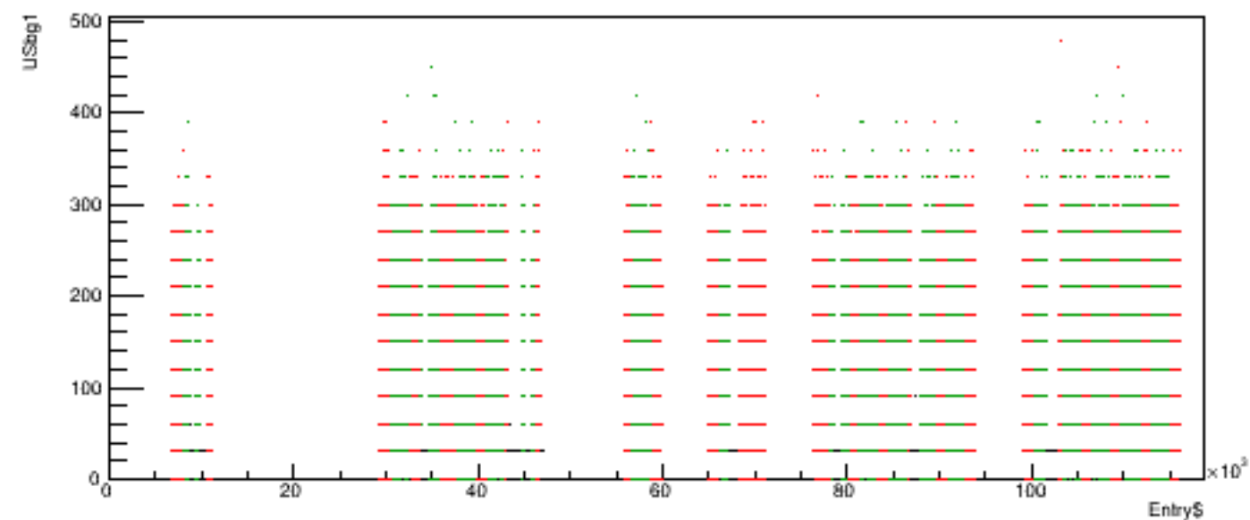
Run 6030 quartetwise, USbg1 vs time
