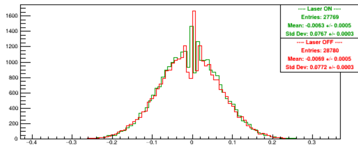
Run 6030 quartetwise, Asyms DSbg1
