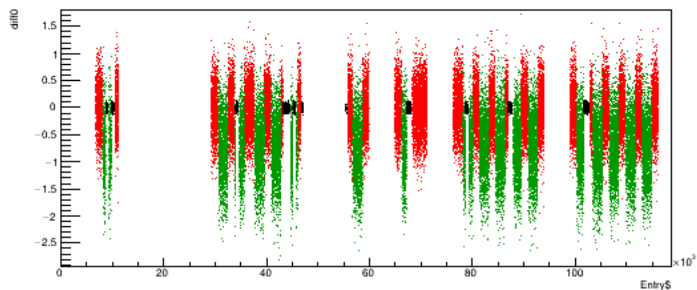
Run 6030 quartetwise, diff0 vs time
