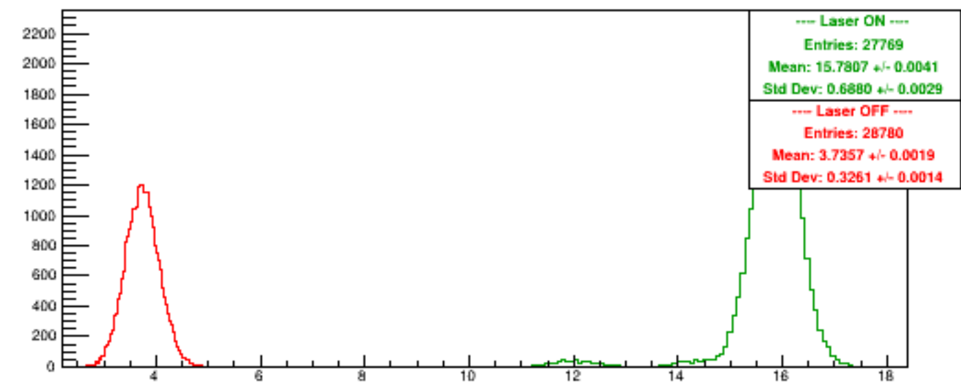
Run 6030 quartetwise, NegHelAcc0/NSamples0
