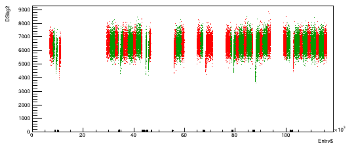
Run 6030 quartetwise, DSbg2 vs time
