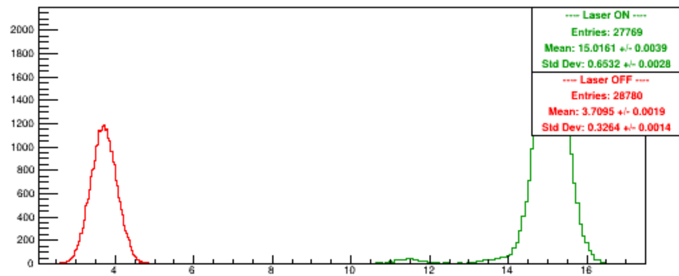
Run 6030 quartetwise, PosHelAcc0/NSamples0
