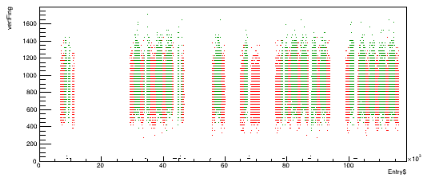
Run 6030 quartetwise, vertFing vs time
