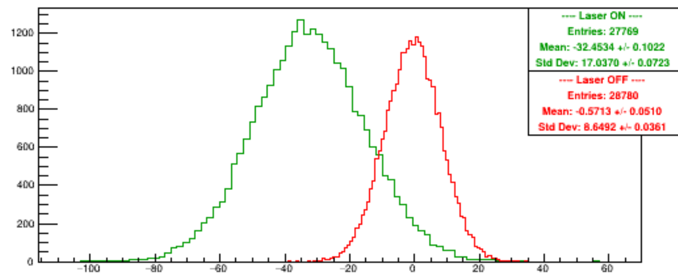
Run 6030 quartetwise, Asyms4
