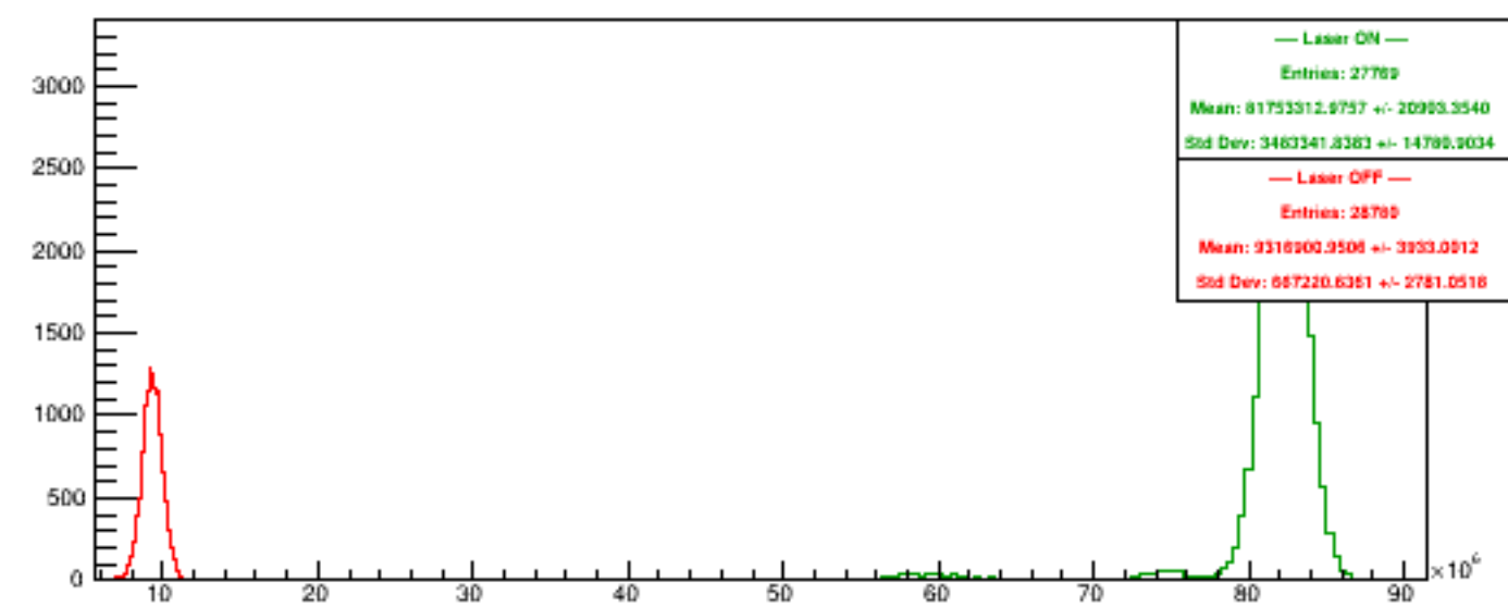
Run 6030 quartetwise, Sums4
