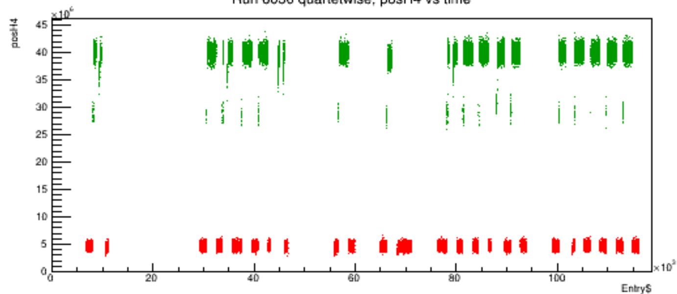
Run 6030 quartetwise, posH4 vs time
