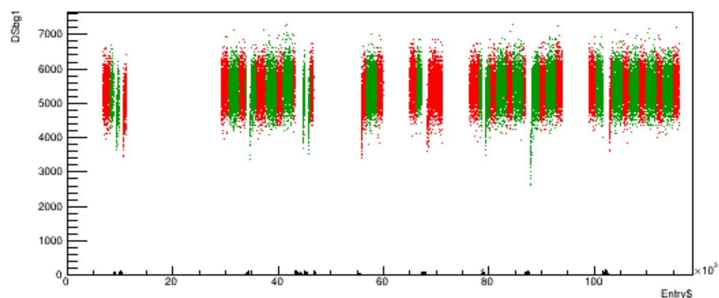
Run 6030 quartetwise, DSbg1 vs time
