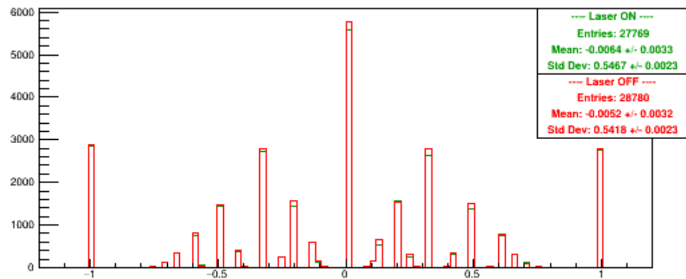
Run 6030 quartetwise, Asyms USbg1
