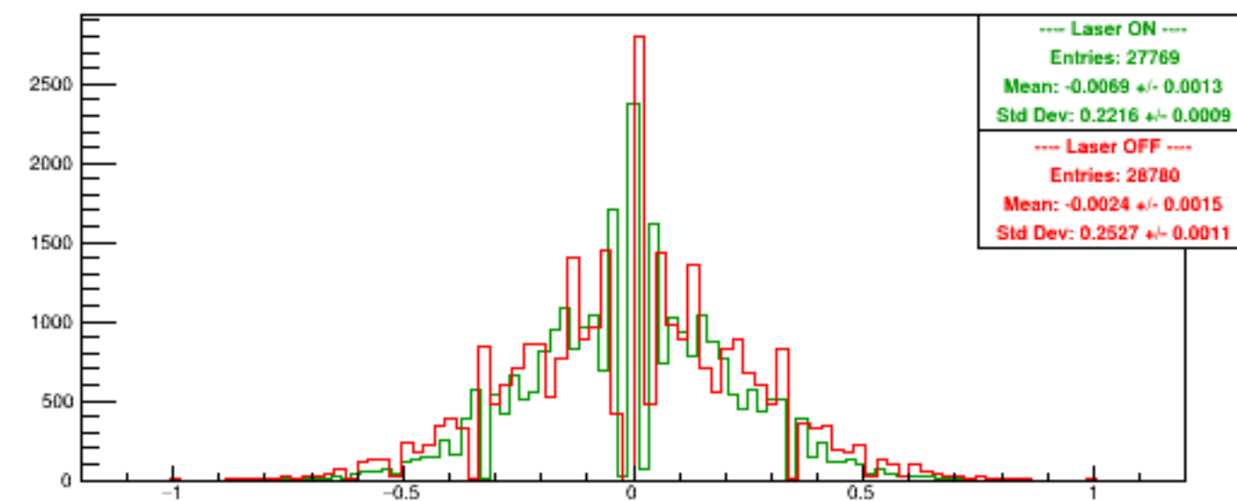
Run 6030 quartetwise, Asyms Vert Finger
