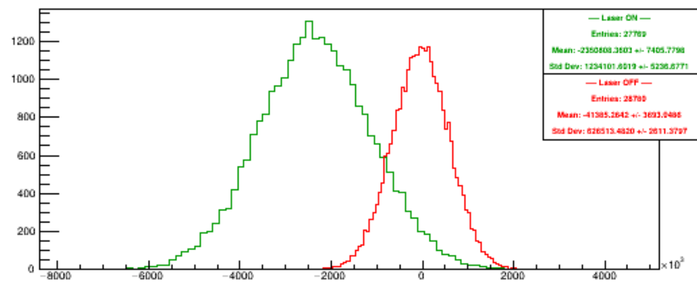
Run 6030 quartetwise, Diffs4
