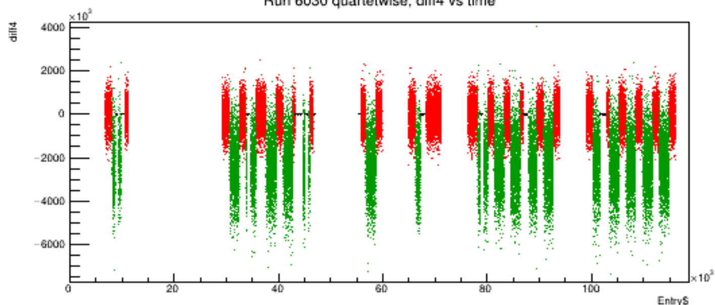
Run 6030 quartetwise, diff4 vs time
