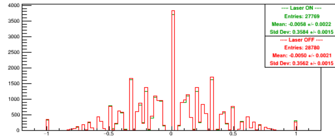
Run 6030 quartetwise, Asyms USbg2
