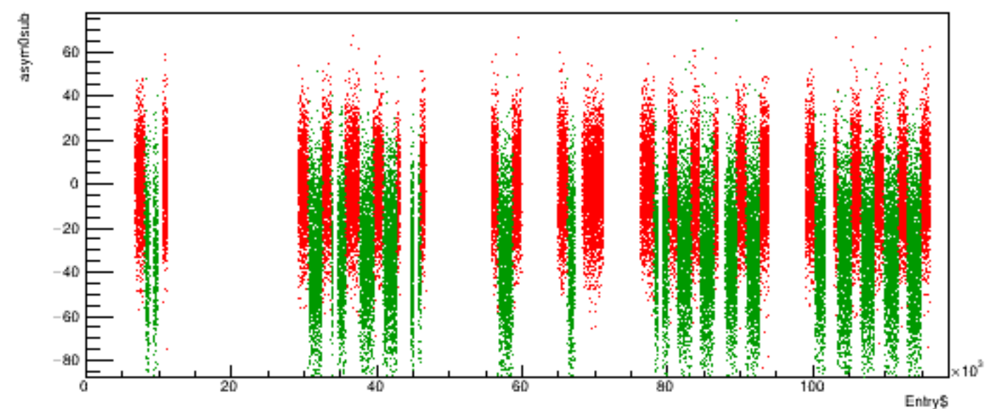
Run 6030 quartetwise, asym0sub vs time
