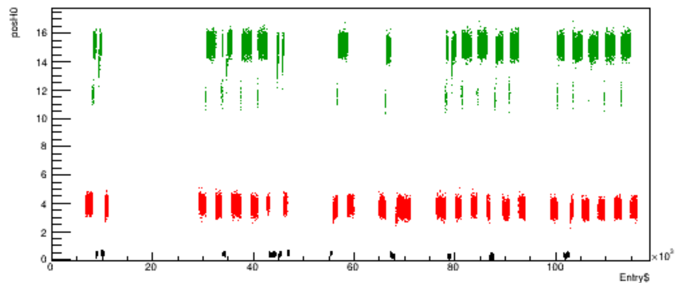
Run 6030 quartetwise, posH0 vs time
