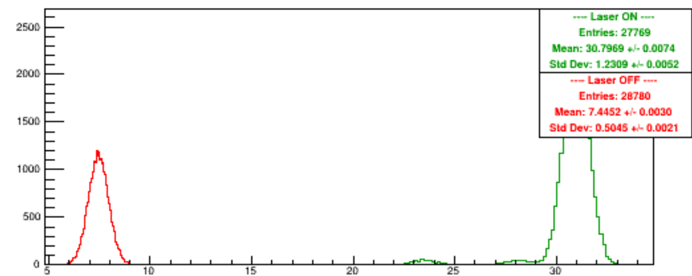
Run 6030 quartetwise, Sums0
