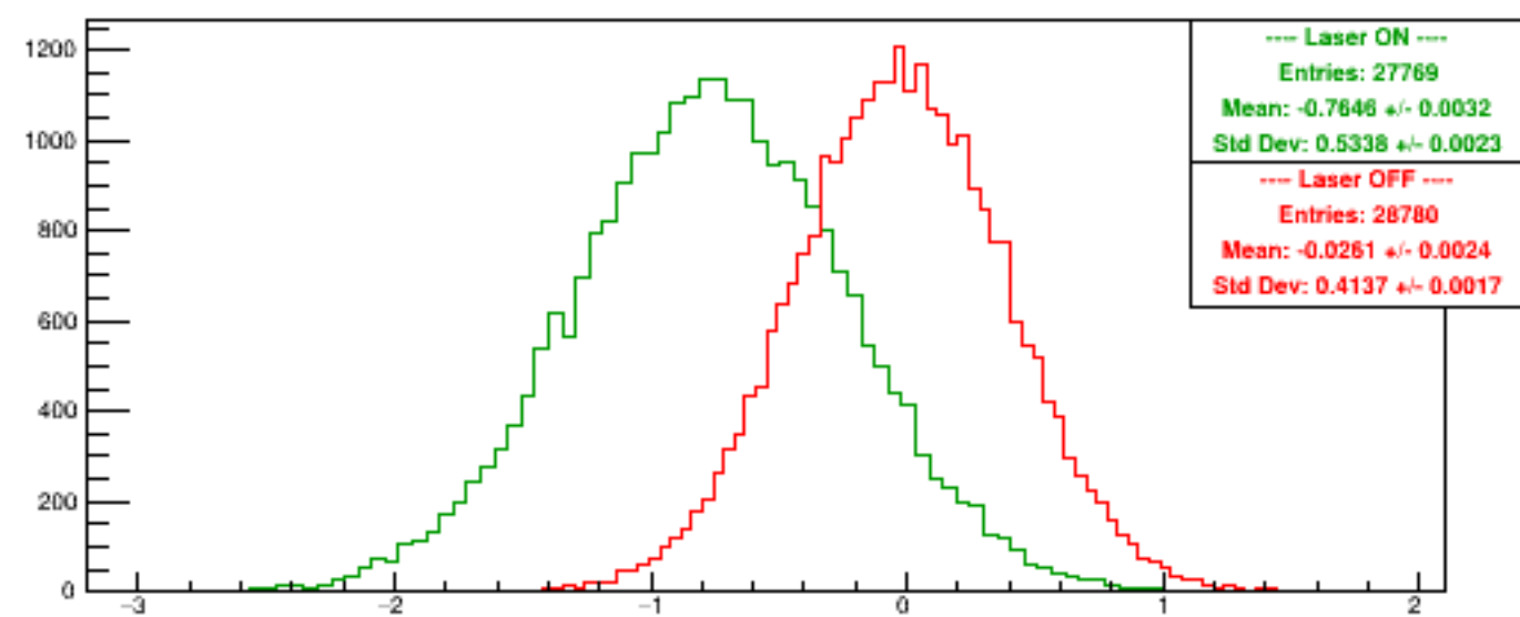
Run 6030 quartetwise, Diffs0
