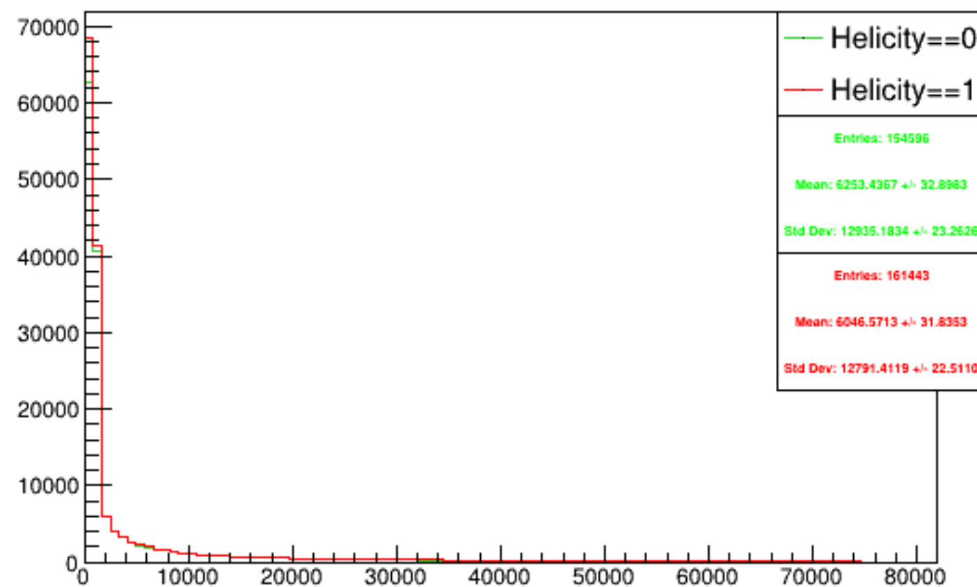
Run 6031 triggerwise, sums: Beam ON, Laser OFF
