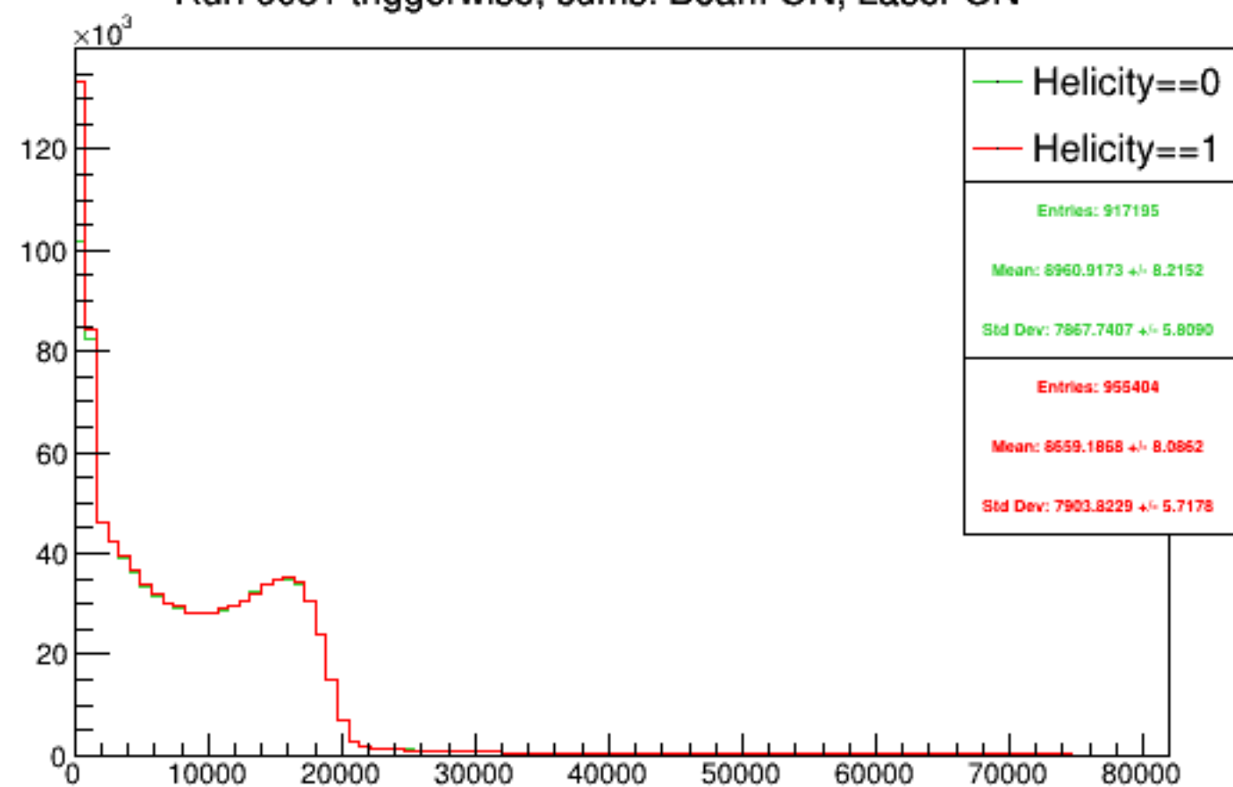
Run 6031 triggerwise, sums: Beam ON, Laser ON
