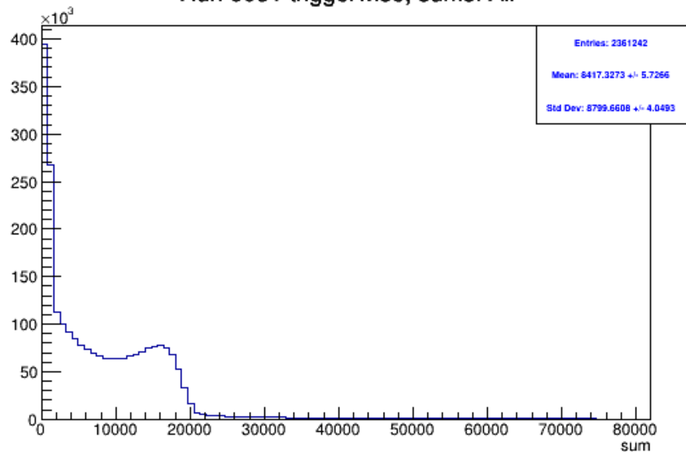
Run 6031 triggerwise, sums: All
