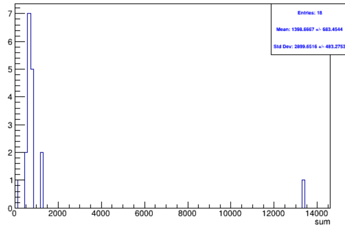
Run 6031 triggerwise, sums: Beam OFF
