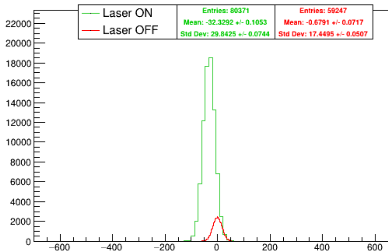
Run 6033 quartetwise, asym0sub: Beam ON
