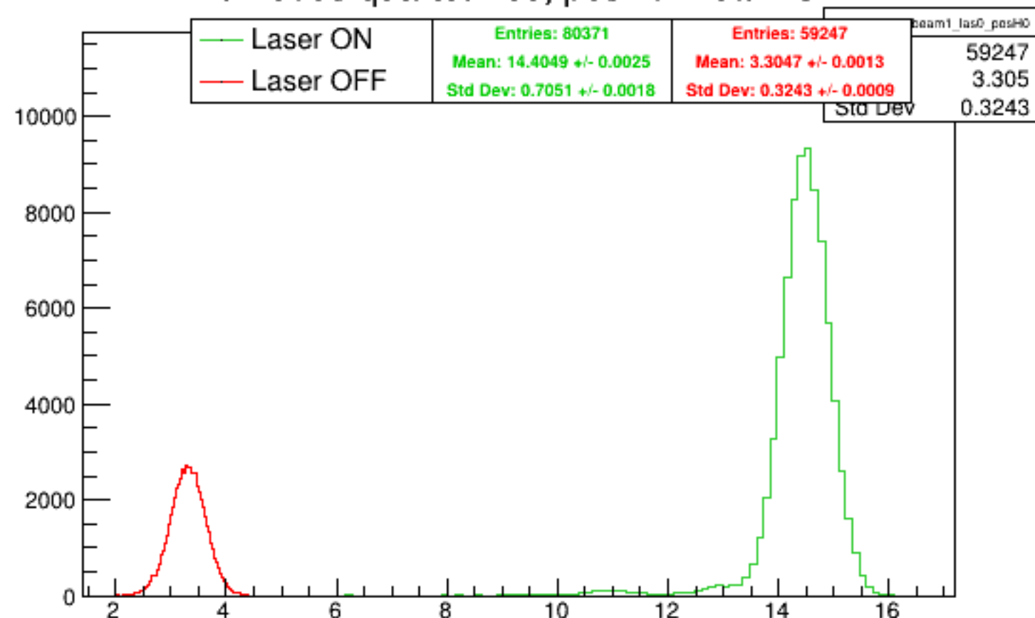
Run 6033 quartetwise, posH0: Beam ON
