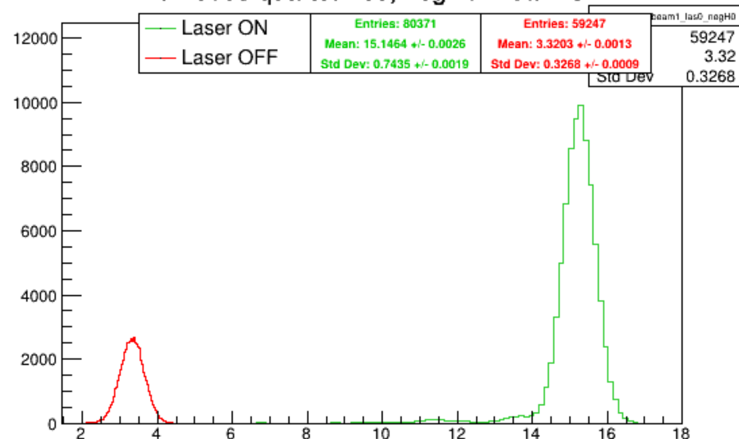
Run 6033 quartetwise, negH0: Beam ON
