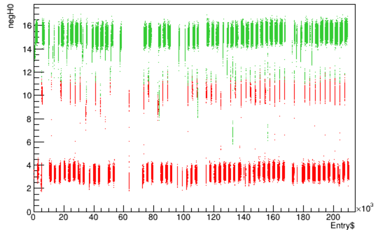
Run 6033 quartetwise, negH0 vs time
