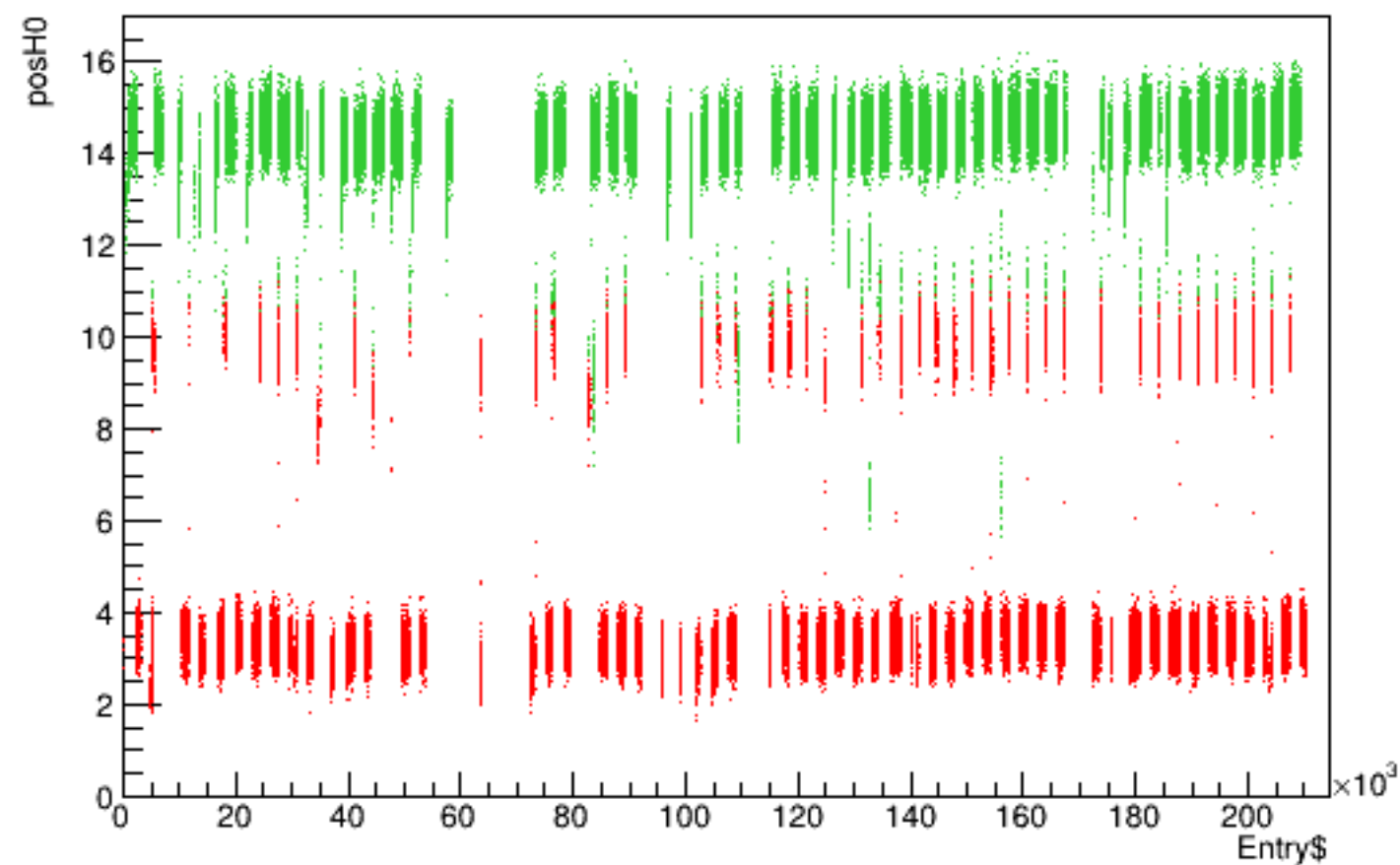
Run 6033 quartetwise, posH0 vs time
