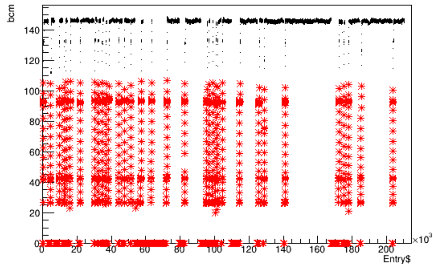
Run 6033 quartetwise, bcm vs time
