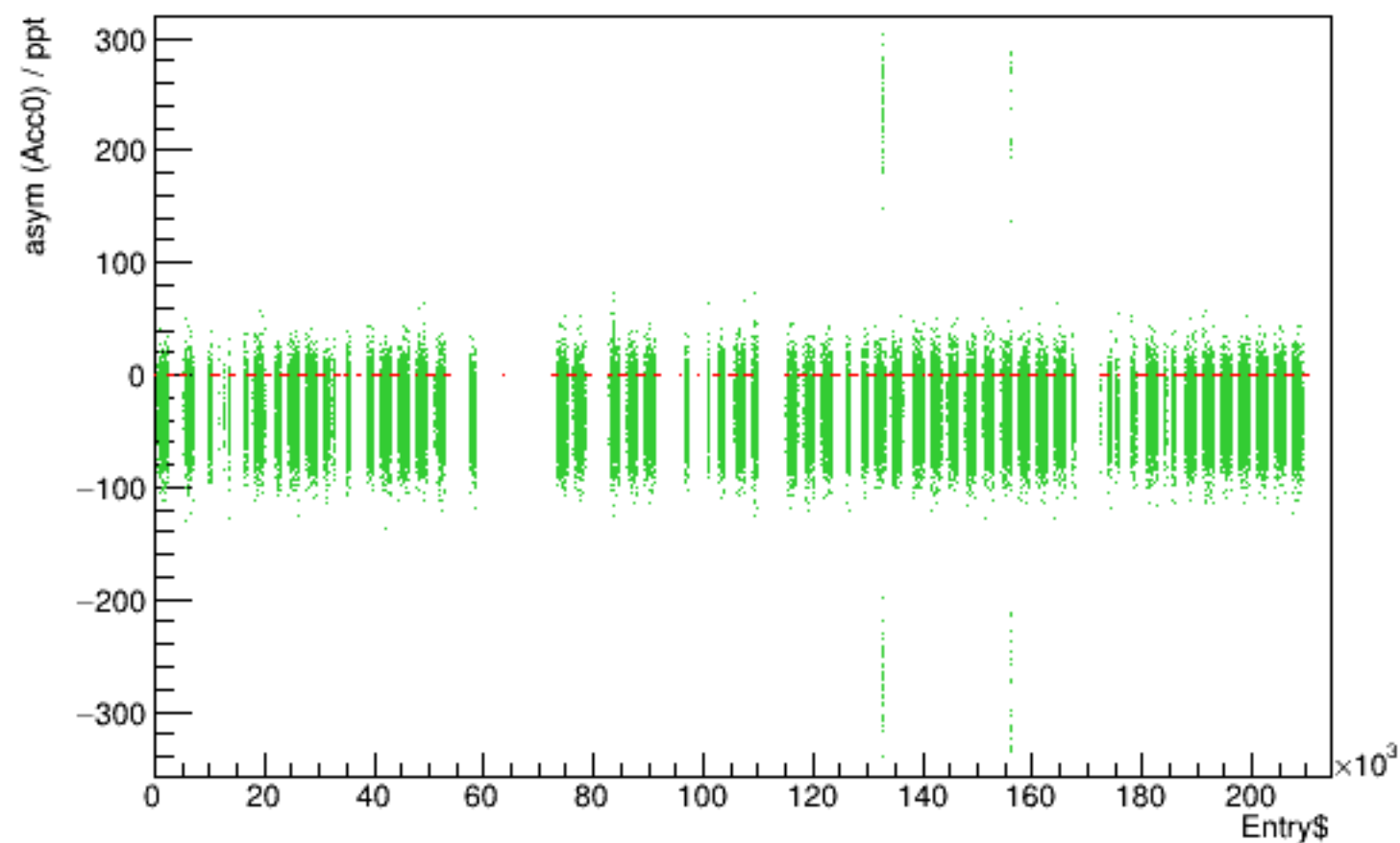
Run 6033 quartetwise, asym0sub vs time
