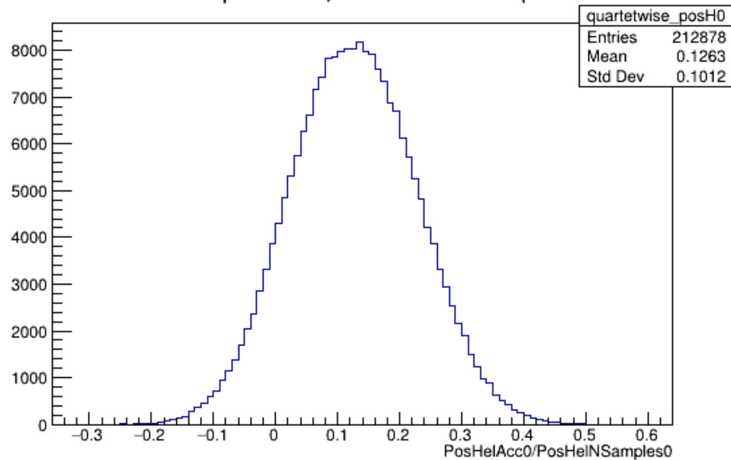
Run 6047 quartetwise, PosHelAcc0/NSamples0: All
