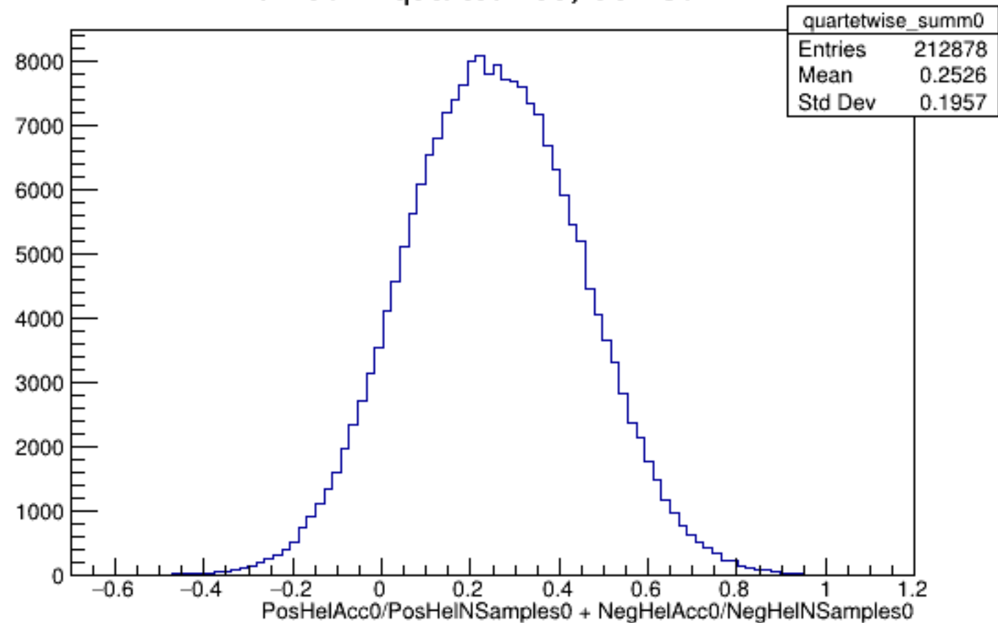
Run 6047 quartetwise, Sums0: All
