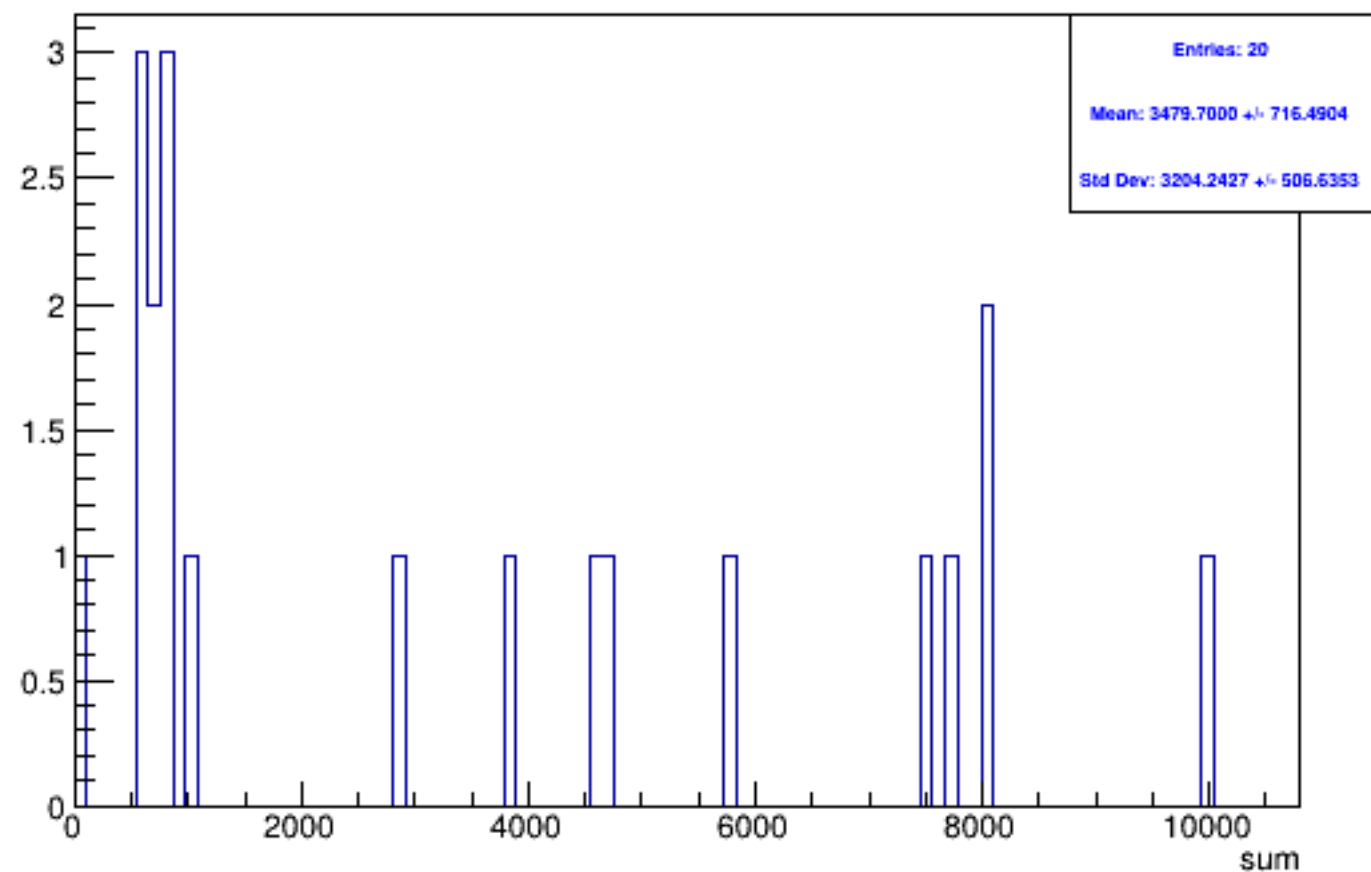
Run 6047 triggerwise, sums: All
