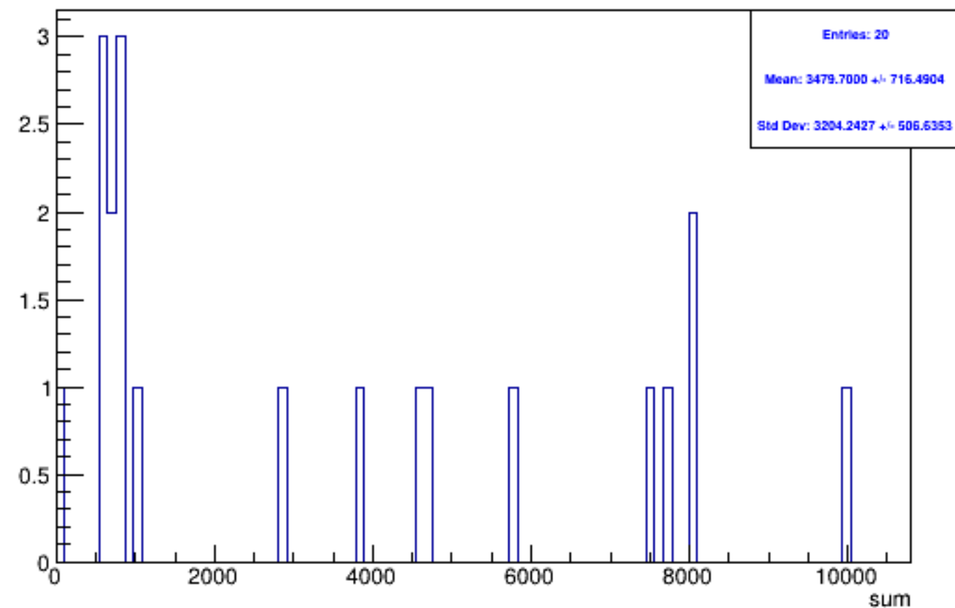
Run 6047 triggerwise, sums: Beam OFF
