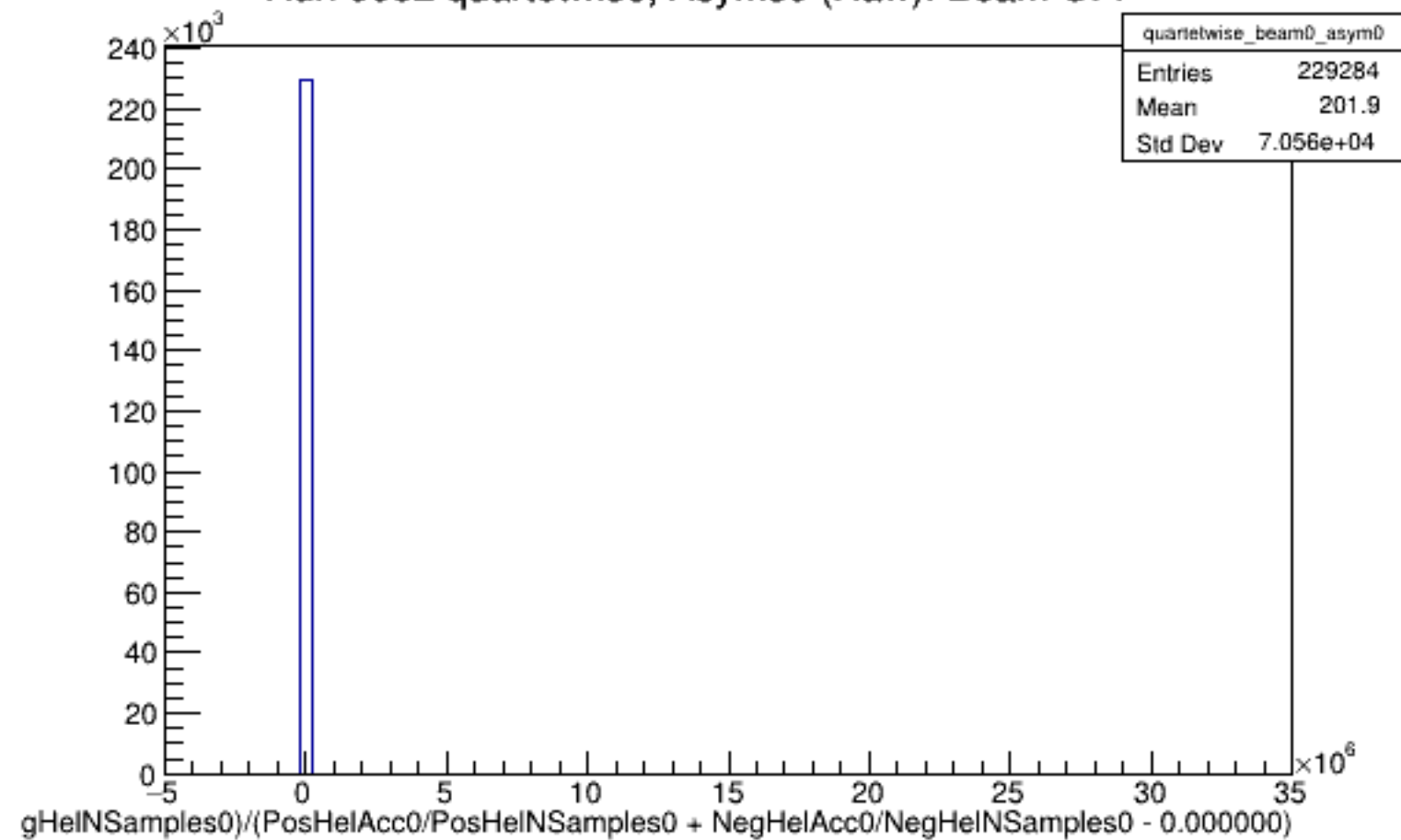
Run 6052 quartetwise, Asyms0 (Raw): Beam OFF
