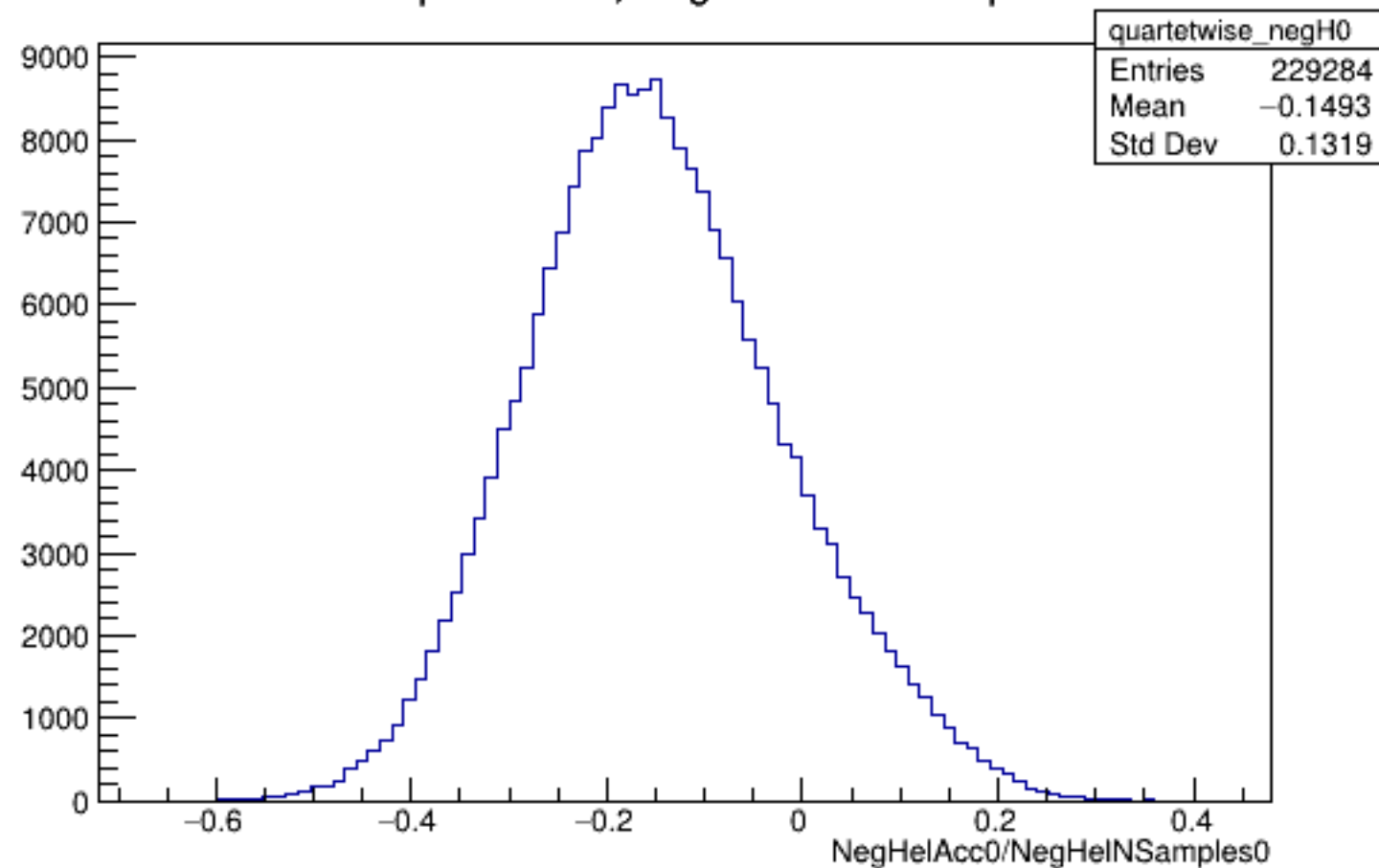
Run 6052 quartetwise, NegHelAcc0/NSamples0: All
