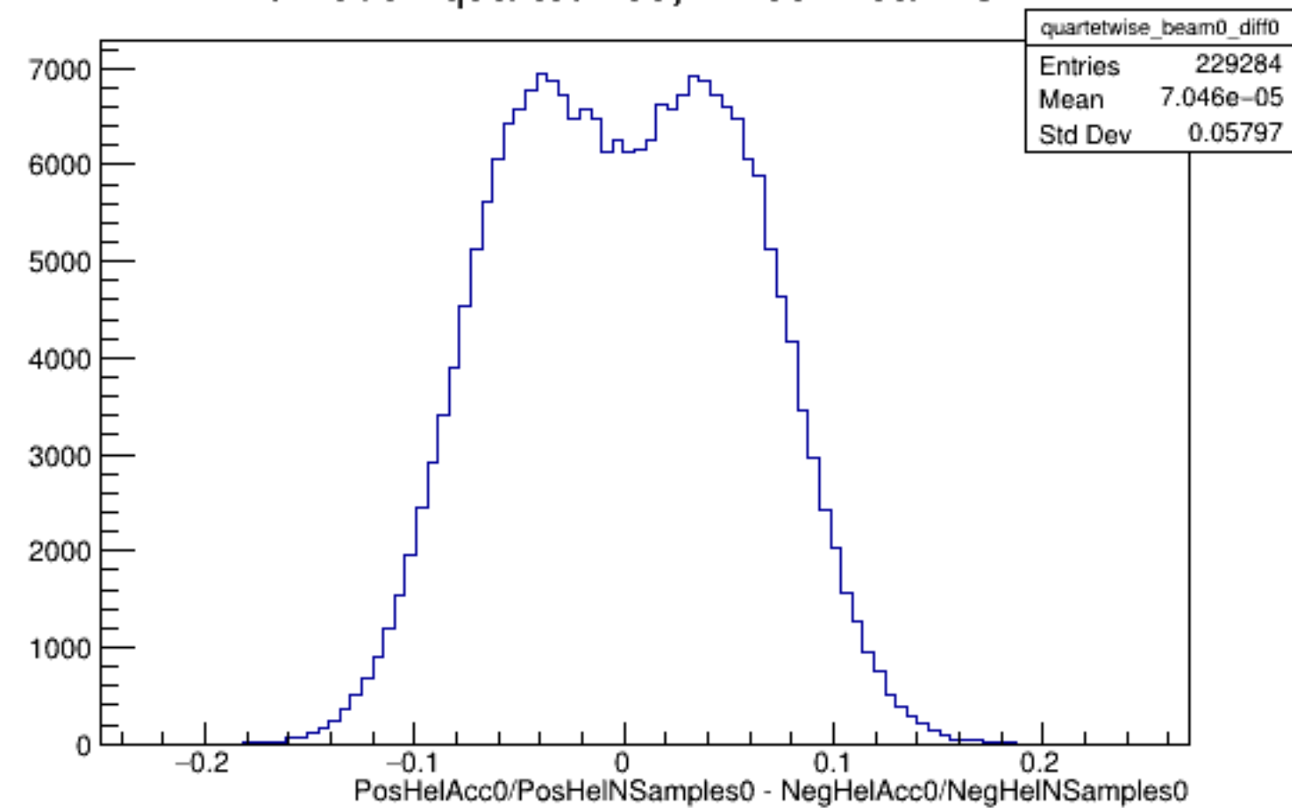
Run 6052 quartetwise, Diffs0: Beam OFF
