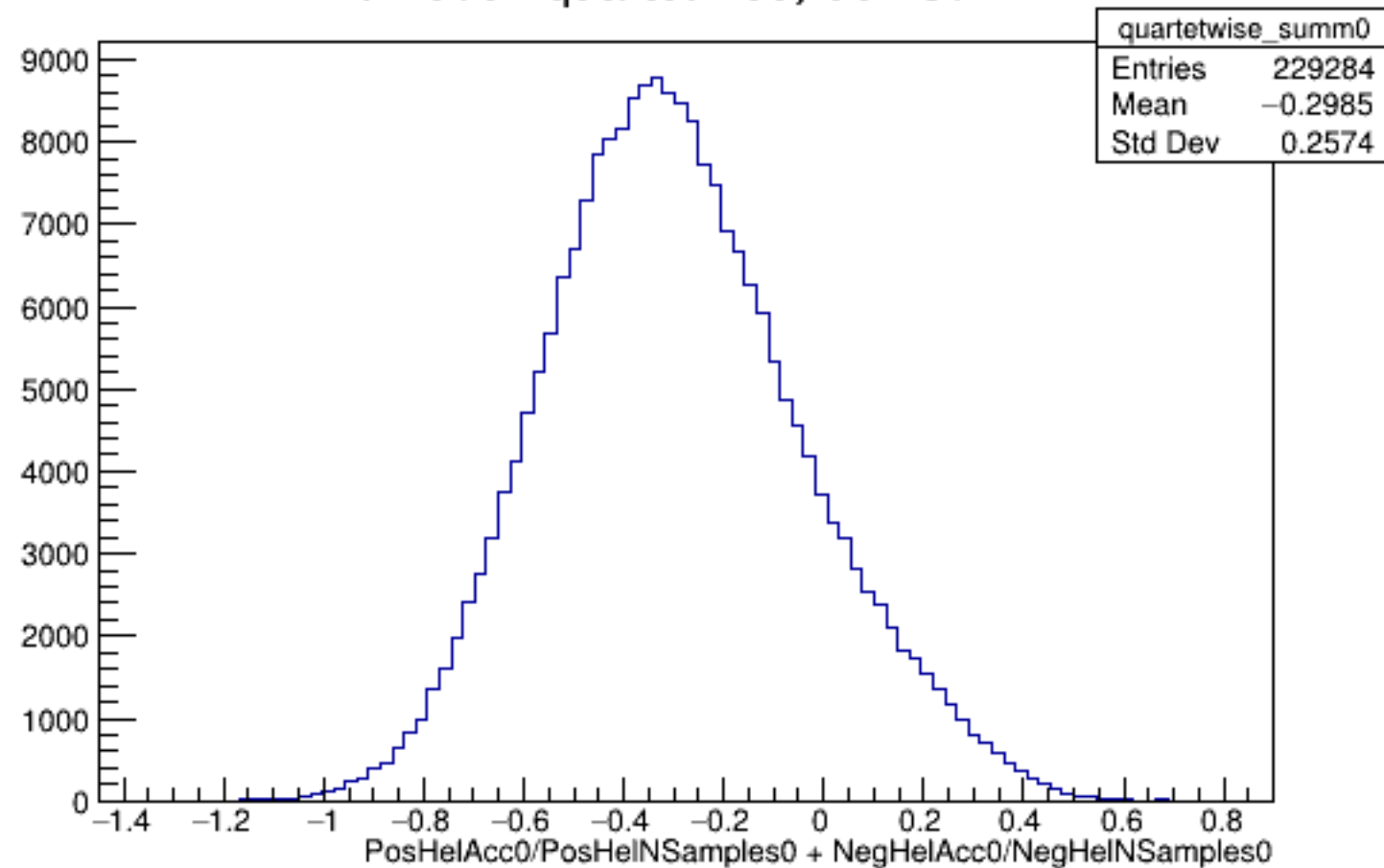
Run 6052 quartetwise, Sums0: All
