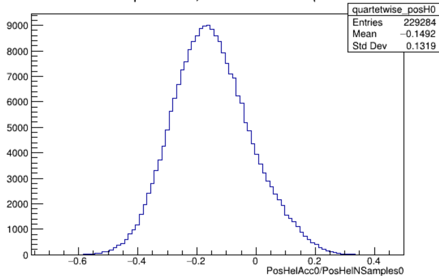
Run 6052 quartetwise, PosHelAcc0/NSamples0: All
