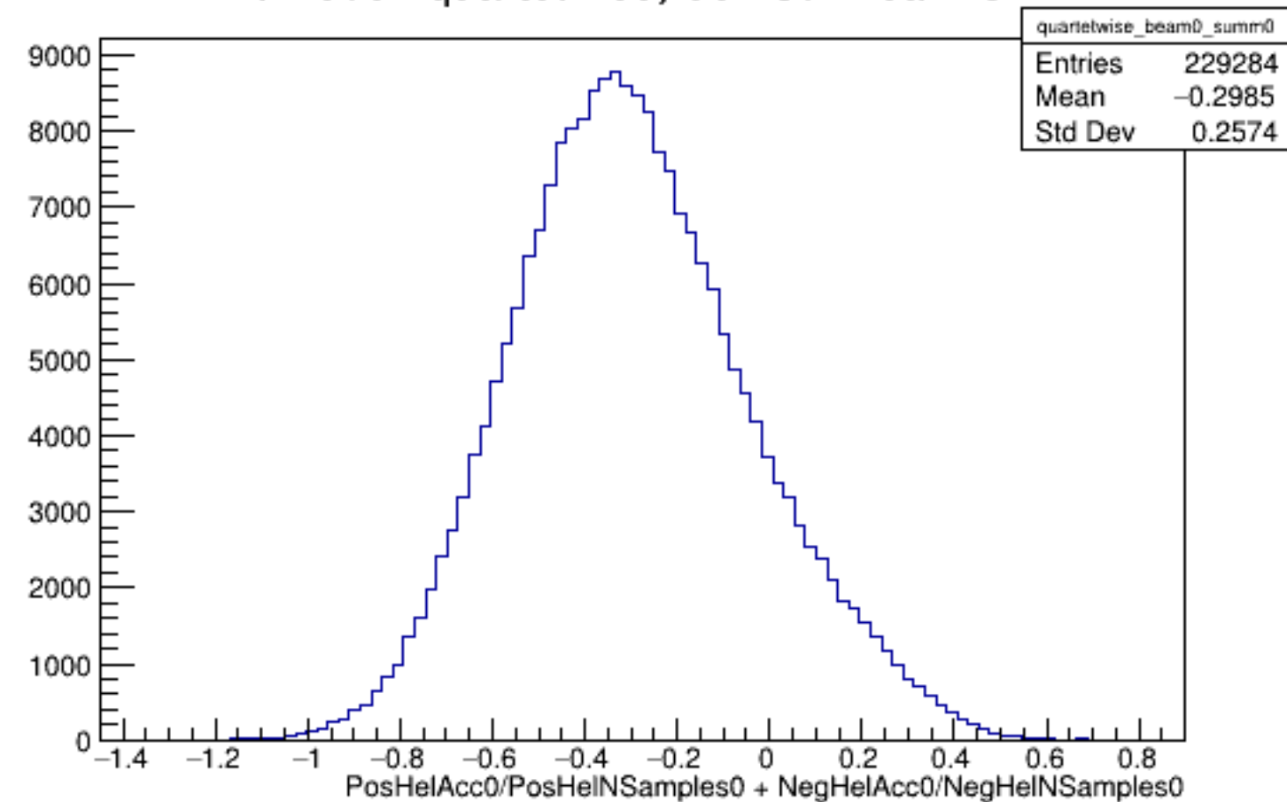
Run 6052 quartetwise, Sums0: Beam OFF
