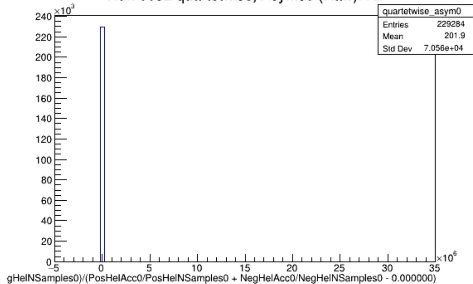
Run 6052 quartetwise, Asyms0 (Raw): All
