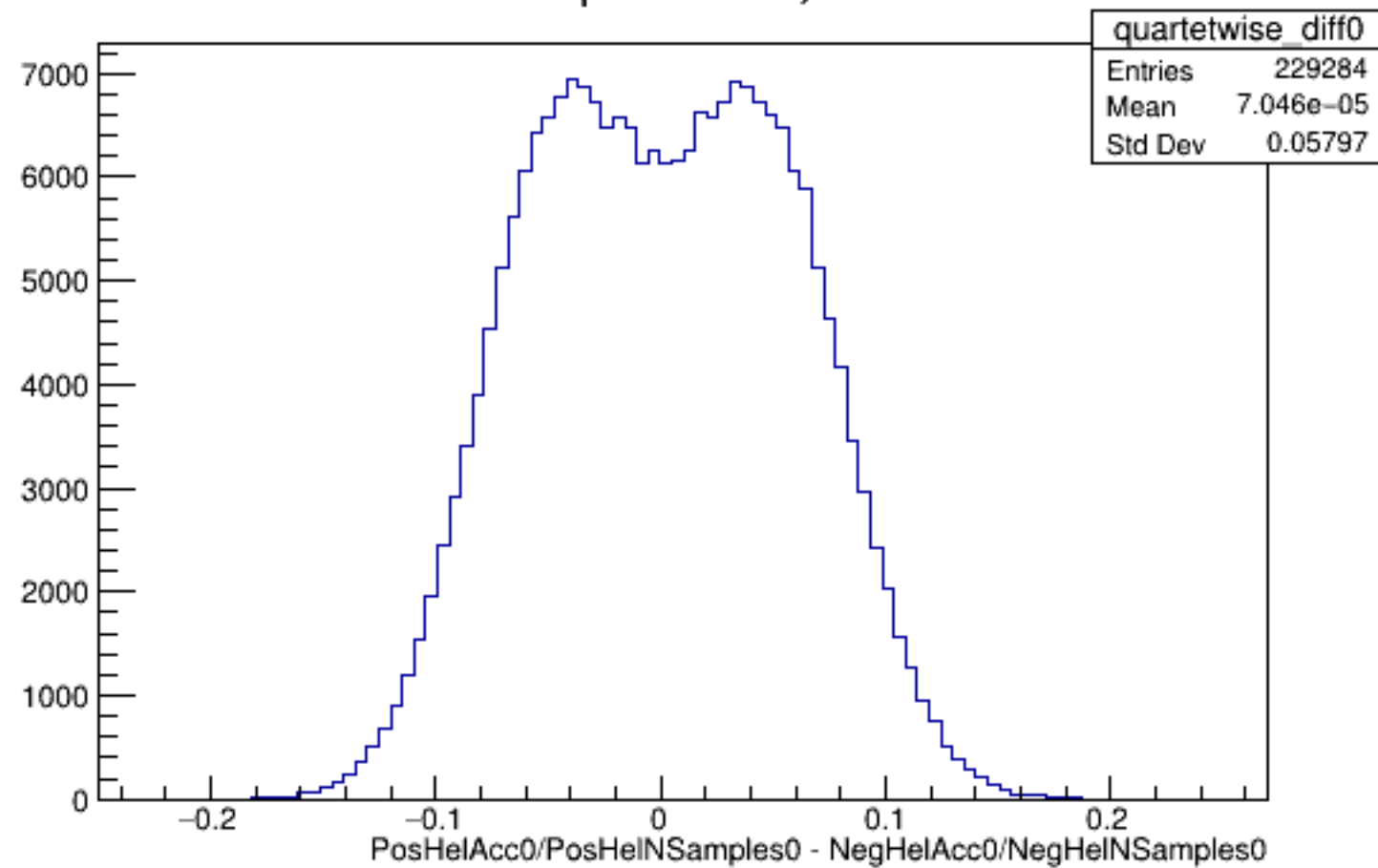
Run 6052 quartetwise, Diffs0: All
