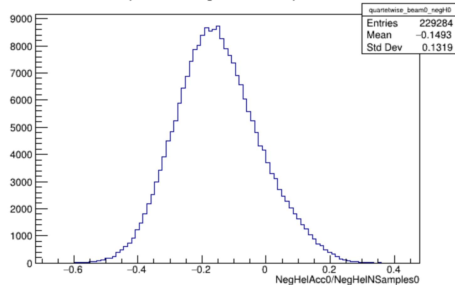
Run 6052 quartetwise, NegHelAcc0/NSamples0: Beam OFF
