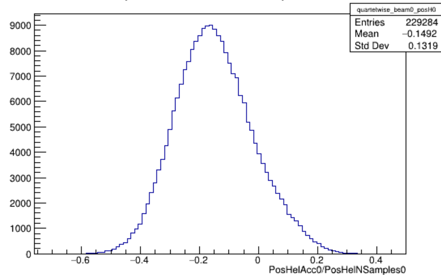
Run 6052 quartetwise, PosHelAcc0/NSamples0: Beam OFF
