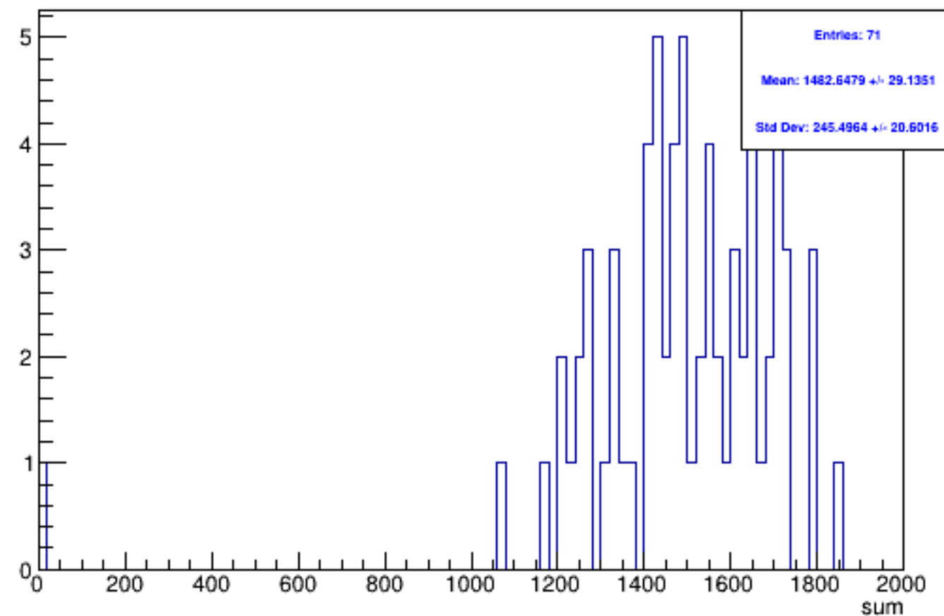
Run 6053 triggerwise, sums: Beam OFF
