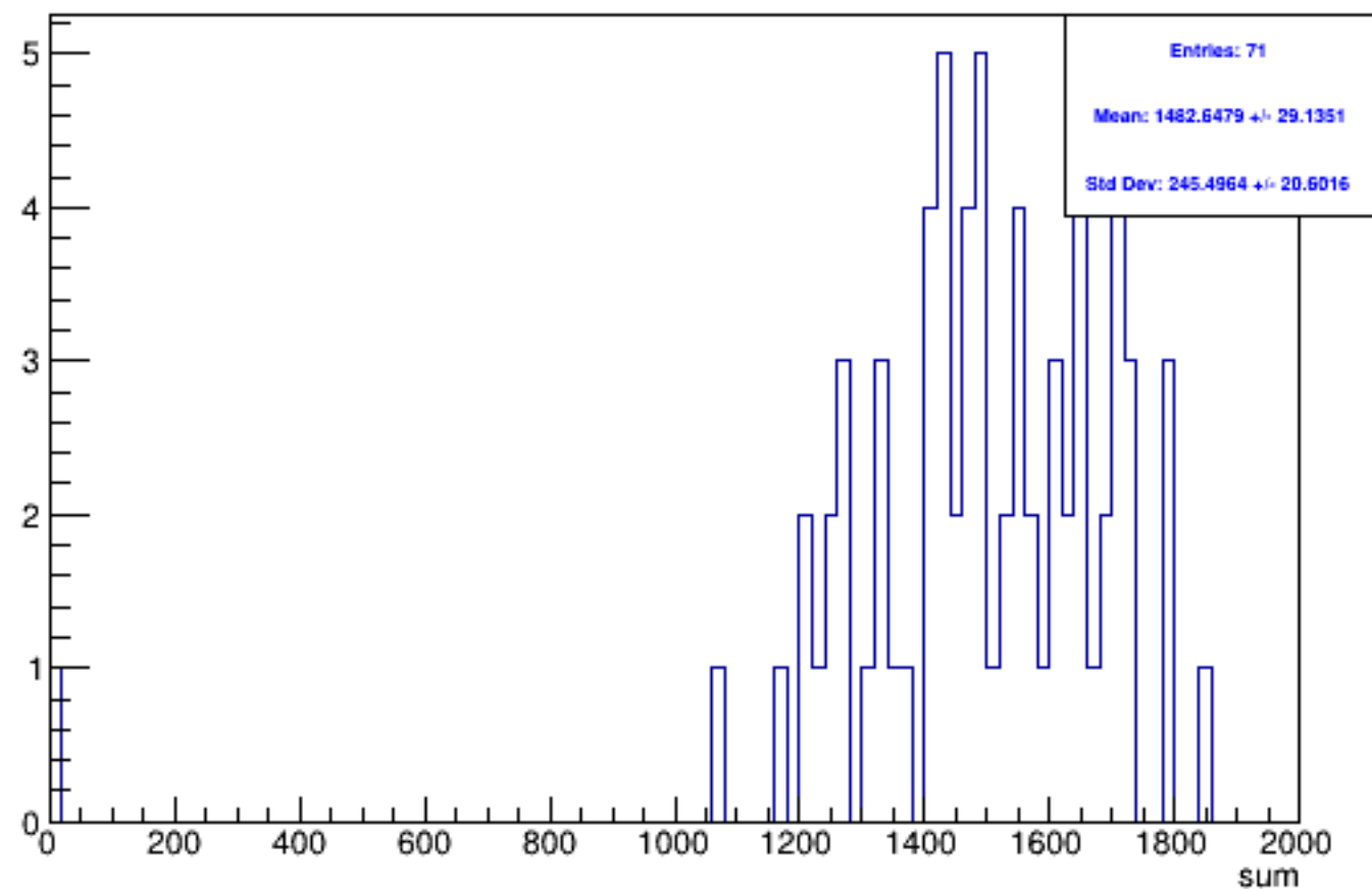
Run 6053 triggerwise, sums: All
