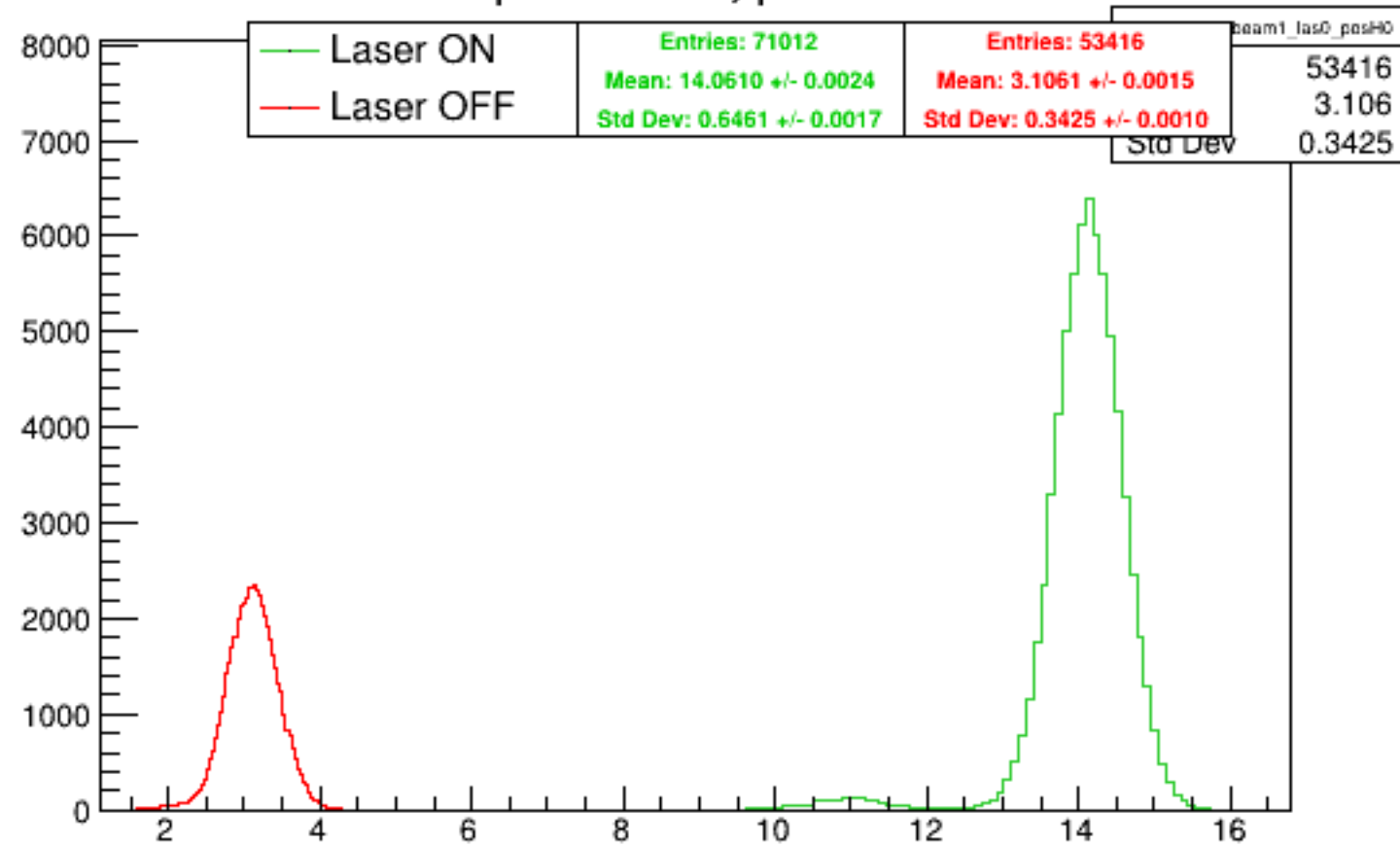
Run 6056 quartetwise, posH0: Beam ON
