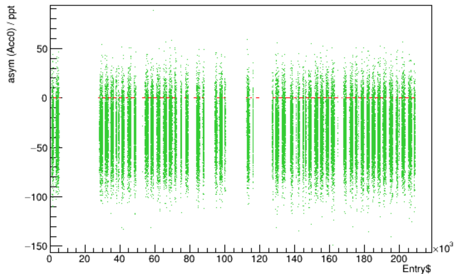
Run 6056 quartetwise, asym0sub vs time
