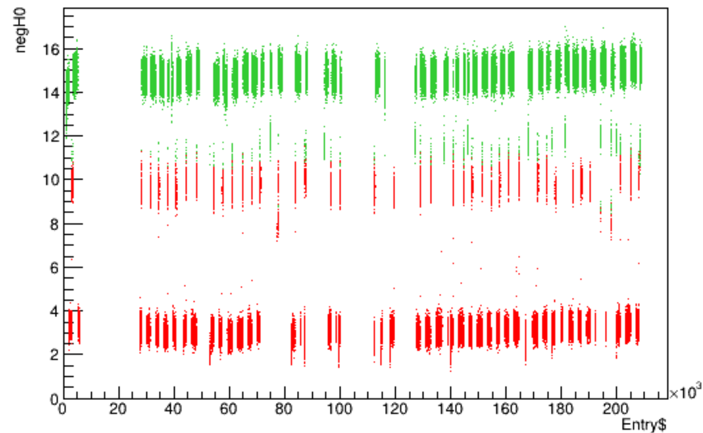
Run 6056 quartetwise, negH0 vs time
