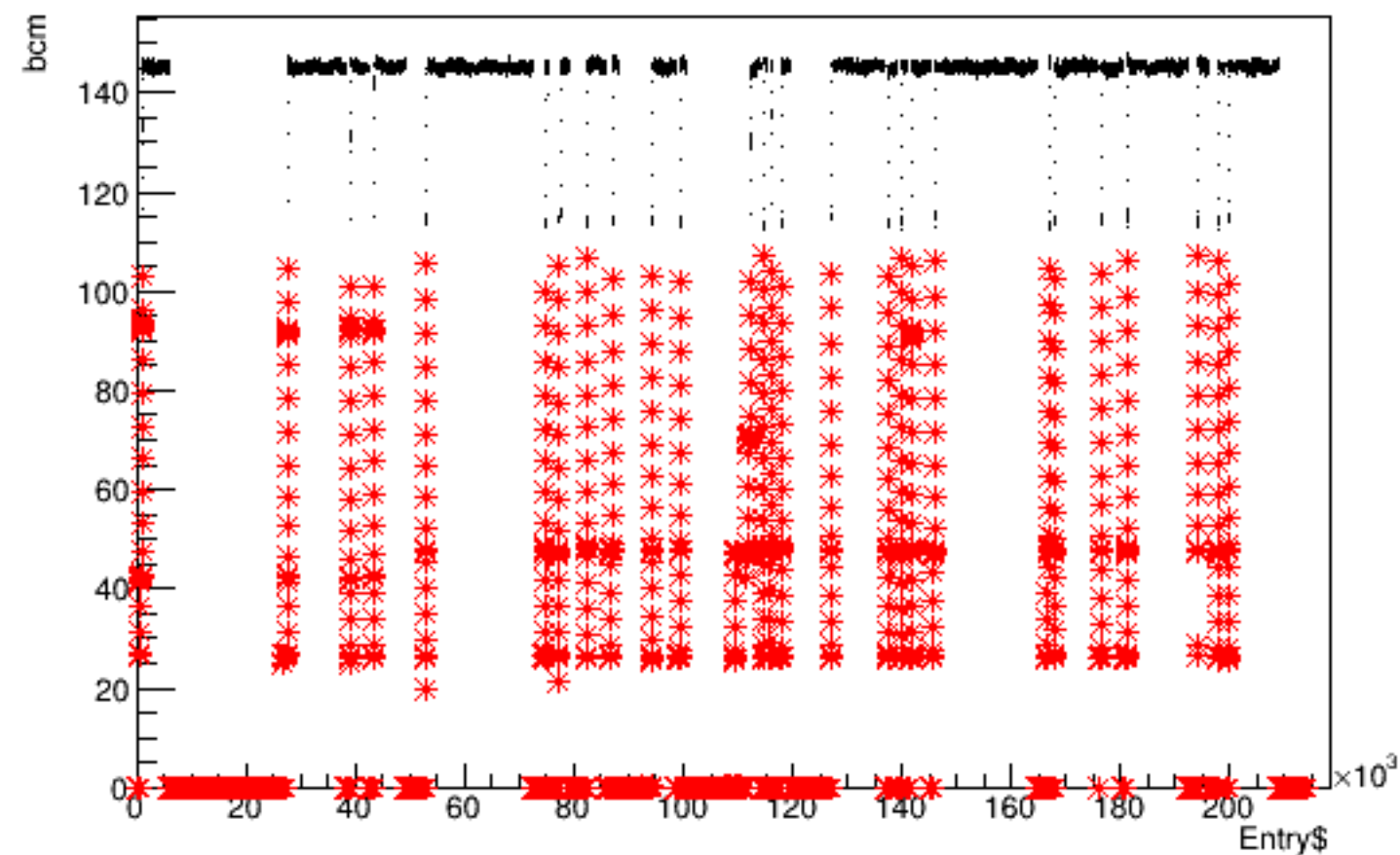
Run 6056 quartetwise, bcm vs time
