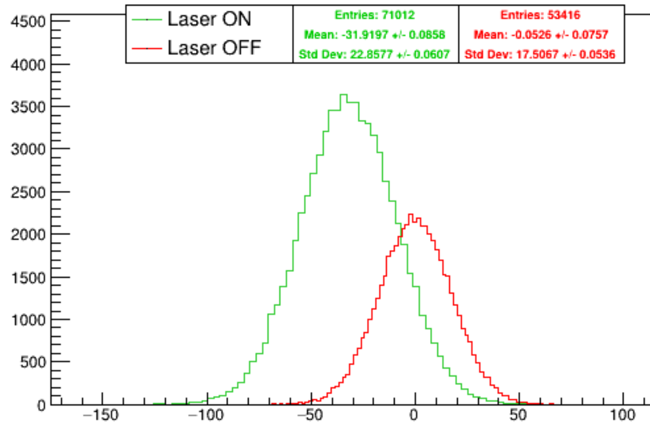
Run 6056 quartetwise, asym0sub: Beam ON
