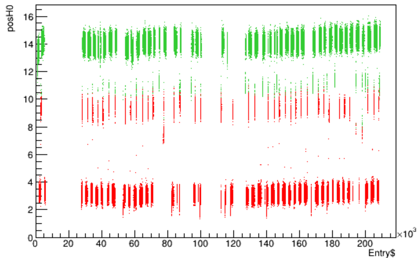
Run 6056 quartetwise, posH0 vs time
