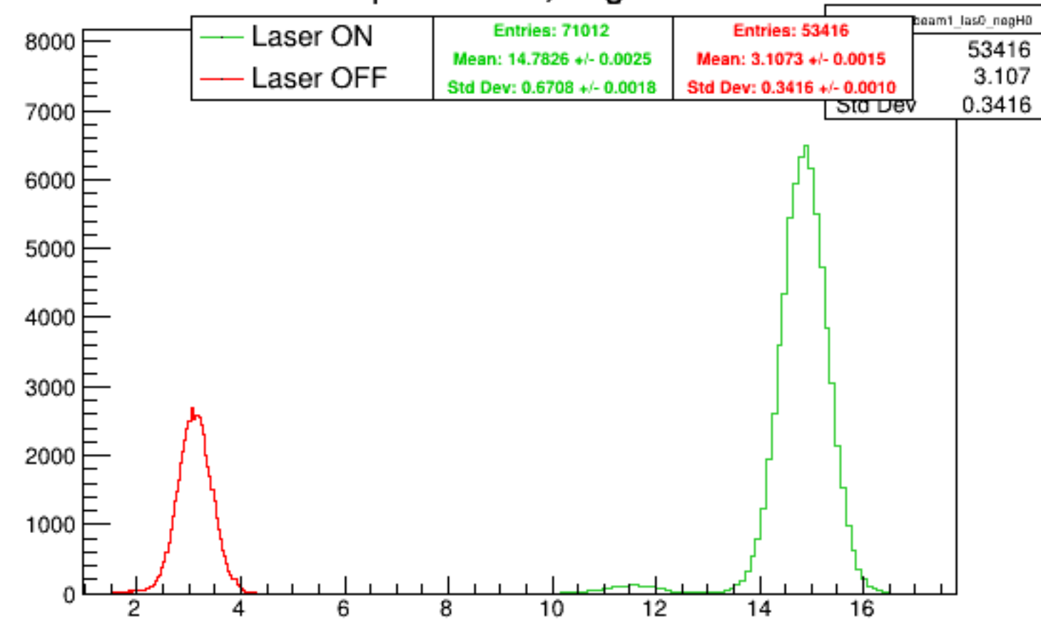
Run 6056 quartetwise, negH0: Beam ON
