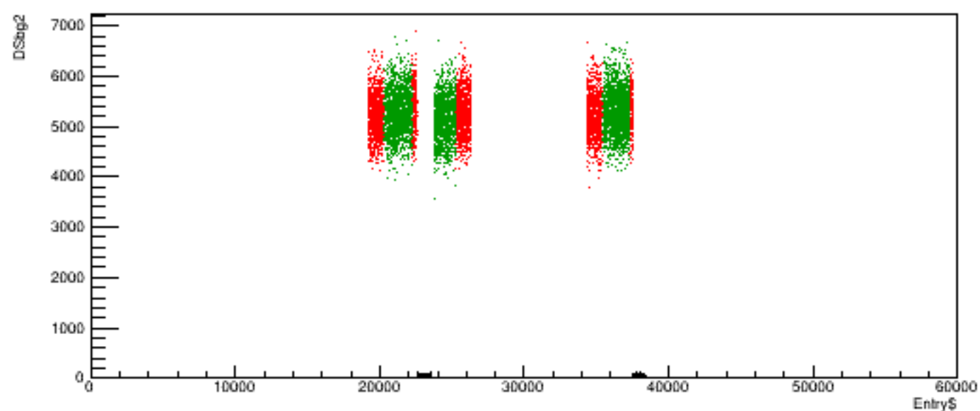
Run 6078 quartetwise, DSbg2 vs time
