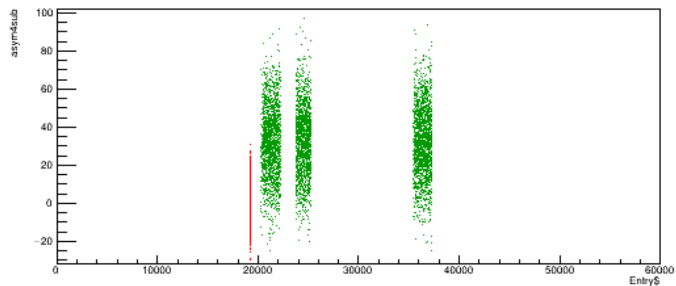
Run 6078 quartetwise, asym4sub vs time
