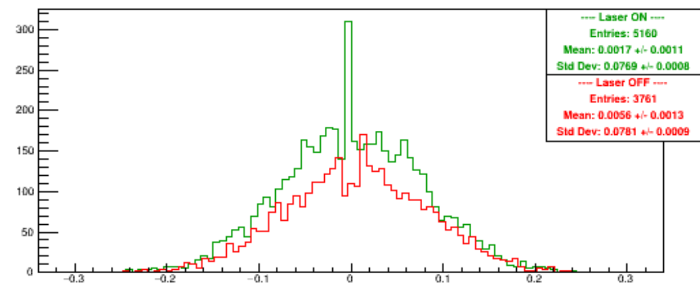
Run 6078 quartetwise, Asyms DSbg2
