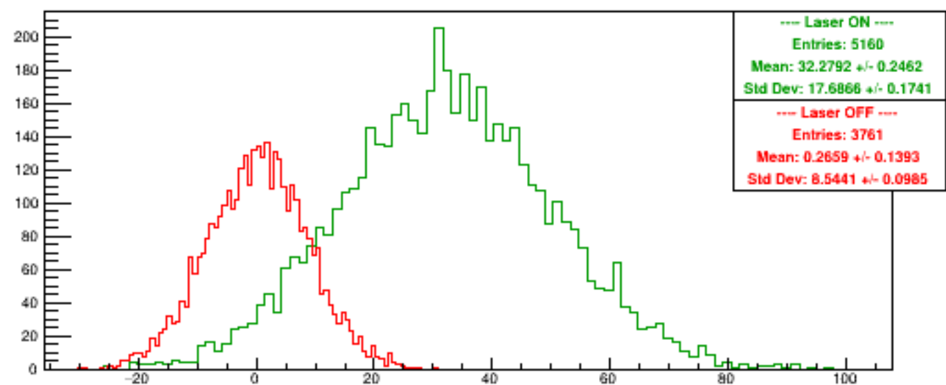
Run 6078 quartetwise, Asyms4
