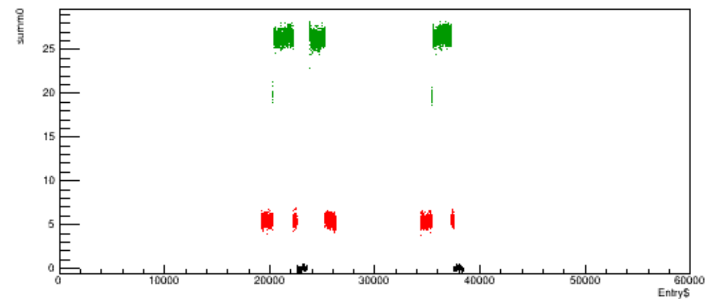
Run 6078 quartetwise, summ0 vs time
