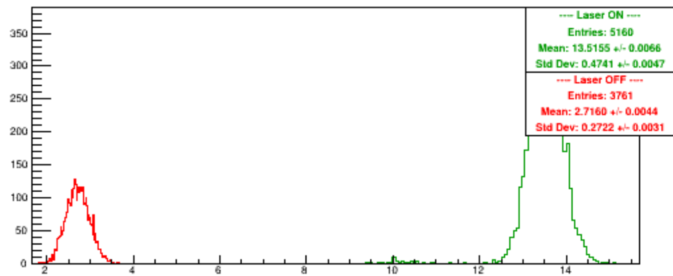
Run 6078 quartetwise, PosHelAcc0/NSamples0
