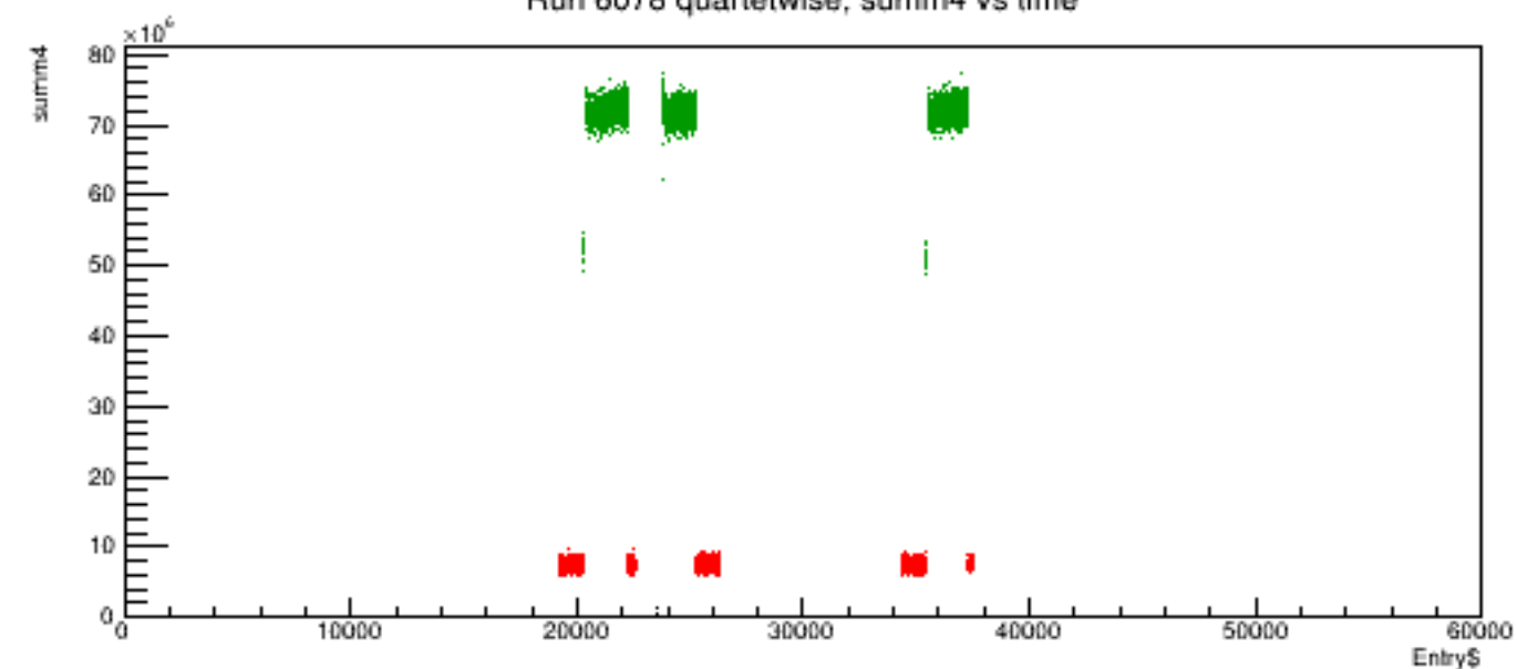
Run 6078 quartetwise, summ4 vs time
