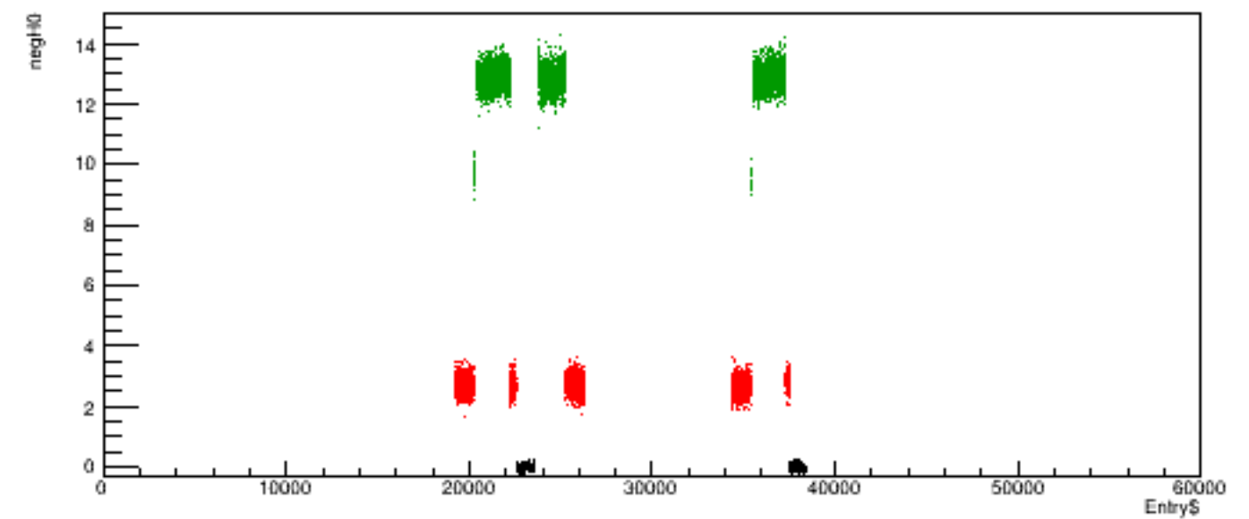
Run 6078 quartetwise, negH0 vs time
