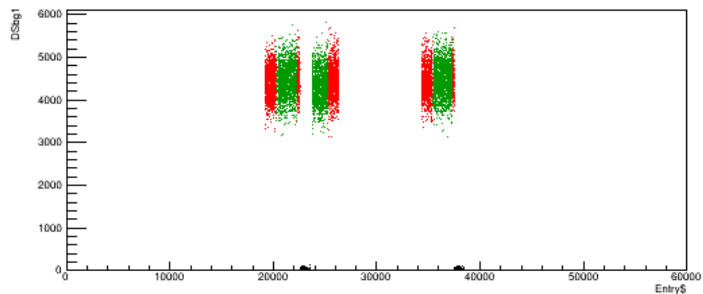
Run 6078 quartetwise, DSbg1 vs time
