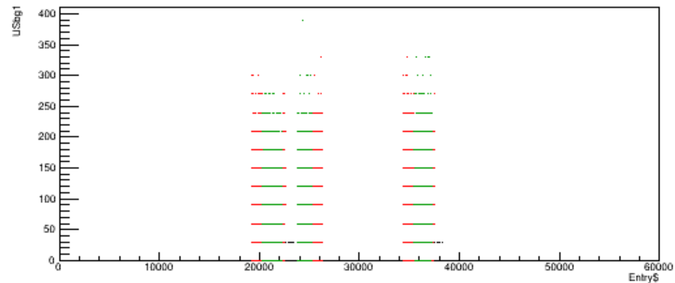
Run 6078 quartetwise, USbg1 vs time
