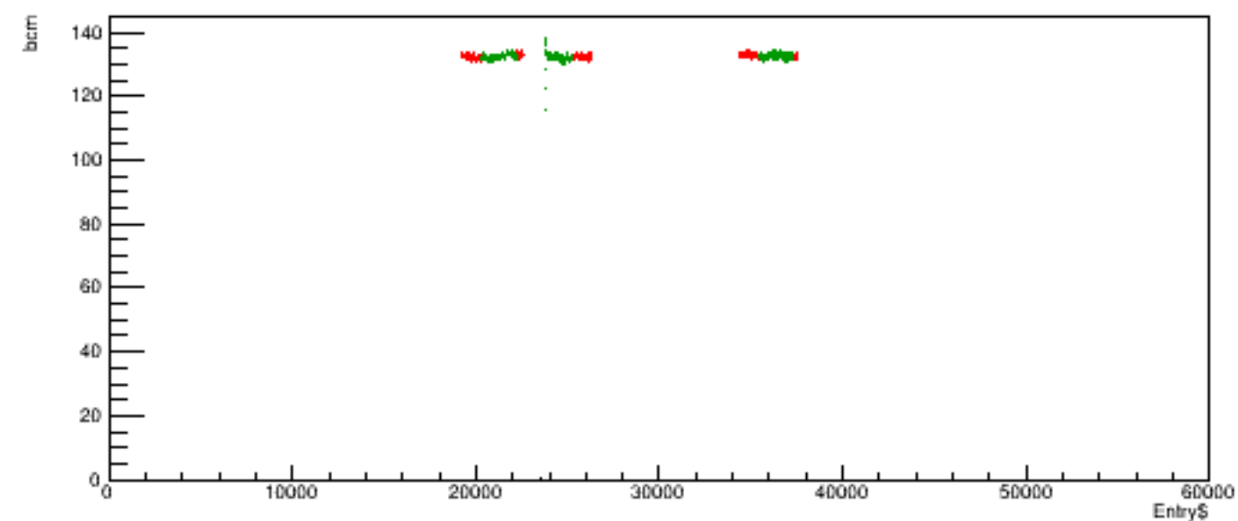
Run 6078 quartetwise, posH4 vs time
