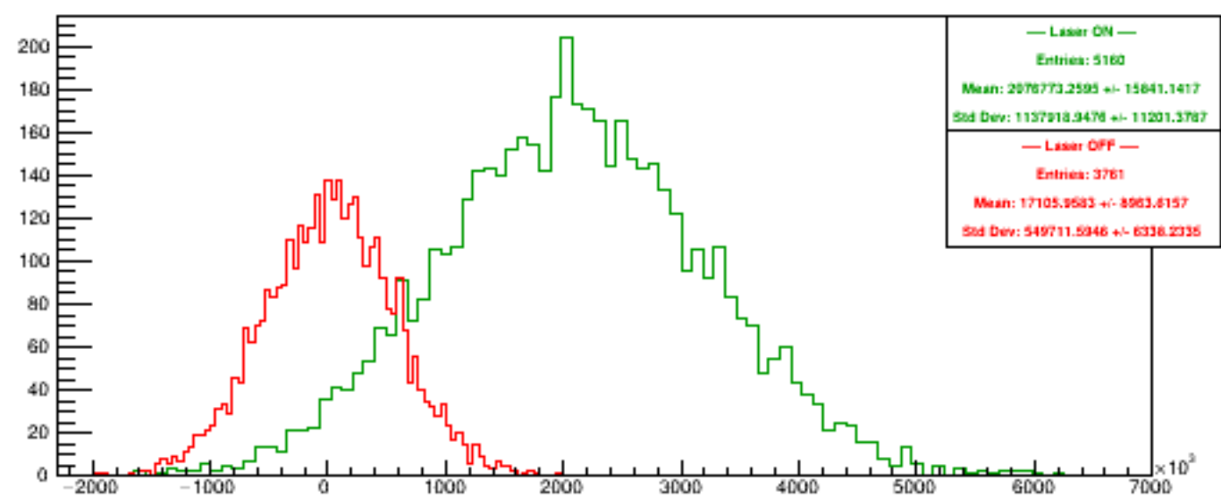
Run 6078 quartetwise, Diffs4
