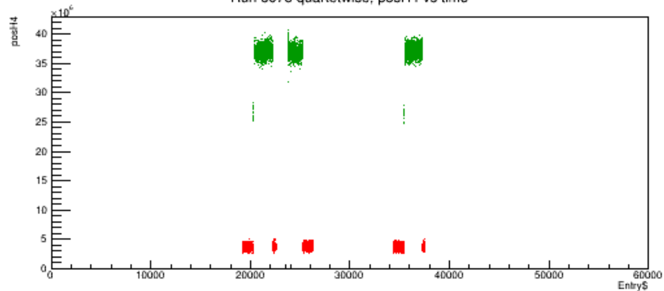
Run 6078 quartetwise, posH4 vs time
