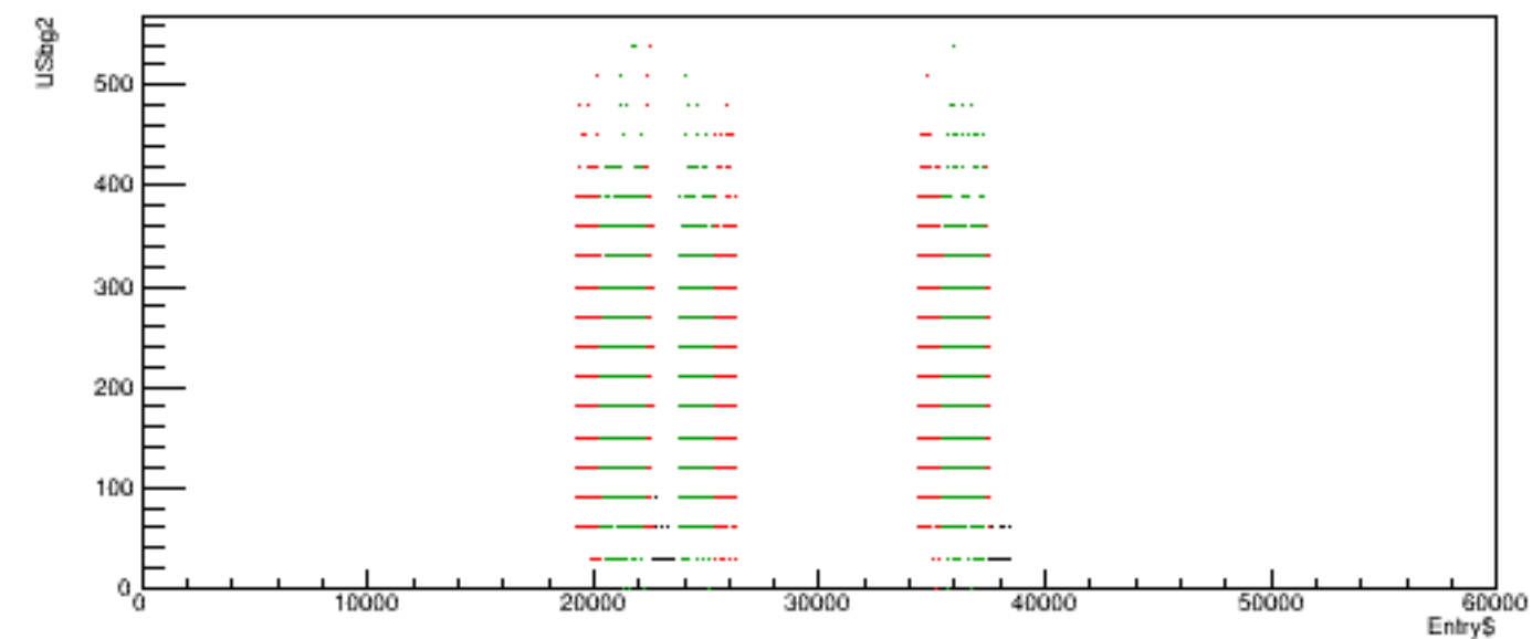
Run 6078 quartetwise, USbg2 vs time
