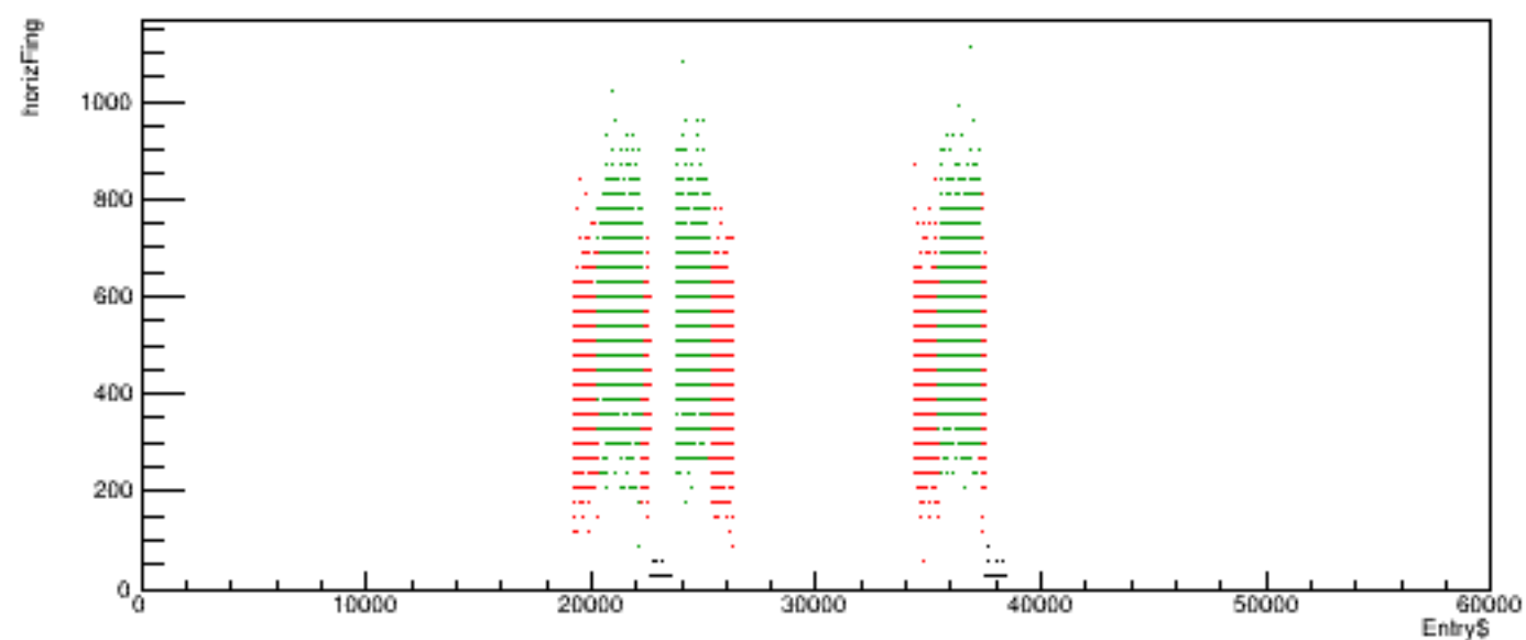
Run 6078 quartetwise, horizFing vs time
