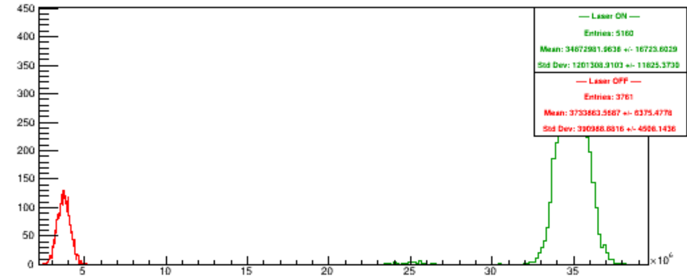
Run 6078 quartetwise, NegHelAcc4
