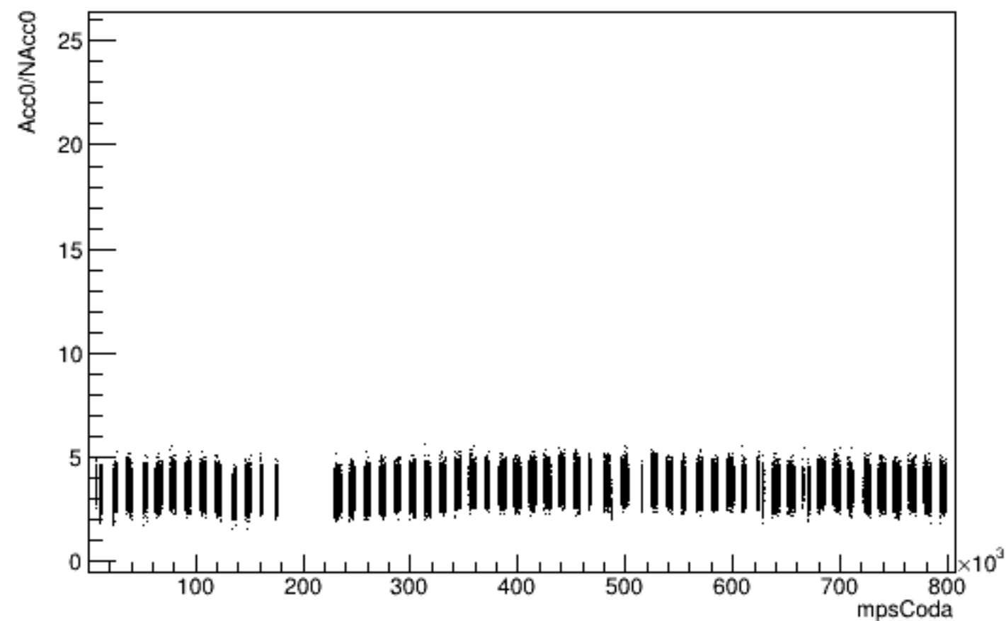
Run 6086 mpwise, Acc0 vs Time: Beam ON, Laser OFF
