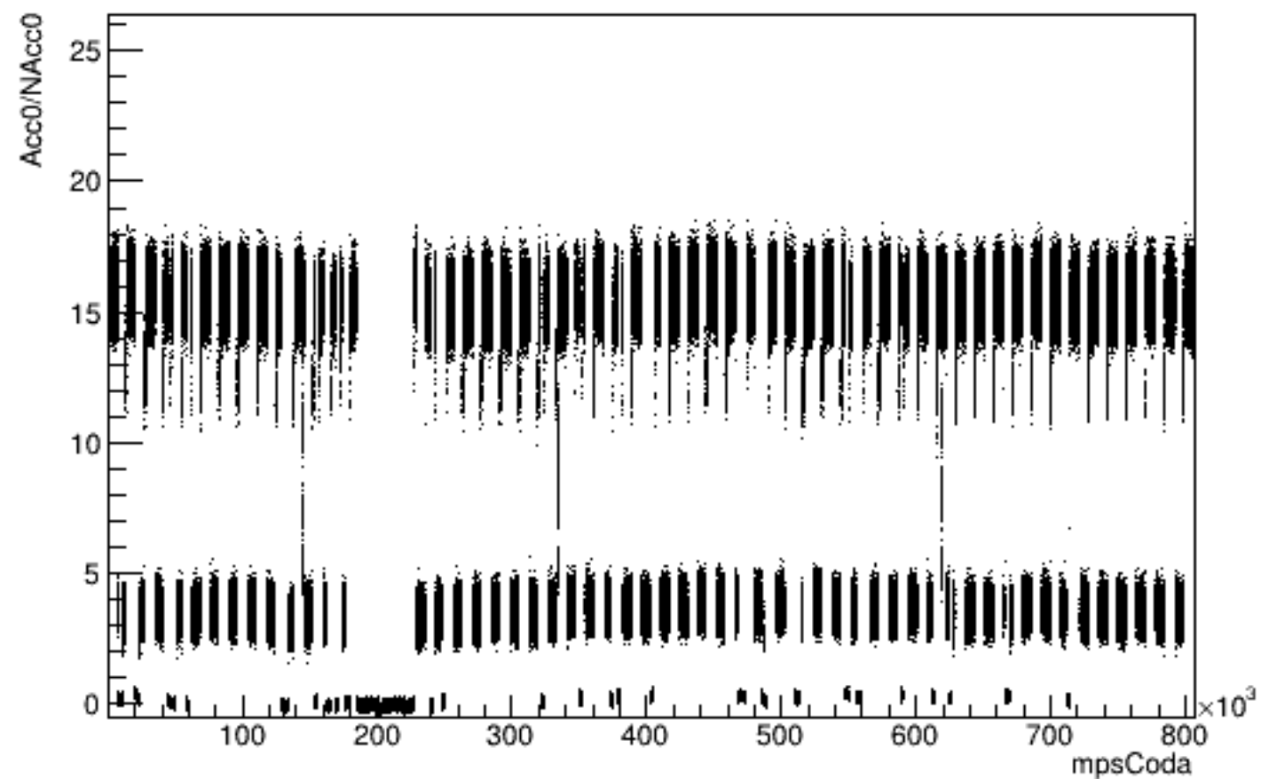
Run 6086 mpwise, Acc0 vs Time: All
