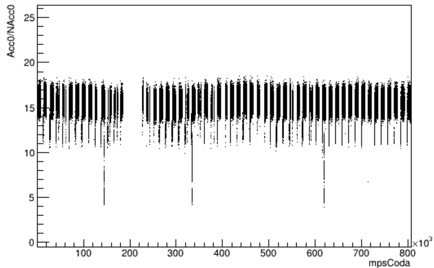
Run 6086 mpwise, Acc0 vs Time: Beam ON, Laser ON
