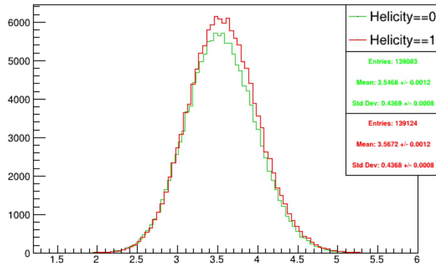
Run 6086 mpwise, acc0: Beam ON, Laser OFF
