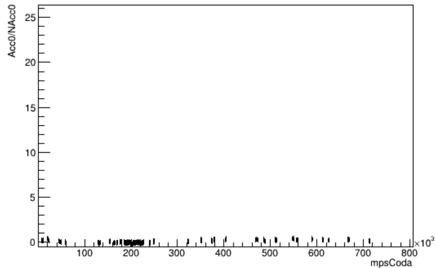
Run 6086 mpwise, Acc0 vs Time: Beam OFF
