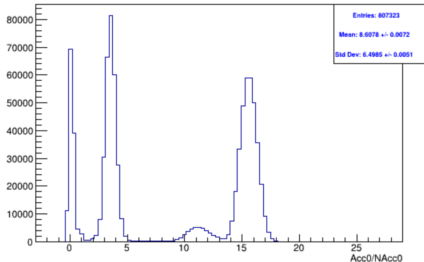
Run 6086 mpwise, acc0: All
