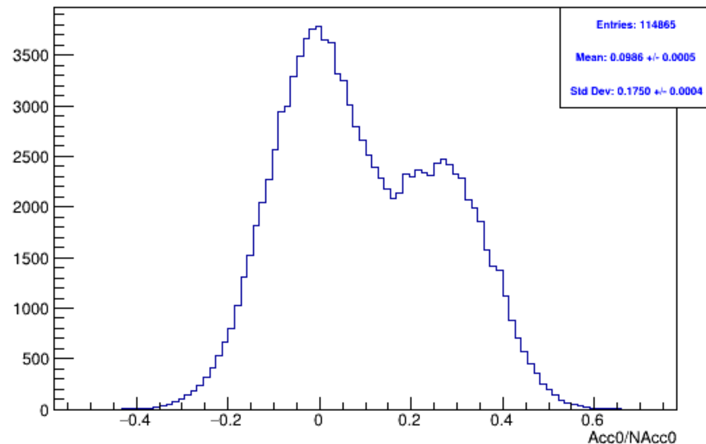
Run 6086 mpwise, acc0: Beam OFF
