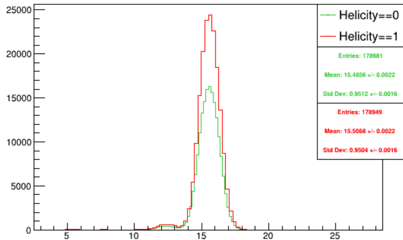
Run 6086 mpwise, acc0: Beam ON, Laser ON
