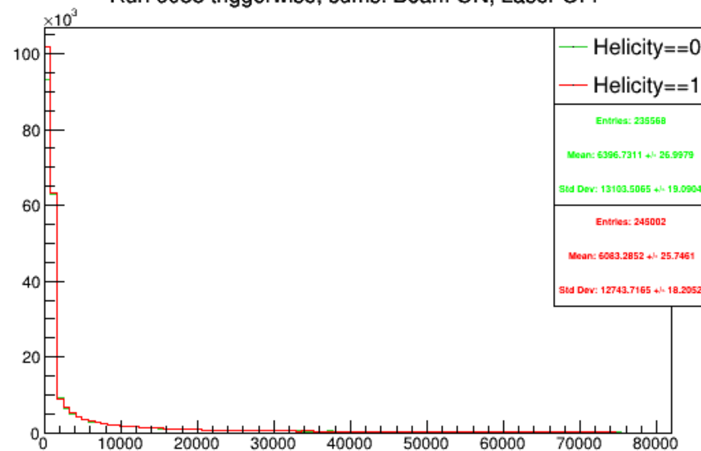
Run 6088 triggerwise, sums: Beam ON, Laser OFF
