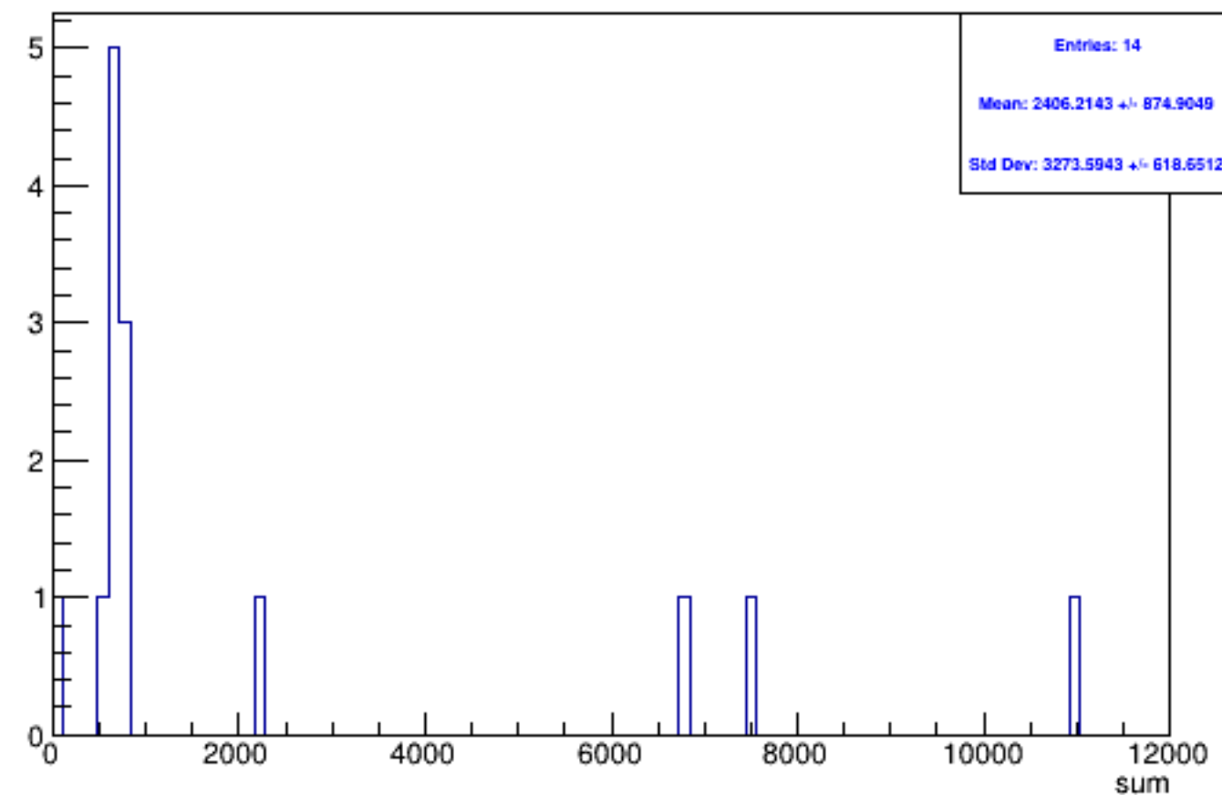
Run 6088 triggerwise, sums: Beam OFF
