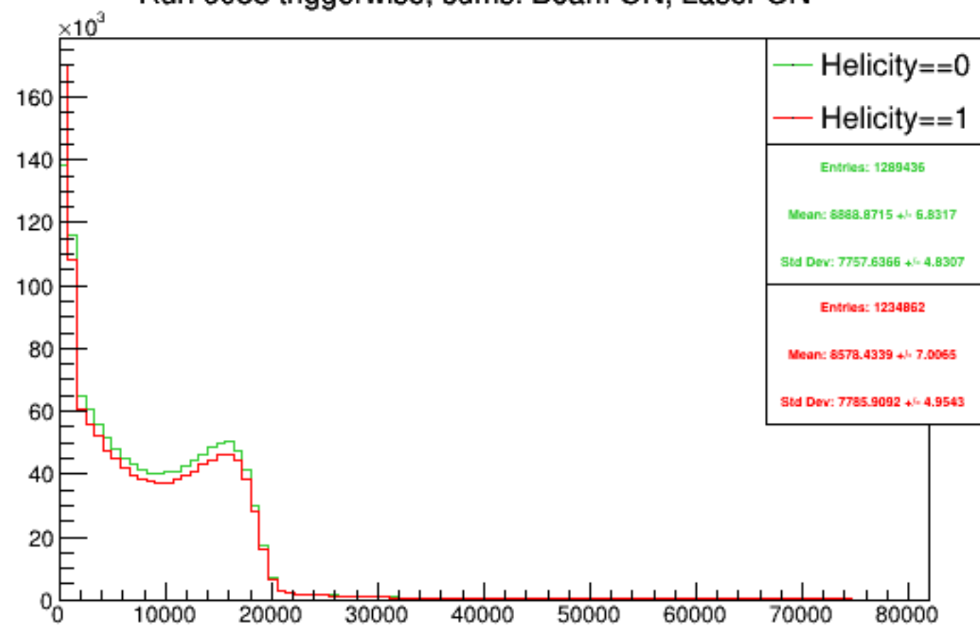
Run 6088 triggerwise, sums: Beam ON, Laser ON
