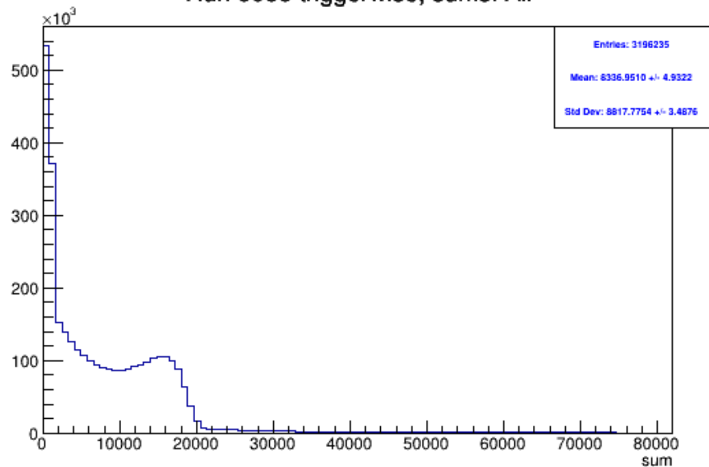
Run 6088 triggerwise, sums: All
