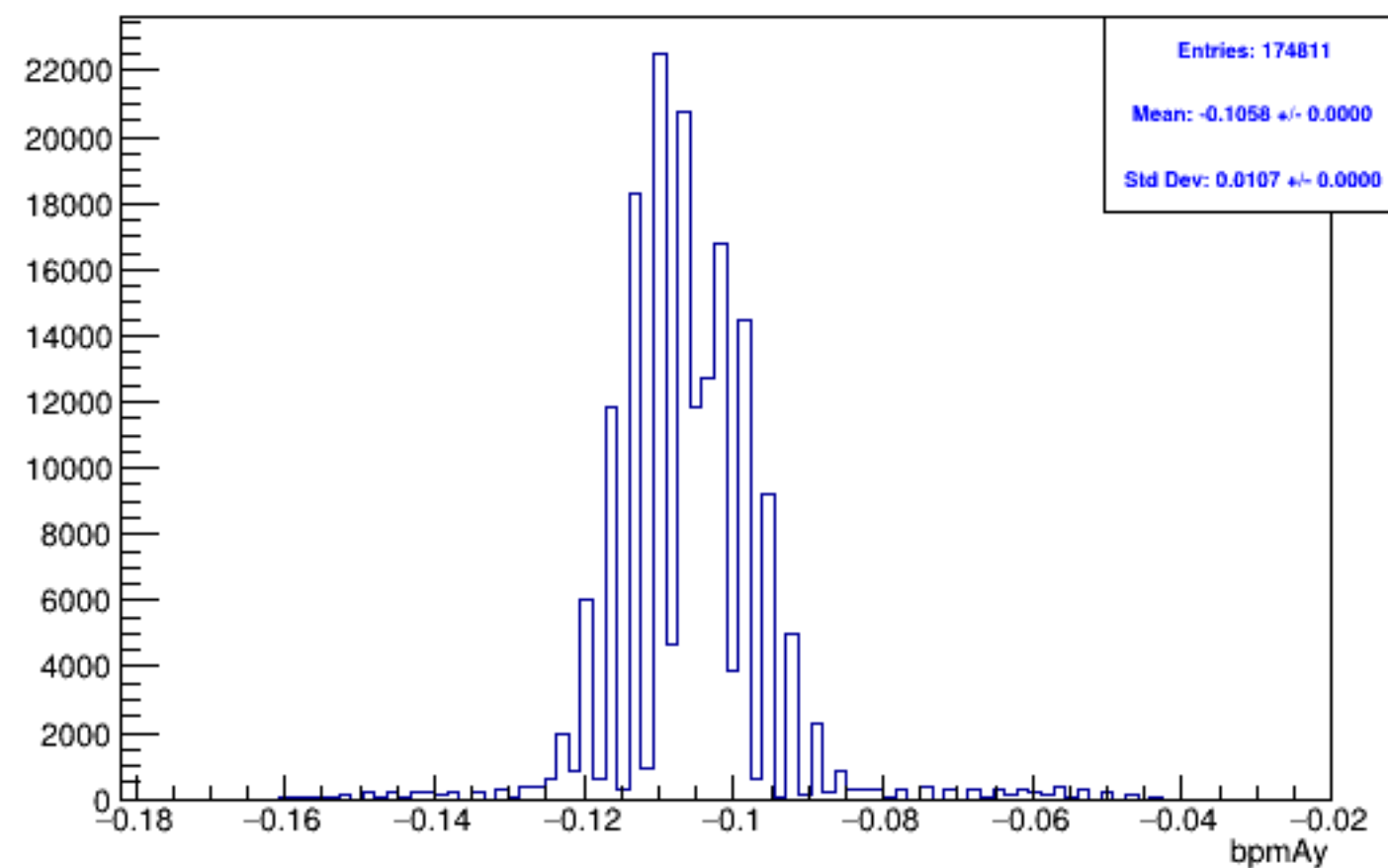
Run 6091, mpswise, bpmAy: Beam ON, Laser OFF
