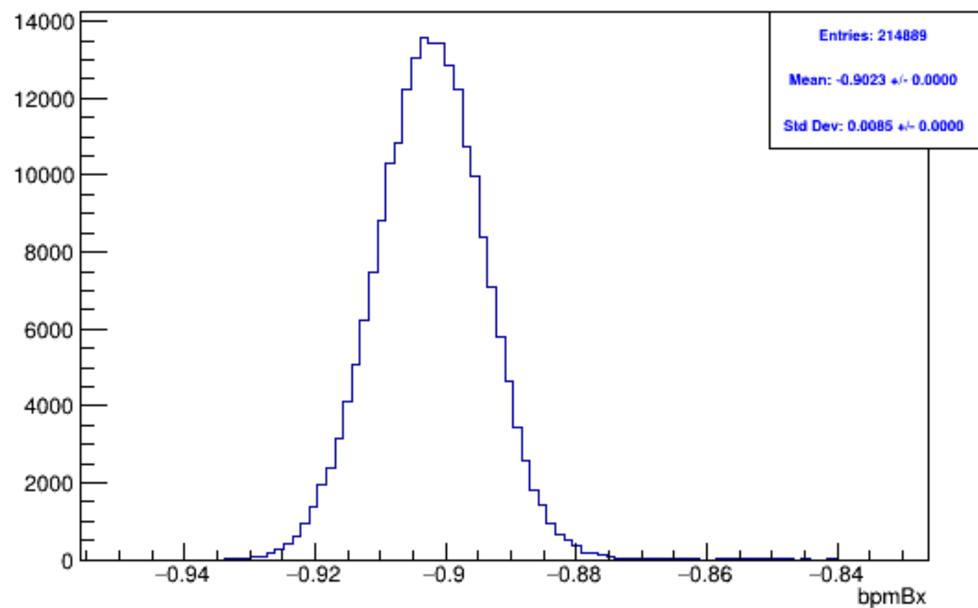
Run 6091, mpswise, bpmBx: Beam ON, Laser ON
