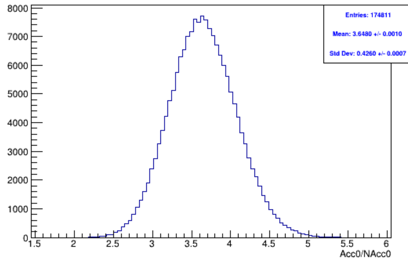
Run 6091, mpwise, acc0: Beam ON, Laser OFF
