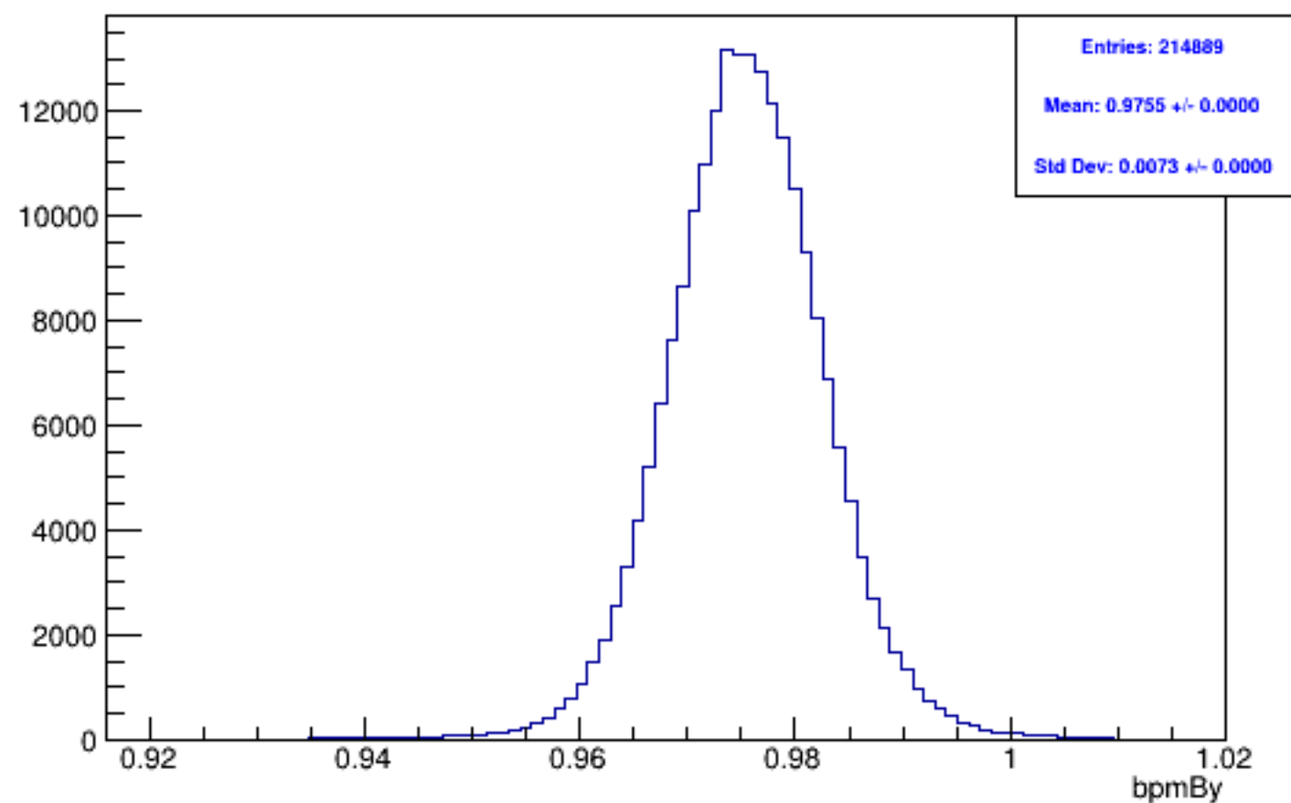
Run 6091, mpswise, bpmBy: Beam ON, Laser ON
