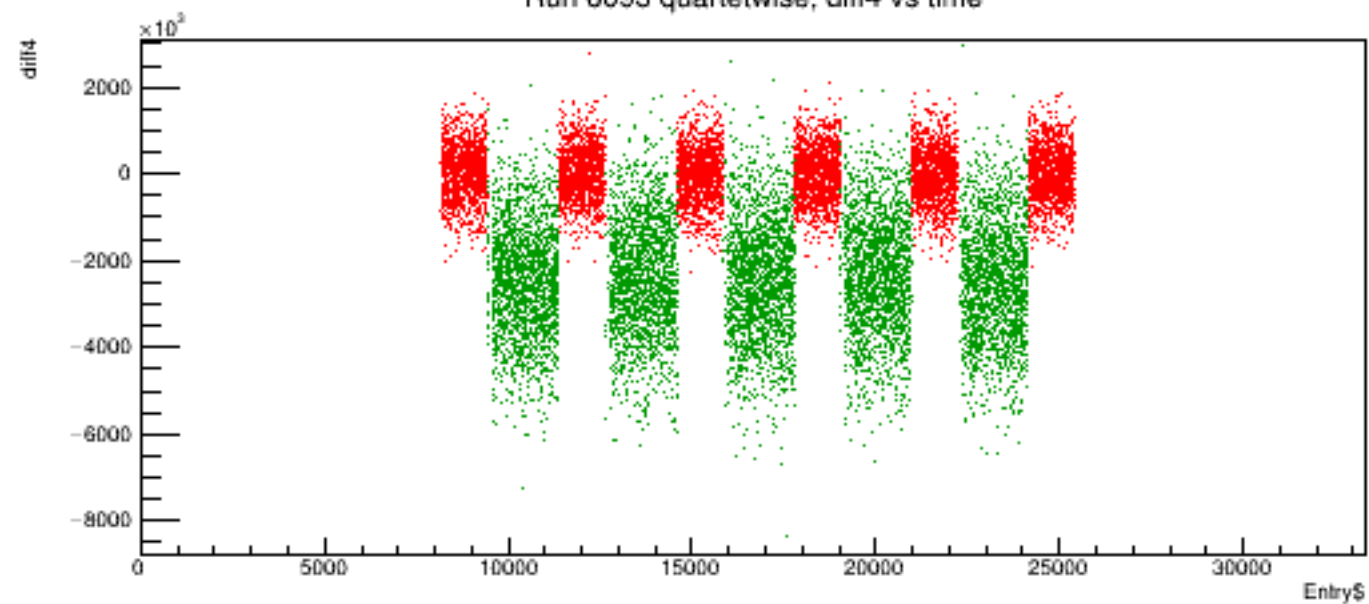
Run 6093 quartetwise, diff4 vs time
