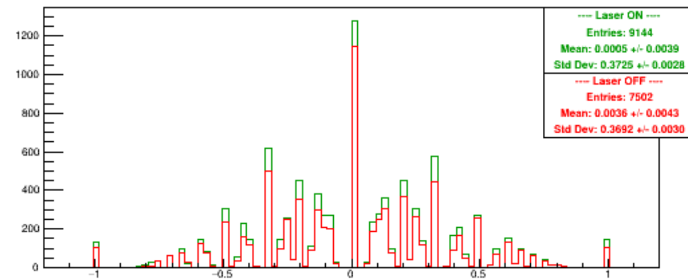
Run 6093 quartetwise, Asyms USbg2
