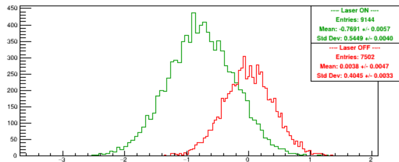
Run 6093 quartetwise, Diffs0
