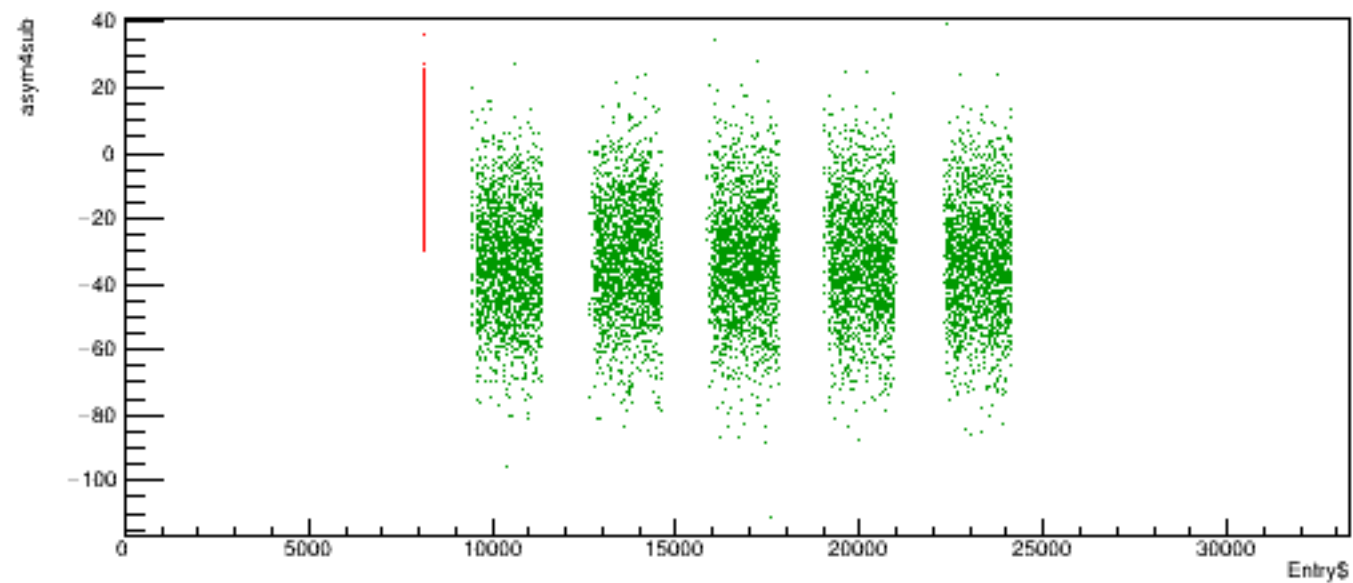
Run 6093 quartetwise, asym4sub vs time
