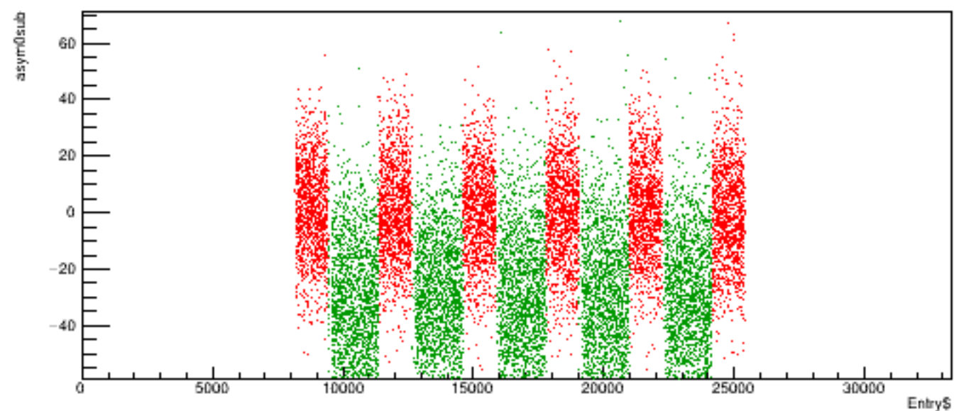
Run 6093 quartetwise, asym0sub vs time
