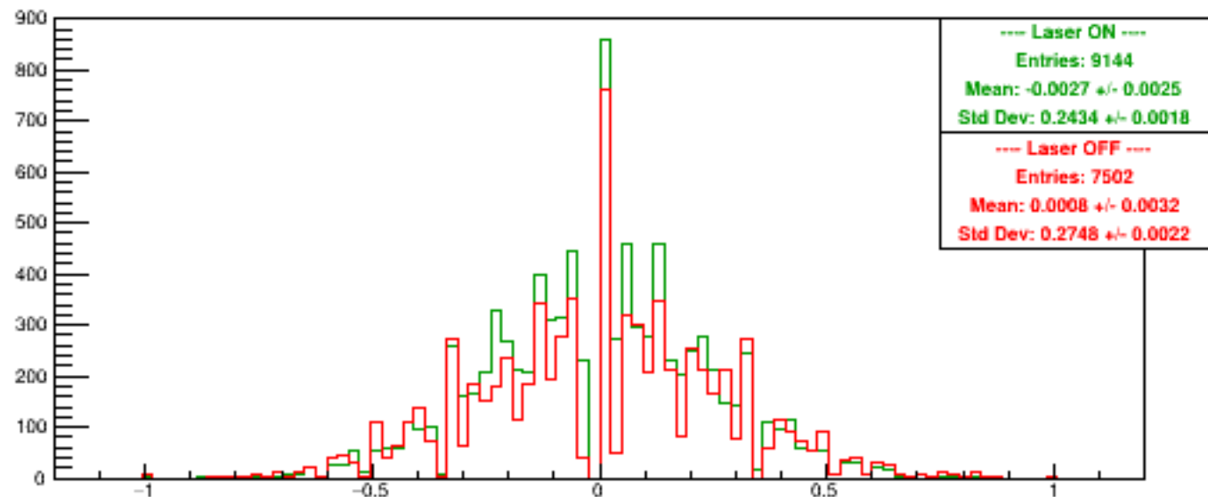
Run 6093 quartetwise, Asyms Horiz Finger
