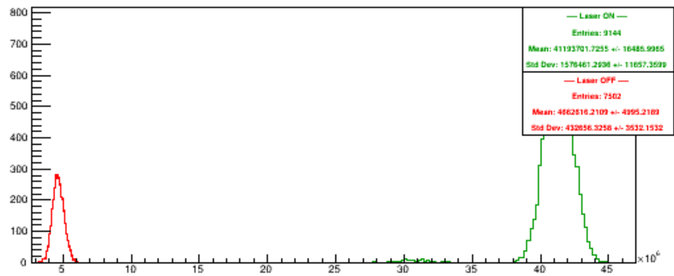
Run 6093 quartetwise, PosHelAcc4
