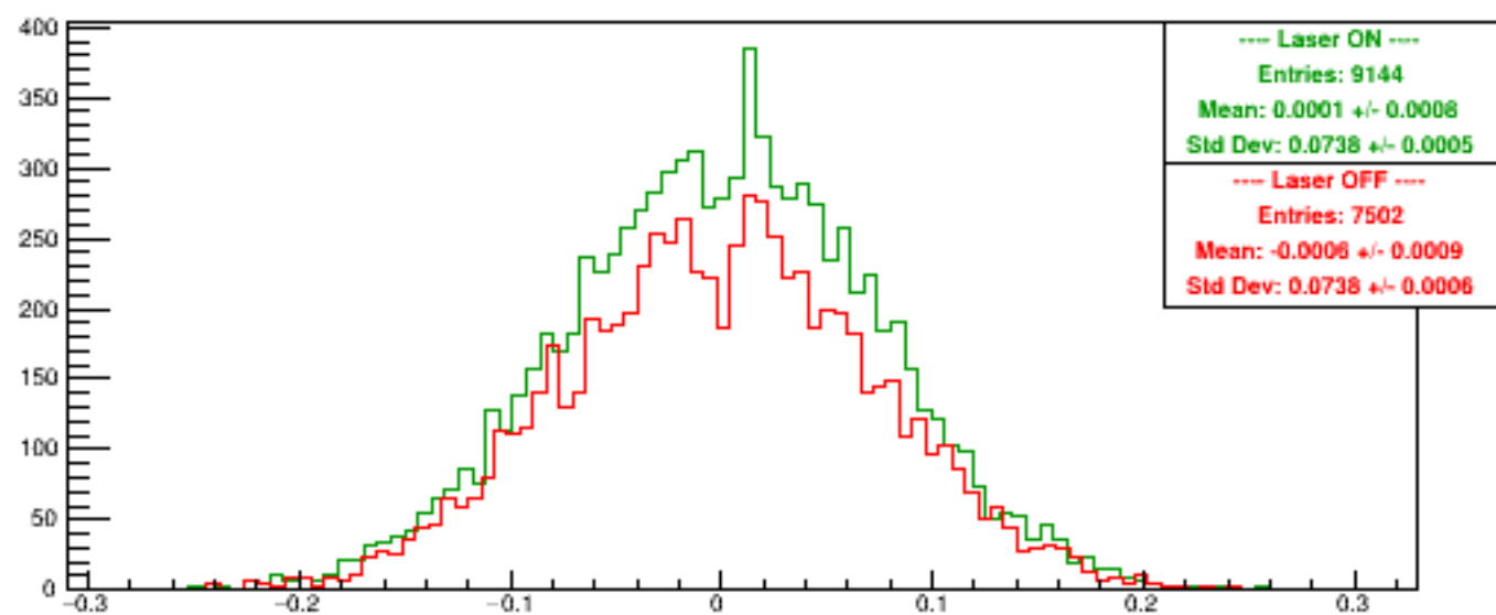
Run 6093 quartetwise, Asyms DSbg1
