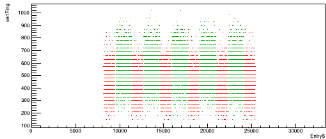
Run 6093 quartetwise, vertFing vs time
