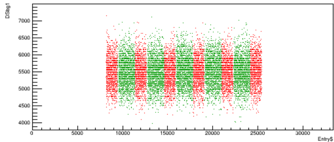
Run 6093 quartetwise, DSbg1 vs time
