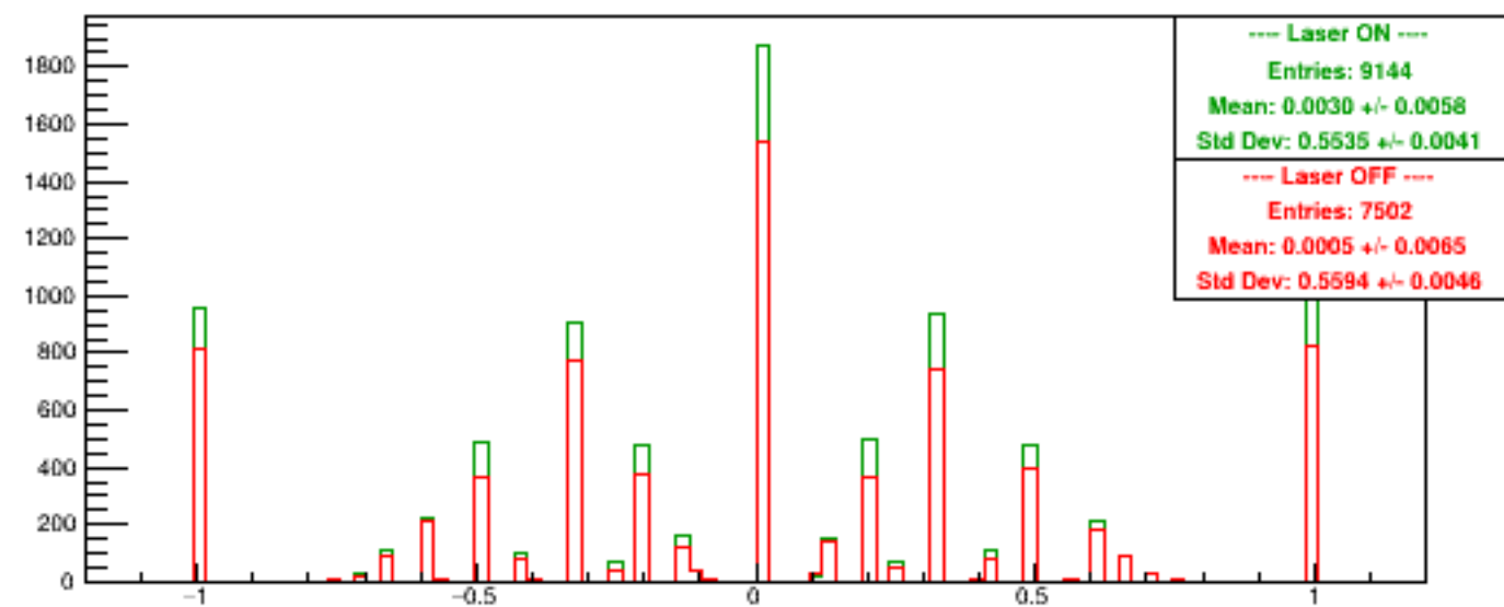
Run 6093 quartetwise, Asyms USbg1
