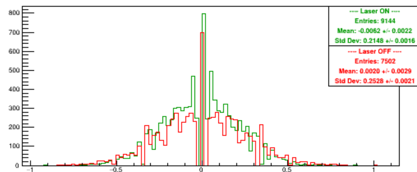
Run 6093 quartetwise, Asyms Vert Finger
