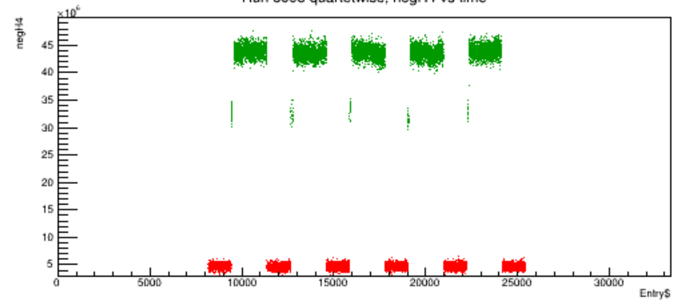
Run 6093 quartetwise, negH4 vs time
