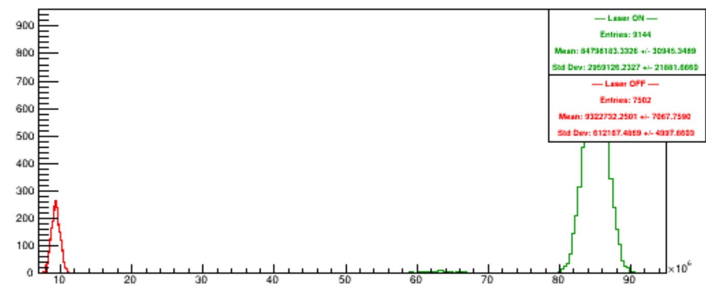
Run 6093 quartetwise, Sums4
