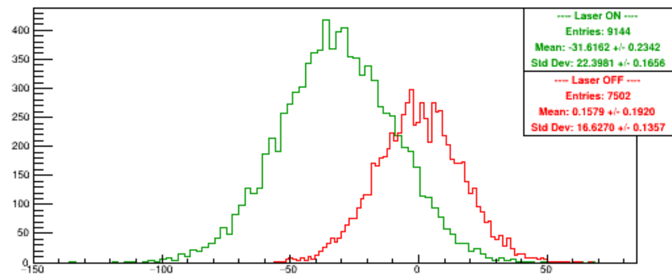
Run 6093 quartetwise, Asyms0
