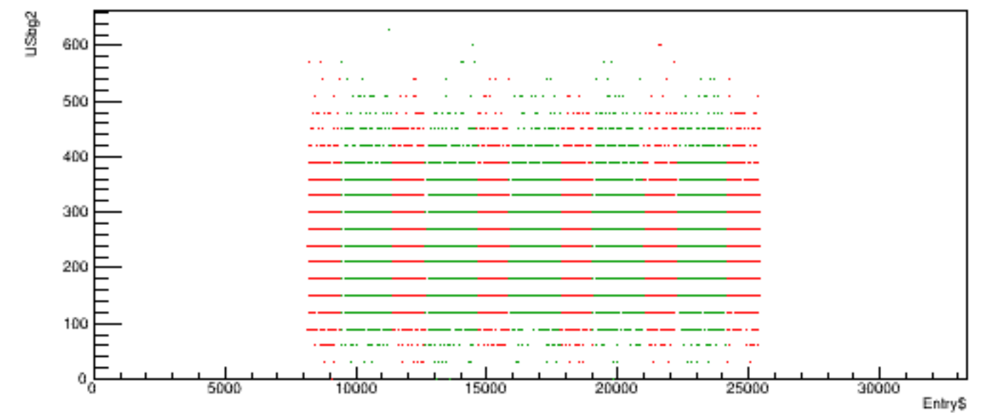
Run 6093 quartetwise, USbg2 vs time
