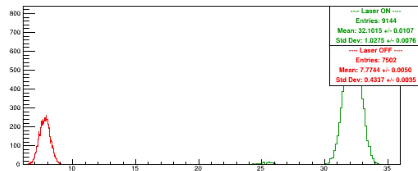
Run 6093 quartetwise, Sums0
