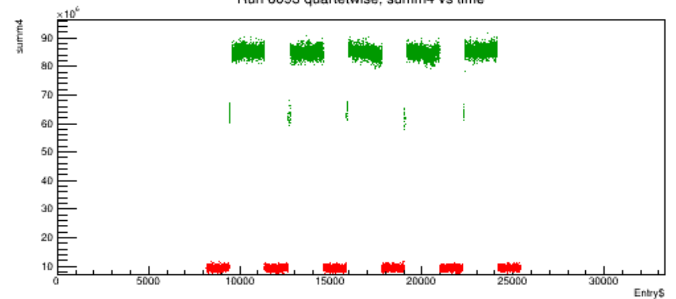
Run 6093 quartetwise, summ4 vs time
