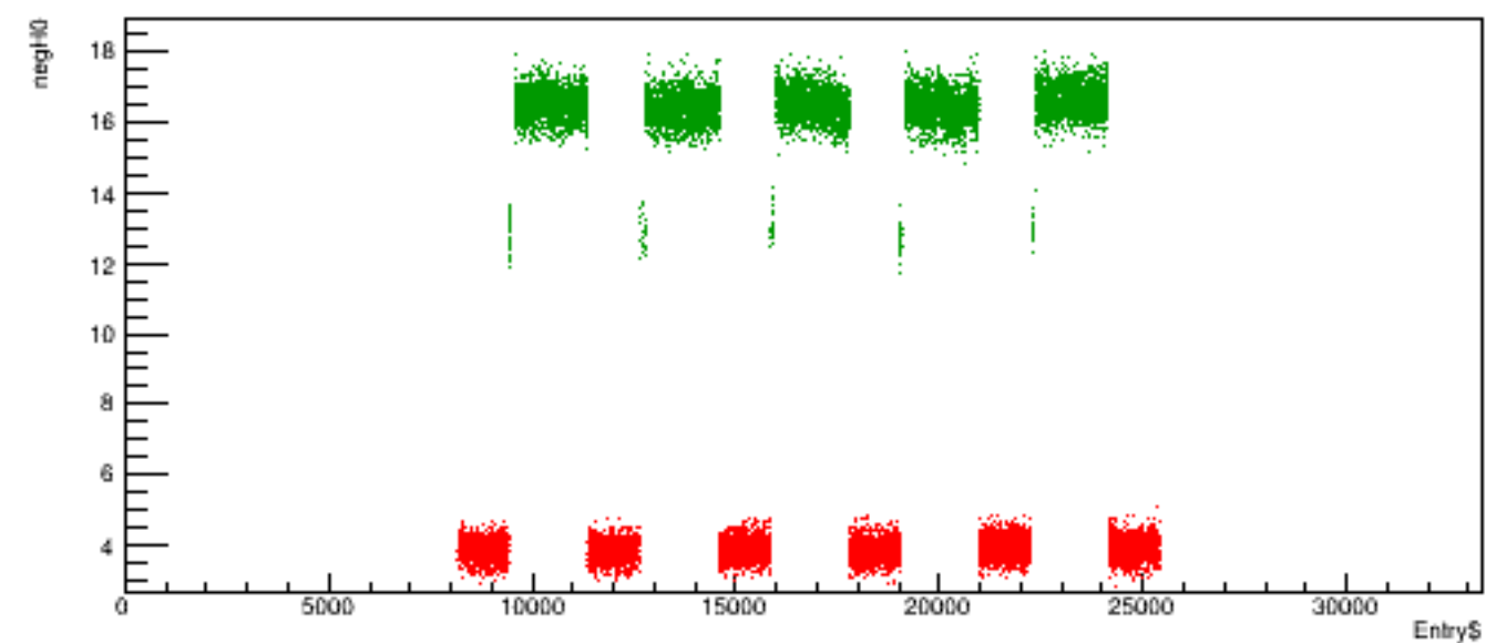
Run 6093 quartetwise, negH0 vs time
