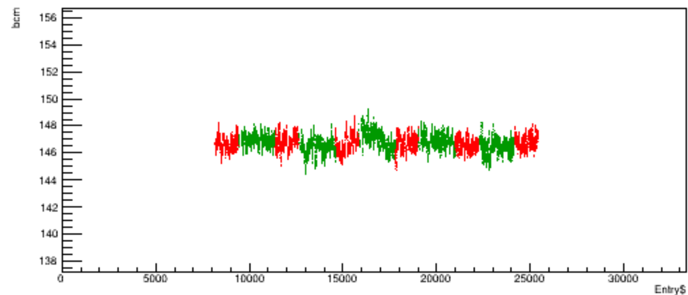
Run 6093 quartetwise, posH4 vs time
