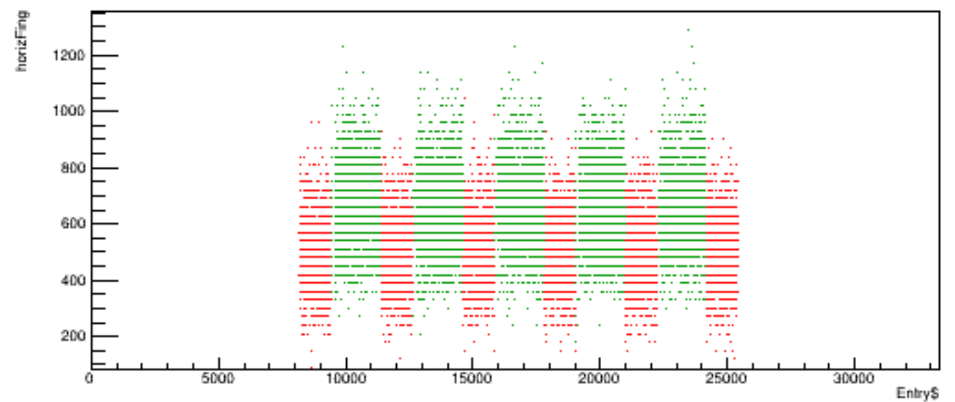
Run 6093 quartetwise, horizFing vs time
