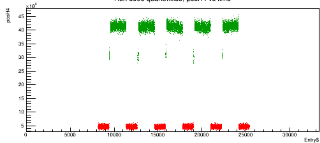
Run 6093 quartetwise, posH4 vs time
