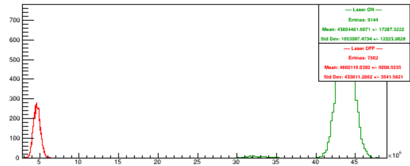
Run 6093 quartetwise, NegHelAcc4
