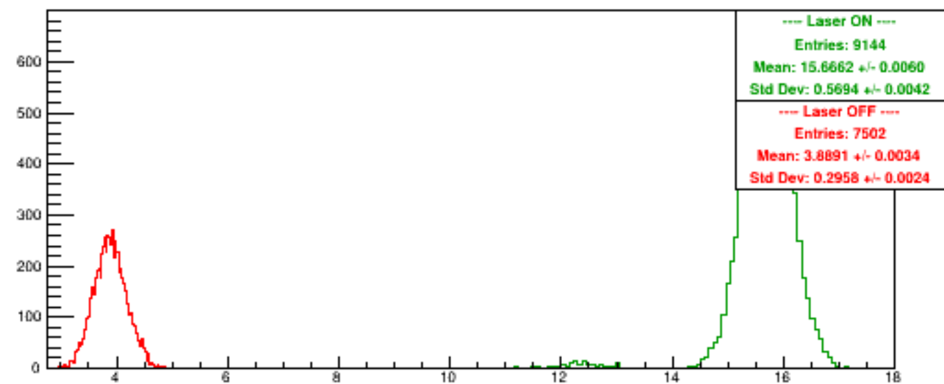
Run 6093 quartetwise, PosHelAcc0/NSamples0
