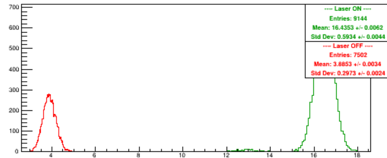
Run 6093 quartetwise, NegHelAcc0/NSamples0
