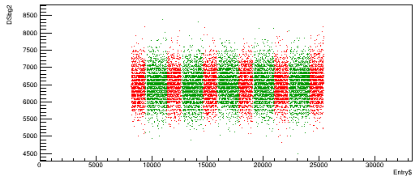
Run 6093 quartetwise, DSbg2 vs time
