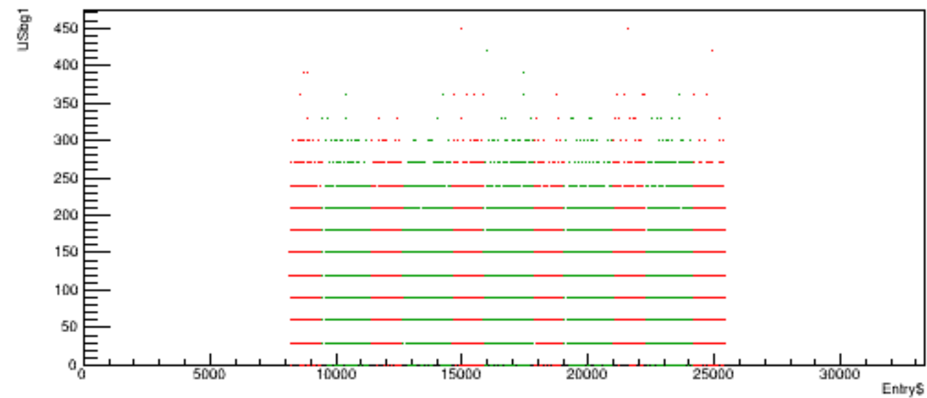
Run 6093 quartetwise, USbg1 vs time
