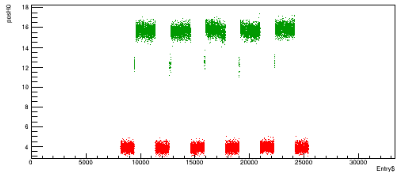
Run 6093 quartetwise, posH0 vs time
