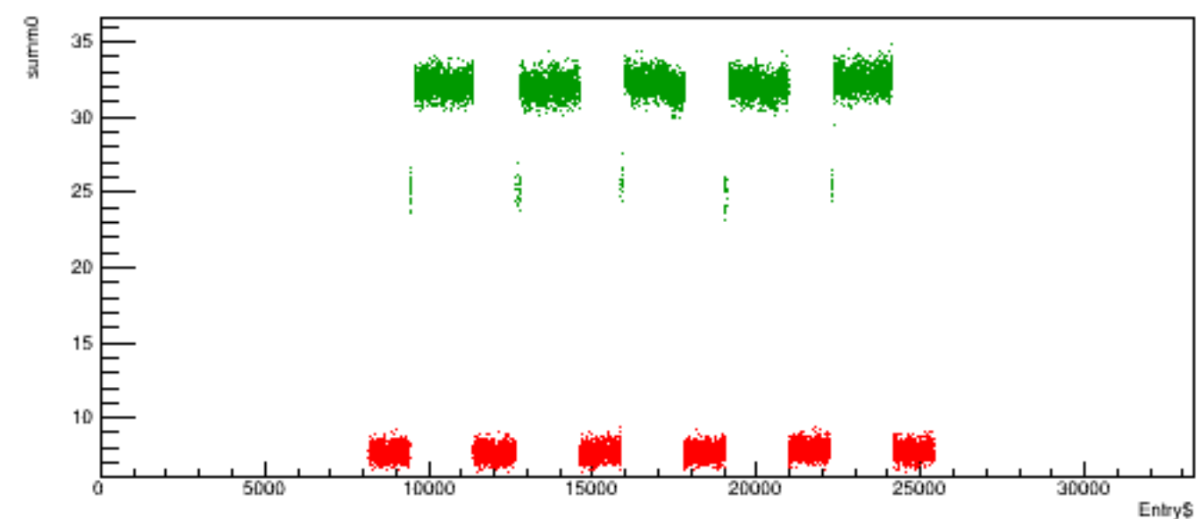
Run 6093 quartetwise, summ0 vs time
