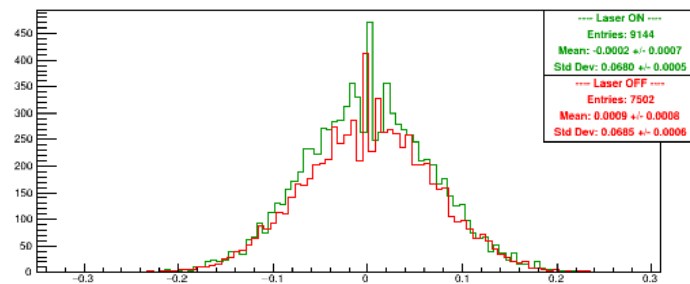
Run 6093 quartetwise, Asyms DSbg2
