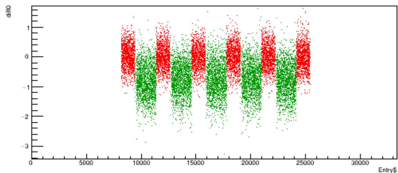
Run 6093 quartetwise, diff0 vs time
