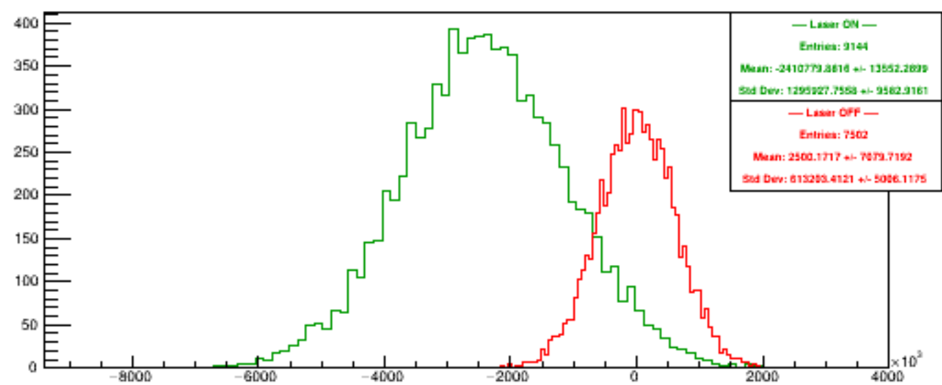
Run 6093 quartetwise, Diffs4
