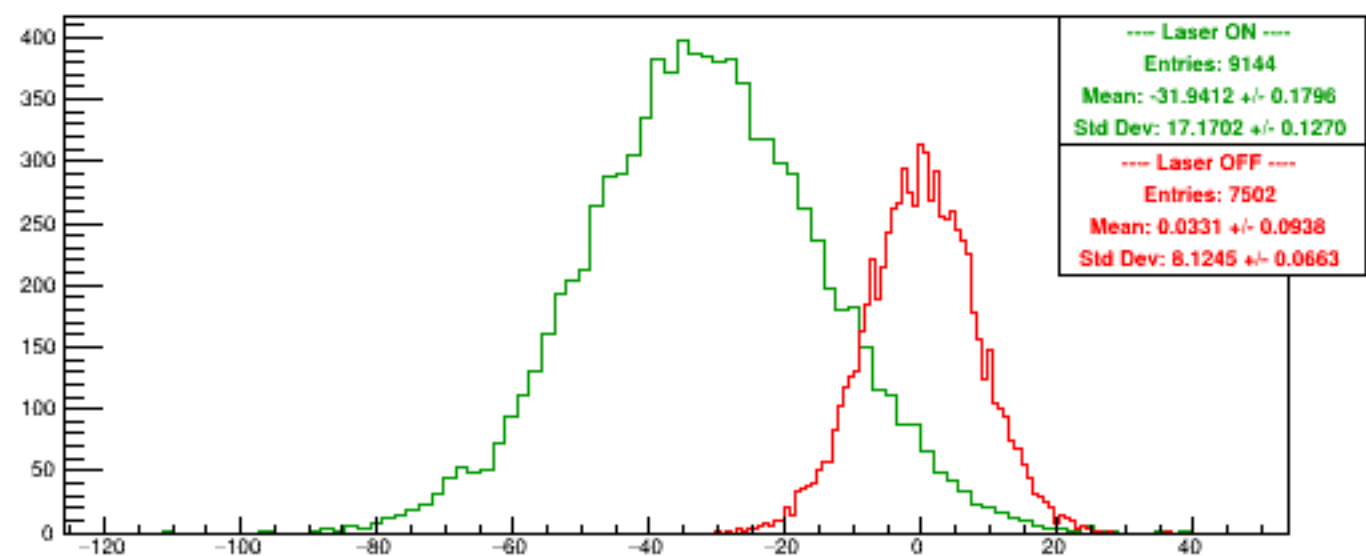
Run 6093 quartetwise, Asyms4
