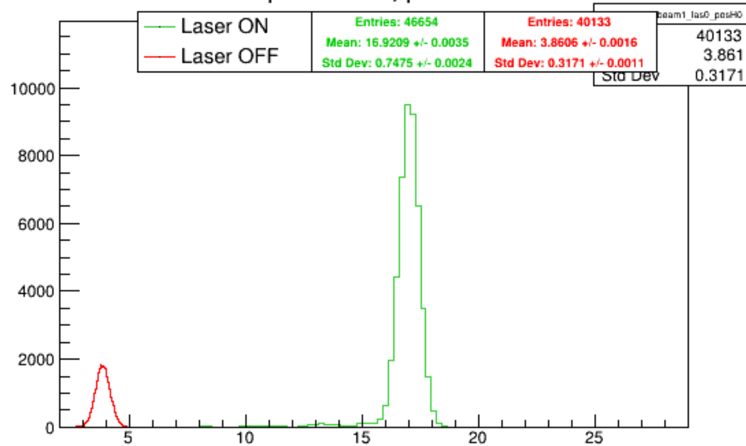
Run 6102 quartetwise, posH0: Beam ON
