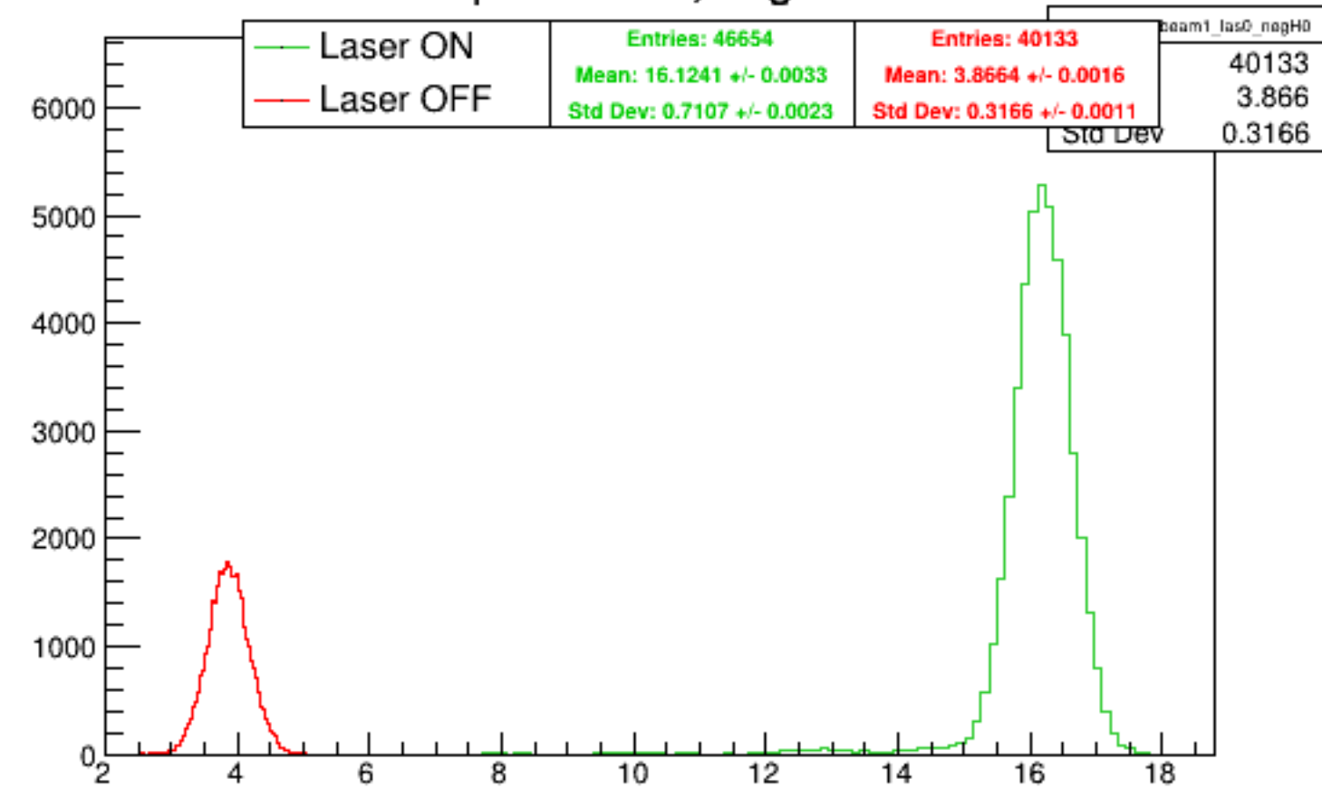
Run 6102 quartetwise, negH0: Beam ON
