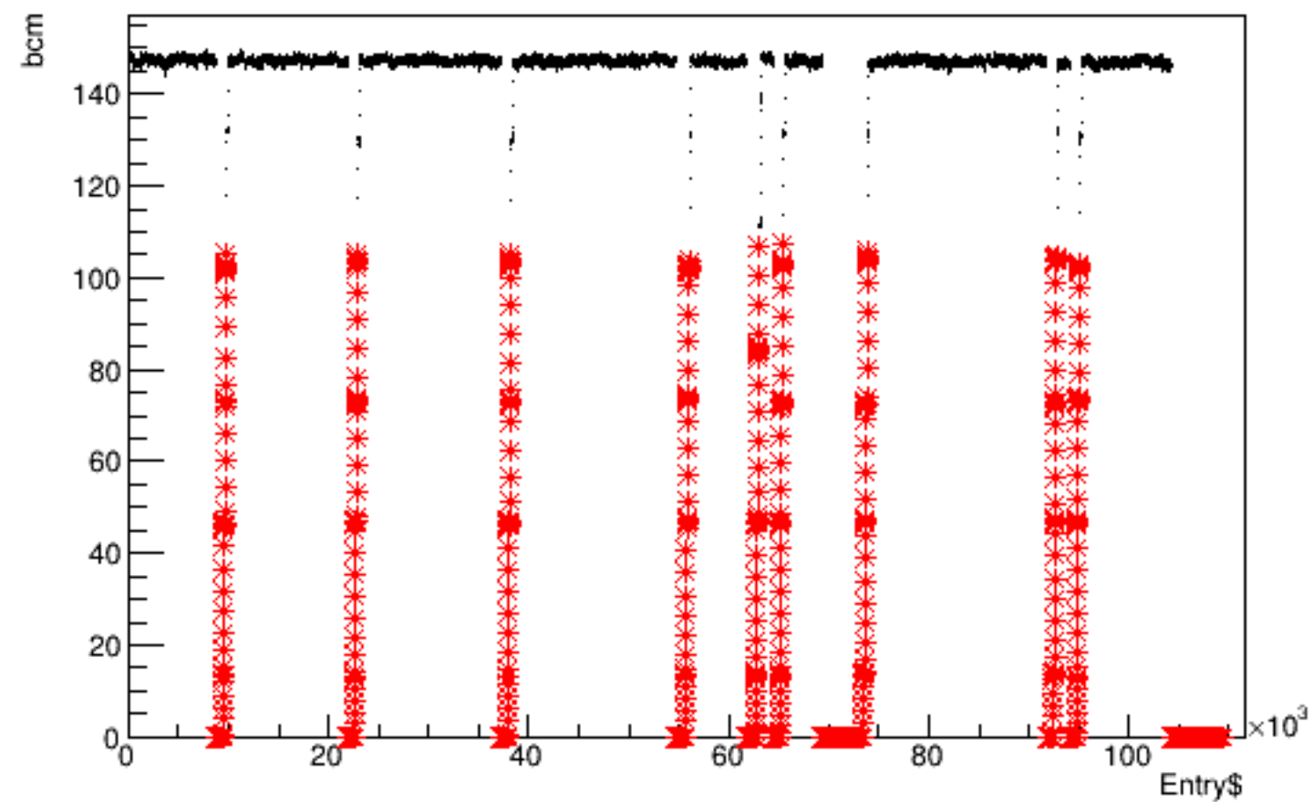
Run 6102 quartetwise, bcm vs time
