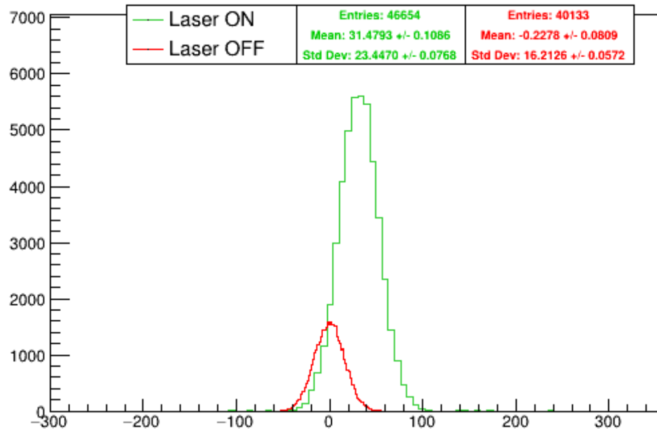
Run 6102 quartetwise, asym0sub: Beam ON
