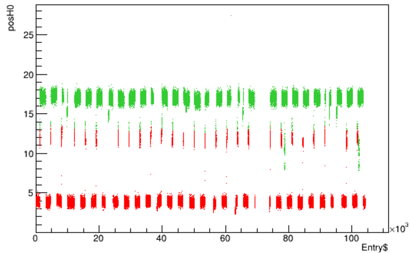
Run 6102 quartetwise, posH0 vs time
