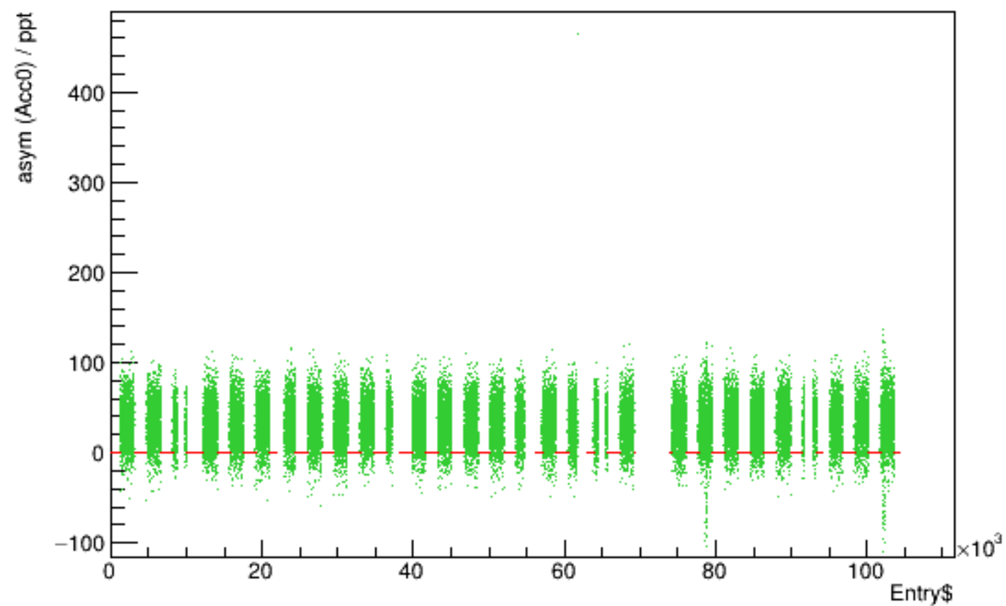
Run 6102 quartetwise, asym0sub vs time
