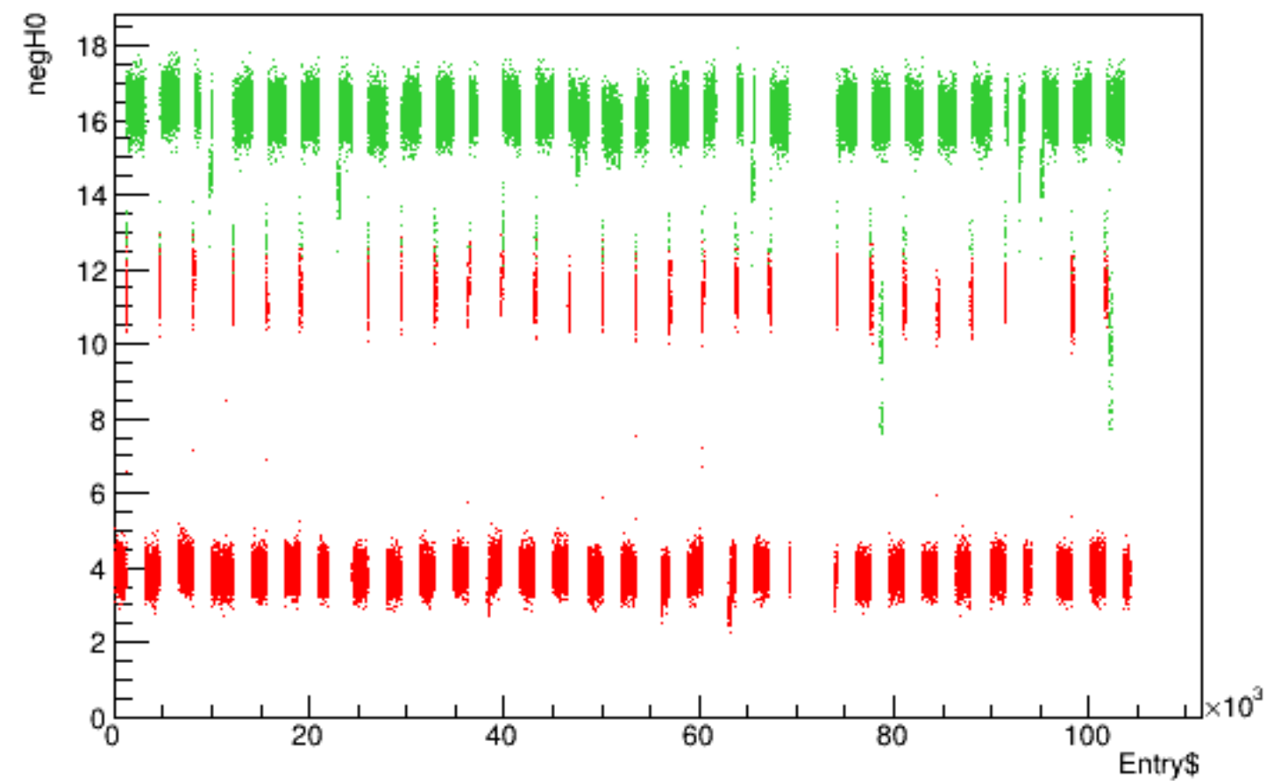
Run 6102 quartetwise, negH0 vs time
