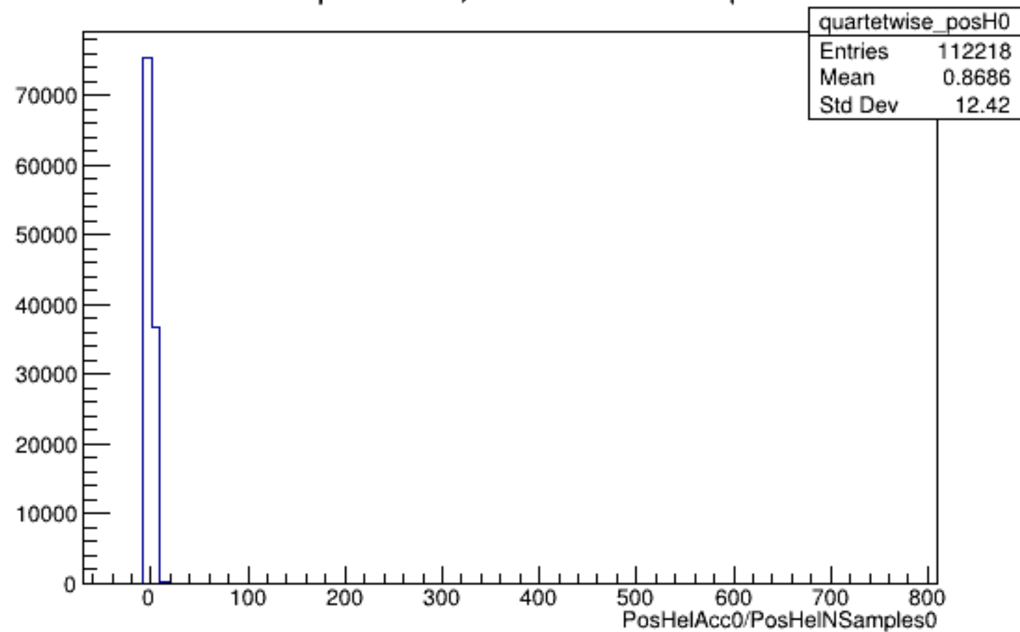
Run 6106 quartetwise, PosHelAcc0/NSamples0: All
