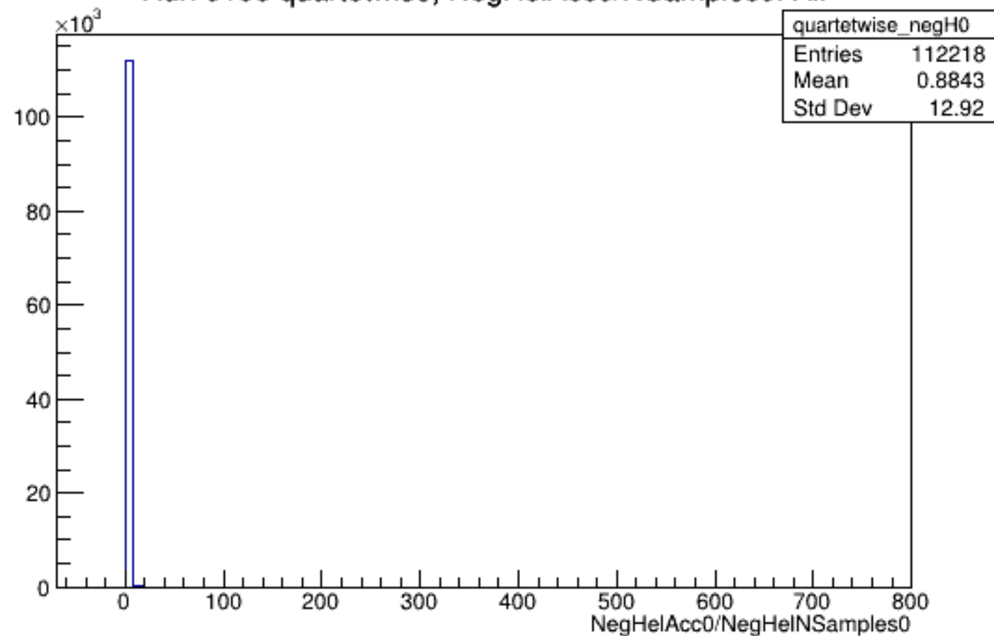
Run 6106 quartetwise, NegHelAcc0/NSamples0: All
