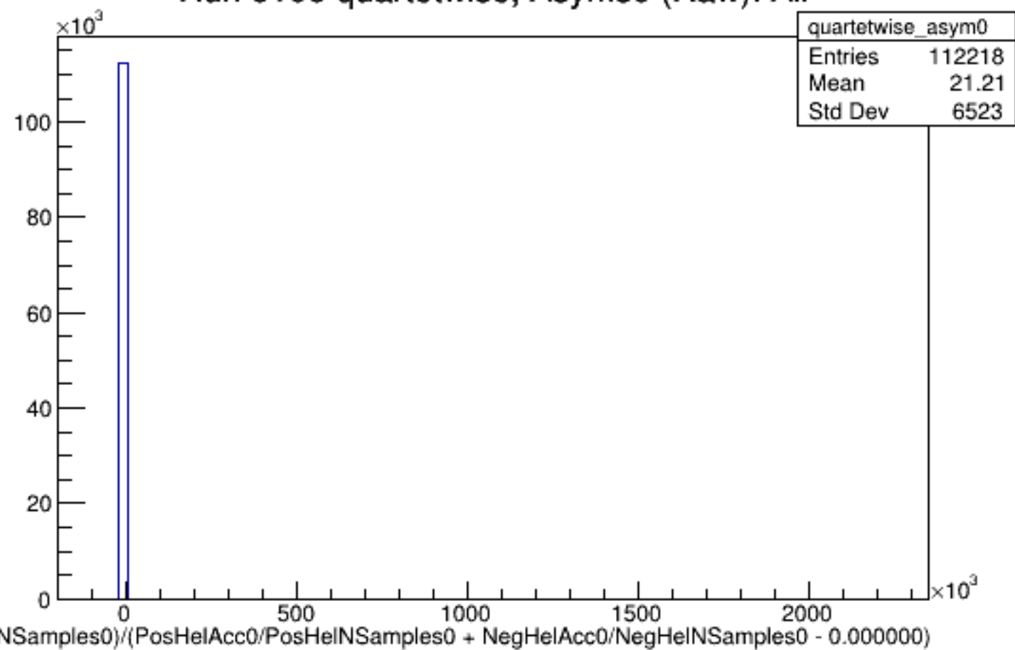
Run 6106 quartetwise, Asyms0 (Raw): All
