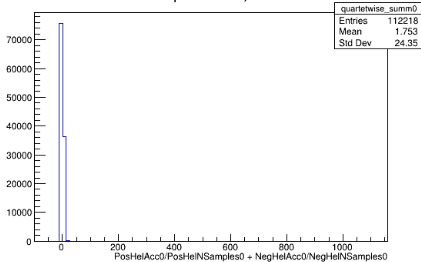
Run 6106 quartetwise, Sums0: All
