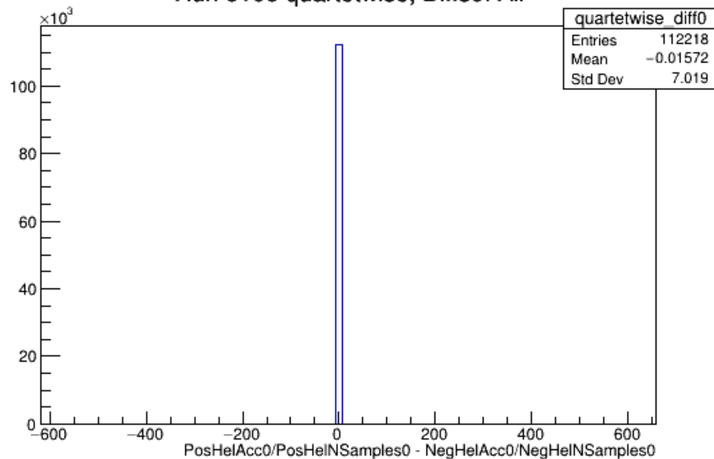
Run 6106 quartetwise, Diffs0: All
