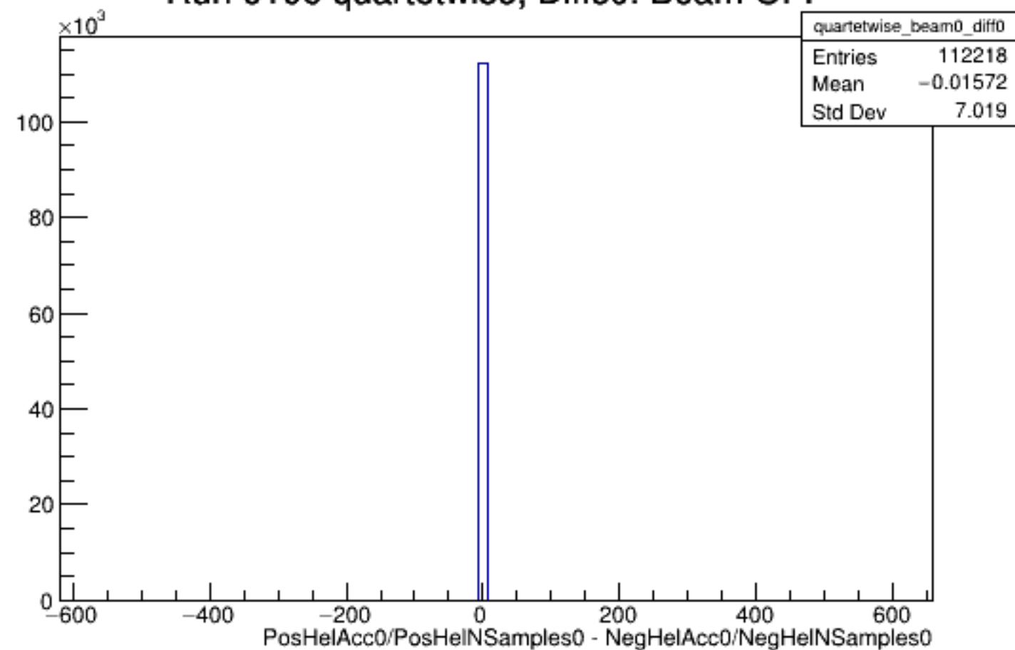
Run 6106 quartetwise, Diffs0: Beam OFF
