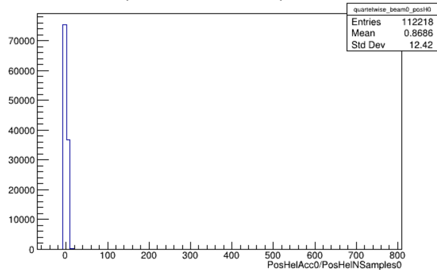
Run 6106 quartetwise, PosHelAcc0/NSamples0: Beam OFF
