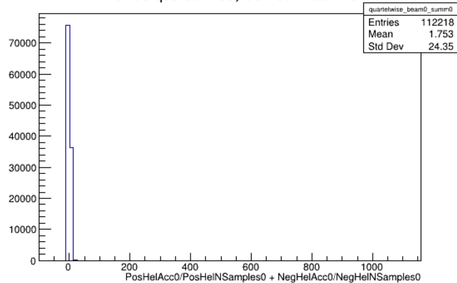
Run 6106 quartetwise, Sums0: Beam OFF
