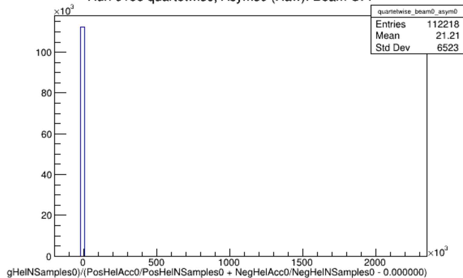
Run 6106 quartetwise, Asyms0 (Raw): Beam OFF
