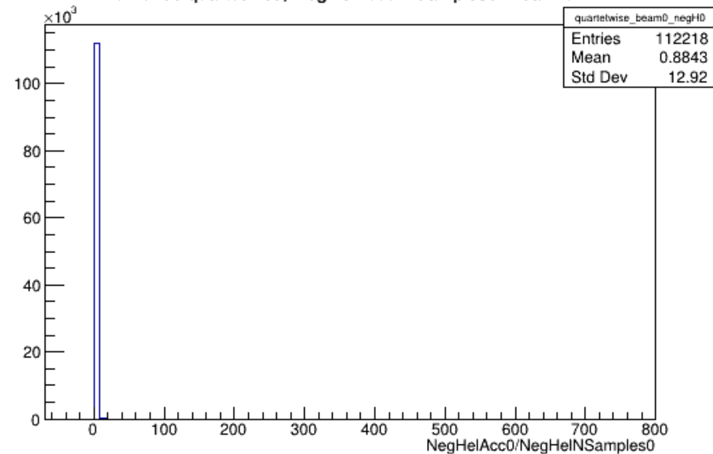
Run 6106 quartetwise, NegHelAcc0/NSamples0: Beam OFF
