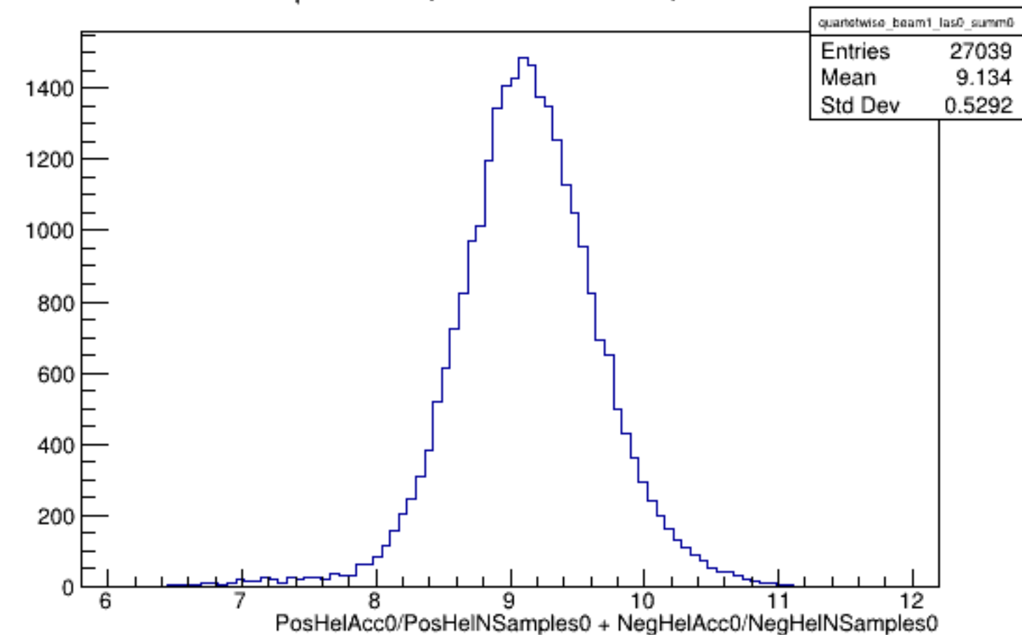
Run 6108 quartetwise, Sums0: Beam ON, Laser OFF
