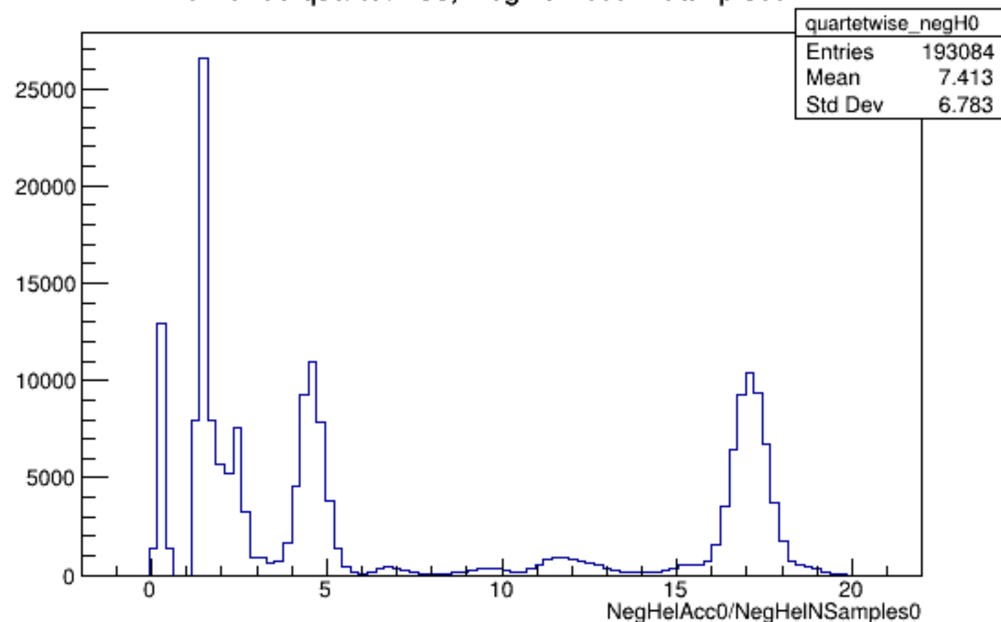
Run 6108 quartetwise, NegHelAcc0/NSamples0: All
