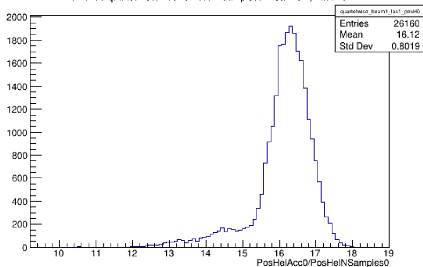
Run 6108 quartetwise, PosHelAcc0/NSamples0: Beam ON, Laser ON
