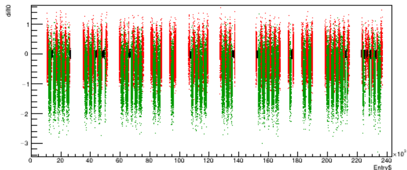
Run 6110 quartetwise, diff0 vs time
