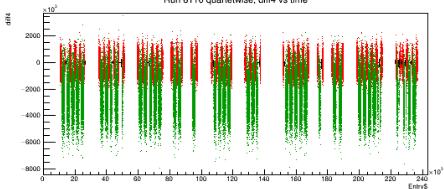
Run 6110 quartetwise, diff4 vs time
