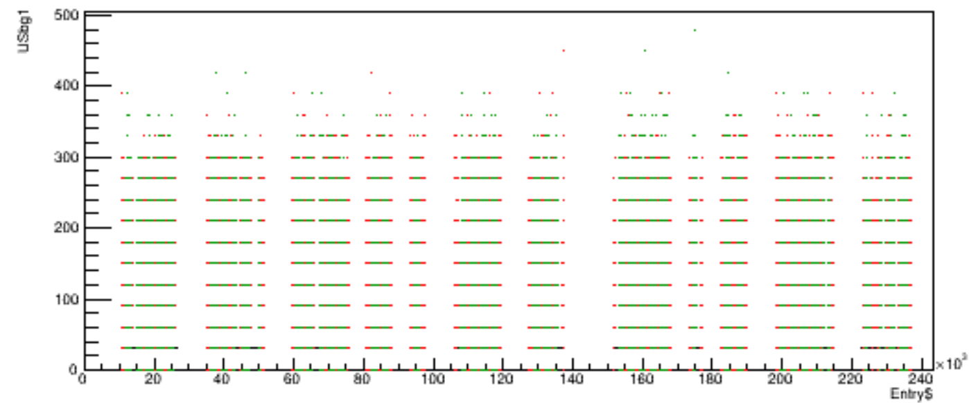
Run 6110 quartetwise, USbg1 vs time
