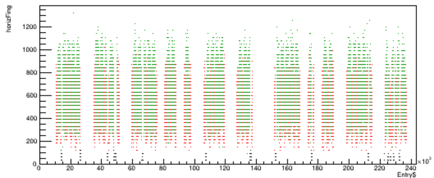
Run 6110 quartetwise, horizFing vs time
