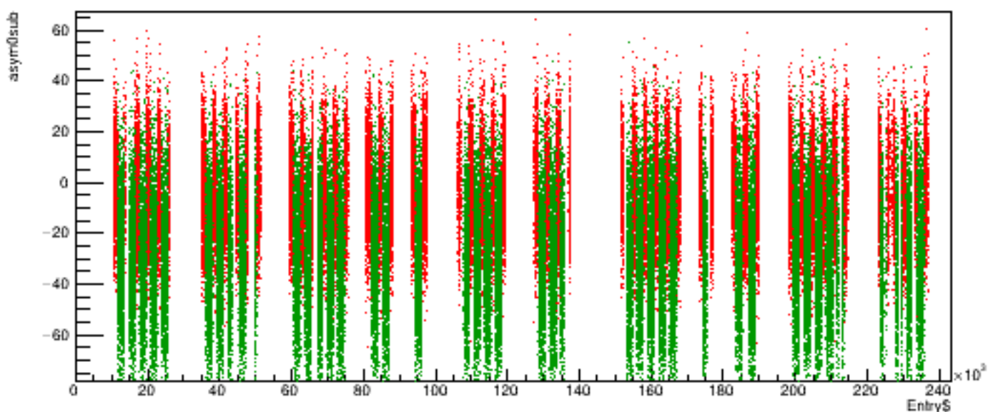
Run 6110 quartetwise, asym0sub vs time
