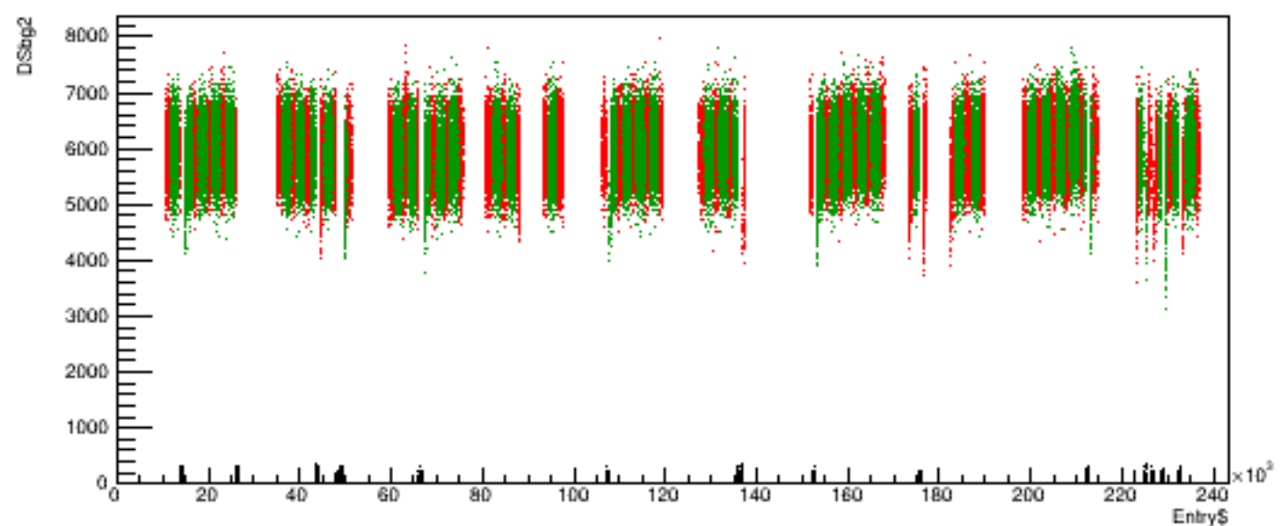
Run 6110 quartetwise, DSbg2 vs time
