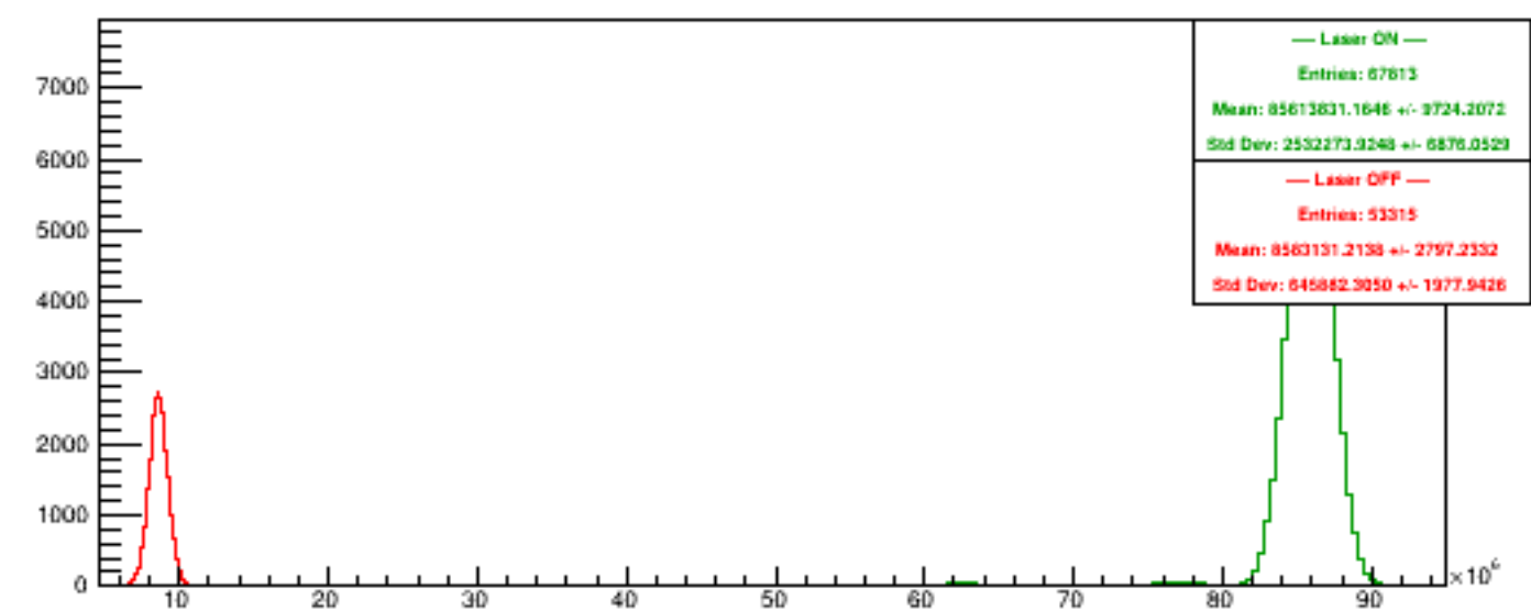
Run 6110 quartetwise, Sums4
