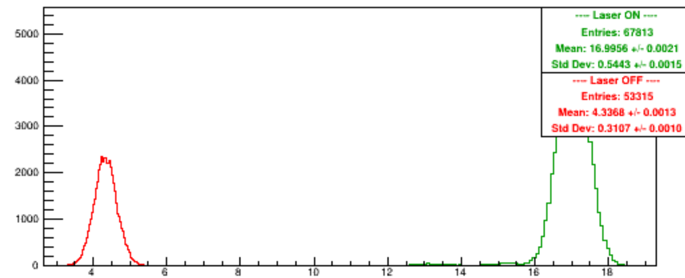
Run 6110 quartetwise, NegHelAcc0/NSamples0
