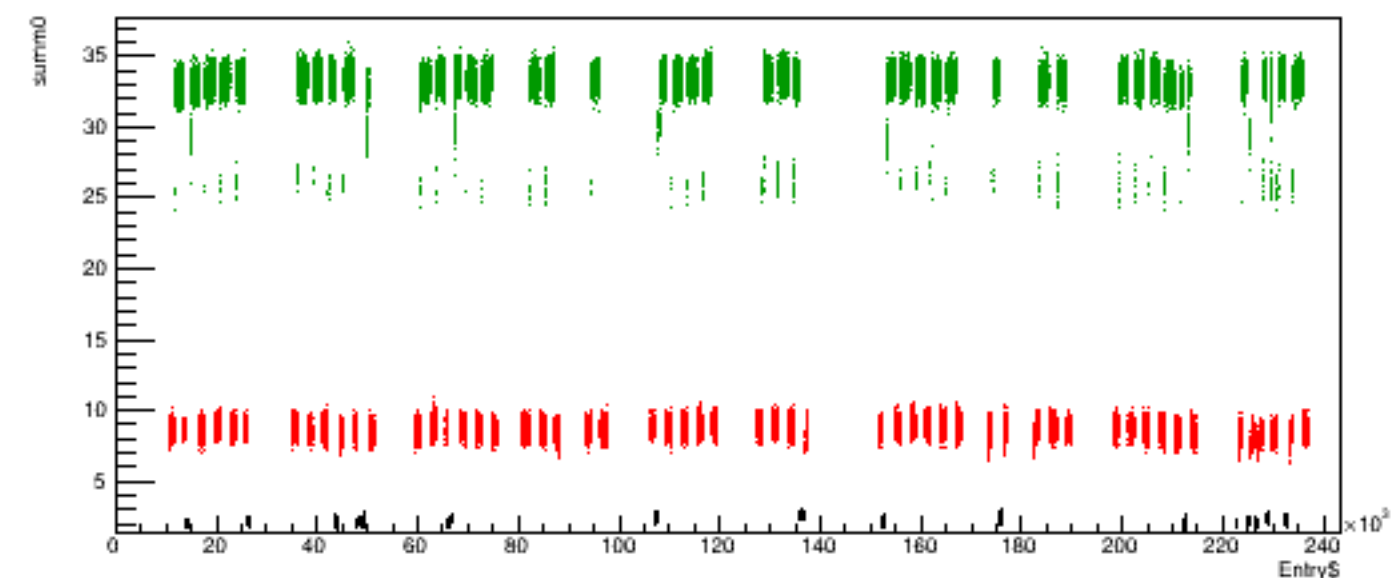
Run 6110 quartetwise, summ0 vs time
