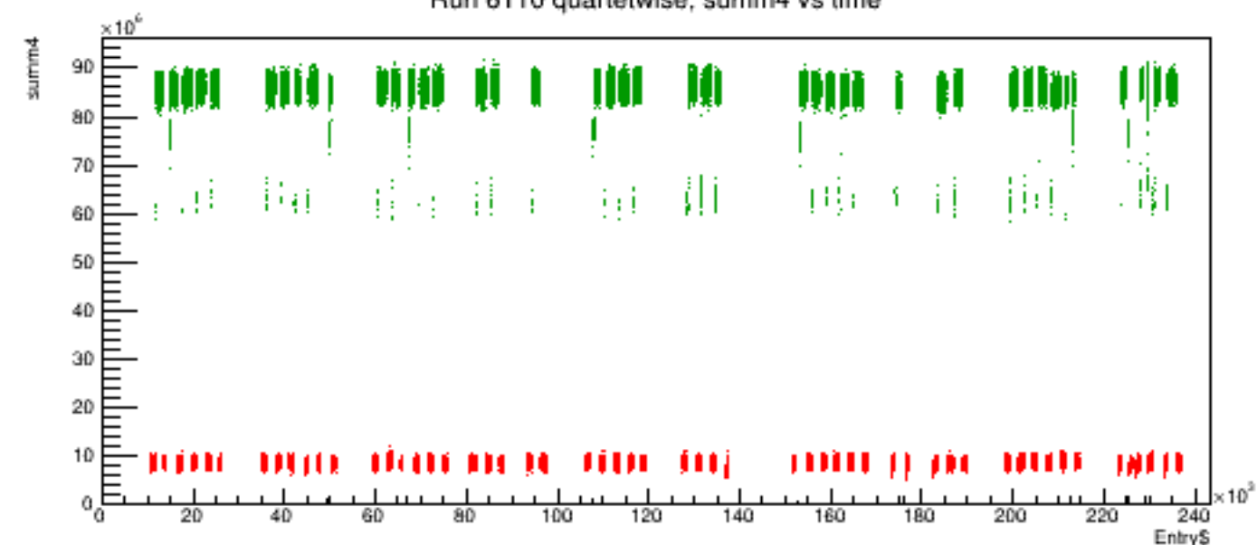
Run 6110 quartetwise, summ4 vs time
