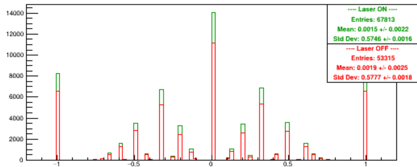
Run 6110 quartetwise, Asyms USbg1
