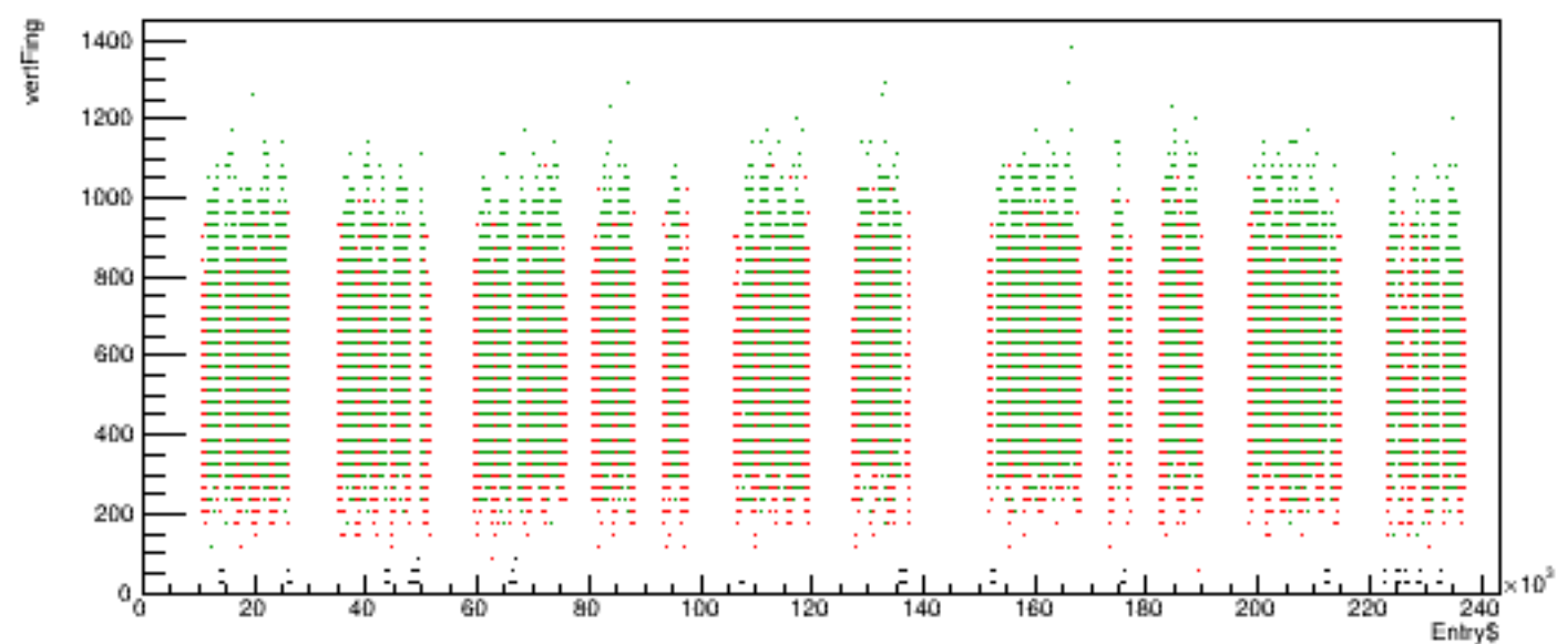
Run 6110 quartetwise, vertFing vs time
