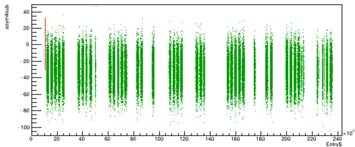
Run 6110 quartetwise, asym4sub vs time
