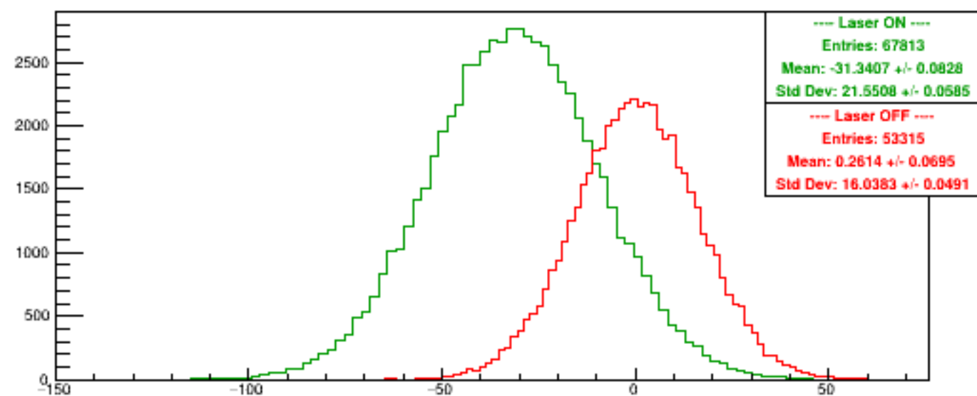
Run 6110 quartetwise, Asyms0
