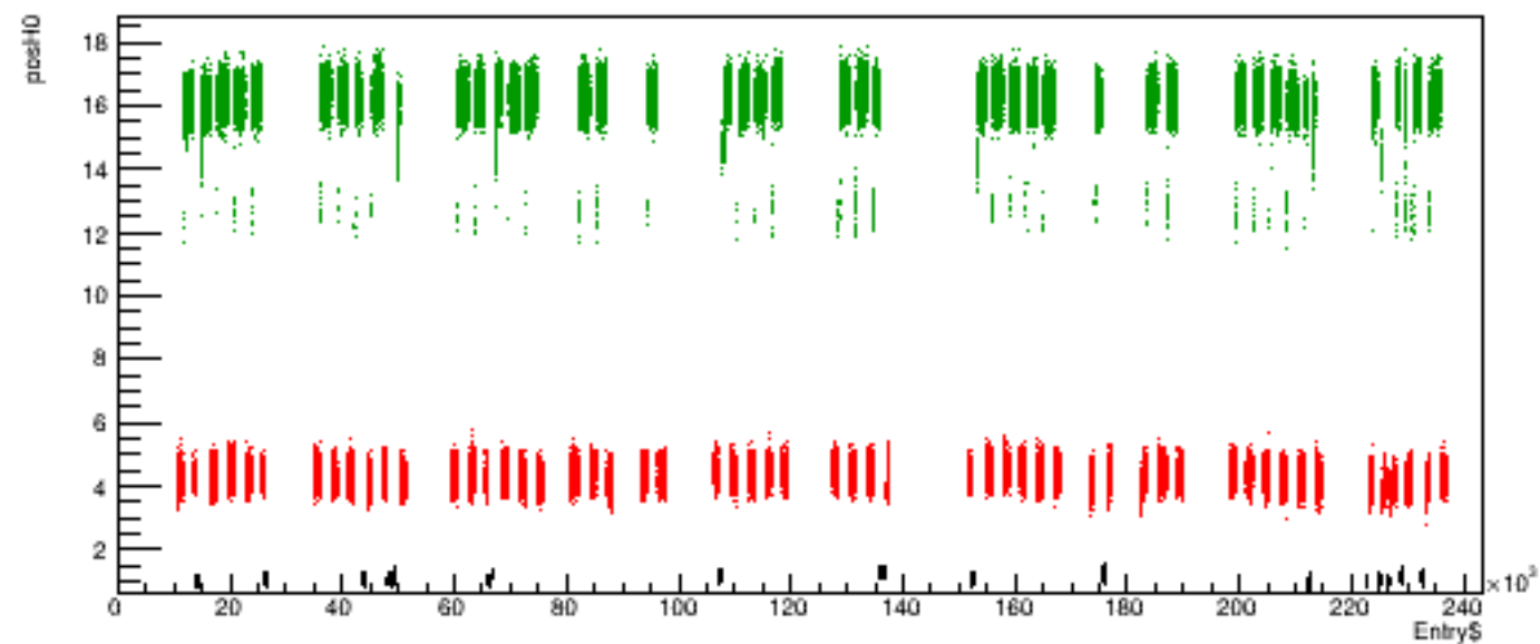
Run 6110 quartetwise, posH0 vs time
