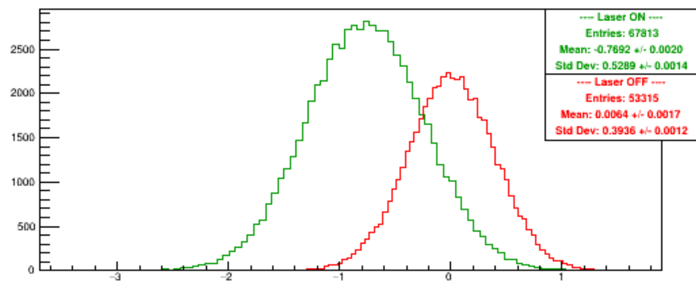
Run 6110 quartetwise, Diffs0
