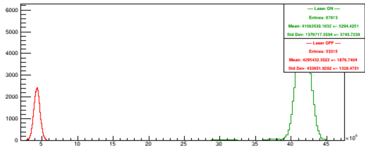
Run 6110 quartetwise, PosHelAcc4
