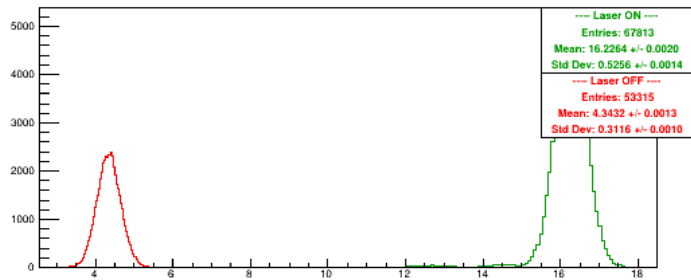
Run 6110 quartetwise, PosHelAcc0/NSamples0
