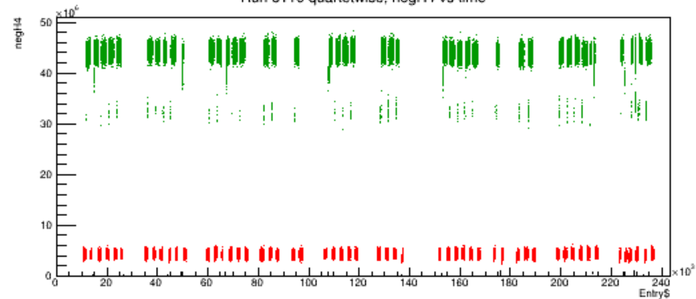
Run 6110 quartetwise, negH4 vs time
