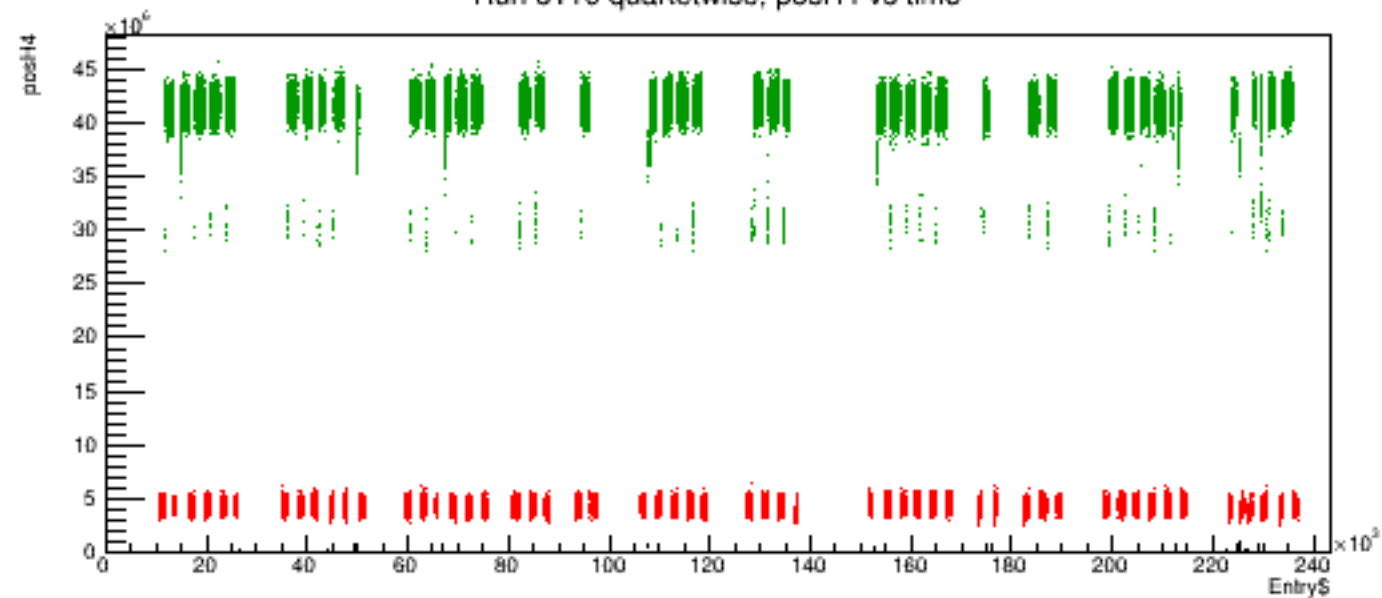
Run 6110 quartetwise, posH4 vs time
