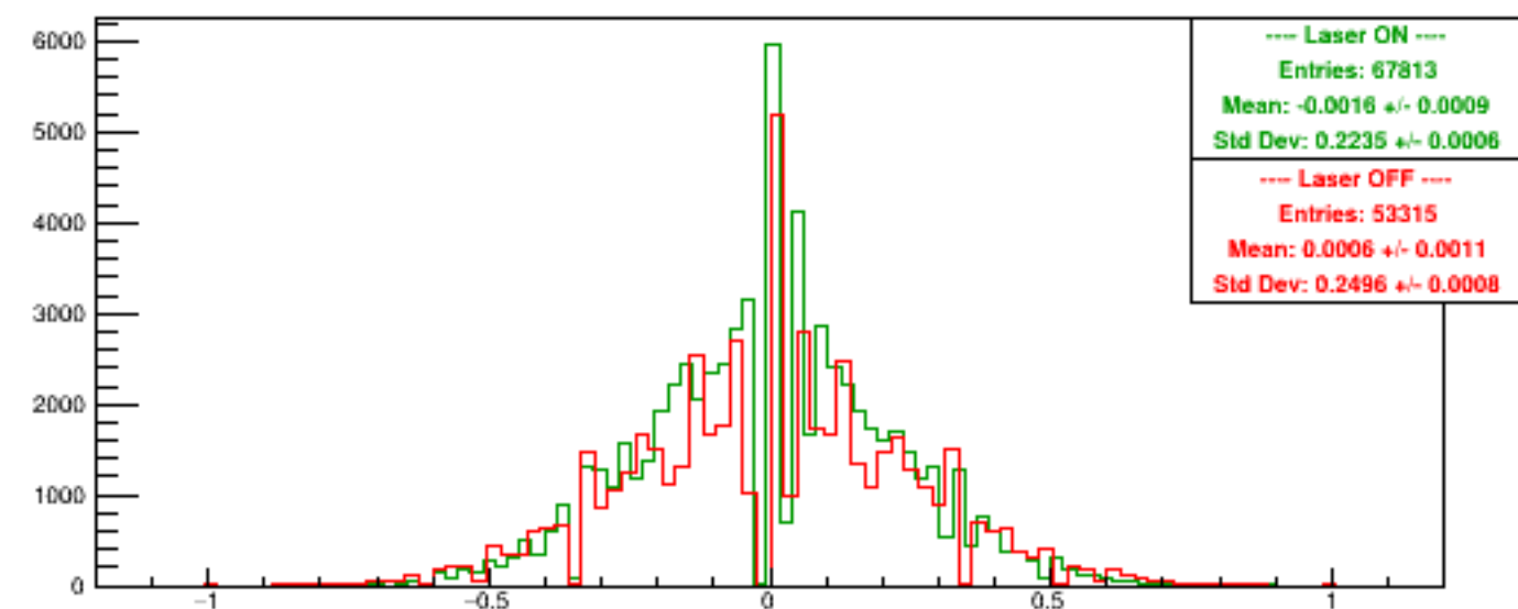
Run 6110 quartetwise, Asyms Horiz Finger
