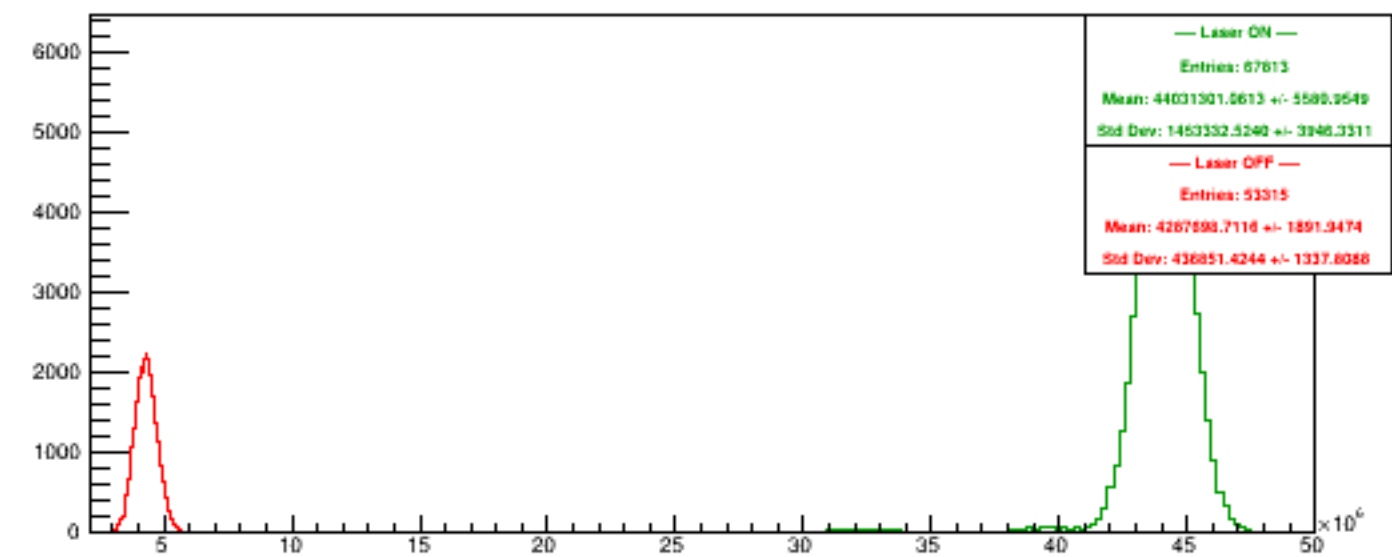
Run 6110 quartetwise, NegHelAcc4
