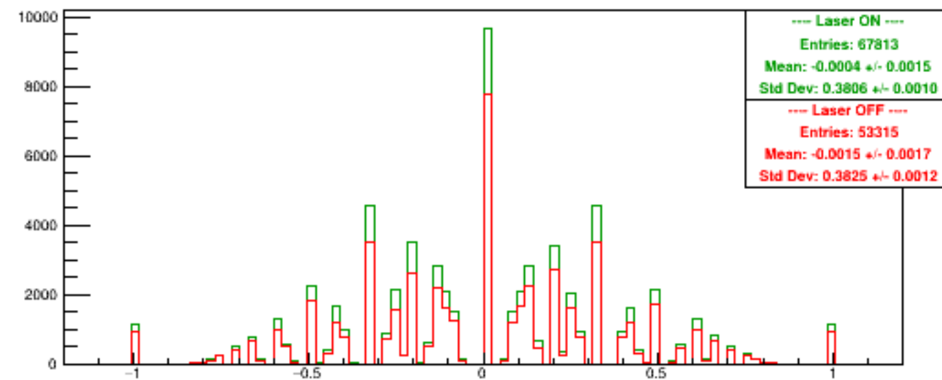
Run 6110 quartetwise, Asyms USbg2
