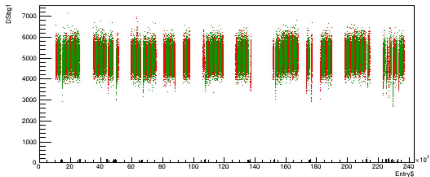
Run 6110 quartetwise, DSbg1 vs time
