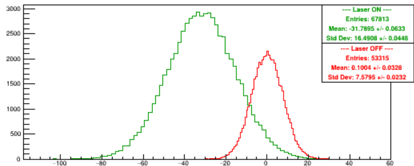
Run 6110 quartetwise, Asyms4
