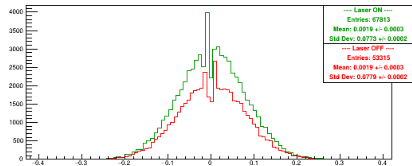
Run 6110 quartetwise, Asyms DSbg1
