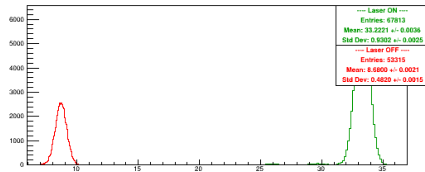
Run 6110 quartetwise, Sums0
