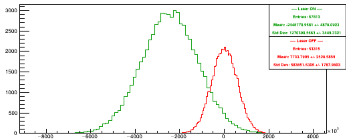
Run 6110 quartetwise, Diffs4
