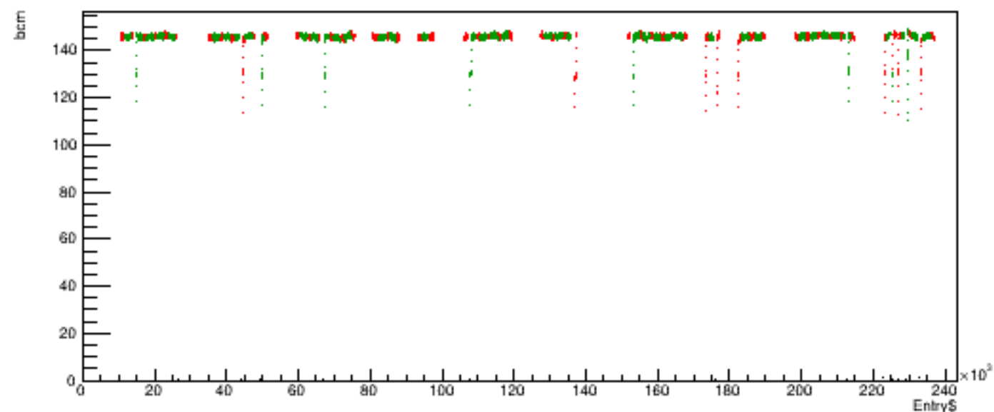
Run 6110 quartetwise, posH4 vs time
