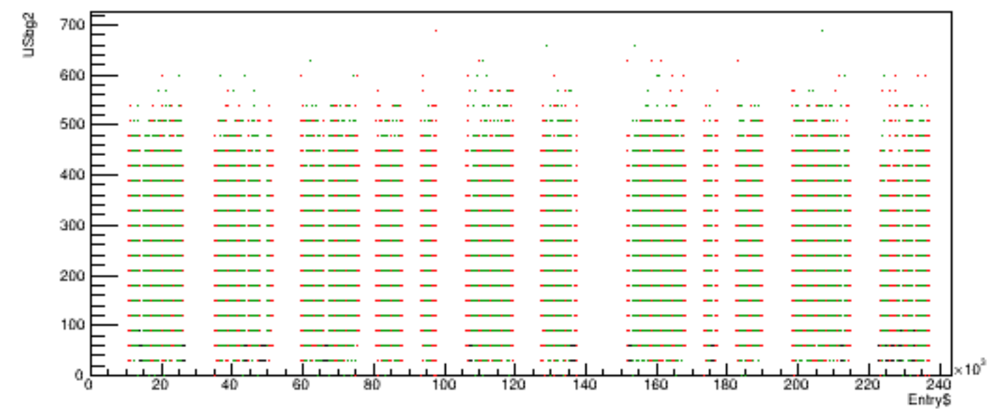
Run 6110 quartetwise, USbg2 vs time
