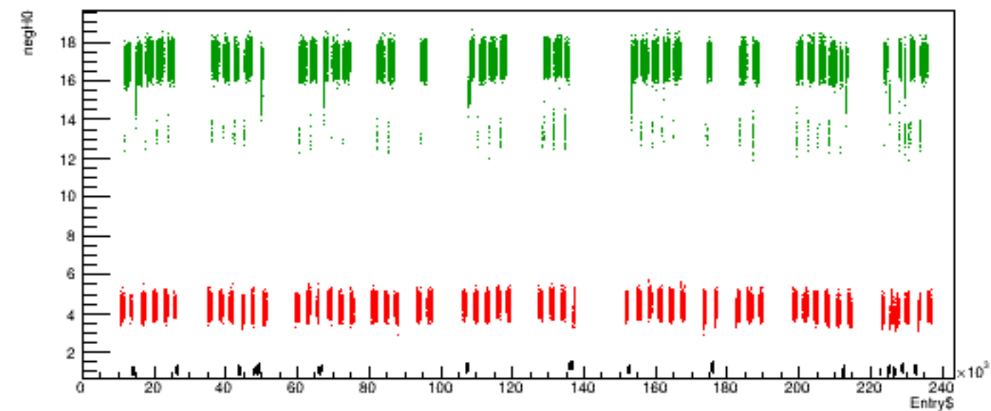
Run 6110 quartetwise, negH0 vs time
