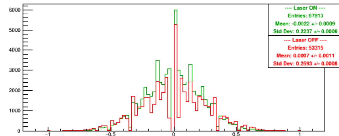
Run 6110 quartetwise, Asyms Vert Finger
