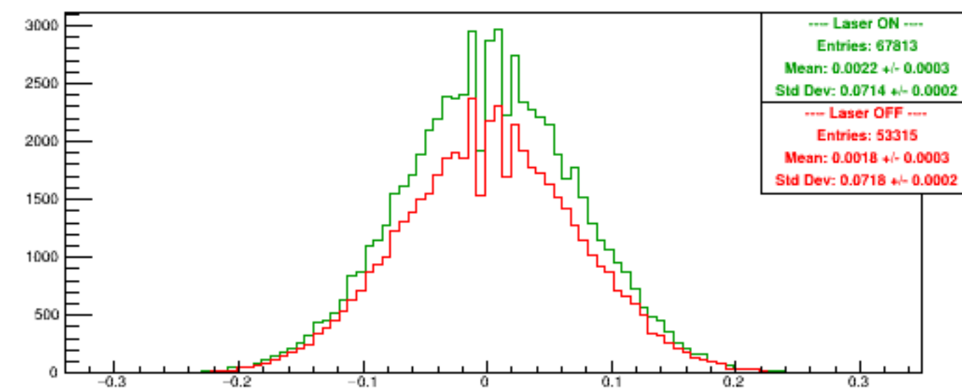
Run 6110 quartetwise, Asyms DSbg2
