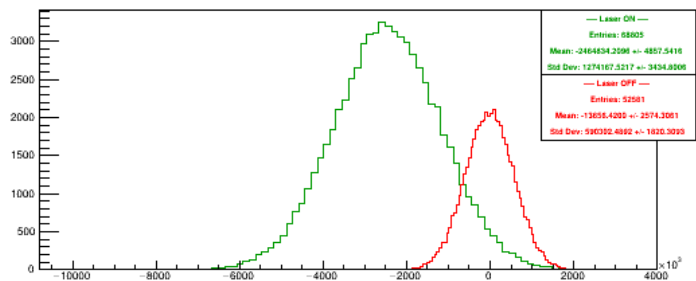
Run 6111 quartetwise, Diffs4
