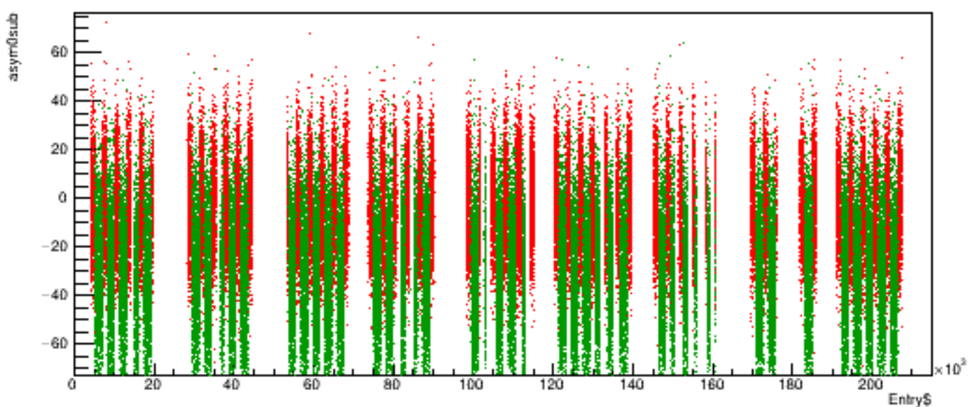
Run 6111 quartetwise, asym0sub vs time
