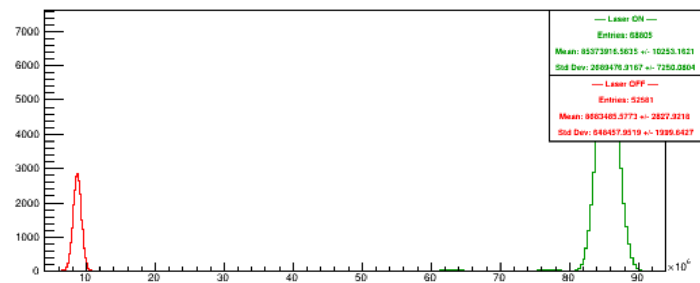
Run 6111 quartetwise, Sums4
