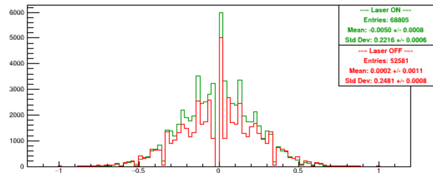
Run 6111 quartetwise, Asyms Horiz Finger
