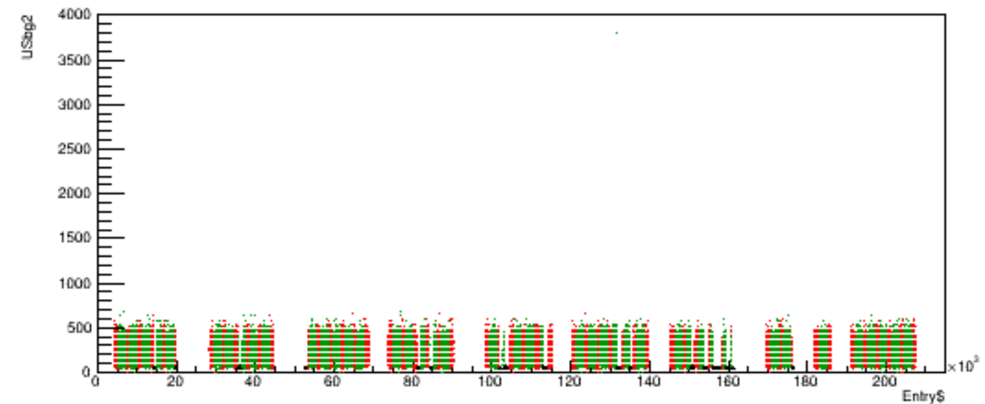
Run 6111 quartetwise, USbg2 vs time
