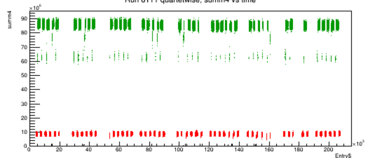
Run 6111 quartetwise, summ4 vs time
