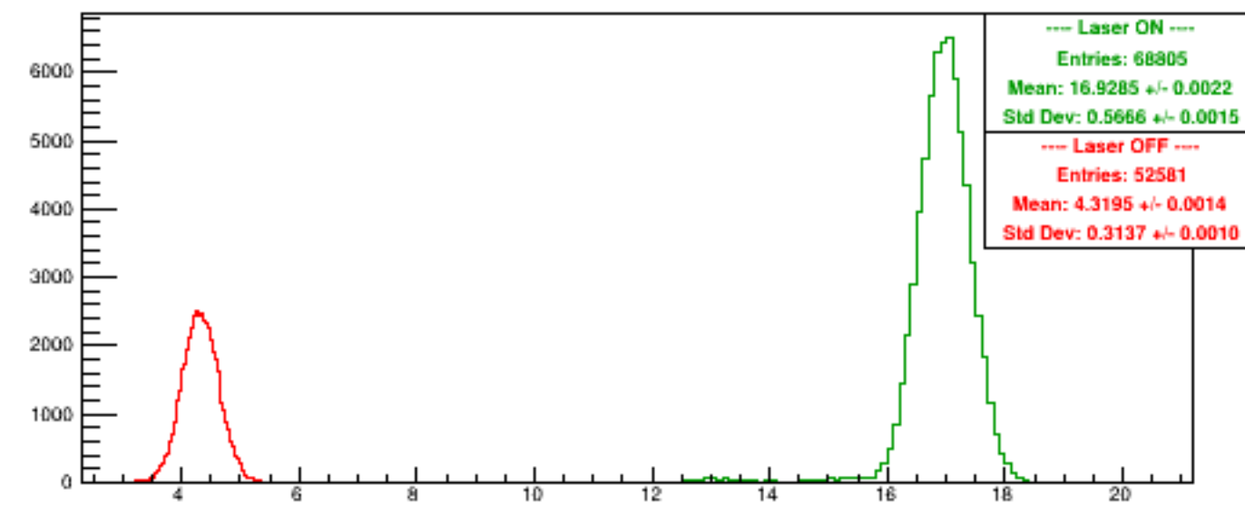
Run 6111 quartetwise, NegHelAcc0/NSamples0
