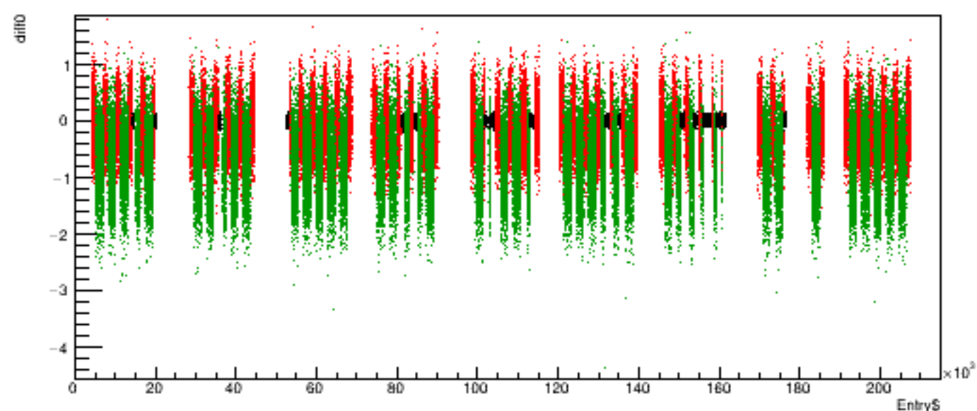
Run 6111 quartetwise, diff0 vs time
