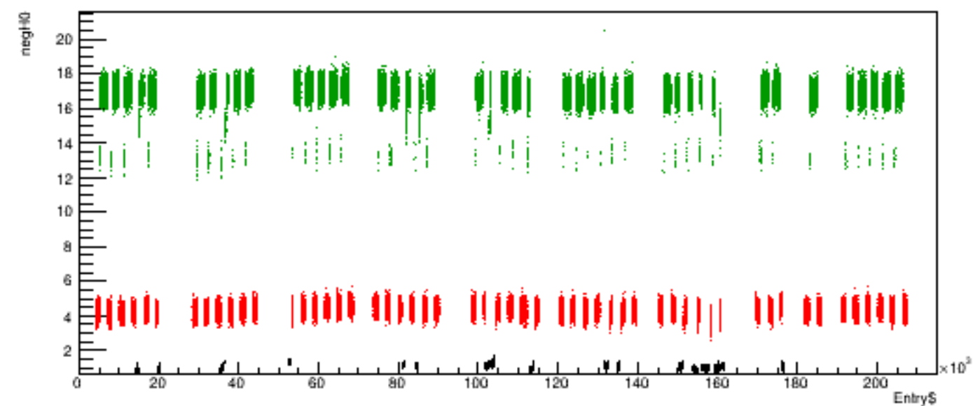
Run 6111 quartetwise, negH0 vs time
