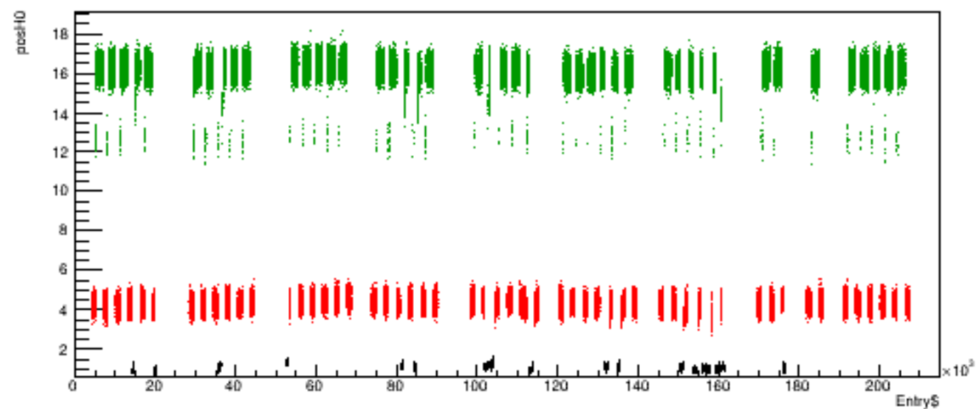
Run 6111 quartetwise, posH0 vs time
