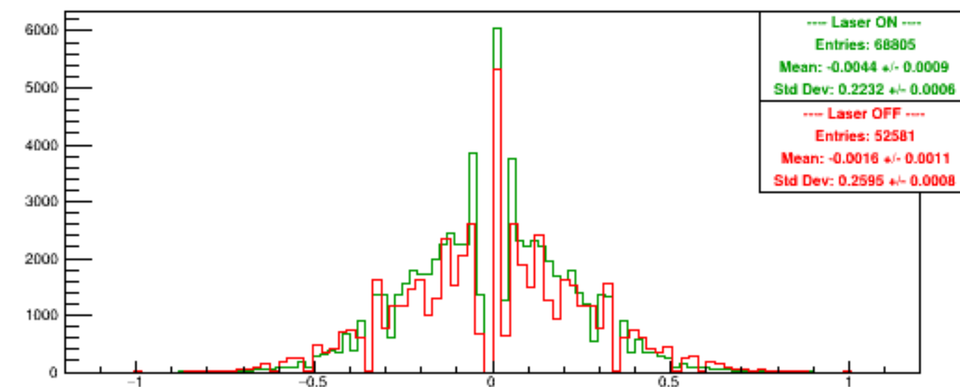
Run 6111 quartetwise, Asyms Vert Finger
