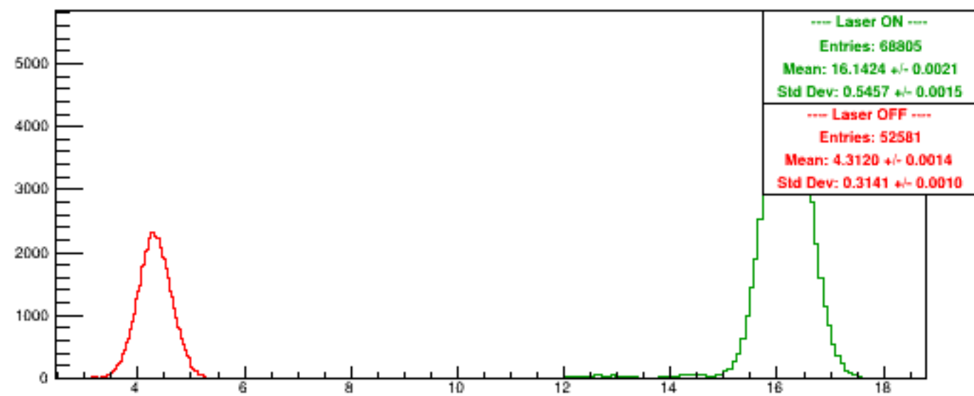
Run 6111 quartetwise, PosHelAcc0/NSamples0
