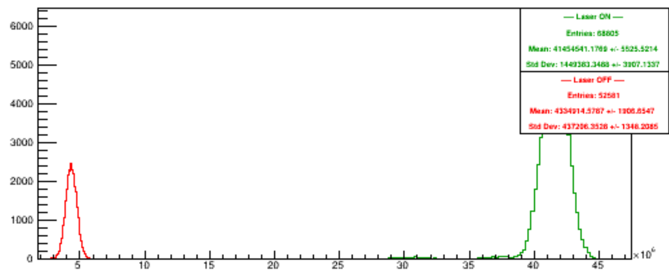
Run 6111 quartetwise, PosHelAcc4
