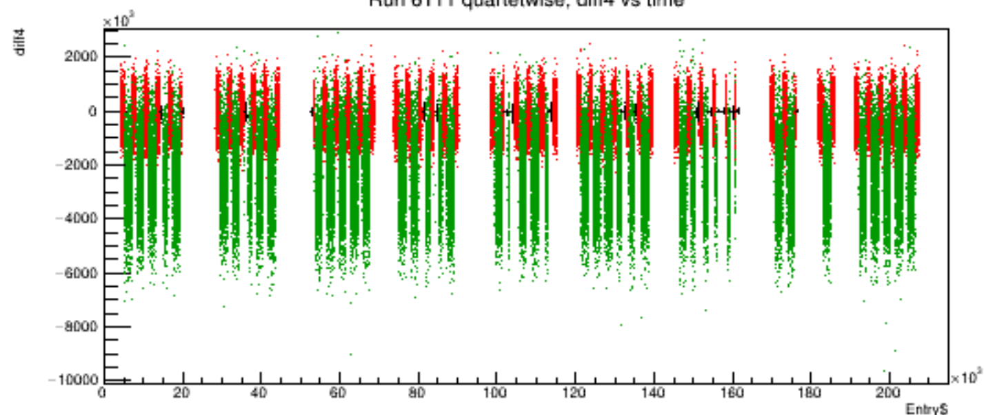
Run 6111 quartetwise, diff4 vs time
