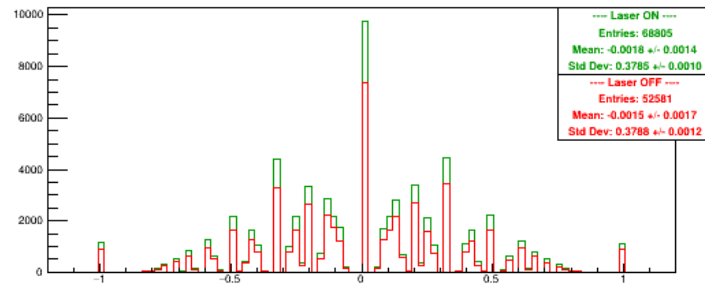
Run 6111 quartetwise, Asyms USbg2
