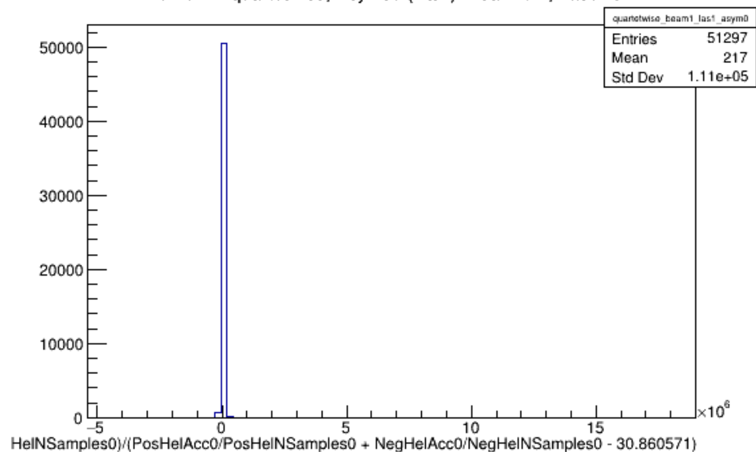
Run 6124 quartetwise, Asyms0 (Raw): Beam ON, Laser ON
