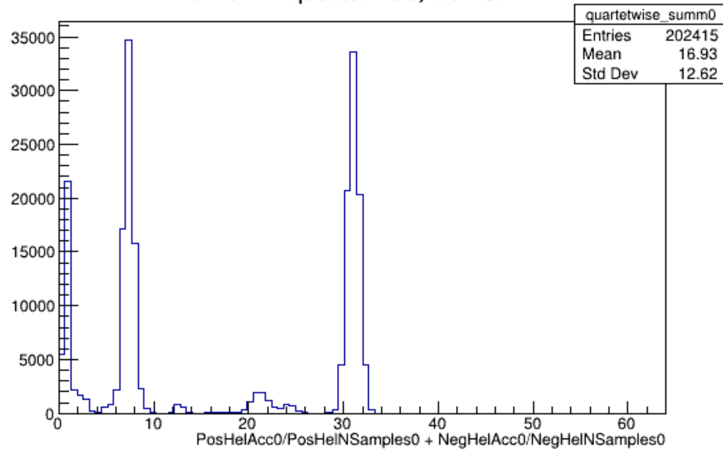
Run 6124 quartetwise, Sums0: All
