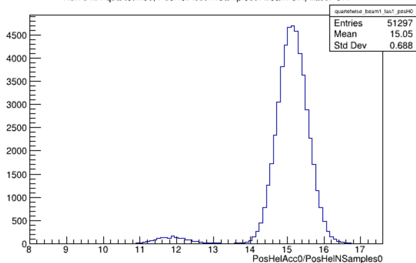
Run 6124 quartetwise, PosHelAcc0/NSamples0: Beam ON, Laser ON
