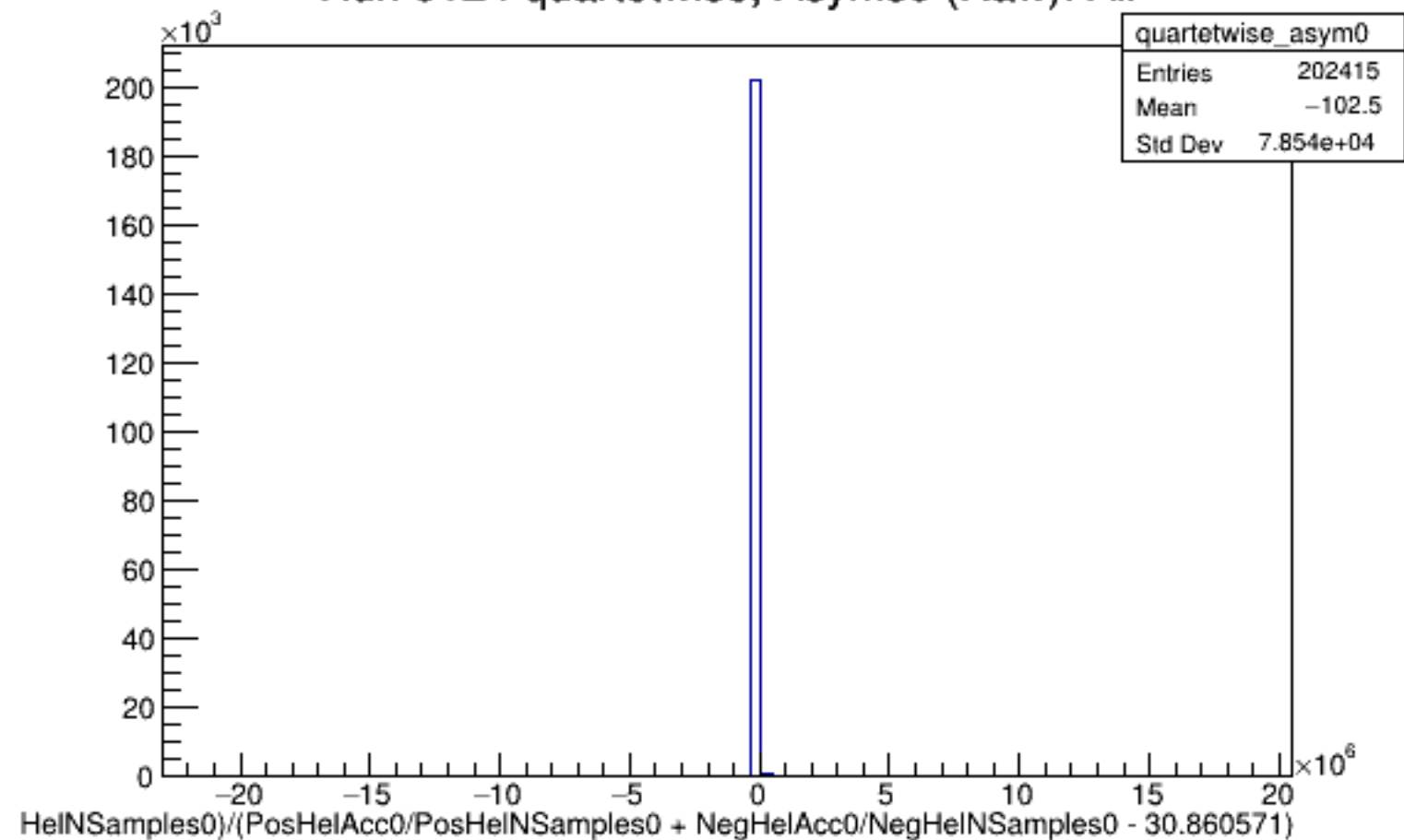
Run 6124 quartetwise, Asyms0 (Raw): All
