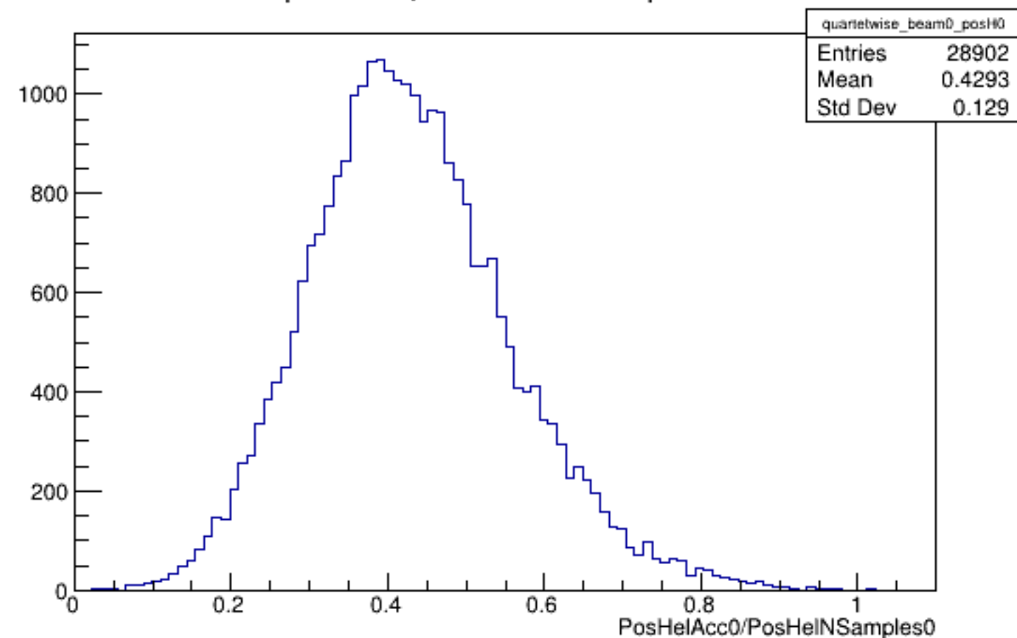
Run 6124 quartetwise, PosHelAcc0/NSamples0: Beam OFF
