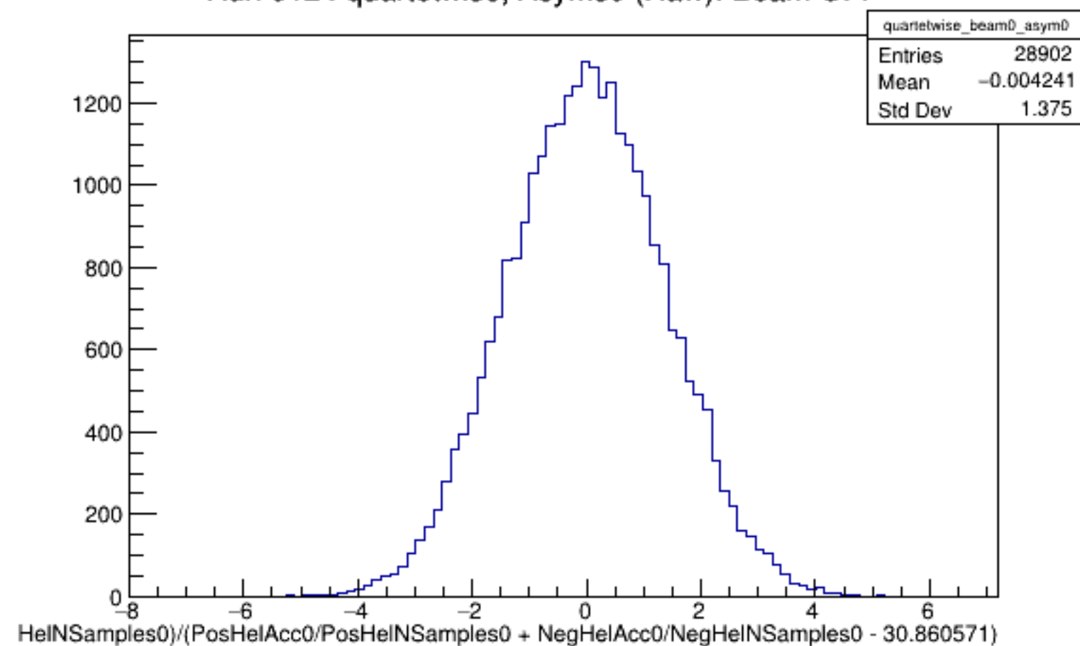
Run 6124 quartetwise, Asyms0 (Raw): Beam OFF
