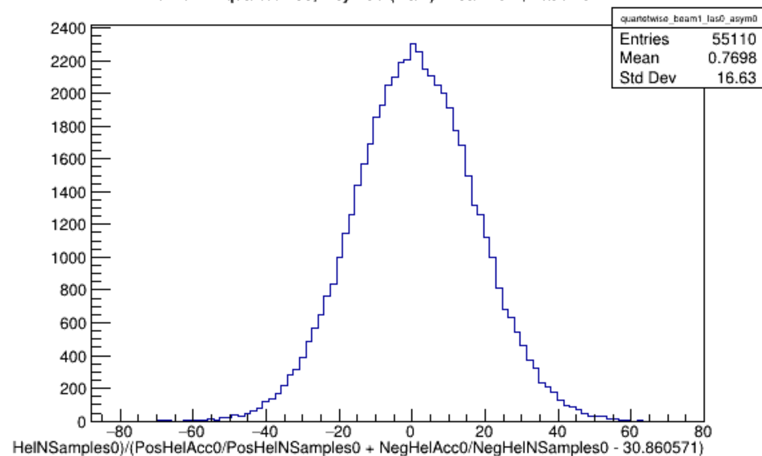
Run 6124 quartetwise, Asyms0 (Raw): Beam ON, Laser OFF
