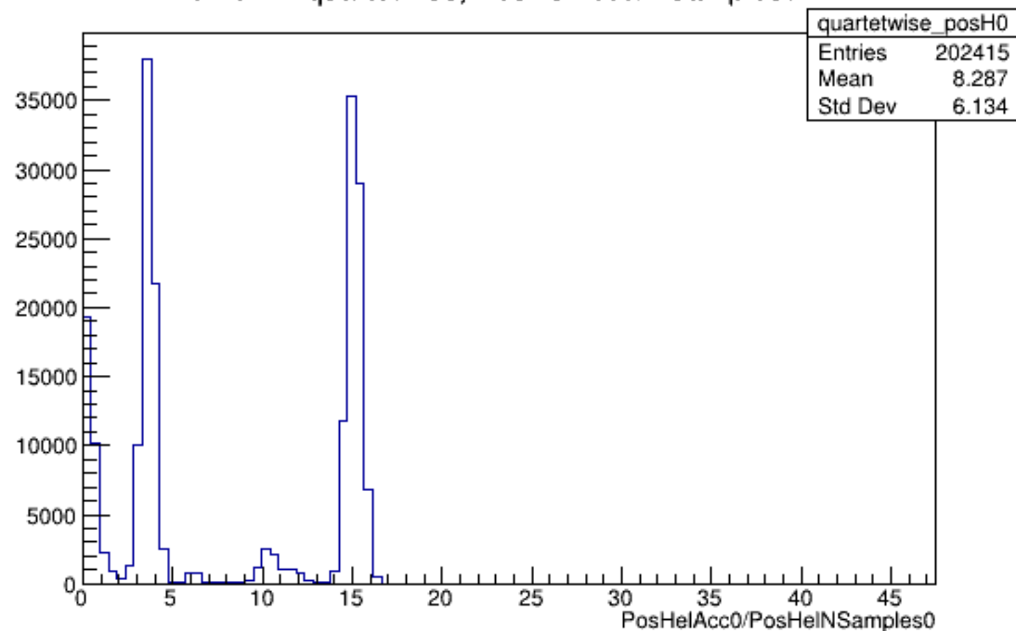
Run 6124 quartetwise, PosHelAcc0/NSamples0: All
