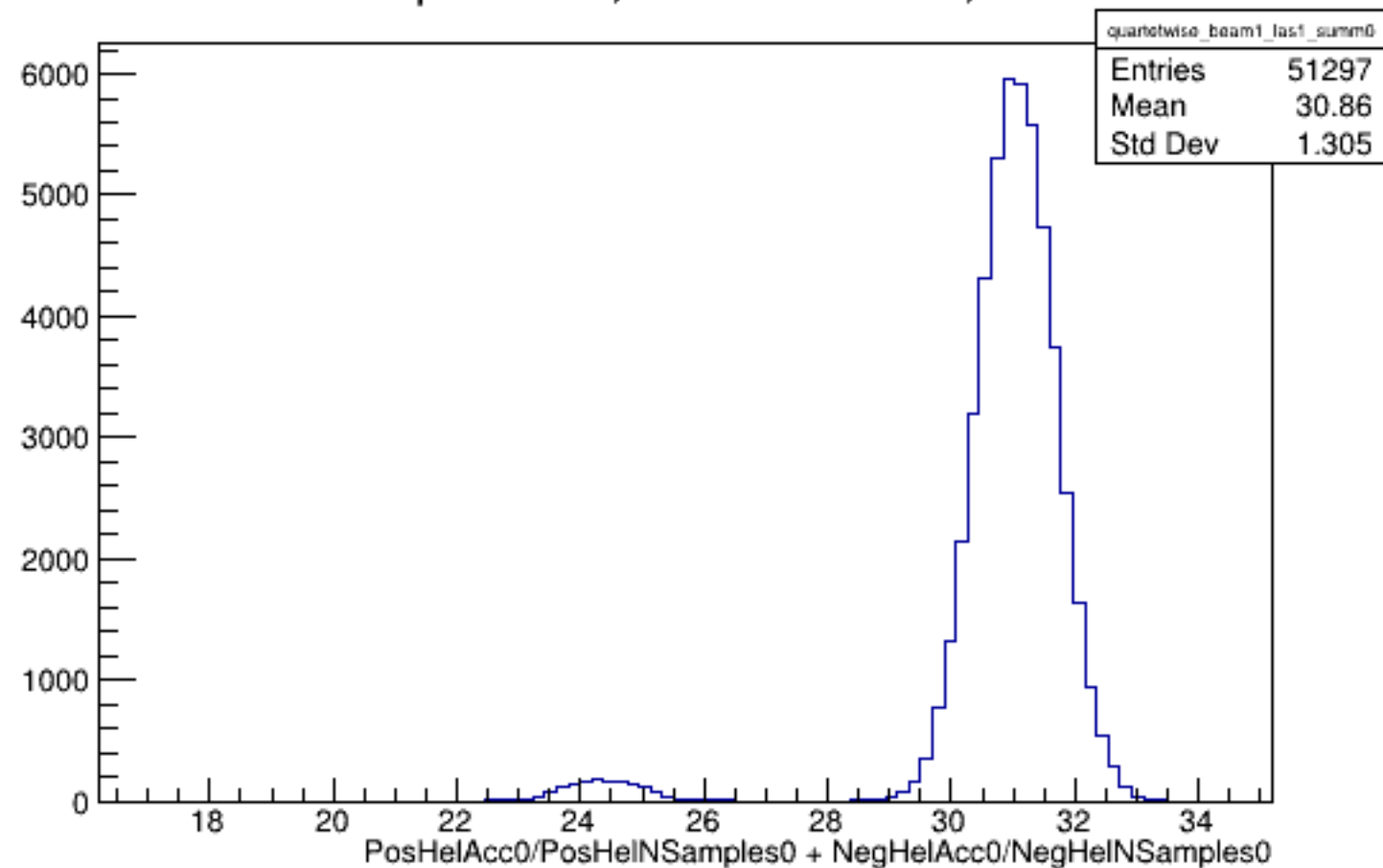
Run 6124 quartetwise, Sums0: Beam ON, Laser ON
