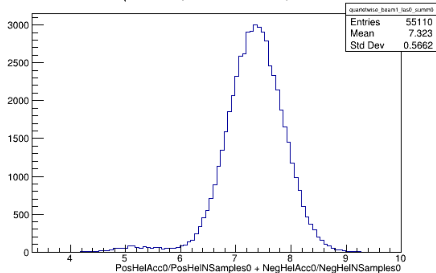
Run 6124 quartetwise, Sums0: Beam ON, Laser OFF
