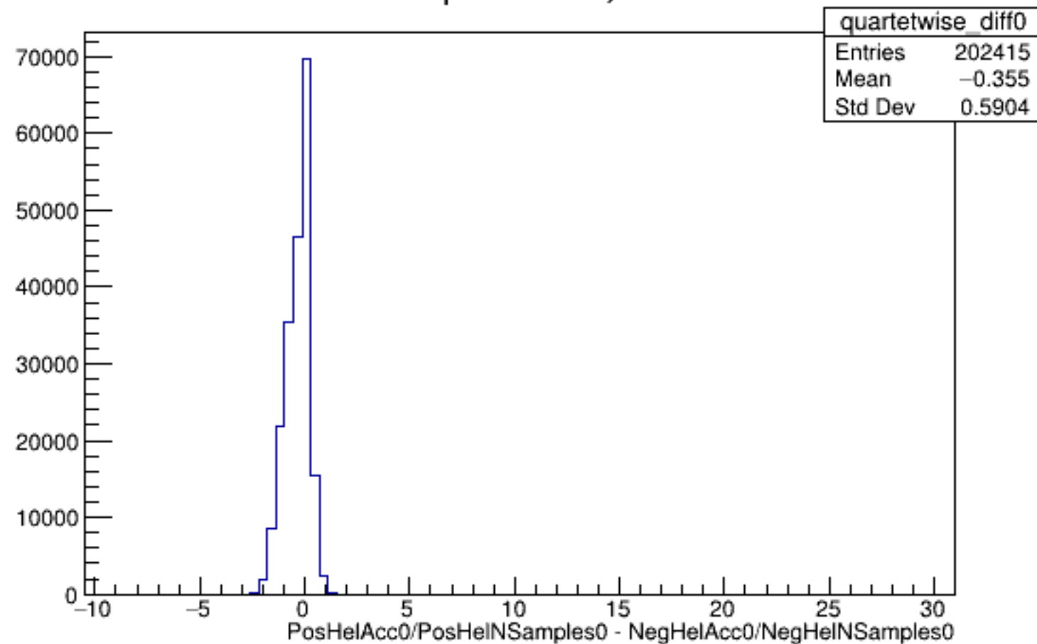
Run 6124 quartetwise, Diffs0: All
