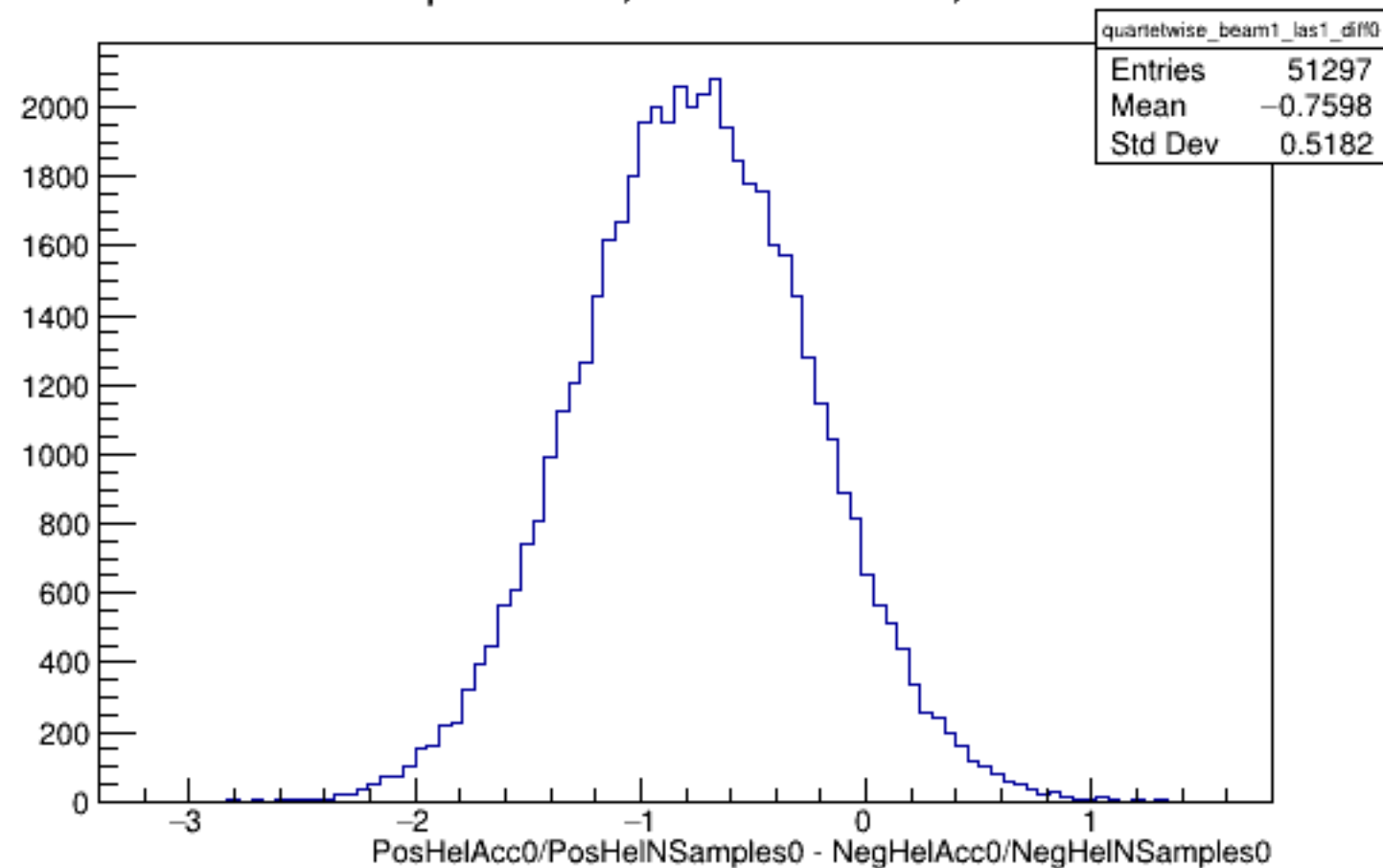
Run 6124 quartetwise, Diffs0: Beam ON, Laser ON
