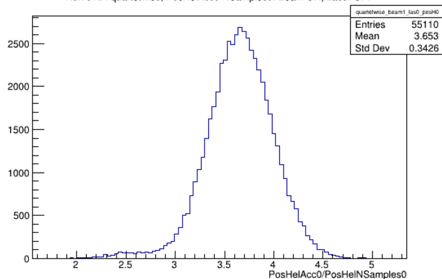
Run 6124 quartetwise, PosHelAcc0/NSamples0: Beam ON, Laser OFF
