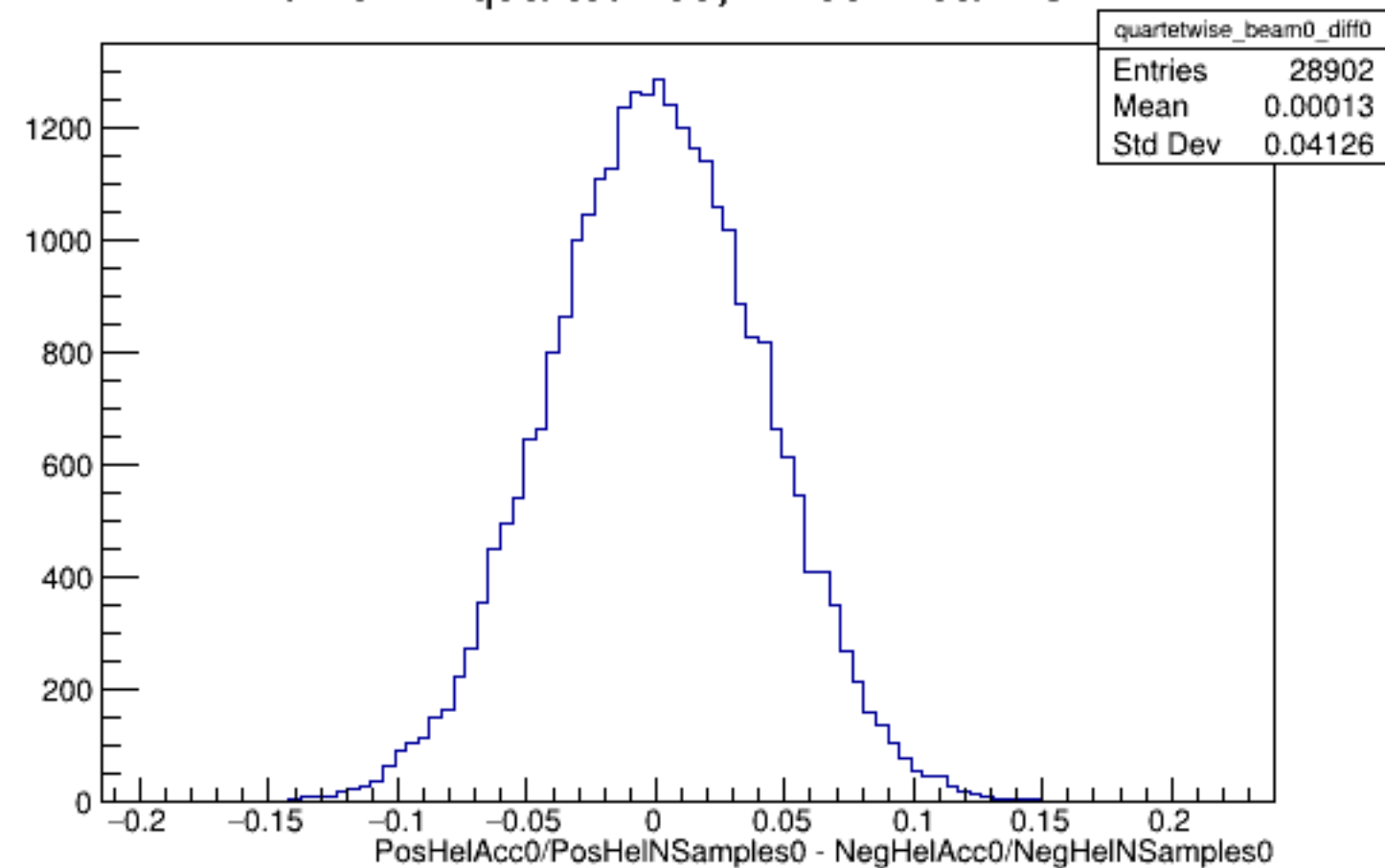
Run 6124 quartetwise, Diffs0: Beam OFF
