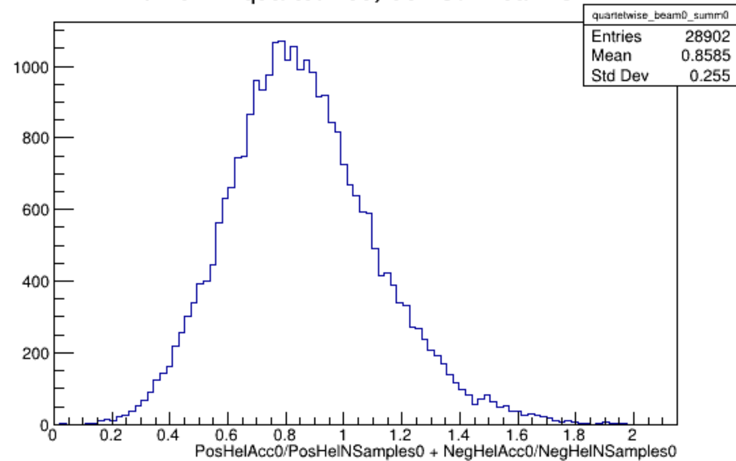
Run 6124 quartetwise, Sums0: Beam OFF
