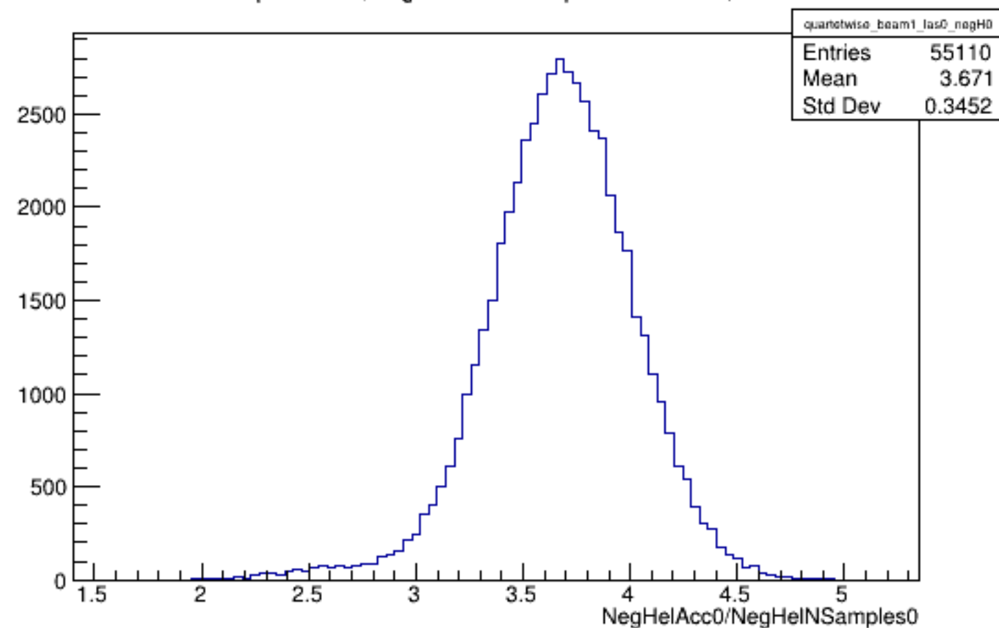
Run 6124 quartetwise, NegHelAcc0/NSamples0: Beam ON, Laser OFF
