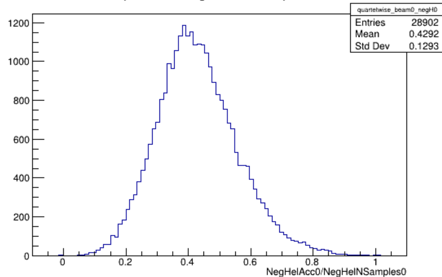
Run 6124 quartetwise, NegHelAcc0/NSamples0: Beam OFF
