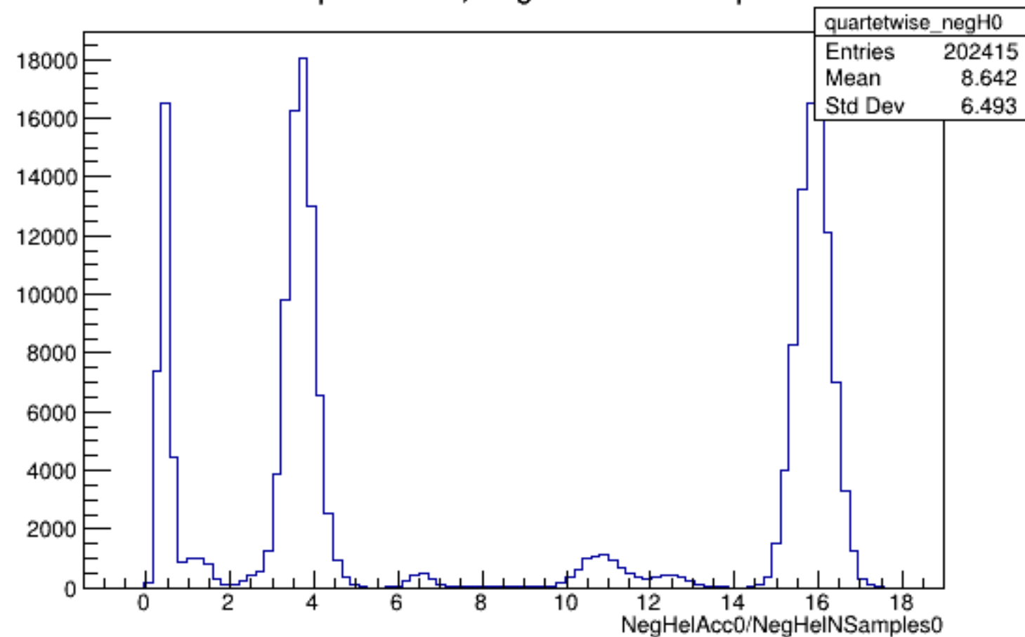
Run 6124 quartetwise, NegHelAcc0/NSamples0: All
