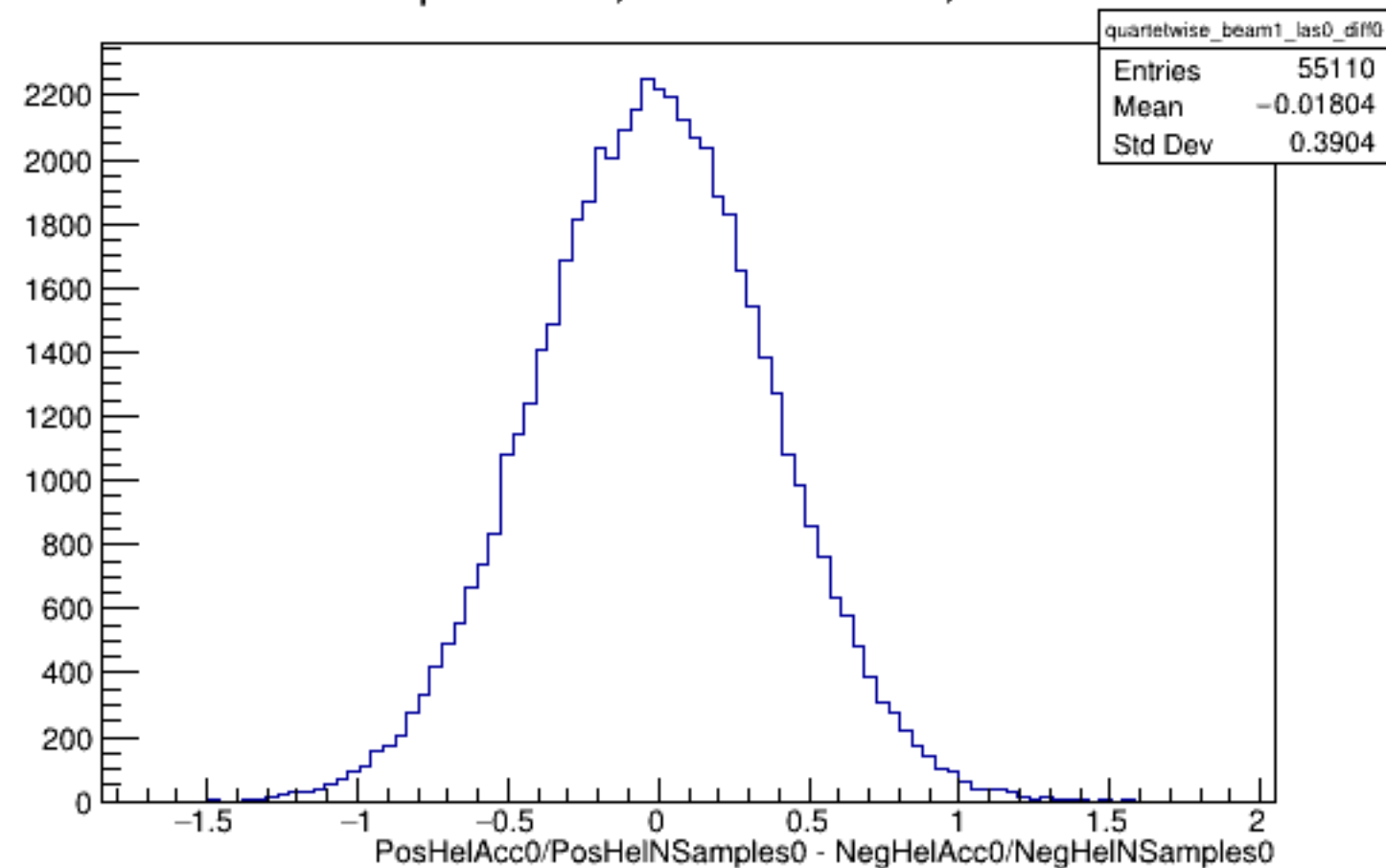
Run 6124 quartetwise, Diffs0: Beam ON, Laser OFF
