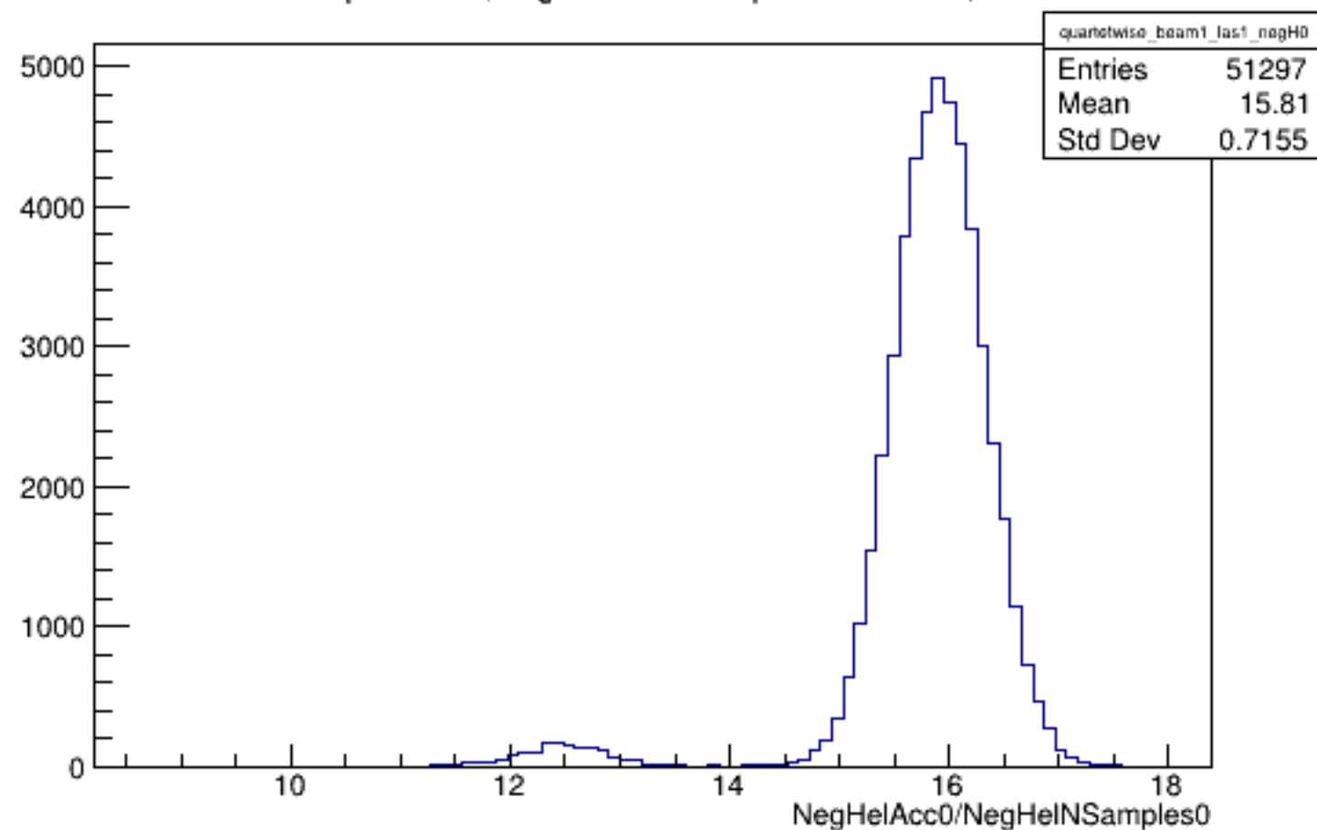
Run 6124 quartetwise, NegHelAcc0/NSamples0: Beam ON, Laser ON
