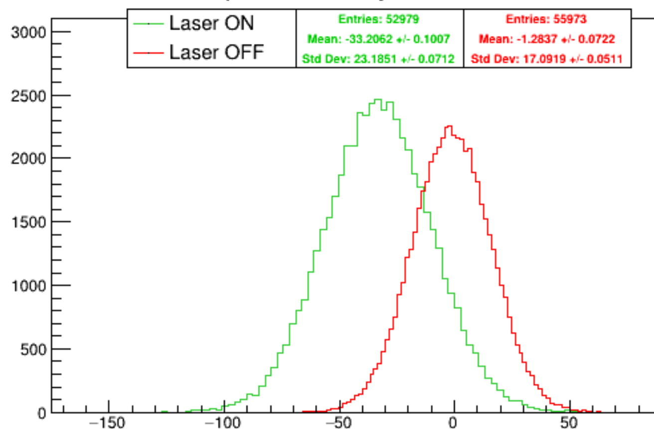
Run 6125 quartetwise, asym0sub: Beam ON
