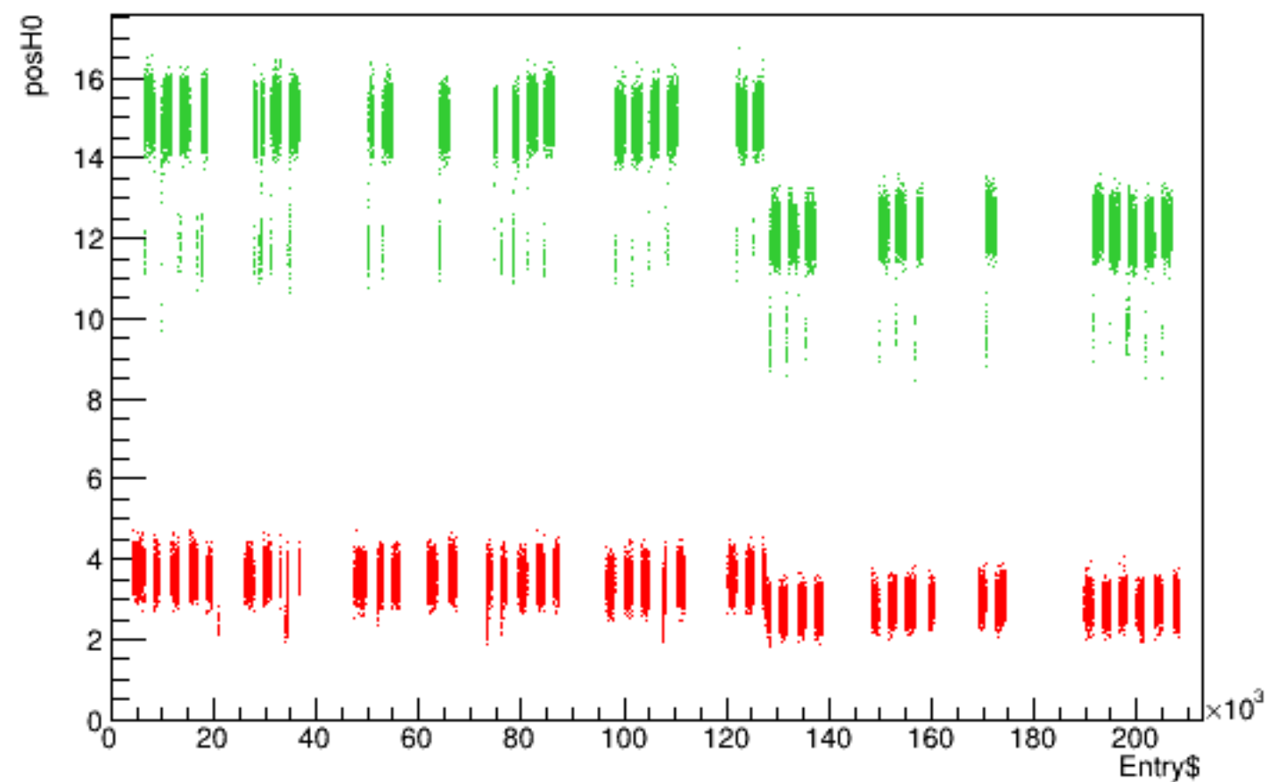
Run 6125 quartetwise, posH0 vs time
