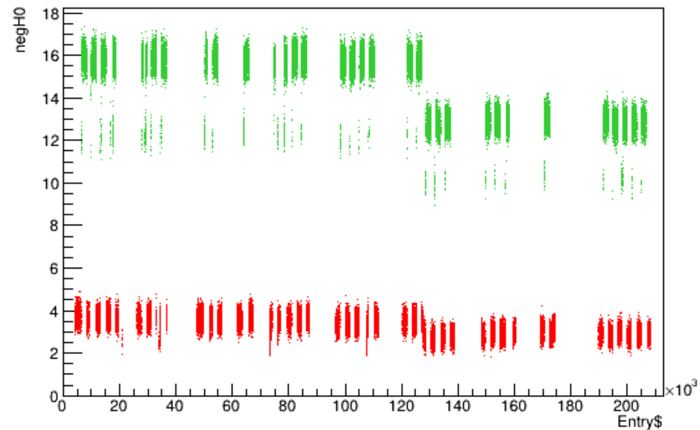
Run 6125 quartetwise, negH0 vs time
