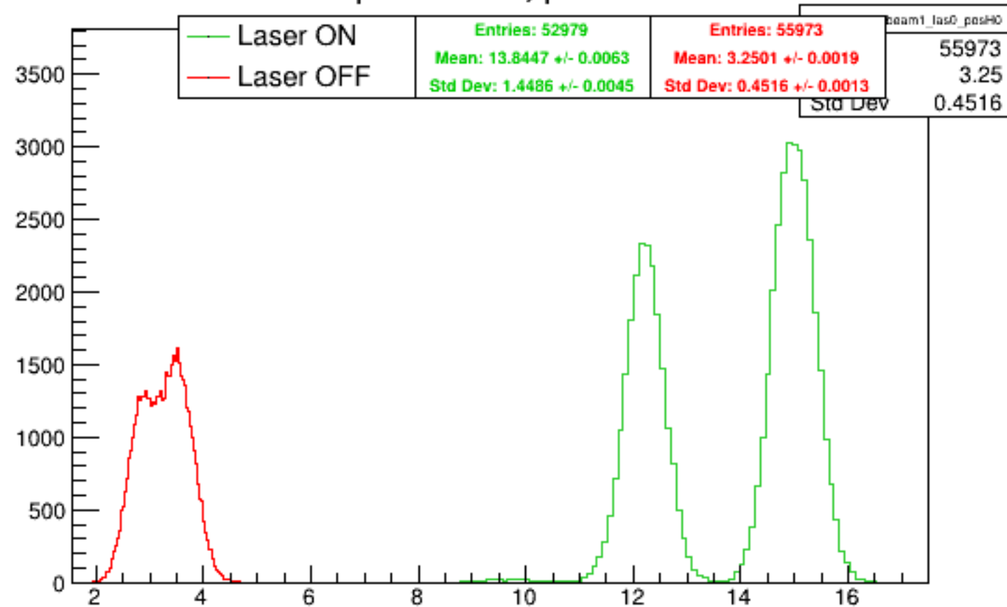
Run 6125 quartetwise, posH0: Beam ON
