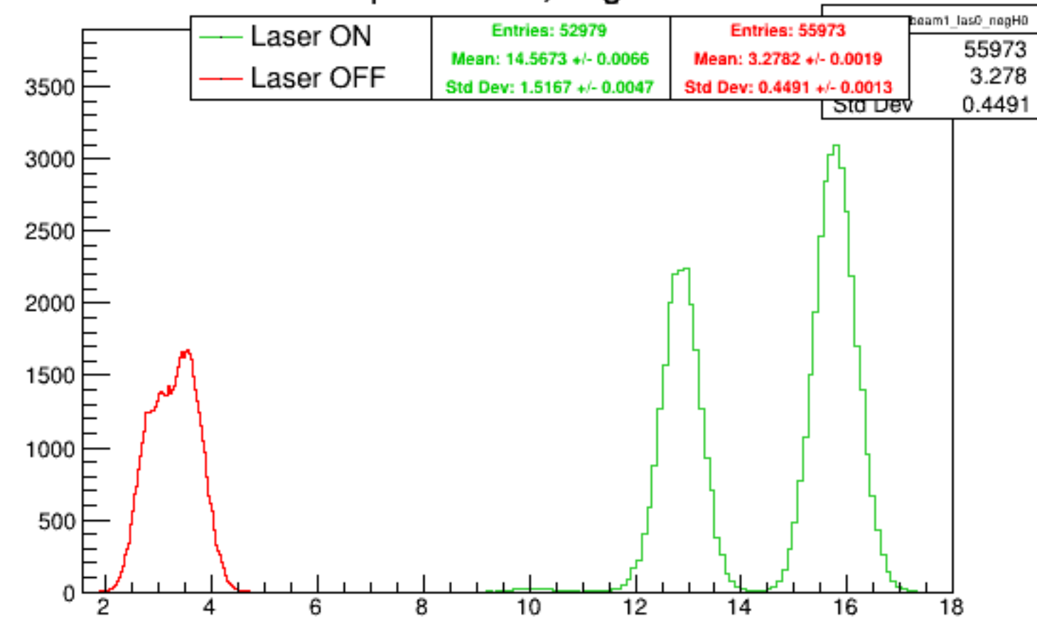
Run 6125 quartetwise, negH0: Beam ON
