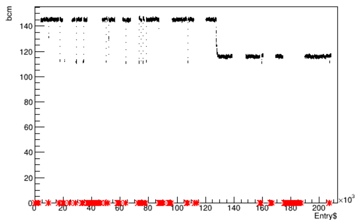
Run 6125 quartetwise, bcm vs time
