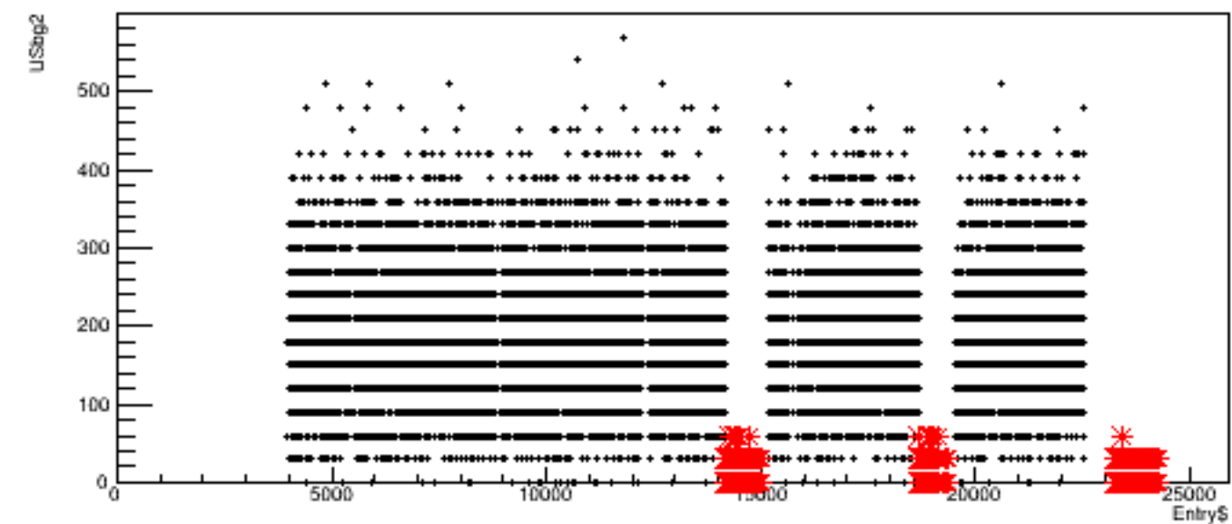
Run 6126, quartetwise: USbg2 vs time
