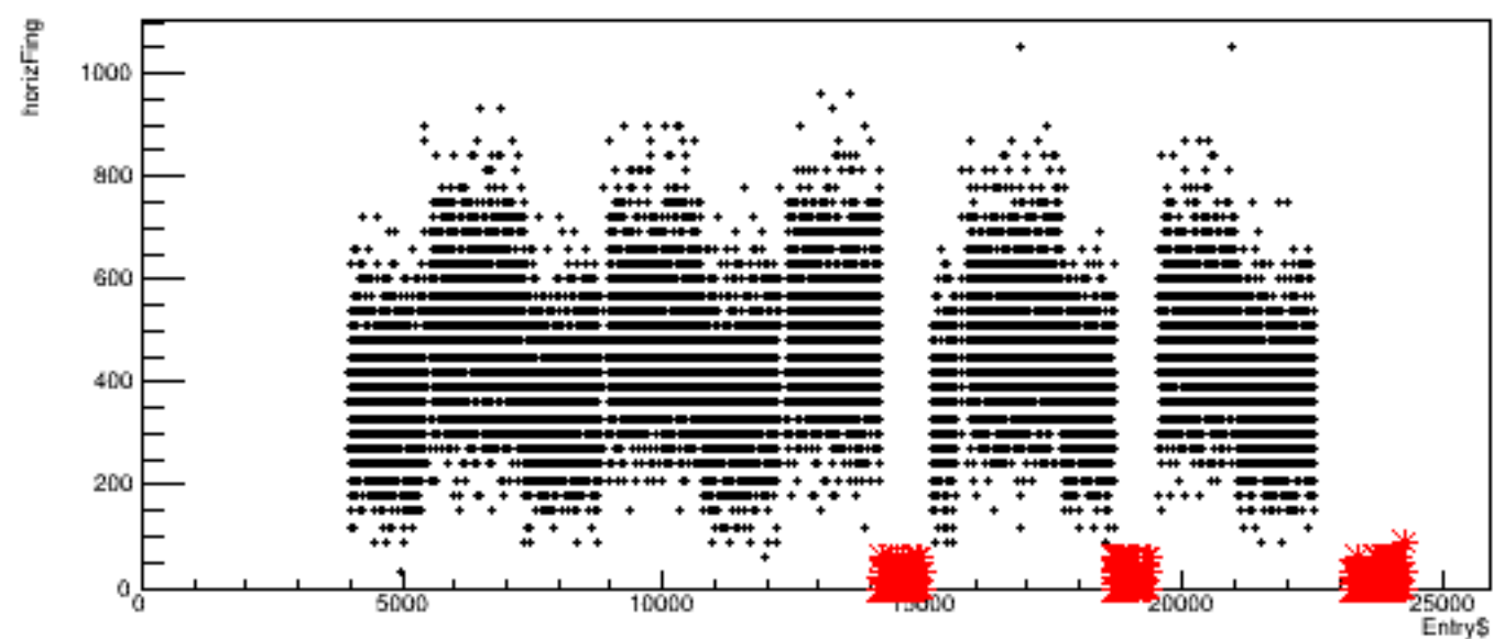
Run 6126, quartetwise: horizFing vs time
