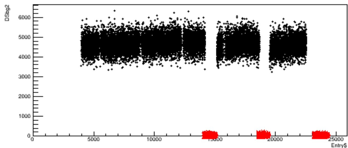
Run 6126, quartetwise: DSbg2 vs time
