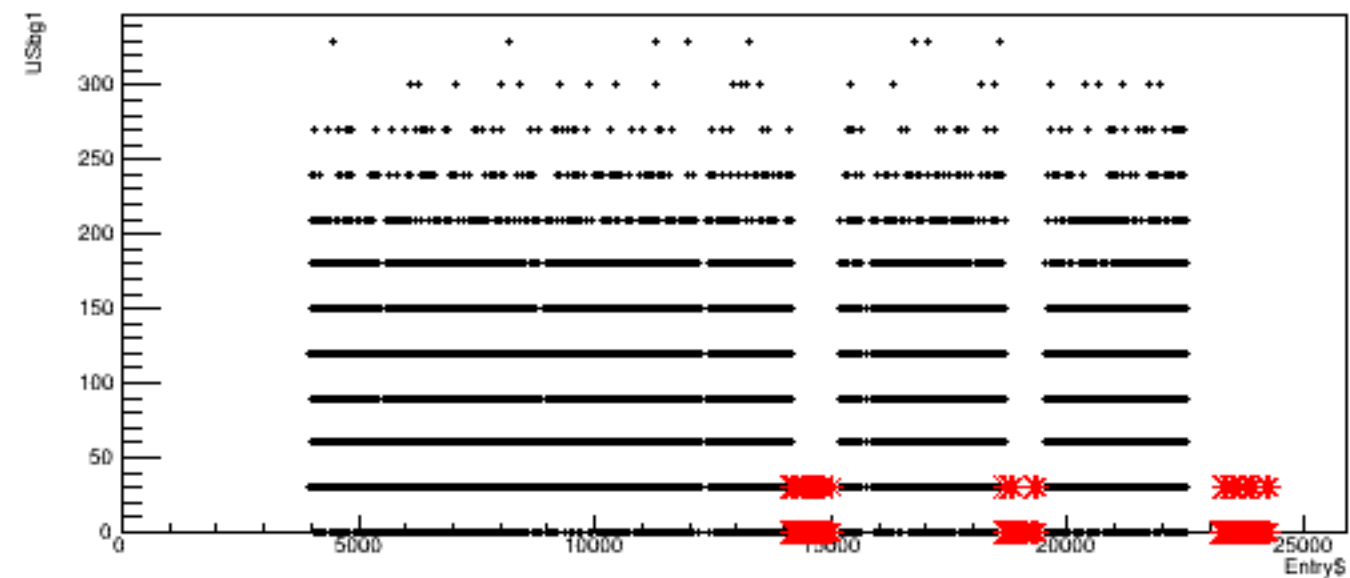
Run 6126, quartetwise: USbg1 vs time
