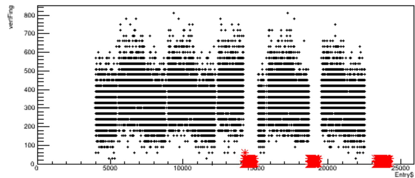
Run 6126, quartetwise: vertFing vs time
