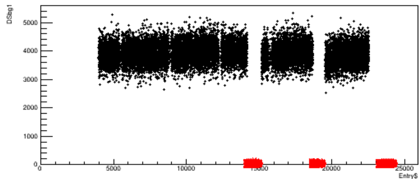
Run 6126, quartetwise: DSbg1 vs time
