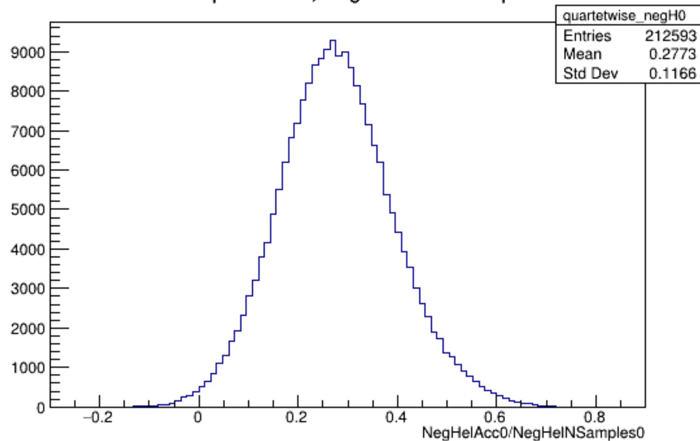
Run 6128 quartetwise, NegHelAcc0/NSamples0: All
