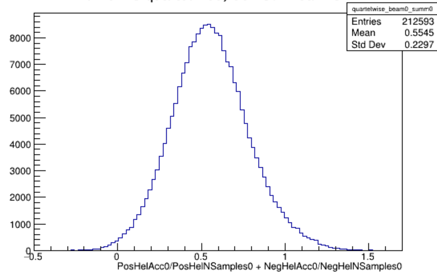
Run 6128 quartetwise, Sums0: Beam OFF
