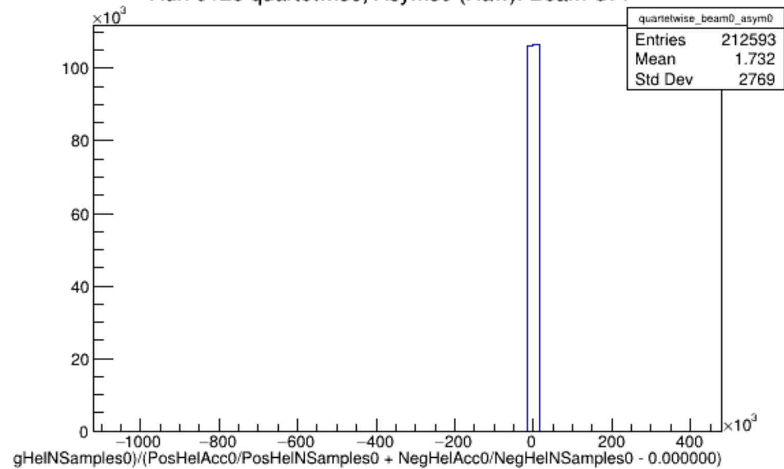
Run 6128 quartetwise, Asyms0 (Raw): Beam OFF
