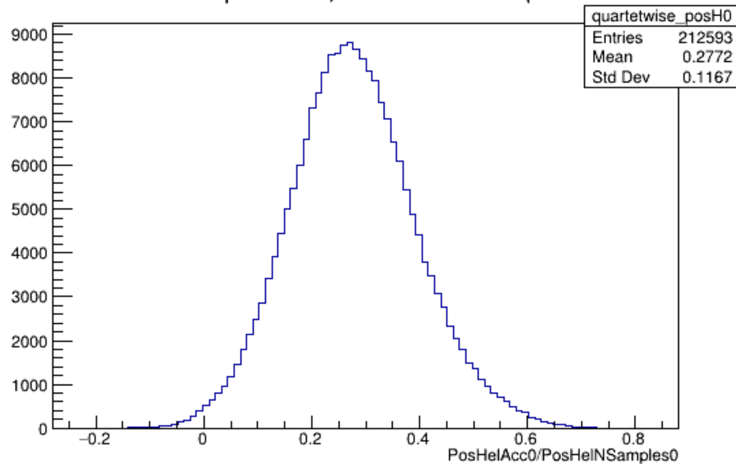
Run 6128 quartetwise, PosHelAcc0/NSamples0: All
