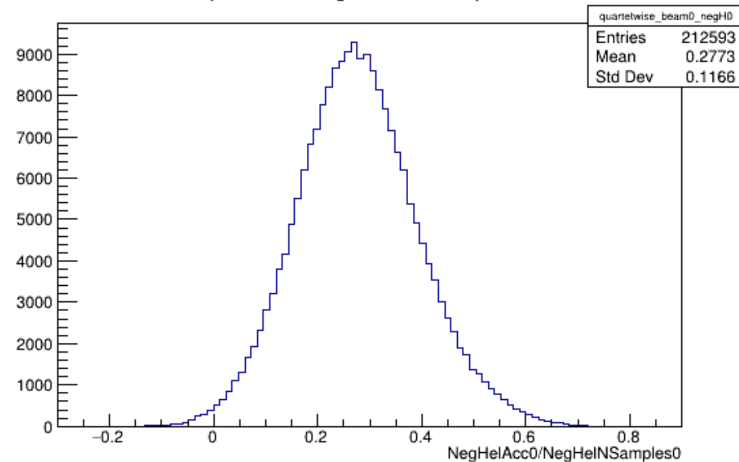
Run 6128 quartetwise, NegHelAcc0/NSamples0: Beam OFF
