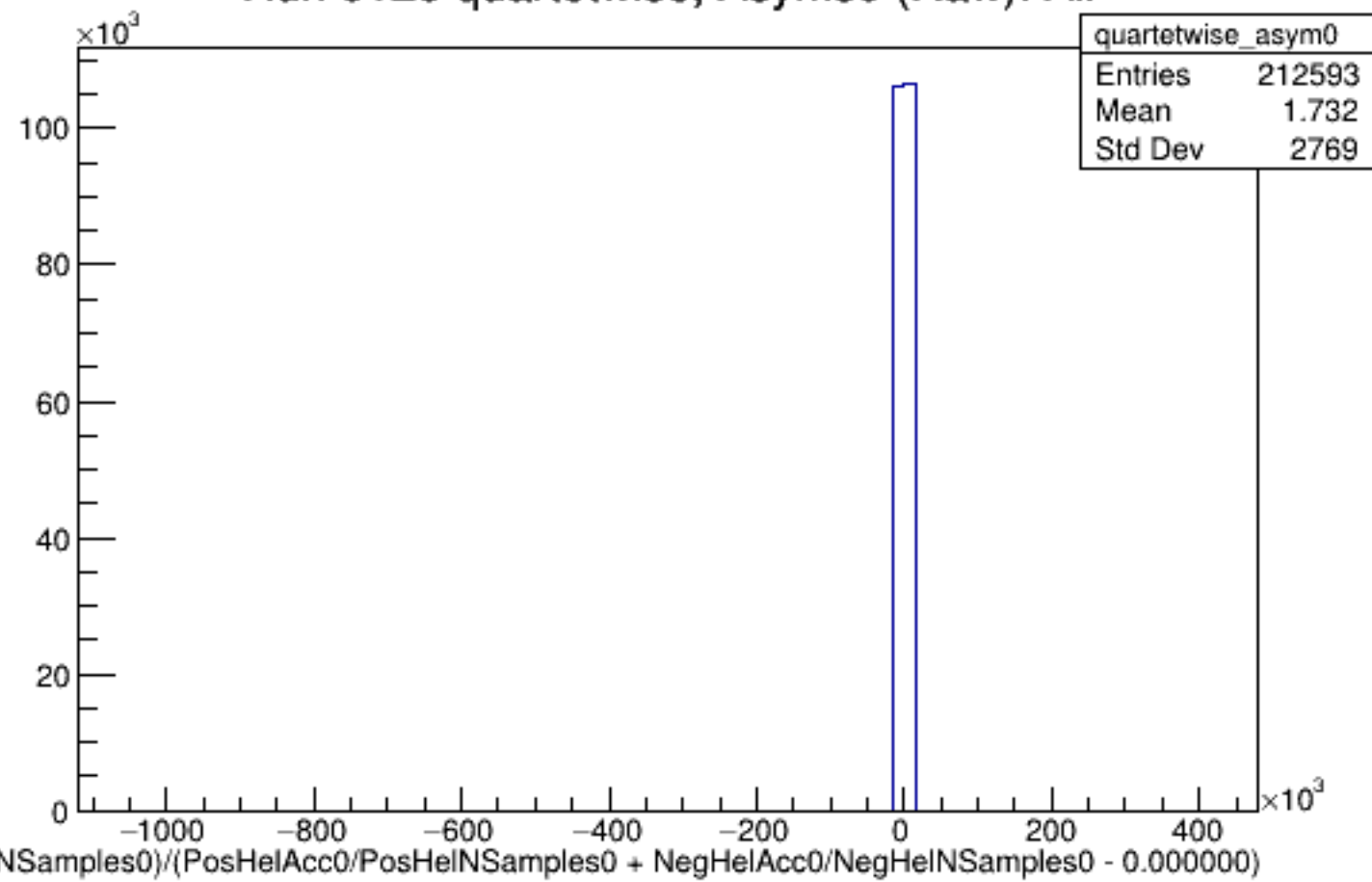
Run 6128 quartetwise, Asyms0 (Raw): All
