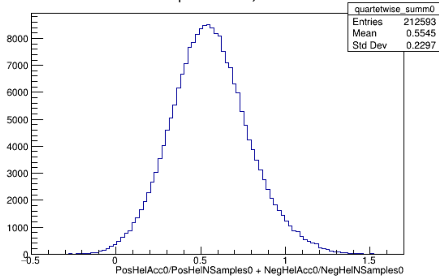
Run 6128 quartetwise, Sums0: All
