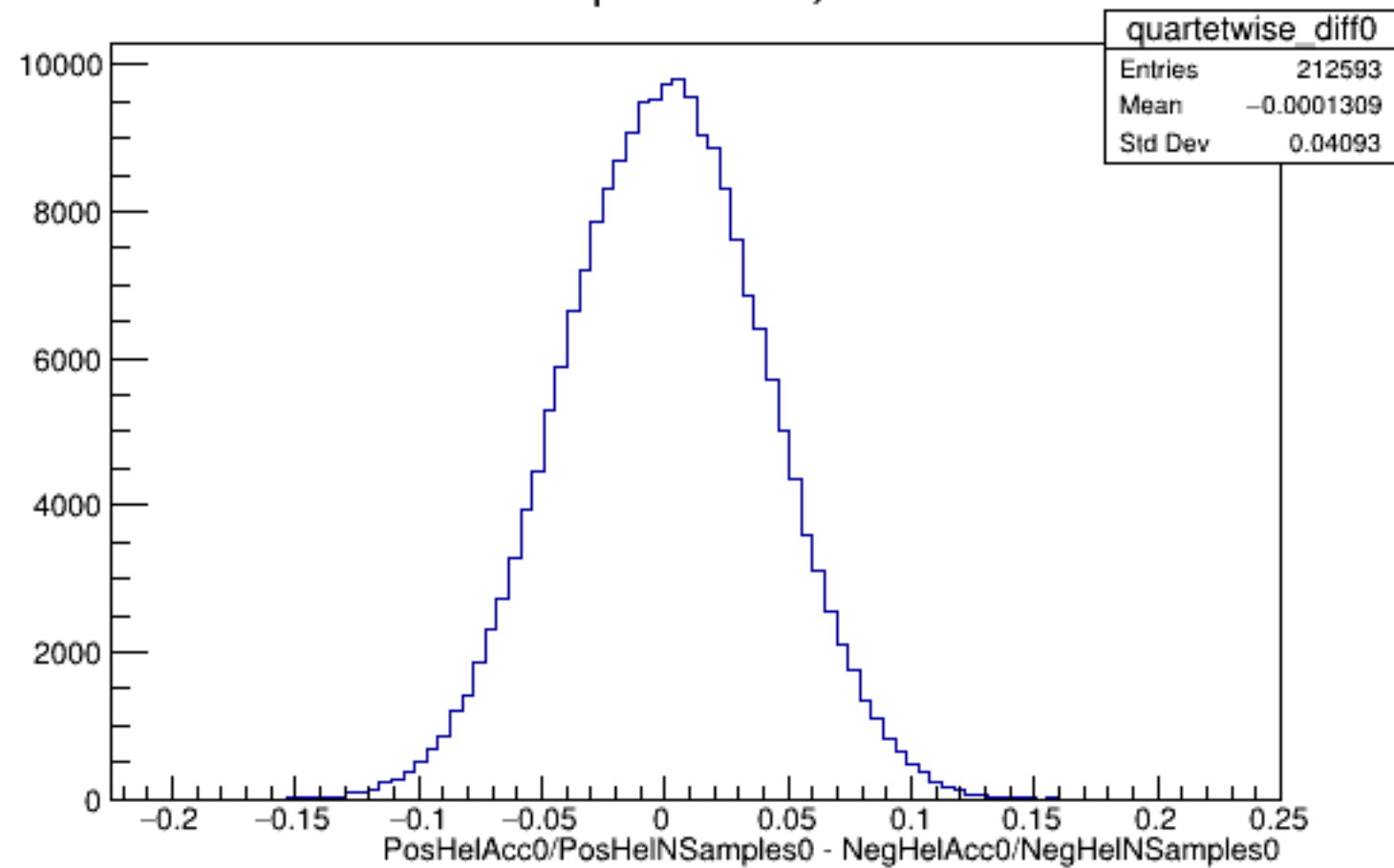
Run 6128 quartetwise, Diffs0: All
