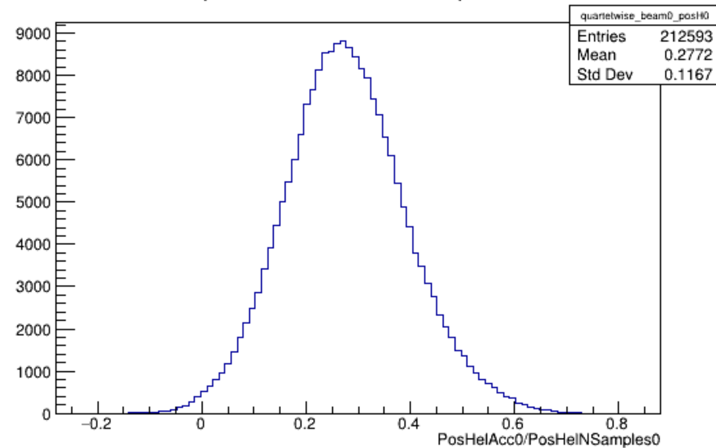
Run 6128 quartetwise, PosHelAcc0/NSamples0: Beam OFF
