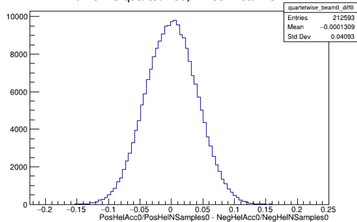
Run 6128 quartetwise, Diffs0: Beam OFF
