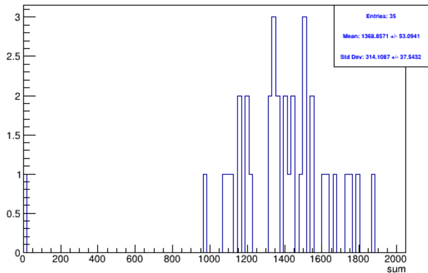
Run 6128 triggerwise, sums: All
