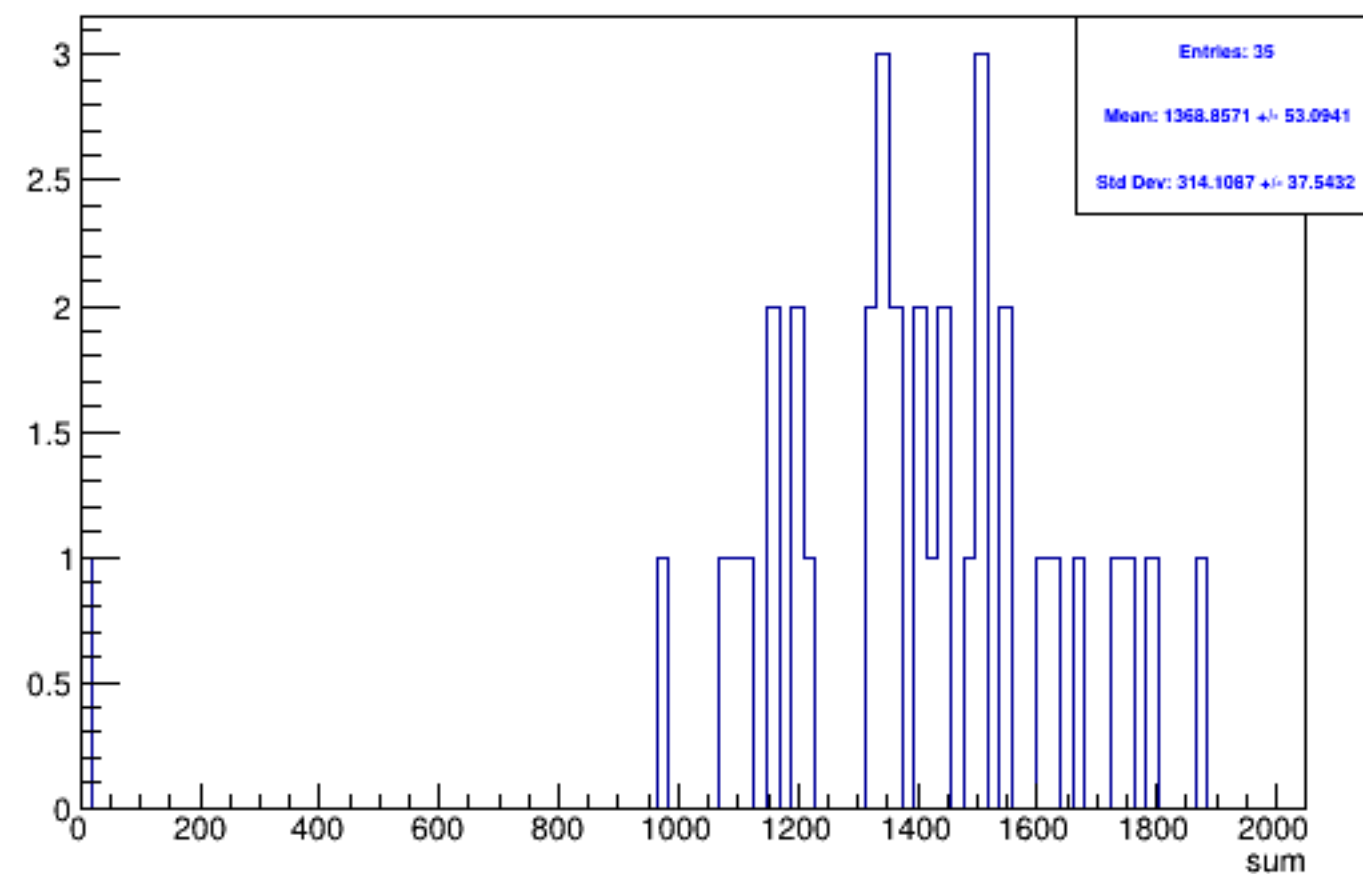
Run 6128 triggerwise, sums: Beam OFF
