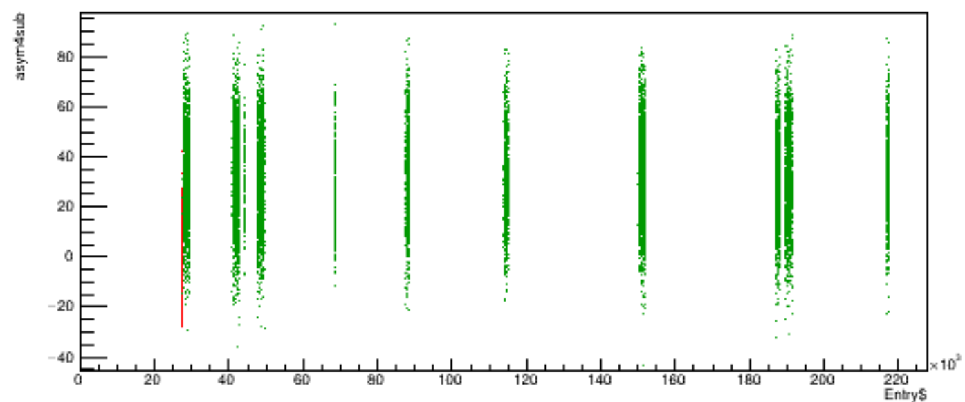
Run 6130 quartetwise, asym4sub vs time
