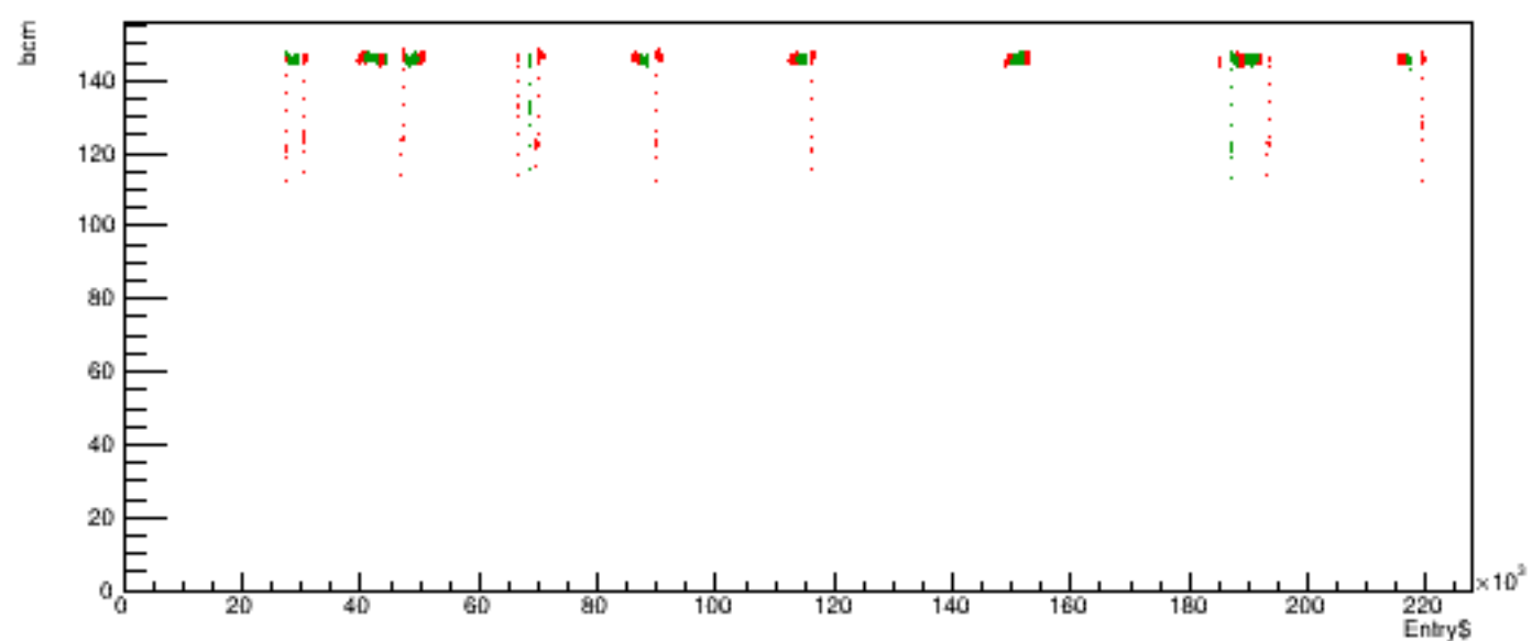
Run 6130 quartetwise, posH4 vs time
