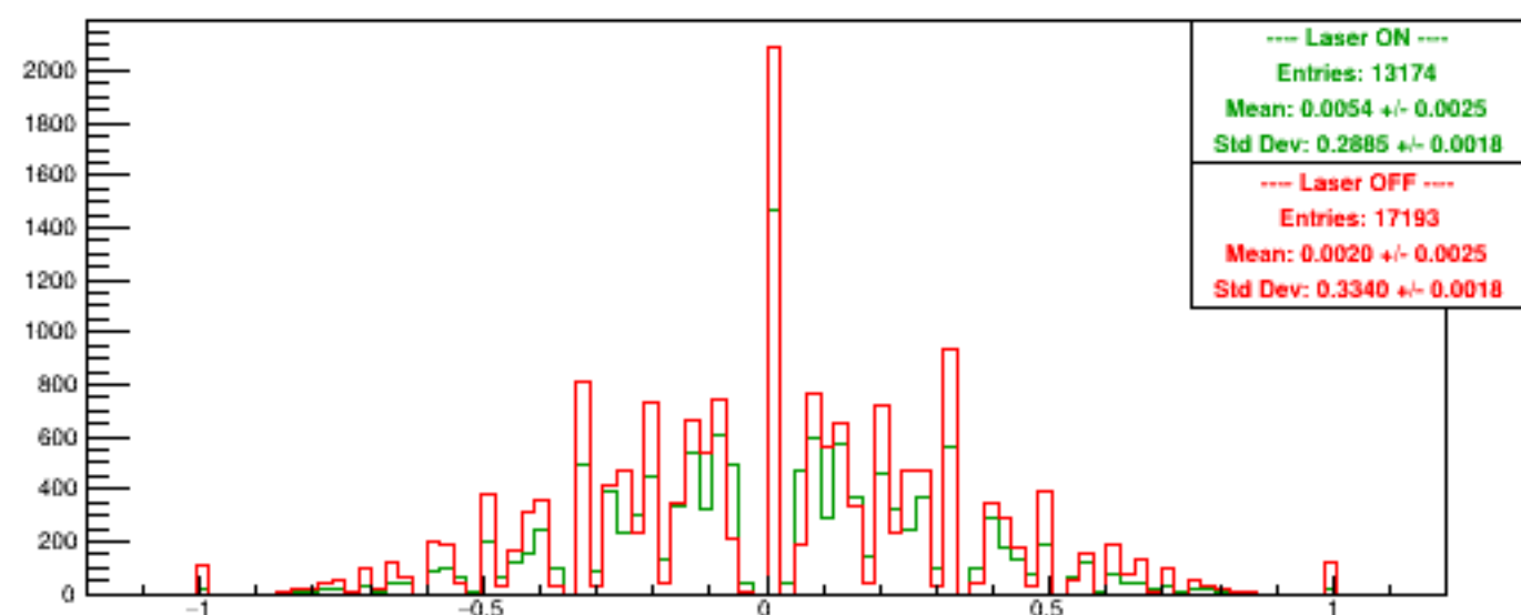
Run 6130 quartetwise, Asyms Horiz Finger
