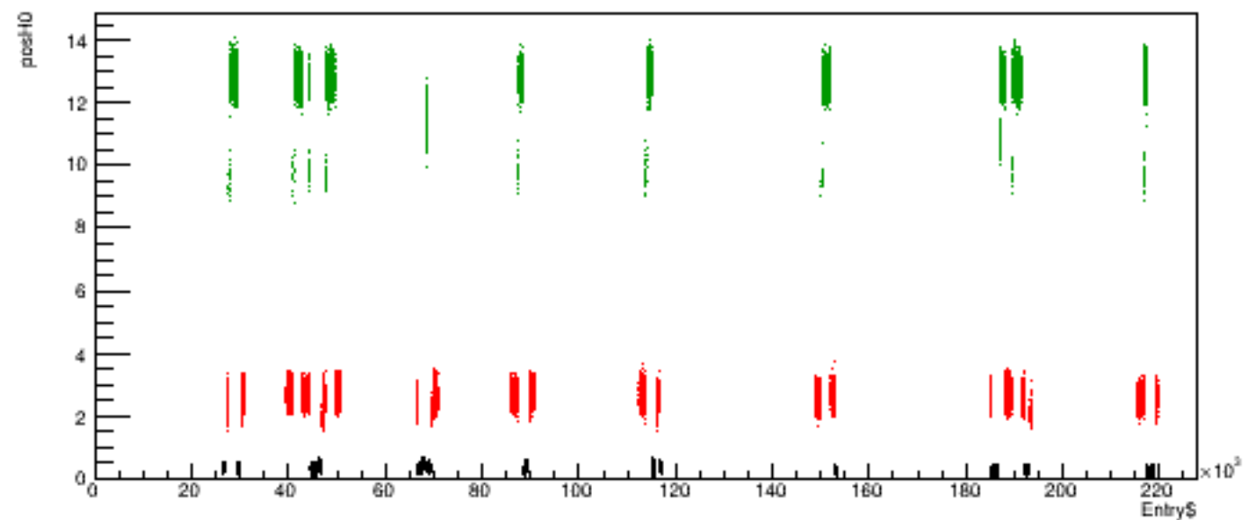
Run 6130 quartetwise, posH0 vs time
