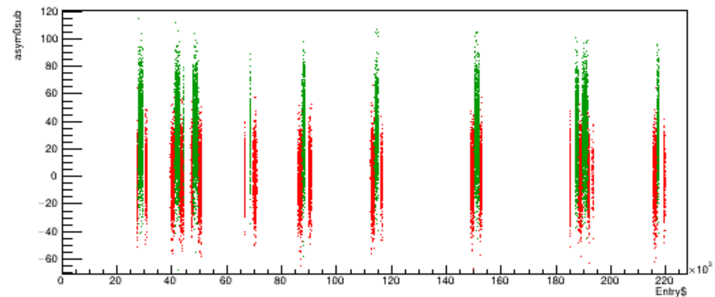
Run 6130 quartetwise, asym0sub vs time
