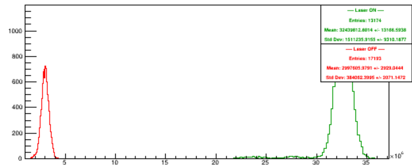
Run 6130 quartetwise, NegHelAcc4
