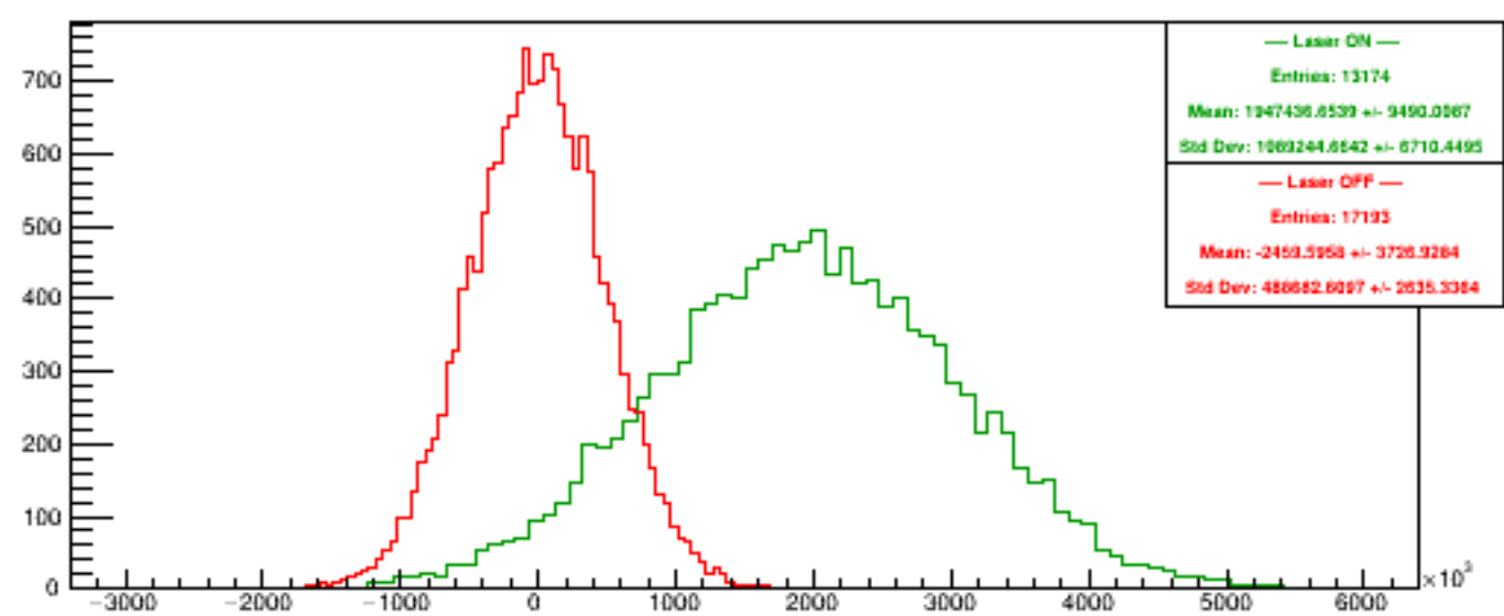
Run 6130 quartetwise, Diffs4
