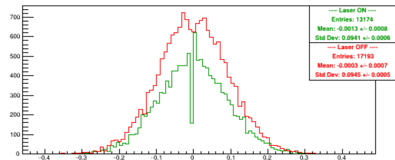
Run 6130 quartetwise, Asyms DSbg1
