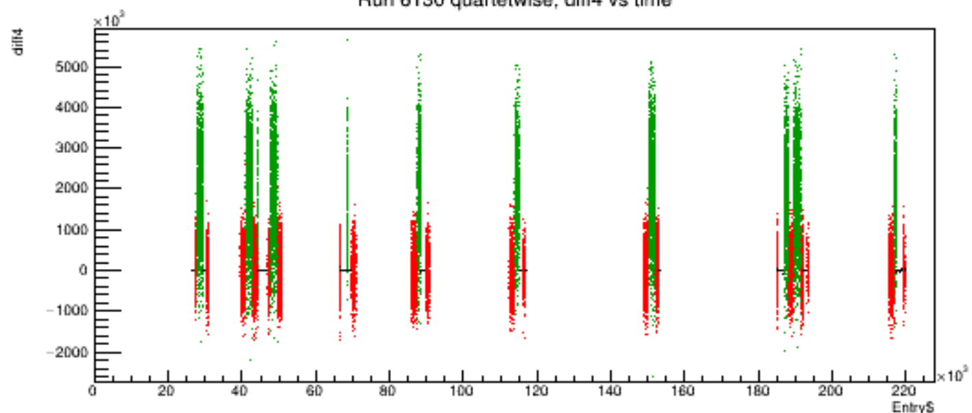
Run 6130 quartetwise, diff4 vs time
