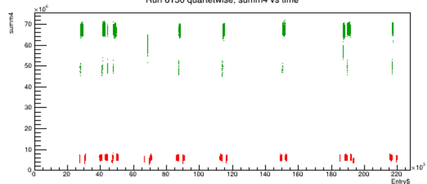
Run 6130 quartetwise, summ4 vs time
