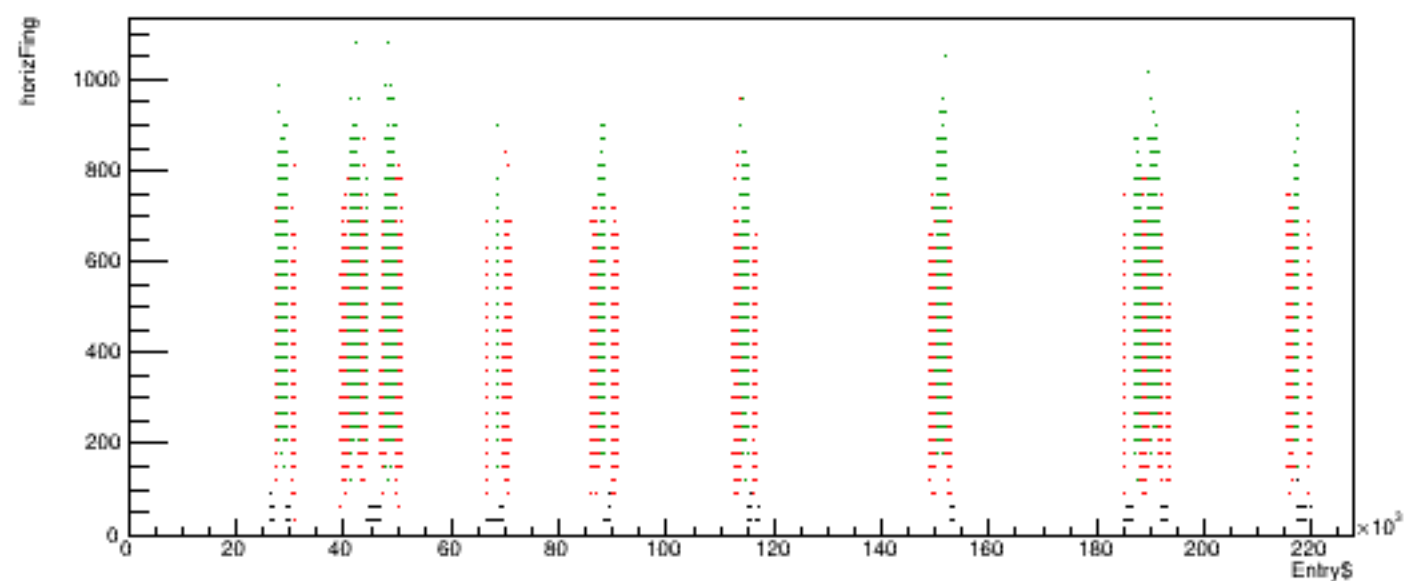
Run 6130 quartetwise, horizFing vs time
