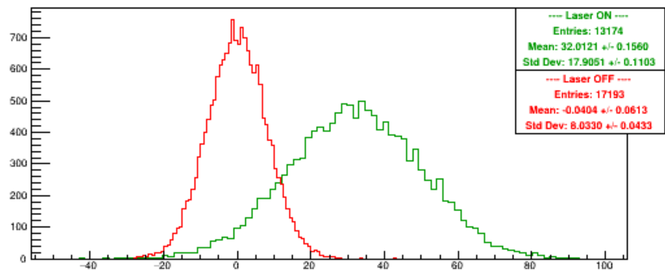
Run 6130 quartetwise, Asyms4
