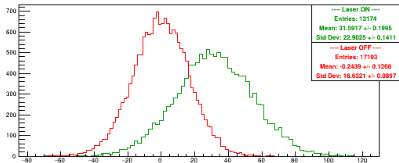
Run 6130 quartetwise, Asyms0
