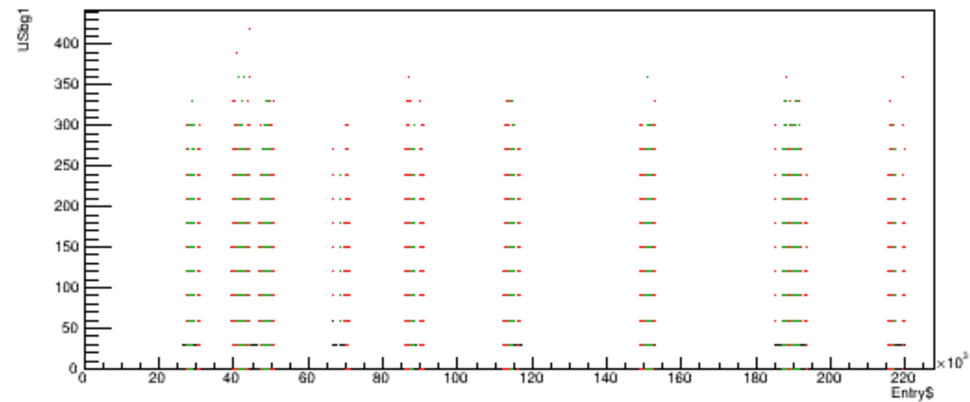
Run 6130 quartetwise, USbg1 vs time
