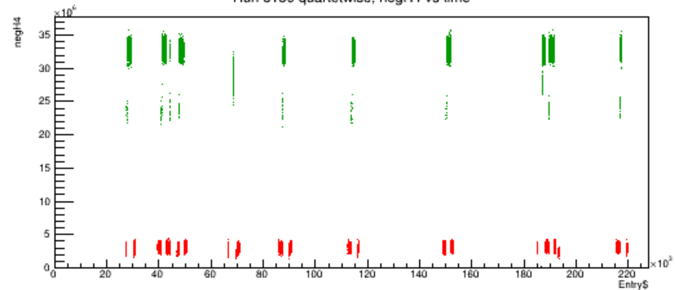
Run 6130 quartetwise, negH4 vs time
