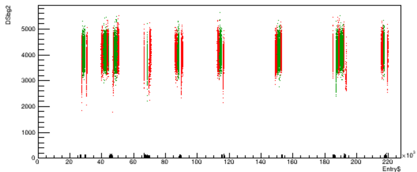
Run 6130 quartetwise, DSbg2 vs time
