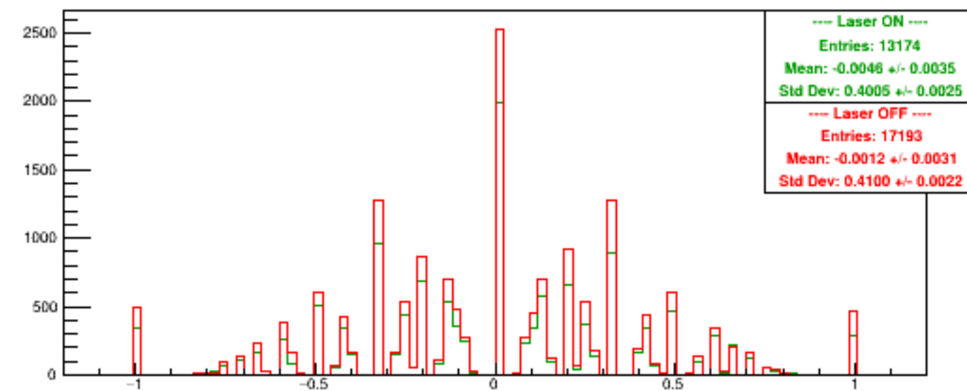
Run 6130 quartetwise, Asyms USbg2
