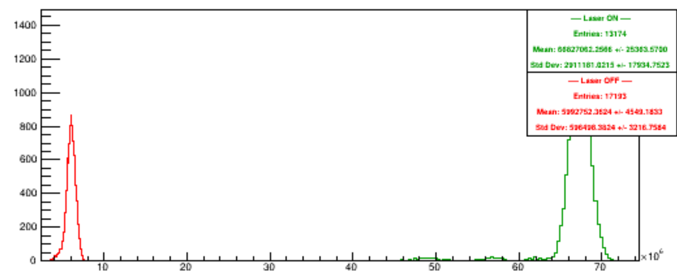
Run 6130 quartetwise, Sums4
