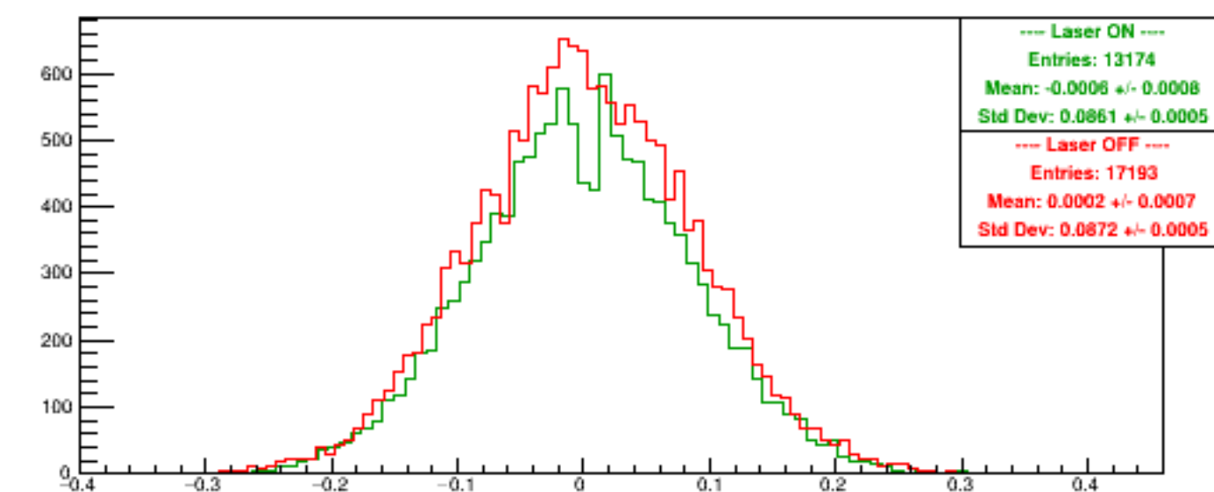
Run 6130 quartetwise, Asyms DSbg2
