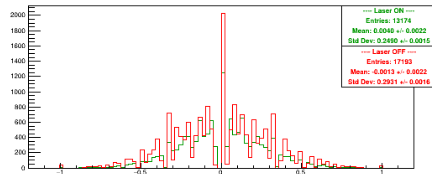
Run 6130 quartetwise, Asyms Vert Finger
