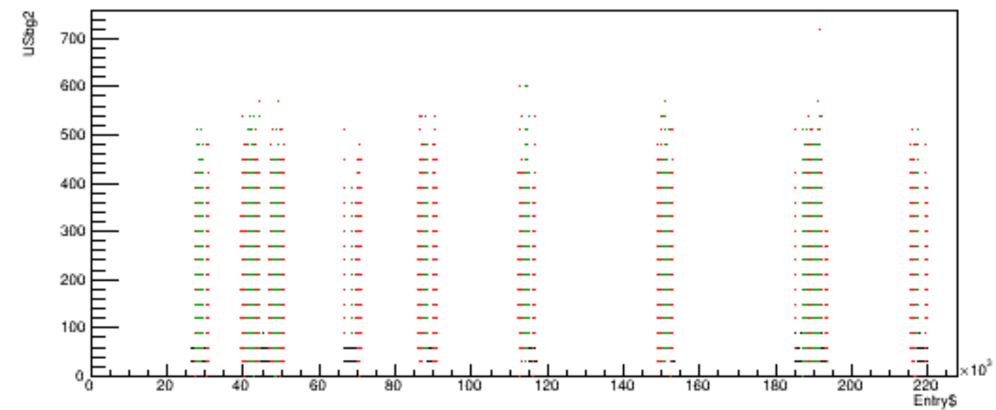
Run 6130 quartetwise, USbg2 vs time
