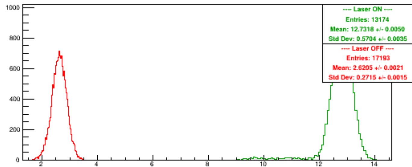
Run 6130 quartetwise, PosHelAcc0/NSamples0
