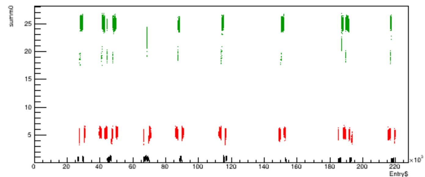
Run 6130 quartetwise, summ0 vs time
