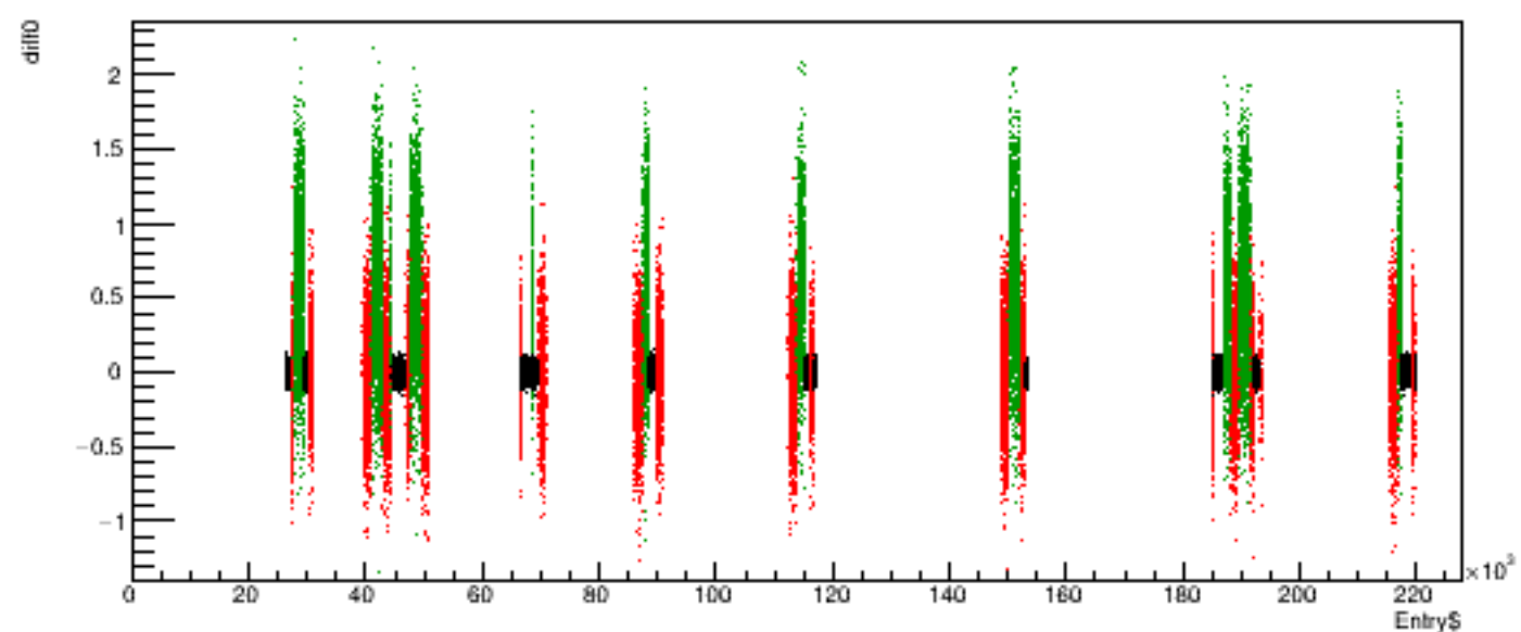
Run 6130 quartetwise, diff0 vs time
