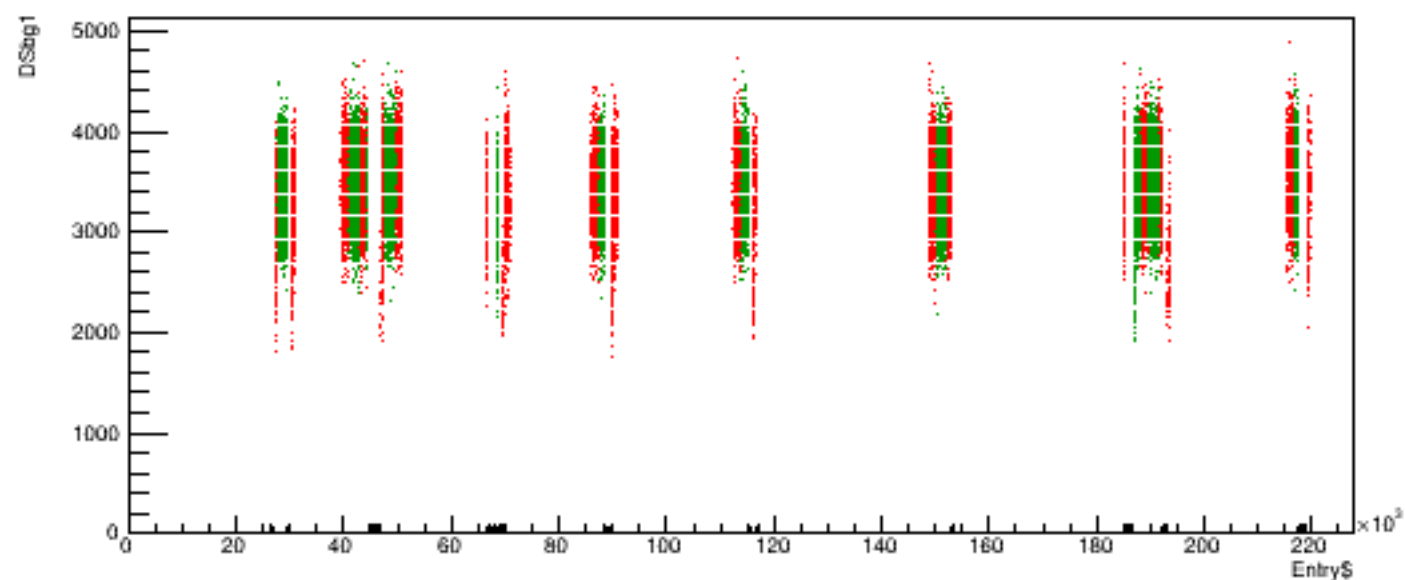
Run 6130 quartetwise, DSbg1 vs time
