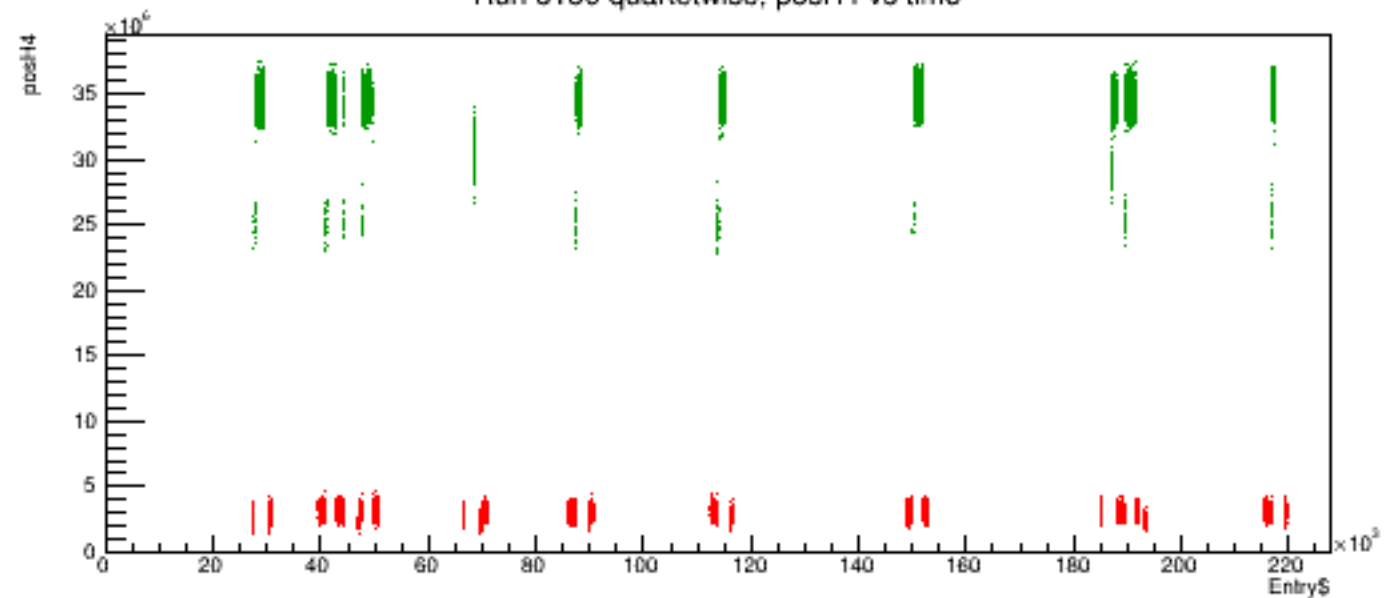
Run 6130 quartetwise, posH4 vs time
