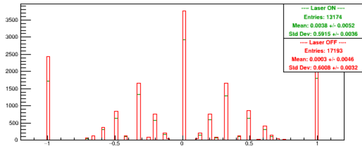
Run 6130 quartetwise, Asyms USbg1
