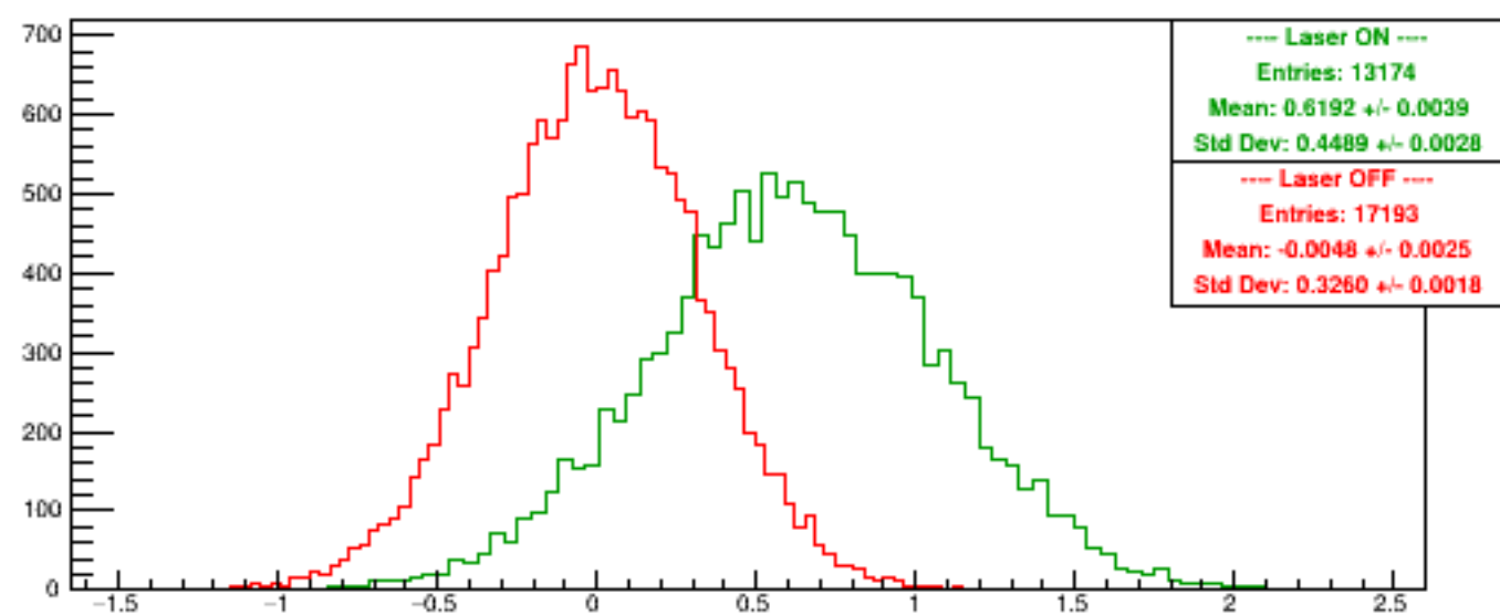
Run 6130 quartetwise, Diffs0
