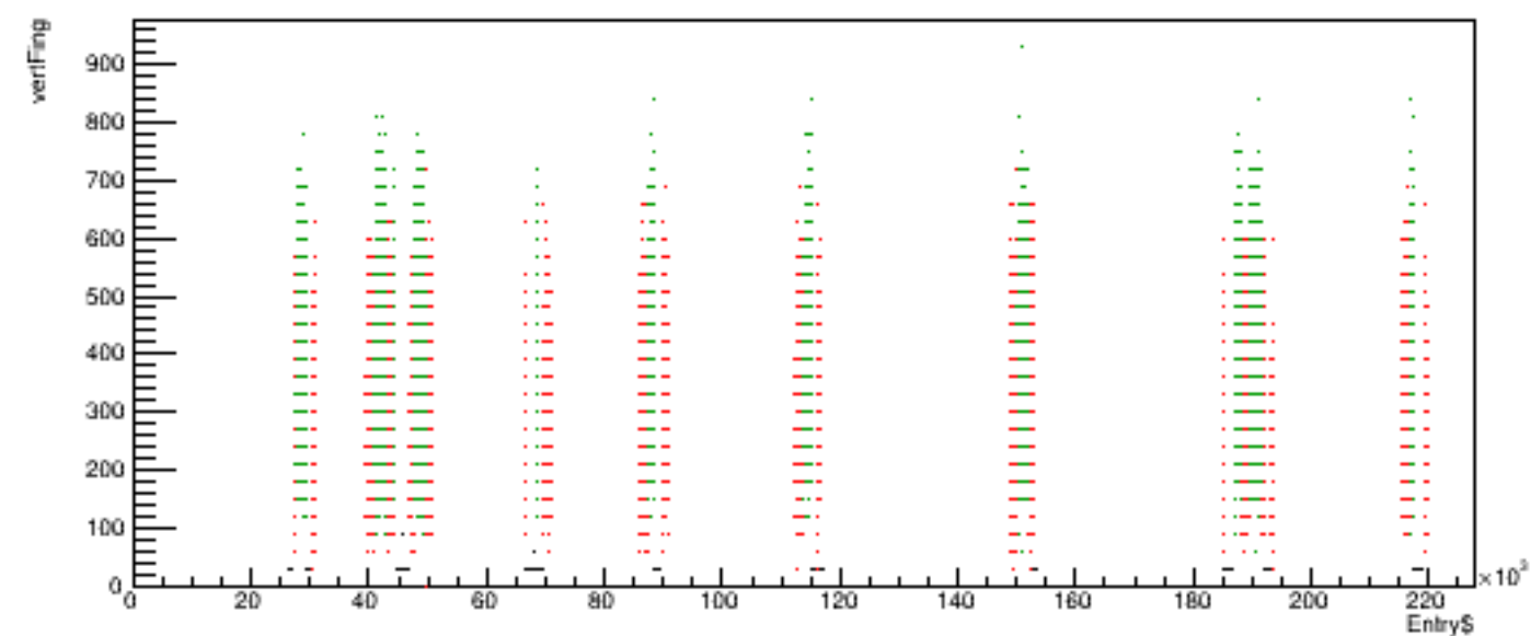
Run 6130 quartetwise, vertFing vs time
