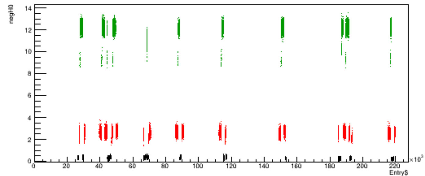
Run 6130 quartetwise, negH0 vs time
