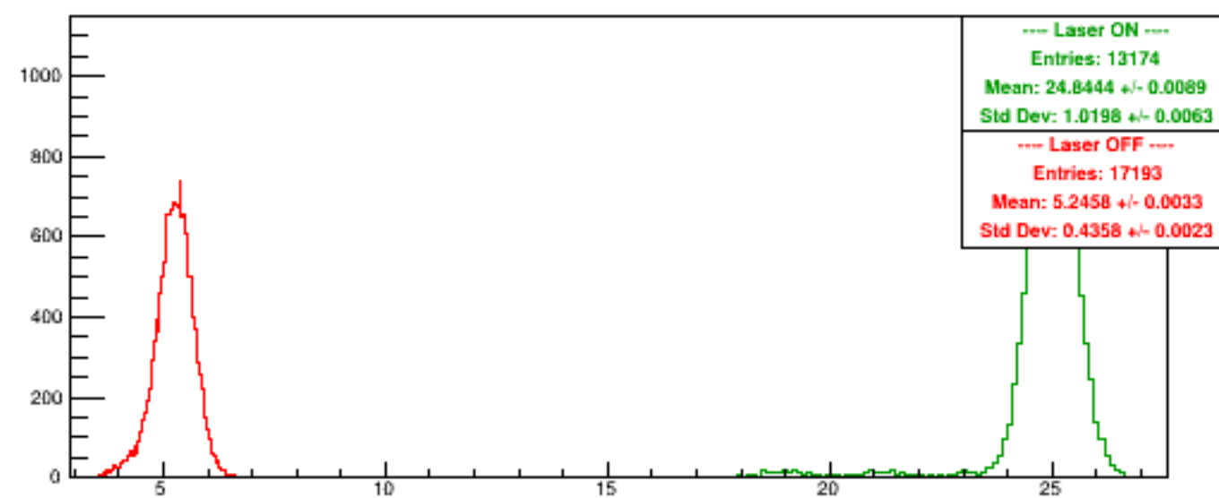
Run 6130 quartetwise, Sums0
