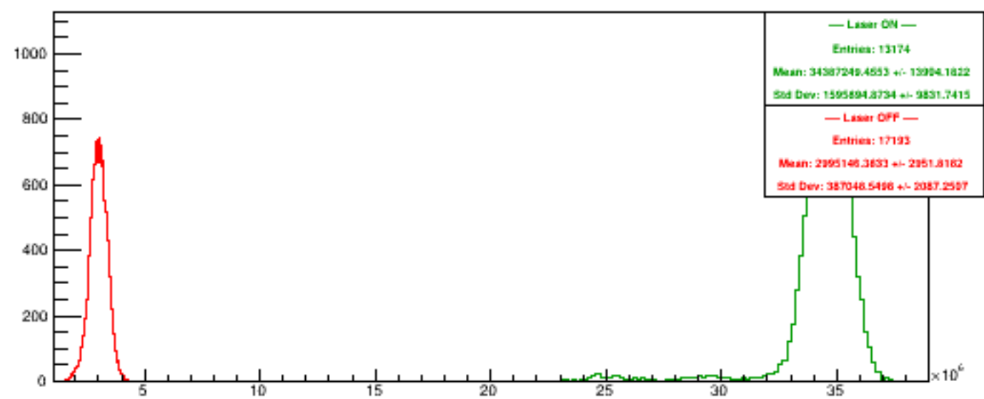
Run 6130 quartetwise, PosHelAcc4
