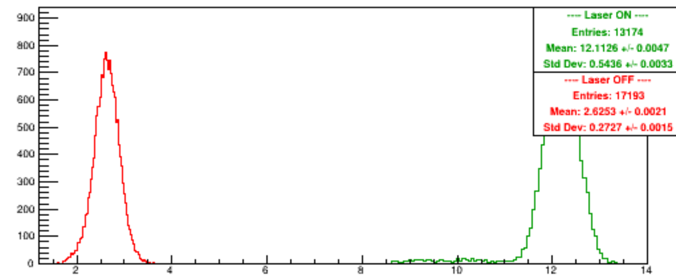
Run 6130 quartetwise, NegHelAcc0/NSamples0
